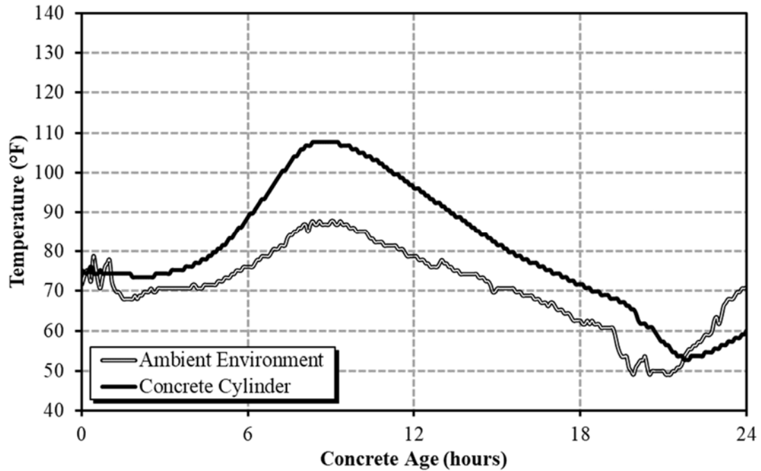
Figure 6-5: Temperature profile for the 11/19/2018 sampling date
