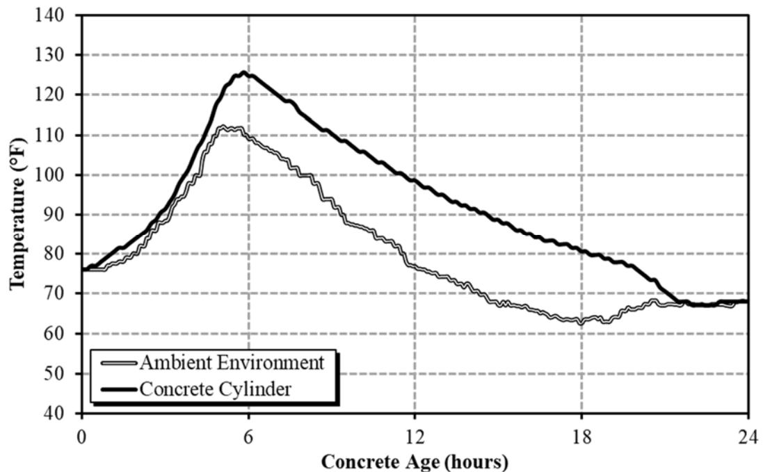
Figure 6-6: Temperature profile for the 04/16/2019 sampling date
