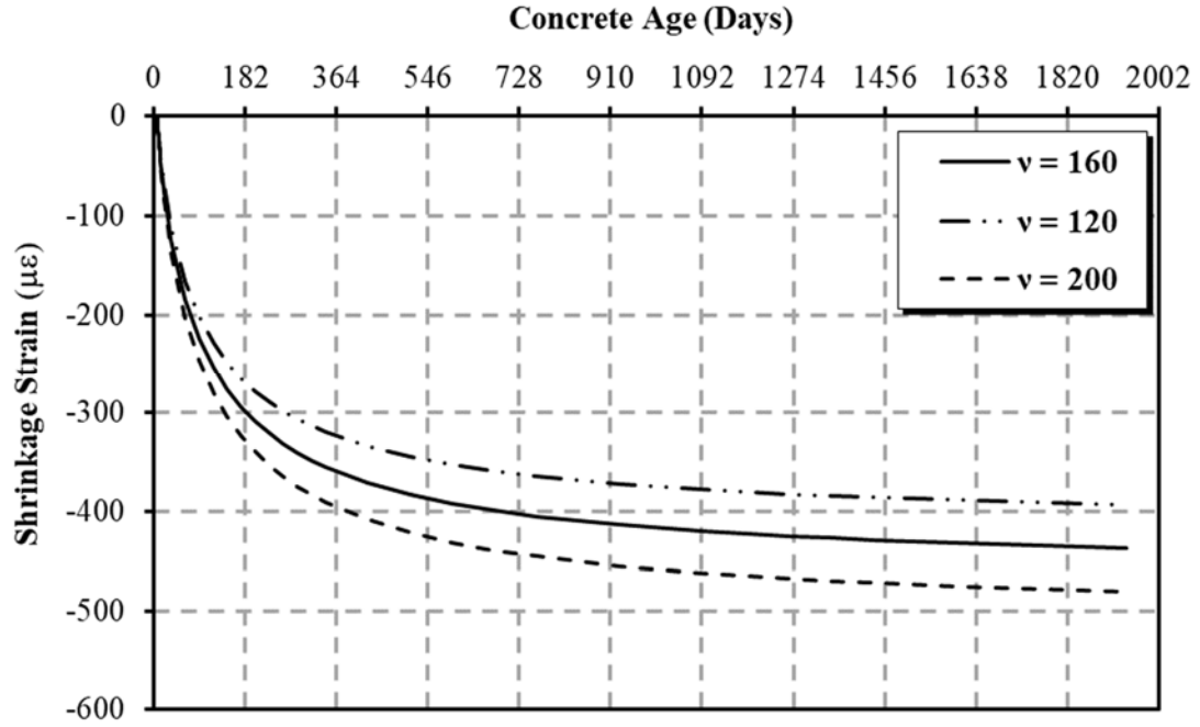
Figure 9-20: Sensitivity of CEB MC 1990 shrinkage with varied \nu
