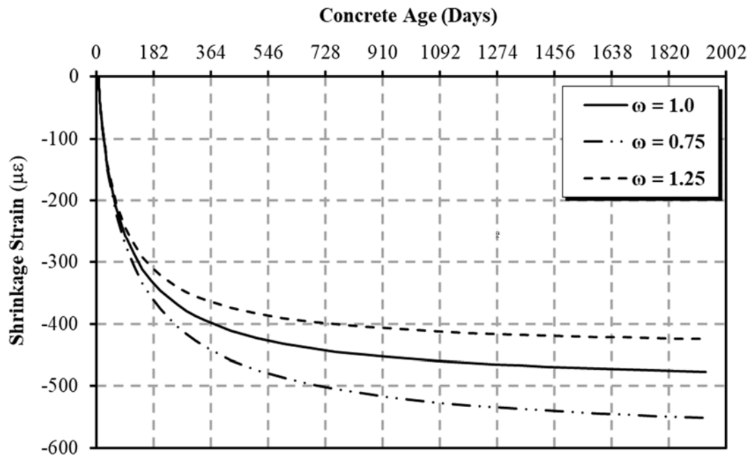
Figure 9-5: Sensitivity of CEB MC 90-99 shrinkage with varied \omega
