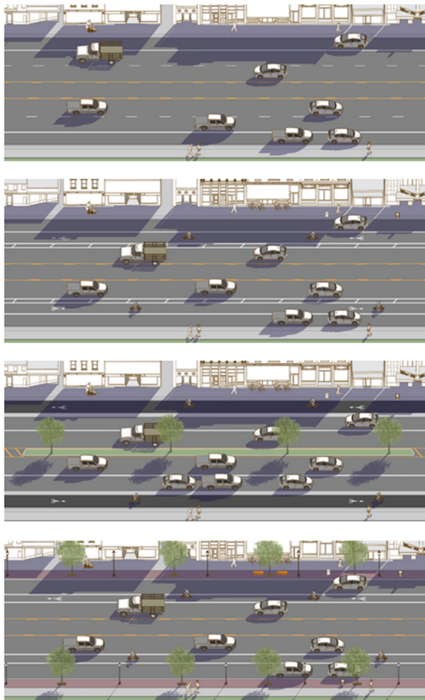
Figure 1. Example of five-lane Main Street (top picture) conversions to Road Diet with Bike Lanes (2nd from top); Median and Separated Bike Lanes (3rd); Streetscape Expansion with Bike Lanes (bottom). (source: FHWA's Small Town & Rural Multimodal Networks)
