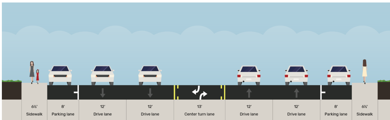
Figure 13. Cross section diagram of US-64 Business / W Broadway Avenue in Farmington, NM.
