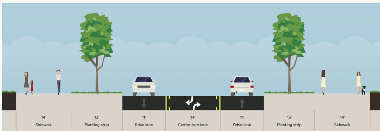
Figure 45. Cross section diagram of design recommendations with no bike lanes or on-street parking (assuming 90' from outside of sidewalk to outside of sidewalk).
