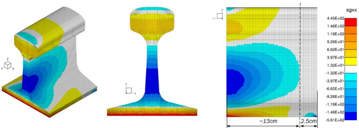
Figure 89. Longitudinal residual stress distribution, 15cm rail model (units MPa)
