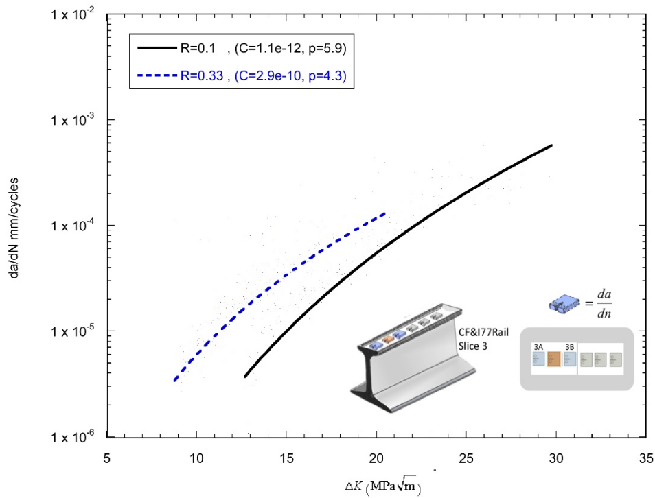
Figure 76. Comparison of horizontal fatigue crack growth rates at two different R -ratios in Slice 3 of CF&I77 rail, R=0.1 and R=0.33
