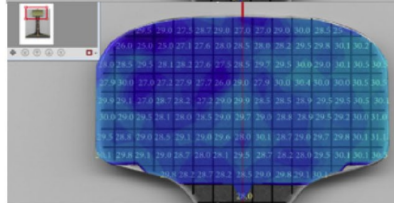
Figure 3. Contour plots showing hardness variation in the railheads using the same HRC scale
