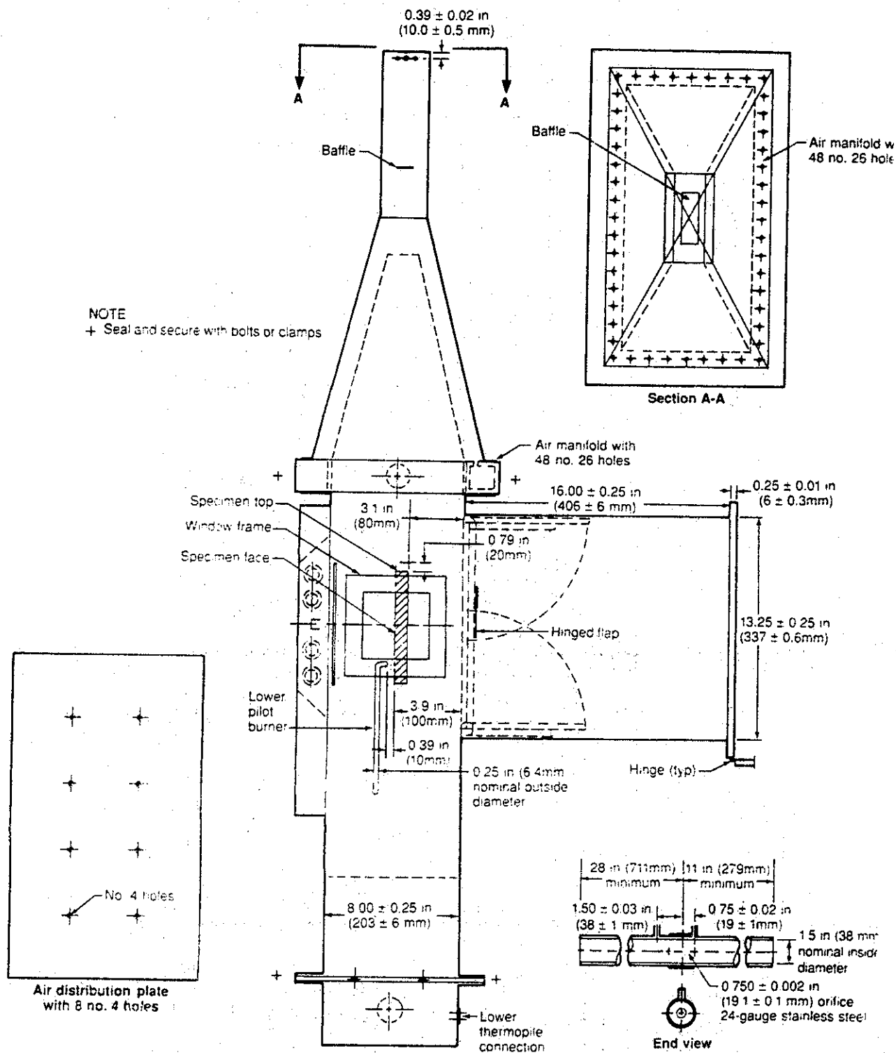
Figure 1B Rate of Heat Release Apparatus
