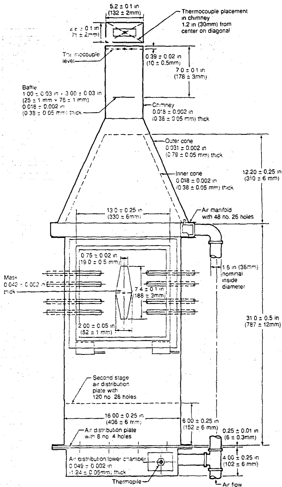
Figure 1A Rate of Heat Release Apparatus
