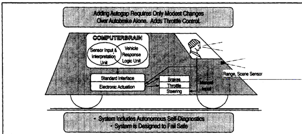
Figure 16. Autobrake and autogap Mechanization Intelligent Cruise Control
