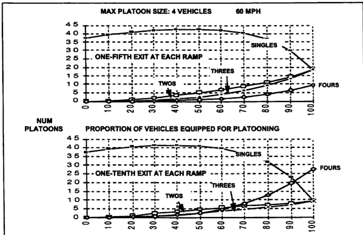
Figure 26. 1-8n. Flow 838 Function of Proportion of vehicles Equipped with the Autoplatoon Feature
