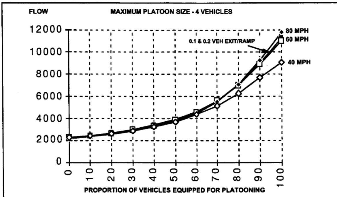
Figure 26. 1-8n. Flow 838 Function of Proportion of vehicles Equipped with the Autoplatoon Feature
