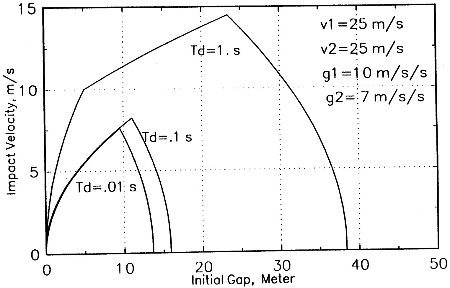
Figure 3.9. Impact Velocity vs. Initial Gap
