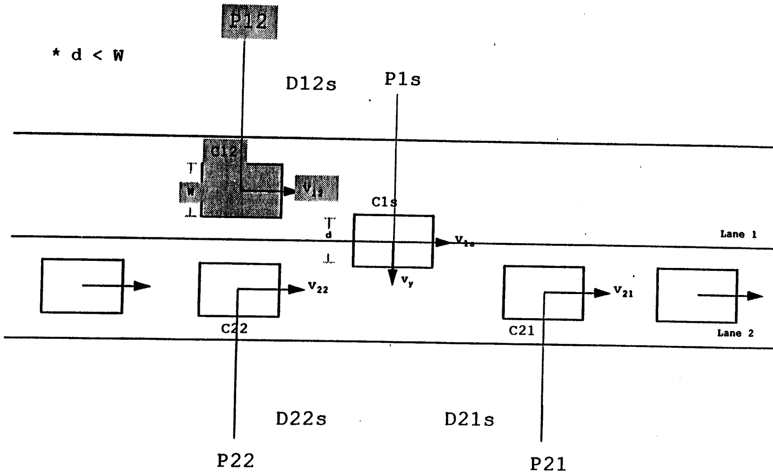
Figure 4.2a. Lane Change Maneuver Config 1: Left to Right - 1/5
