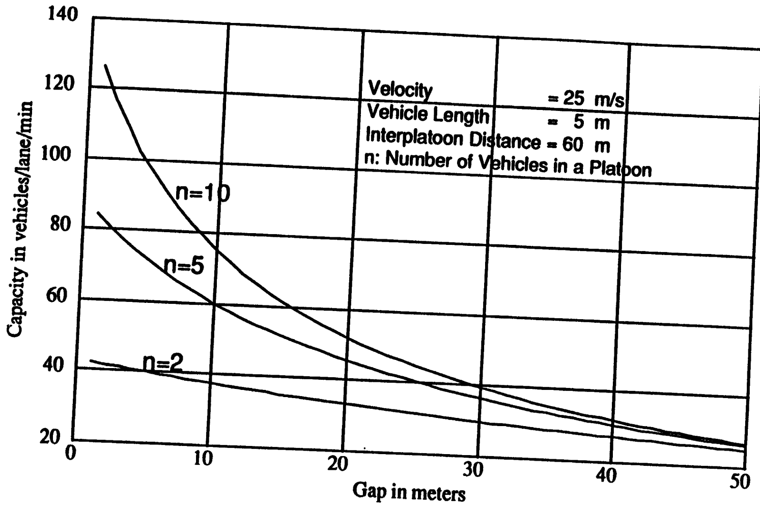
Figure 3.5. Capacity vs Gap
