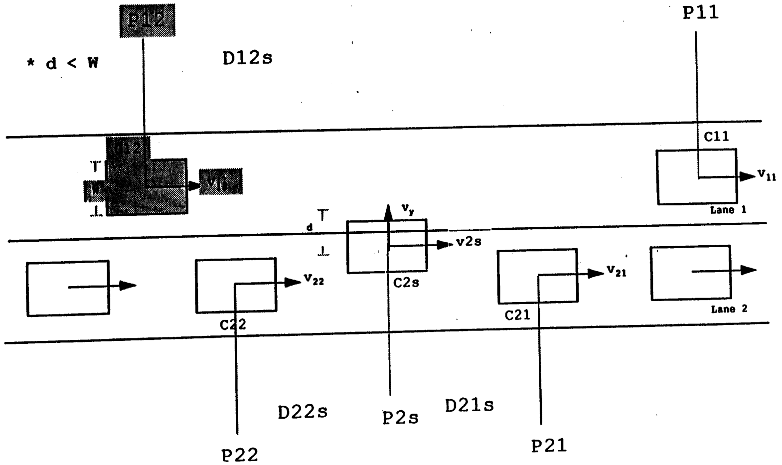
Figure 4.2g. Lane Change Maneuver Config 2: Right to Left - 2/5
