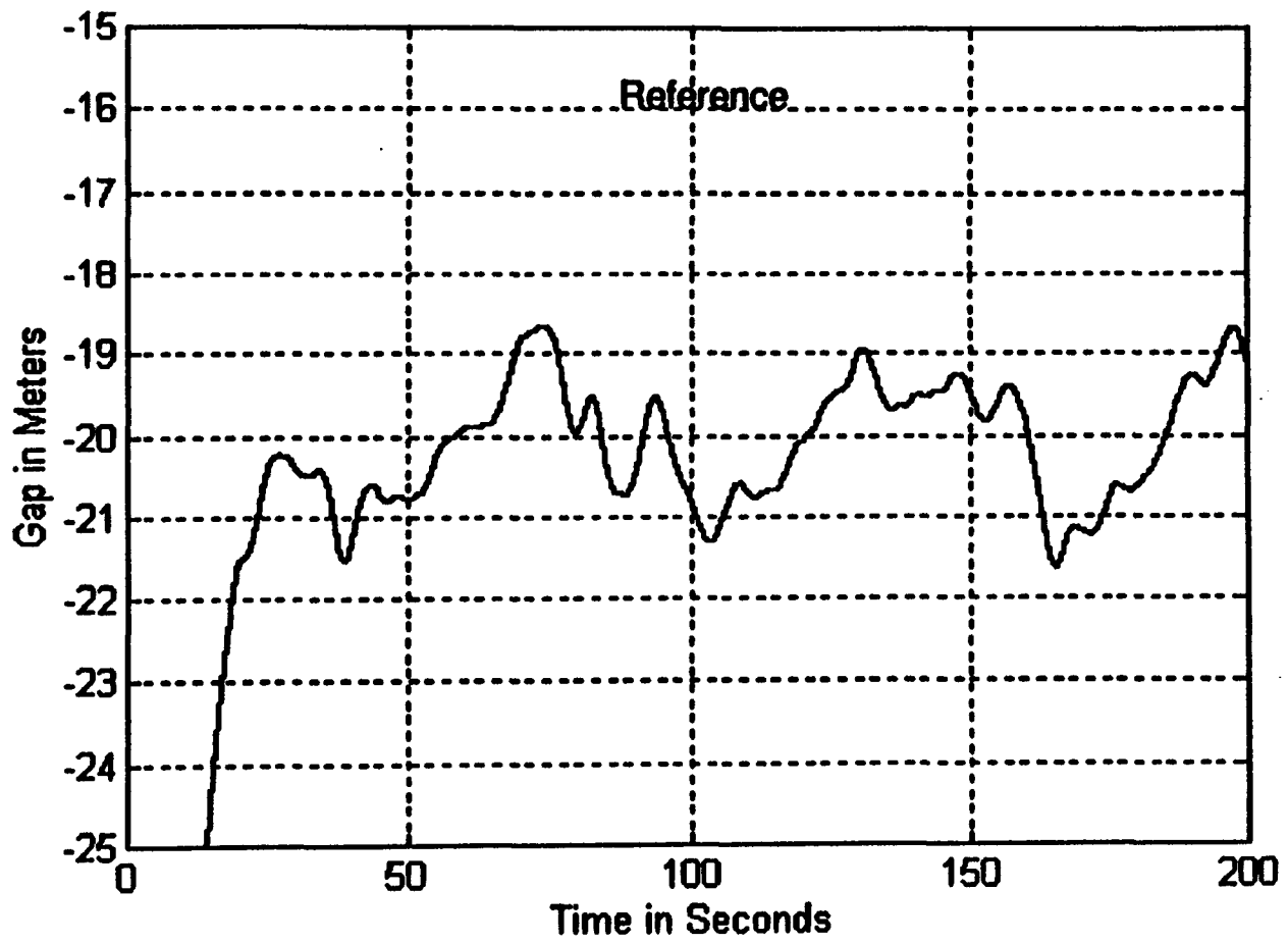
Figure 3.14. 20m Headway Maintenance
