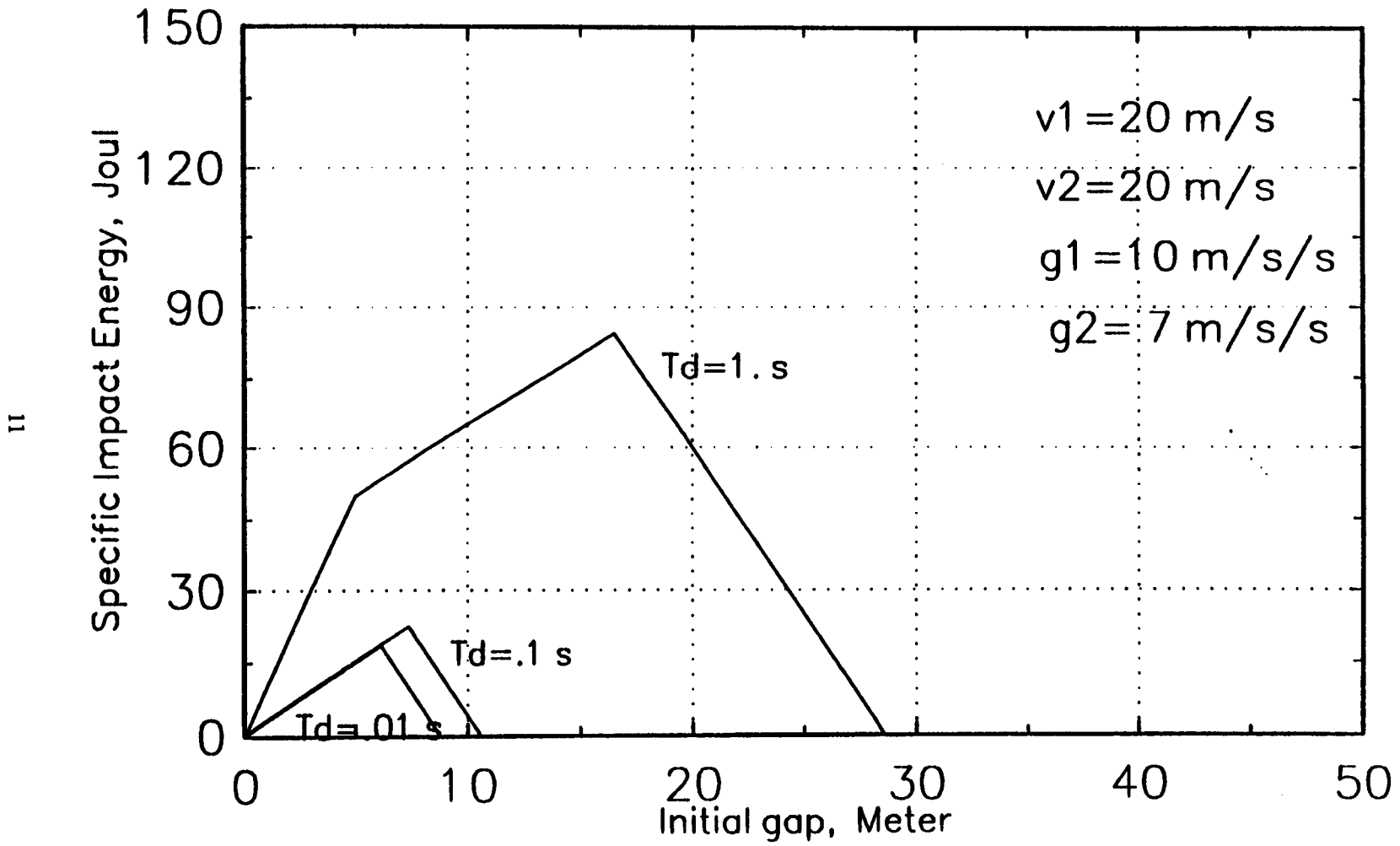
Figure 3.7. Impact Energy vs. Initial Gap
