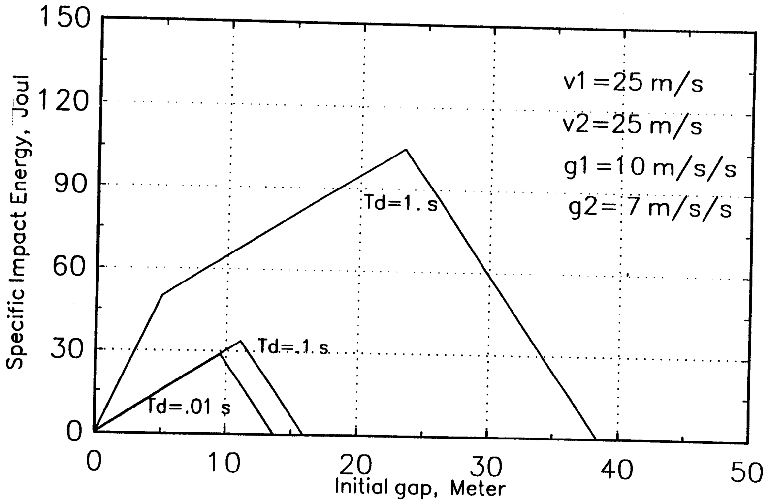
Figure 3.6. Impact Energy vs. Initial Gap
