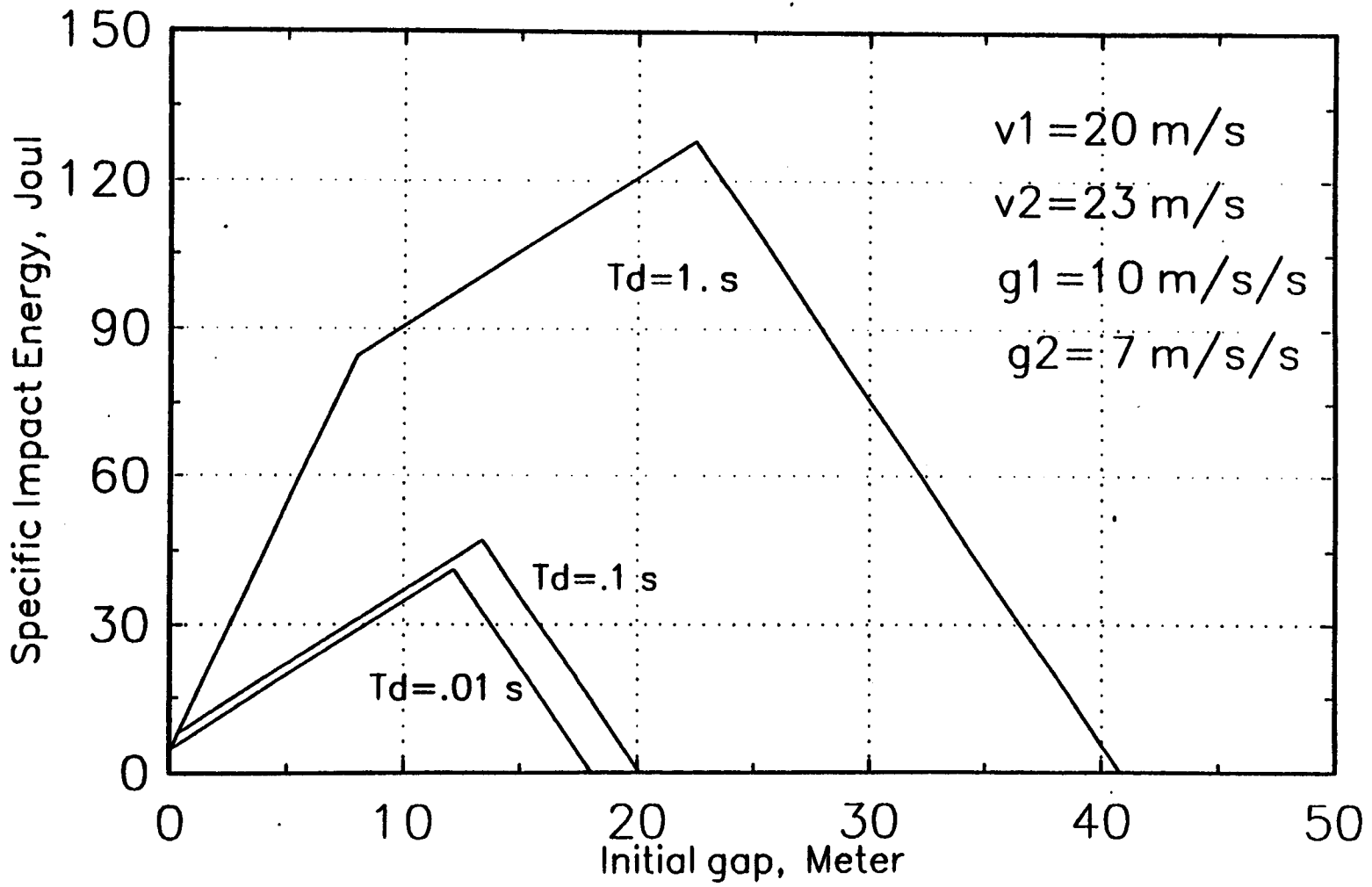
Figure 3.8. Impact Energy vs. Initial Gap
