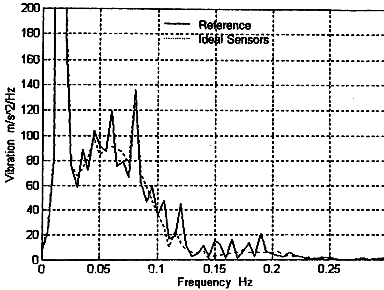
Figure 3.15. Ride Comfort of 5m Platoon
