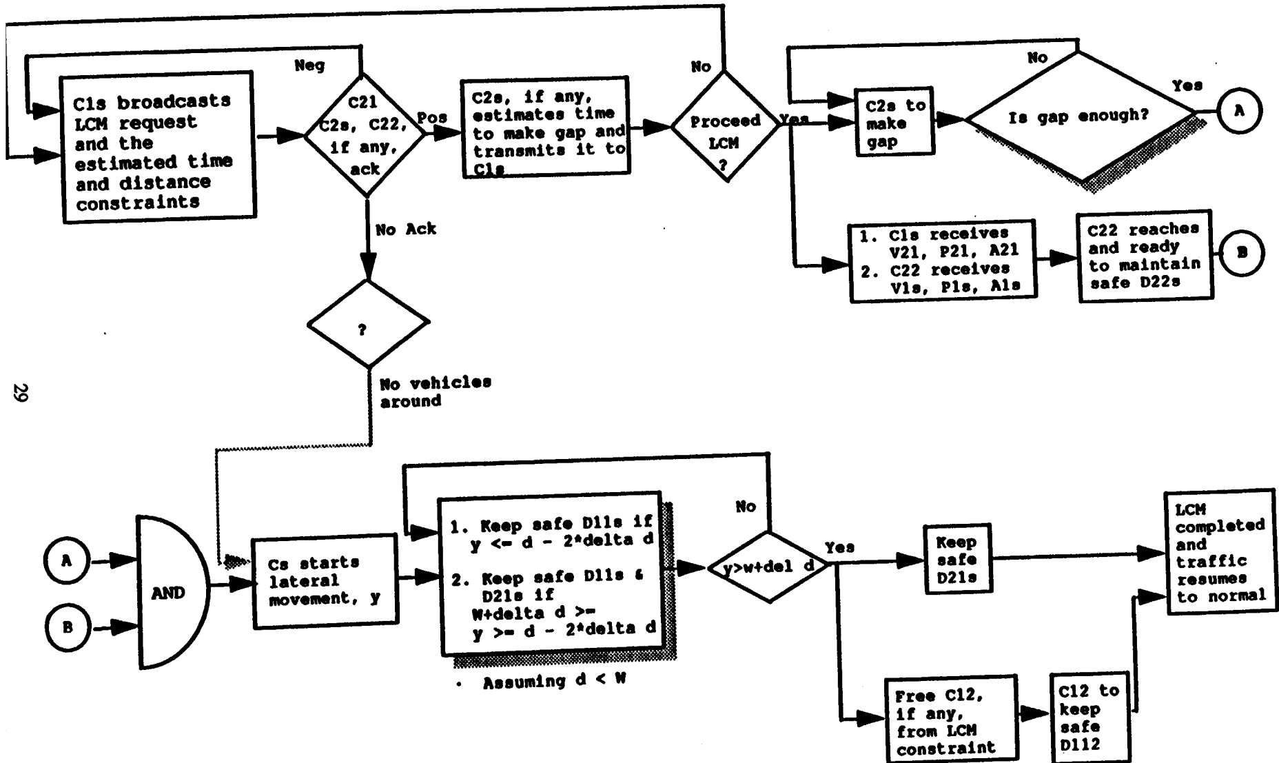
Figure 4.1. Lane Change Maneuver Flow Block Diagram
