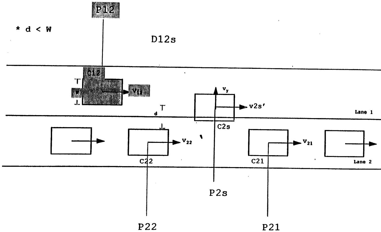
Figure 4.2i. Lane Change Maneuver Config 2: Right to Left - 4/5
