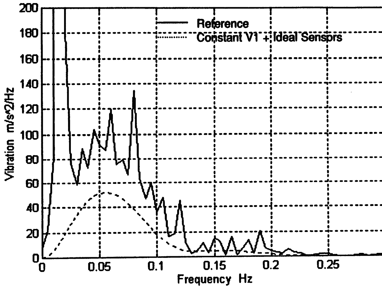
Figure 3.13. Ride Comfort of 5m Platoon
