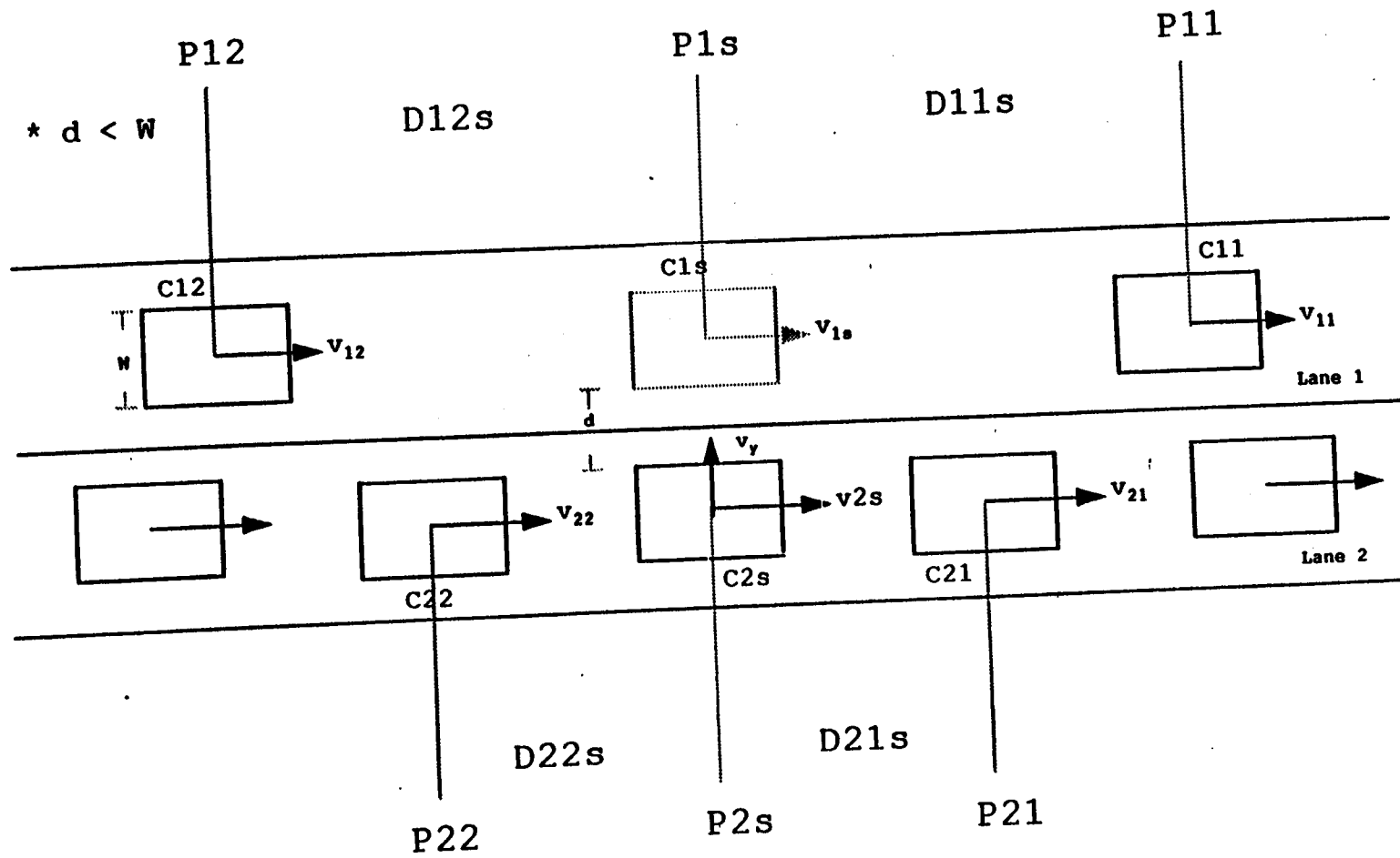
Figure 4.2f. Lane Change Maneuver Config 2: Right to Left - 1/5
