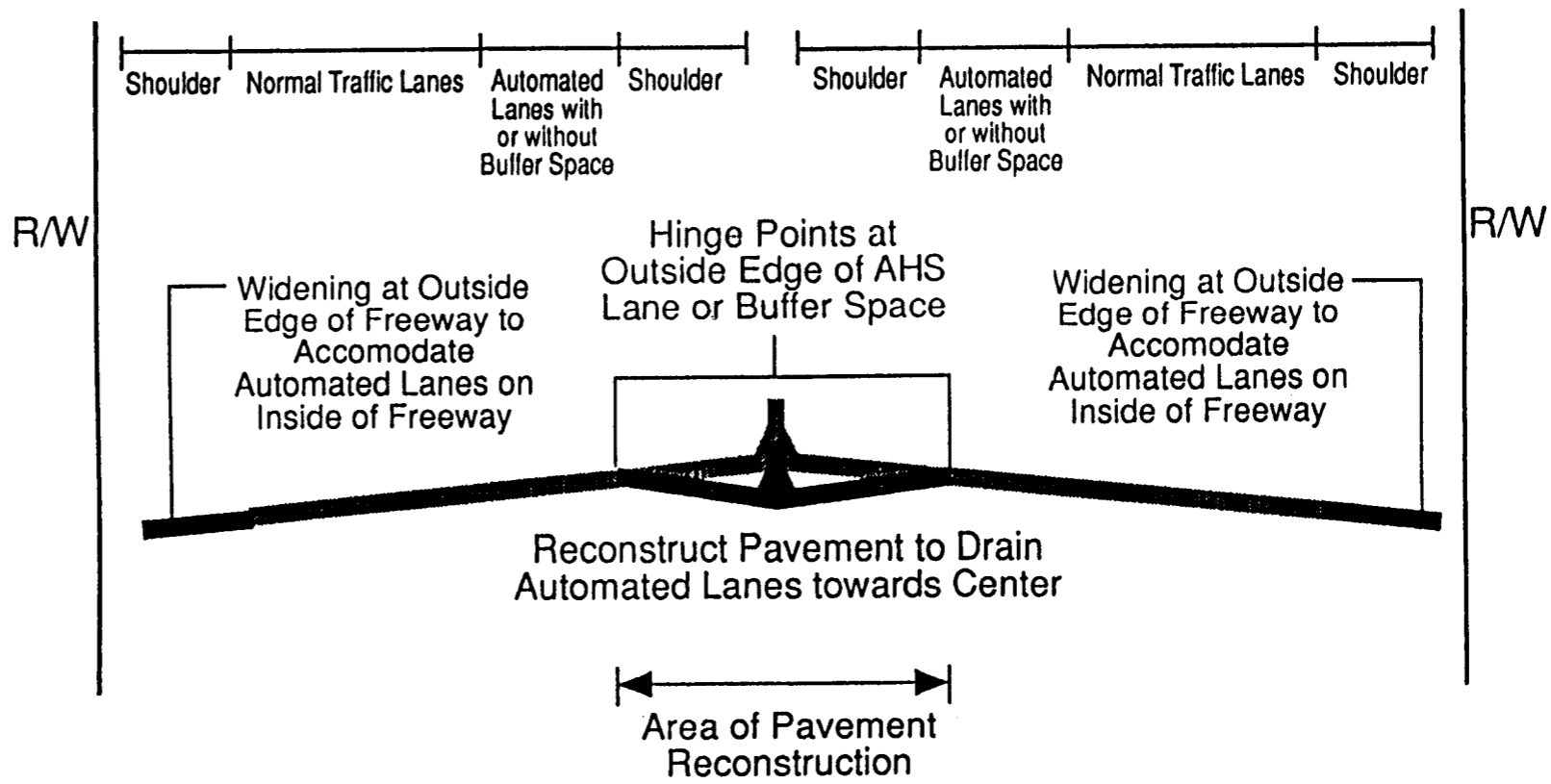
Figure 27. Impact of introducing inside AHS lanes with center drainage.
