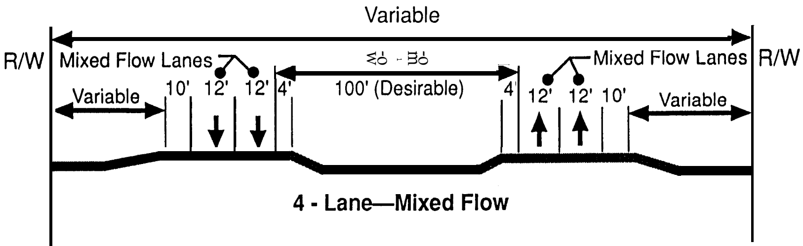
Figure 15. Cross section. RSC 4.
