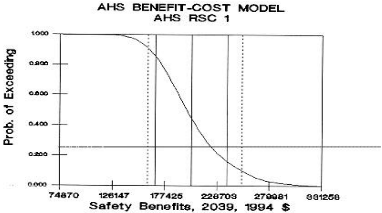
Figure 32. Distribution Function Of Year 2039 Safety Benefits
