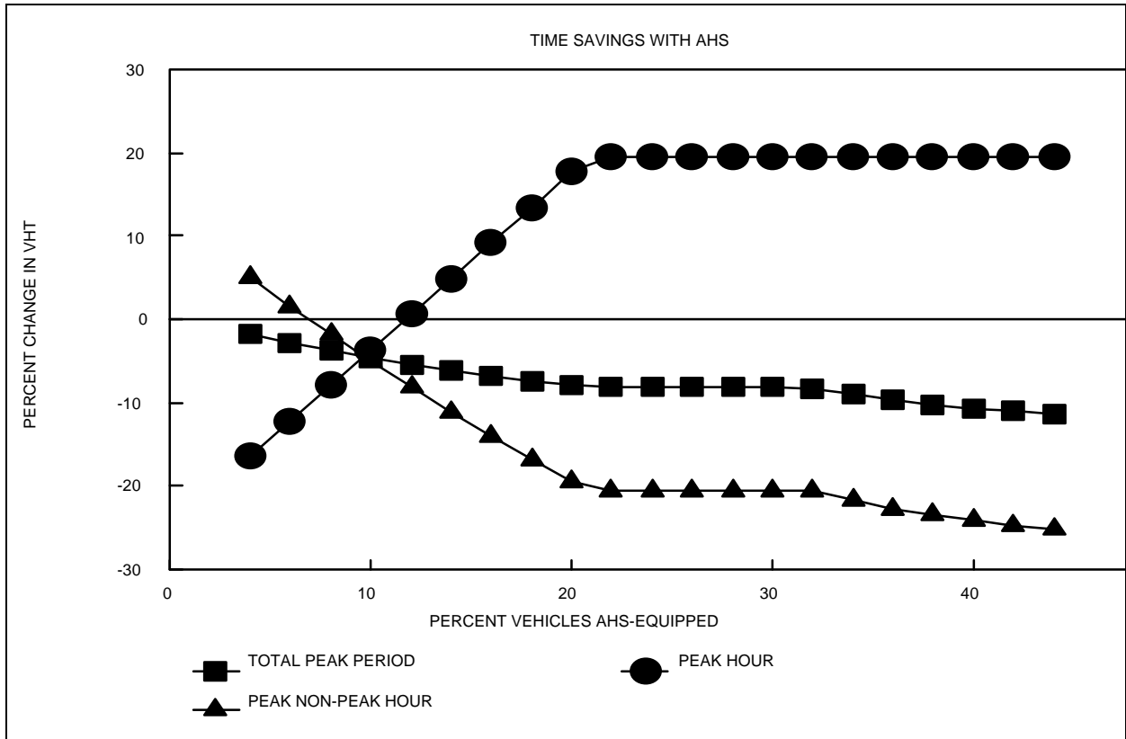
Figure 3. Time Savings And AHS Penetration
