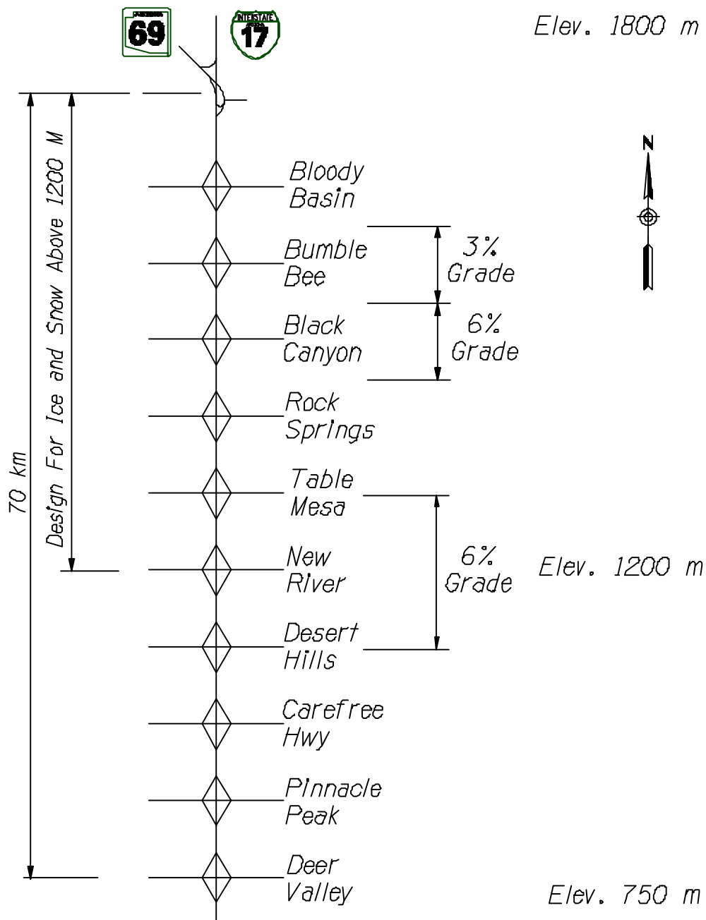
Figure 2. Hypothetical rural freeway section.
