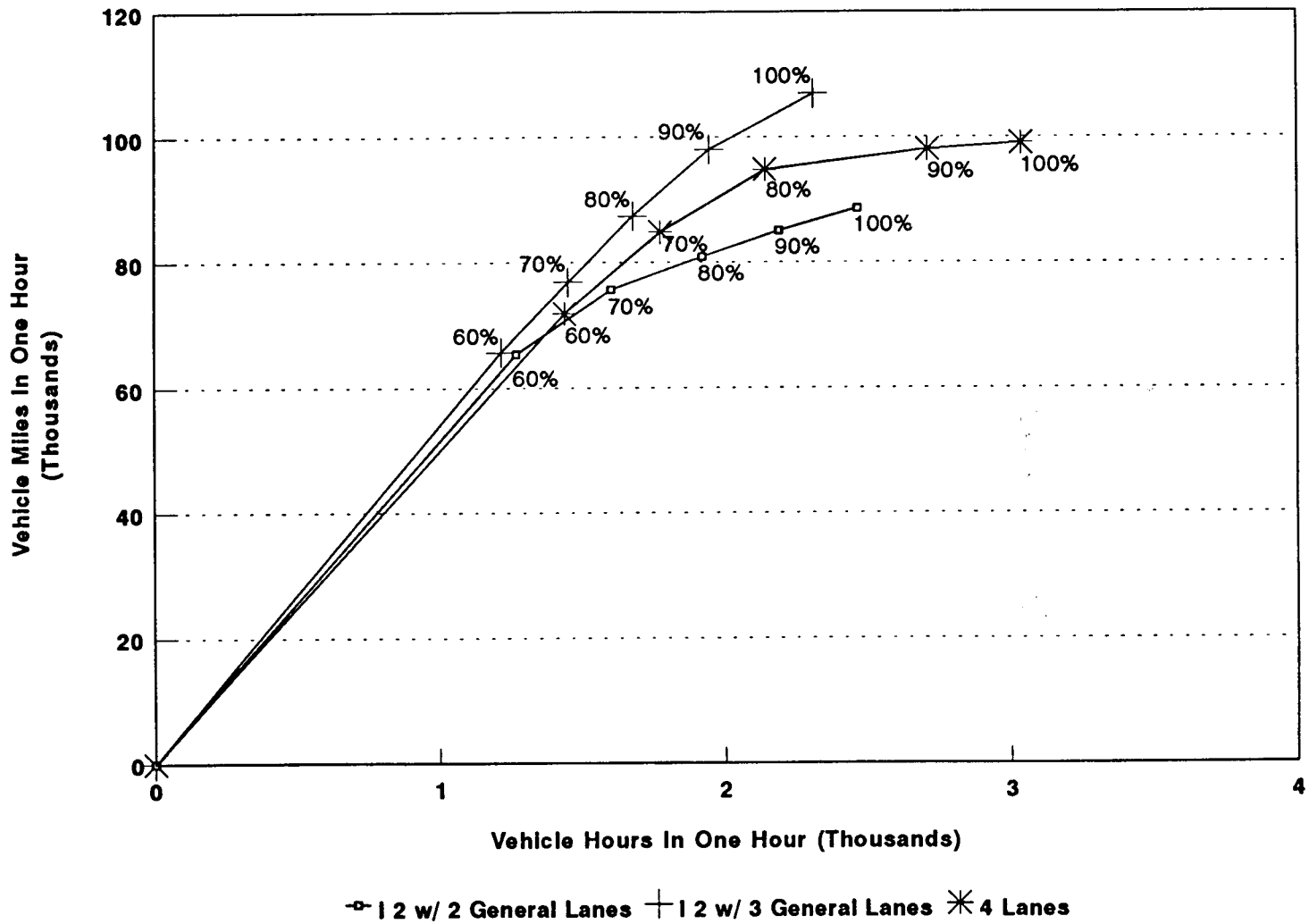
Figure 2-14. Comparison of Throughput for Long Island Expressway AHS Against Four Lane LIE
