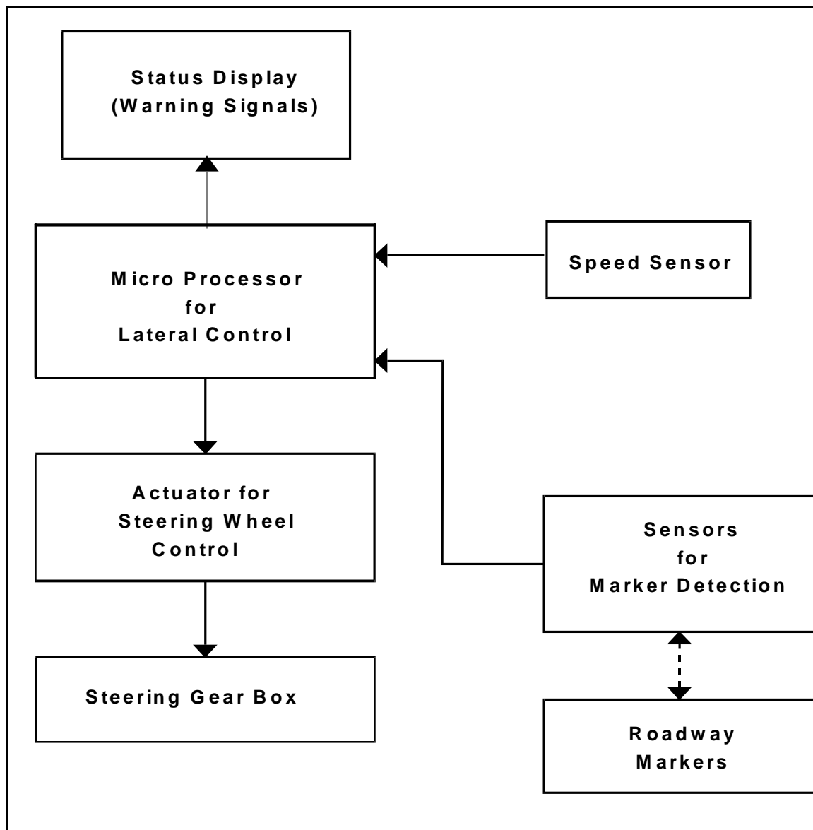
Figure 5-2. Automatic Steering Using Lane Marker Detection
