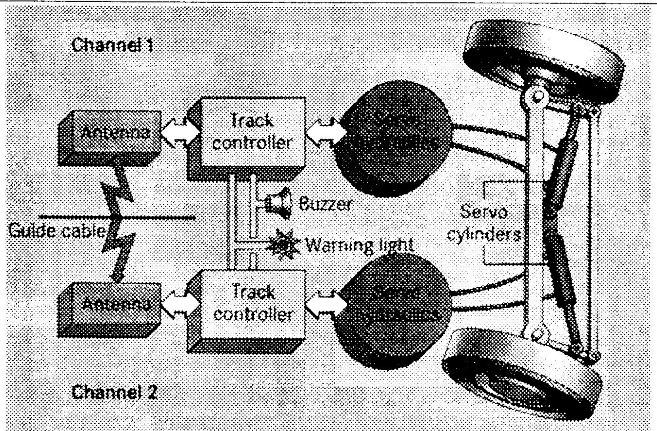
Figure 34. Electronic track guidance
