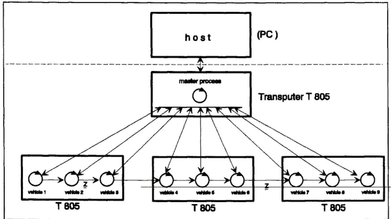
Figure 19. Platoon simulation on Transputer system
