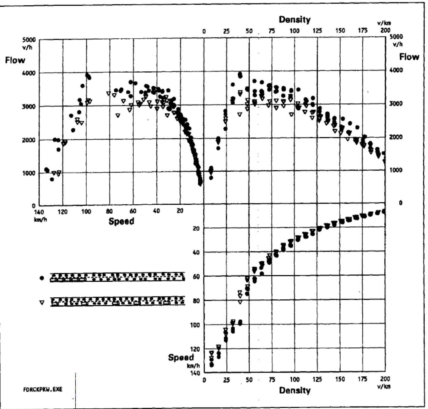
Figure 15. Simulation of mixed MIS and non-MIS traffic on two-lane freeways. Ratio of 1:7 for number of trucks to number of cars.
