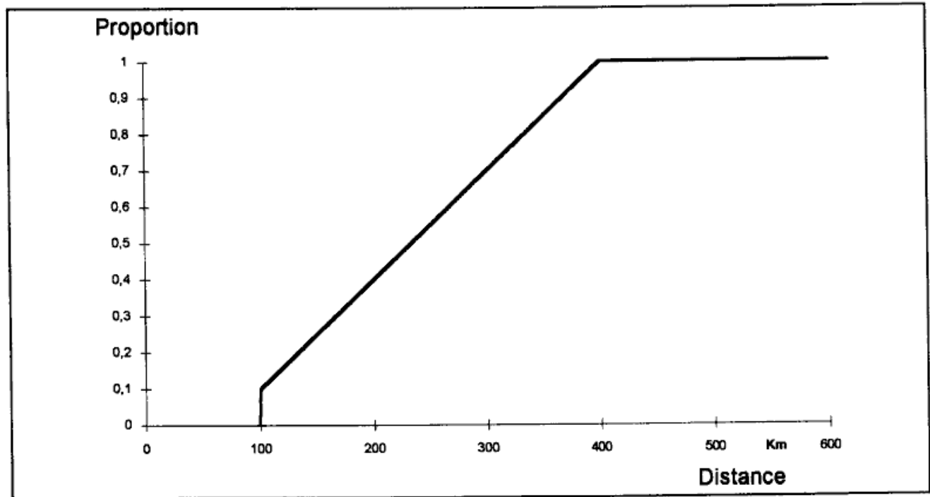
Figure 3. Valuation filter
