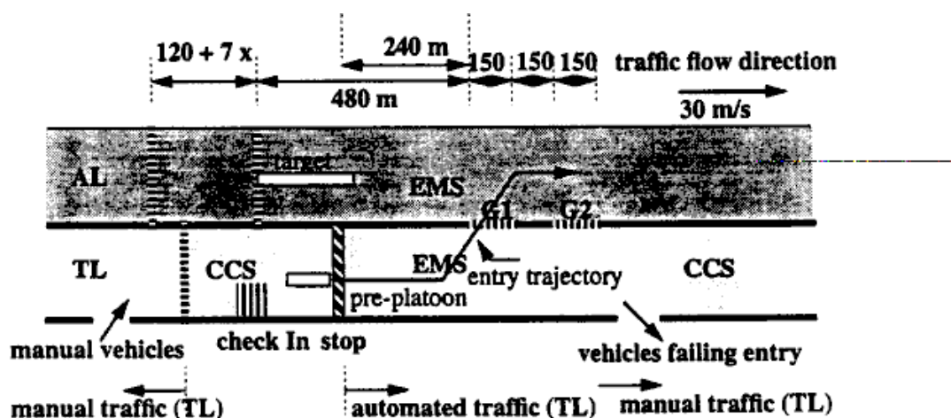
Figure 10: Regulation layer for entry: Arrangements 1,3,4
