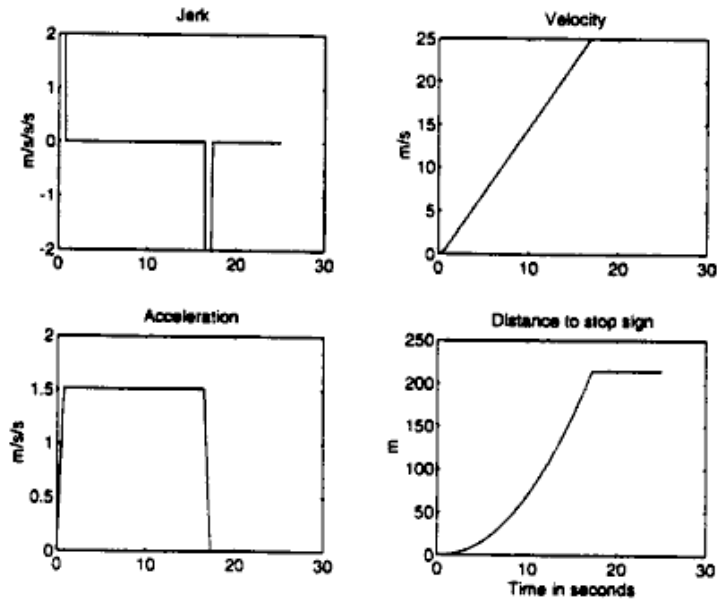
Figure 17: Desired trajectory for accelerate-to-enter
