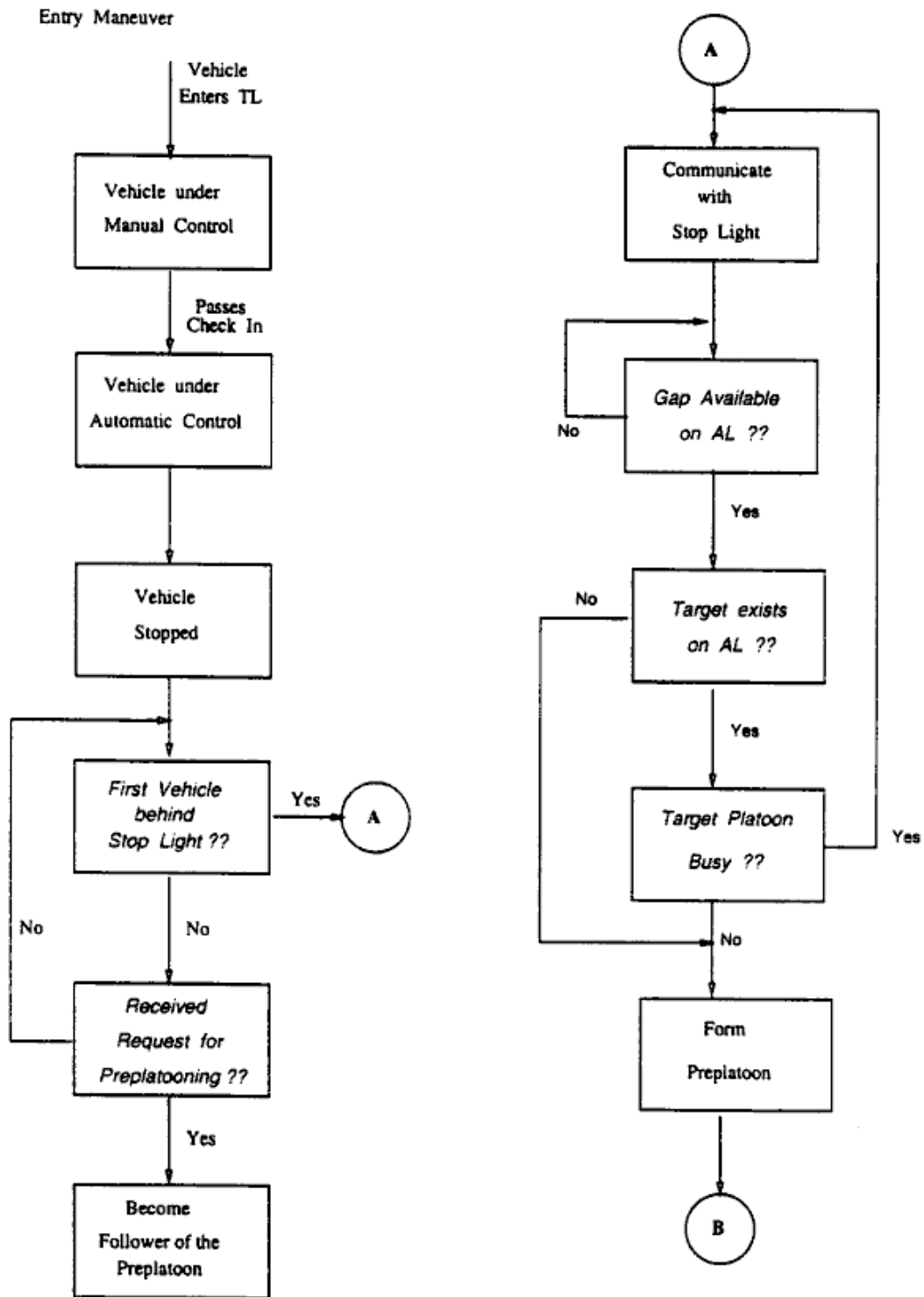
Figure 12: Flowchart for entry maneuver
