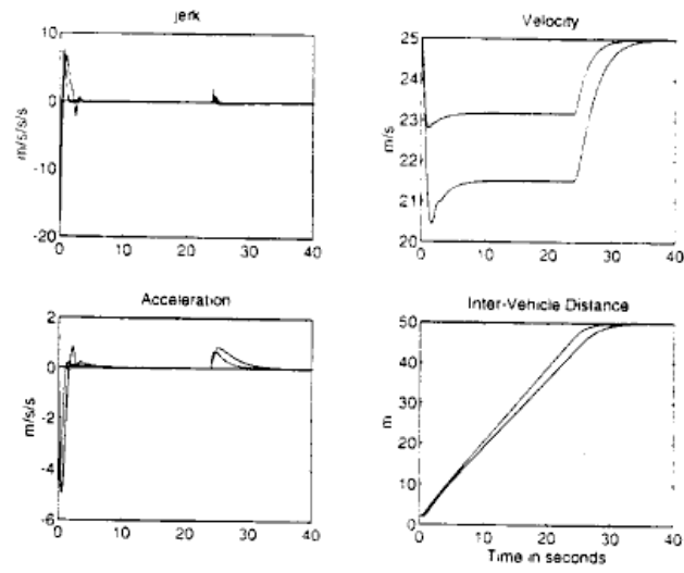
Figure 19: Break up of a three vehicle post-platoon
