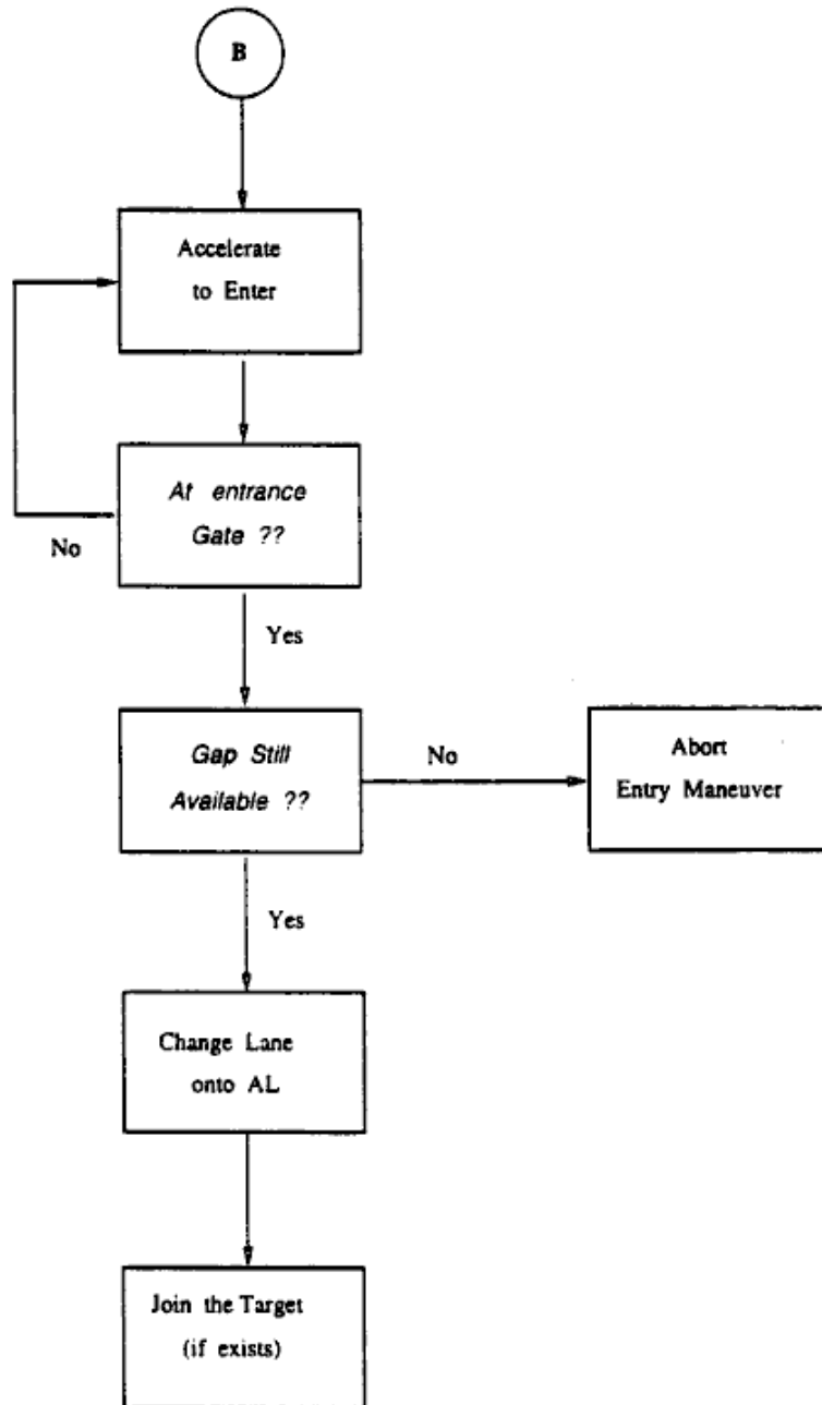
Figure 13: Flowchart for entry maneuver: continued
