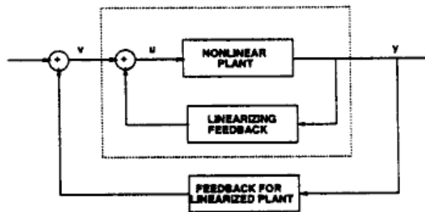
Figure 16: Two stage feedback.
