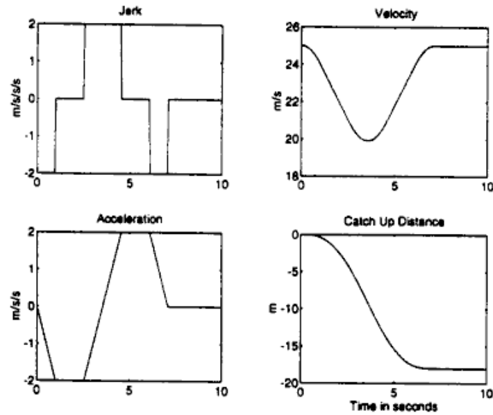
Figure 18: Desired trajectory for catch up
