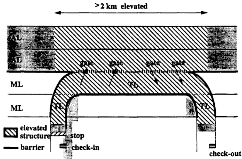
Figure 6: Entry/exit arrangement 4b
