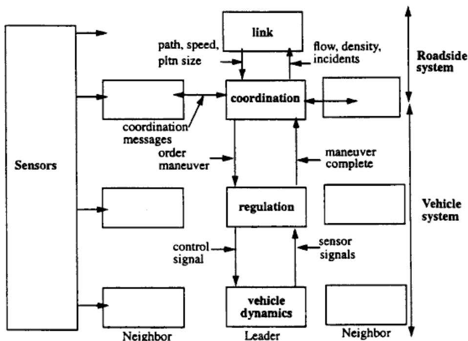
Figure 9: Coordination and control architecture
