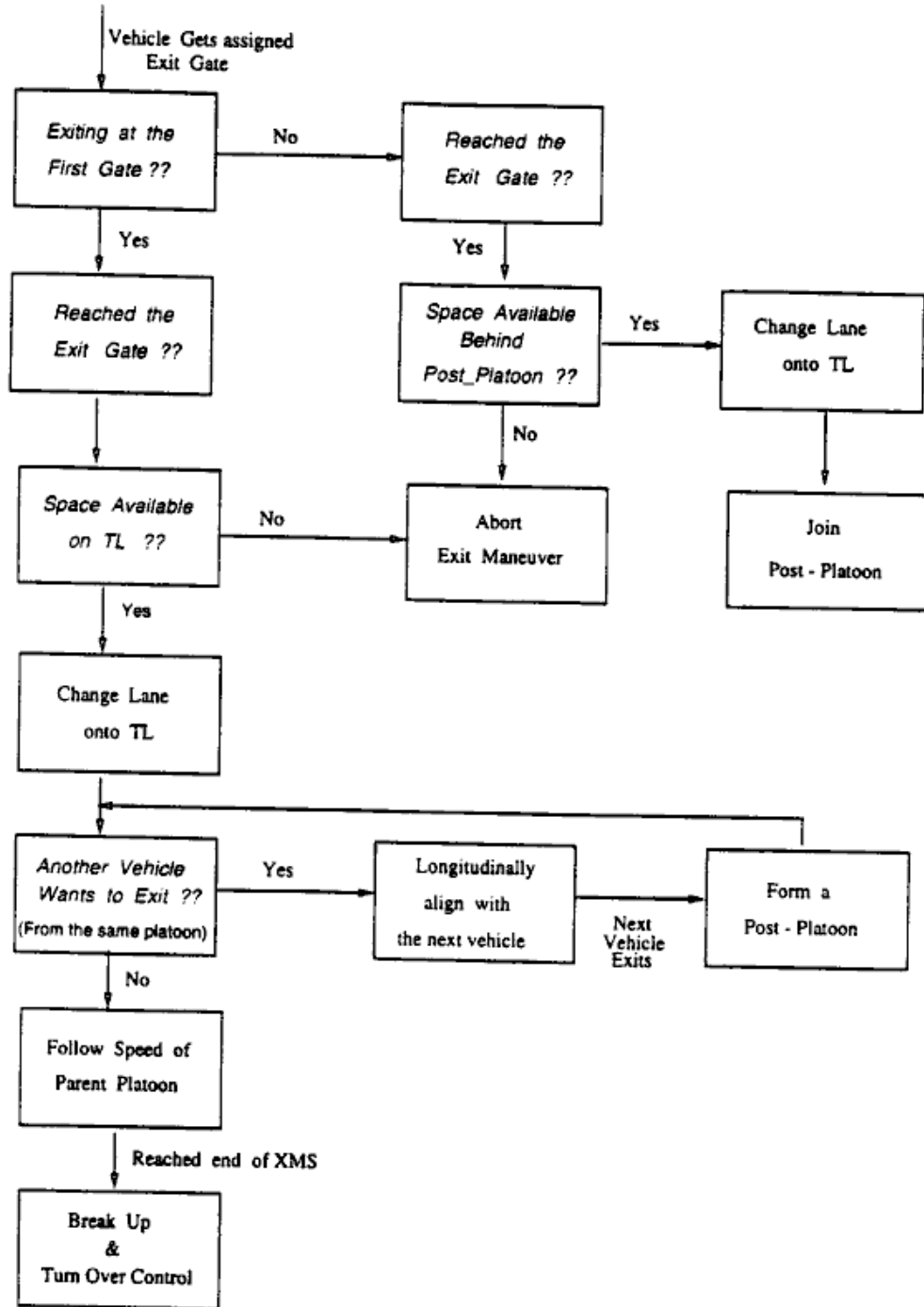
Figure 14: Flowchart for exit maneuver
