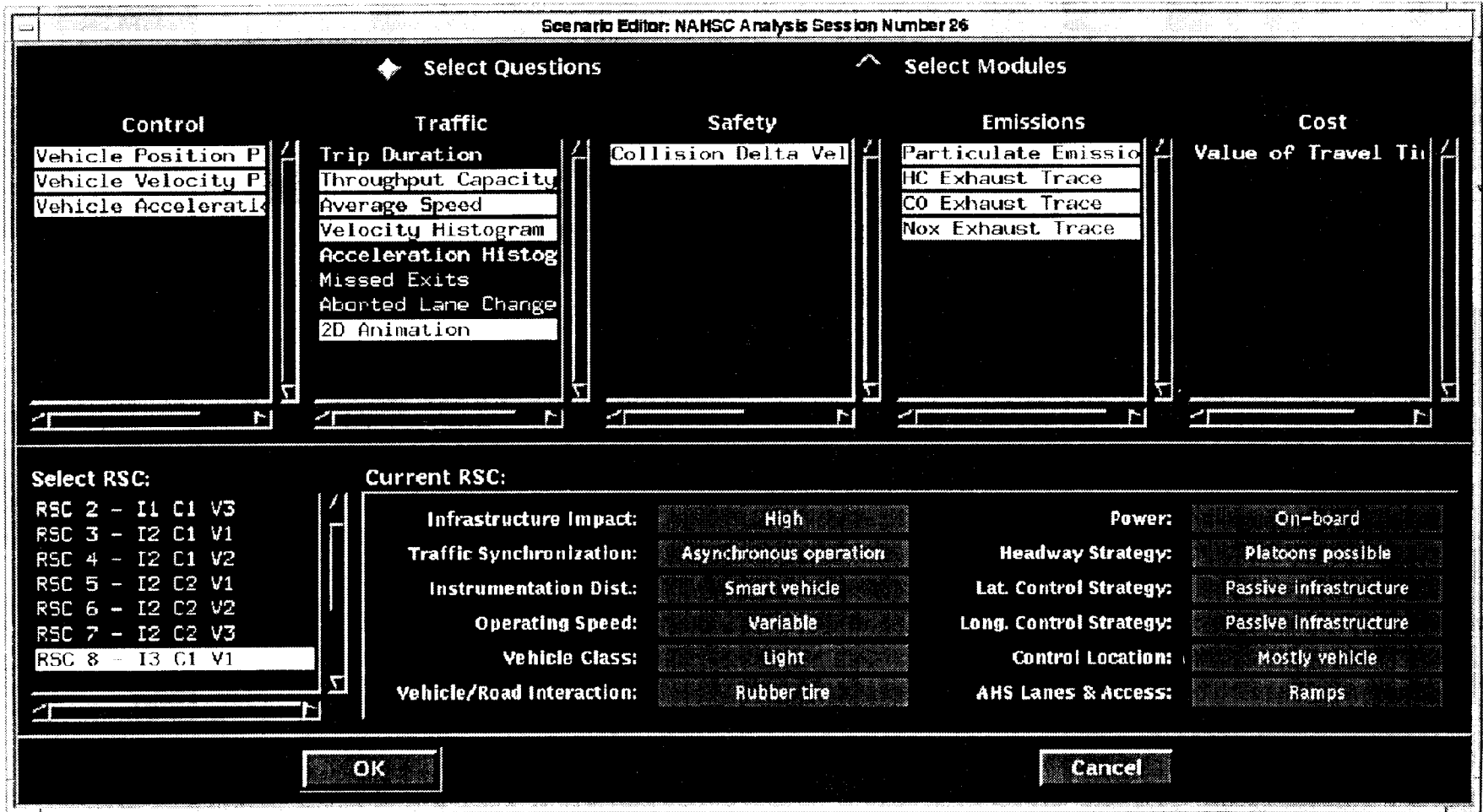
Figure 5-4 Scenario Editor
