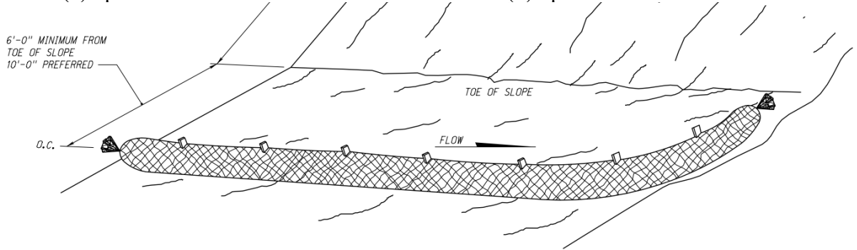
(e) installation detail at toe of slope
