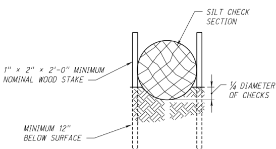
(c) option C for installation
