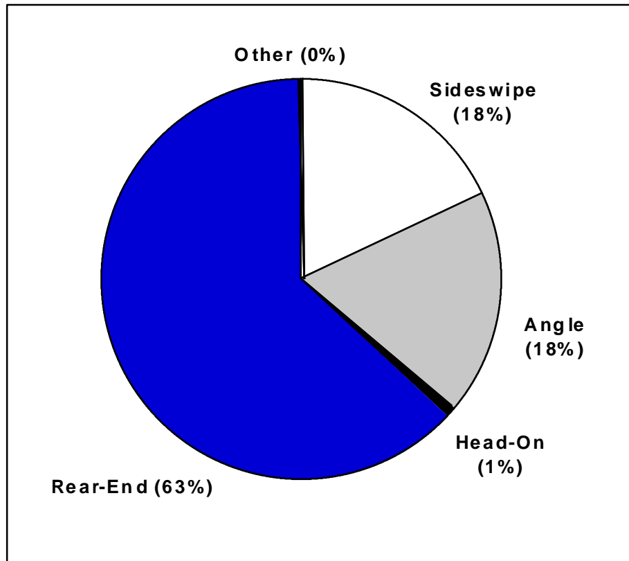
Figure 15. Manner of collision, two-vehicle crashes on interstate, non-junction, non-interchange
