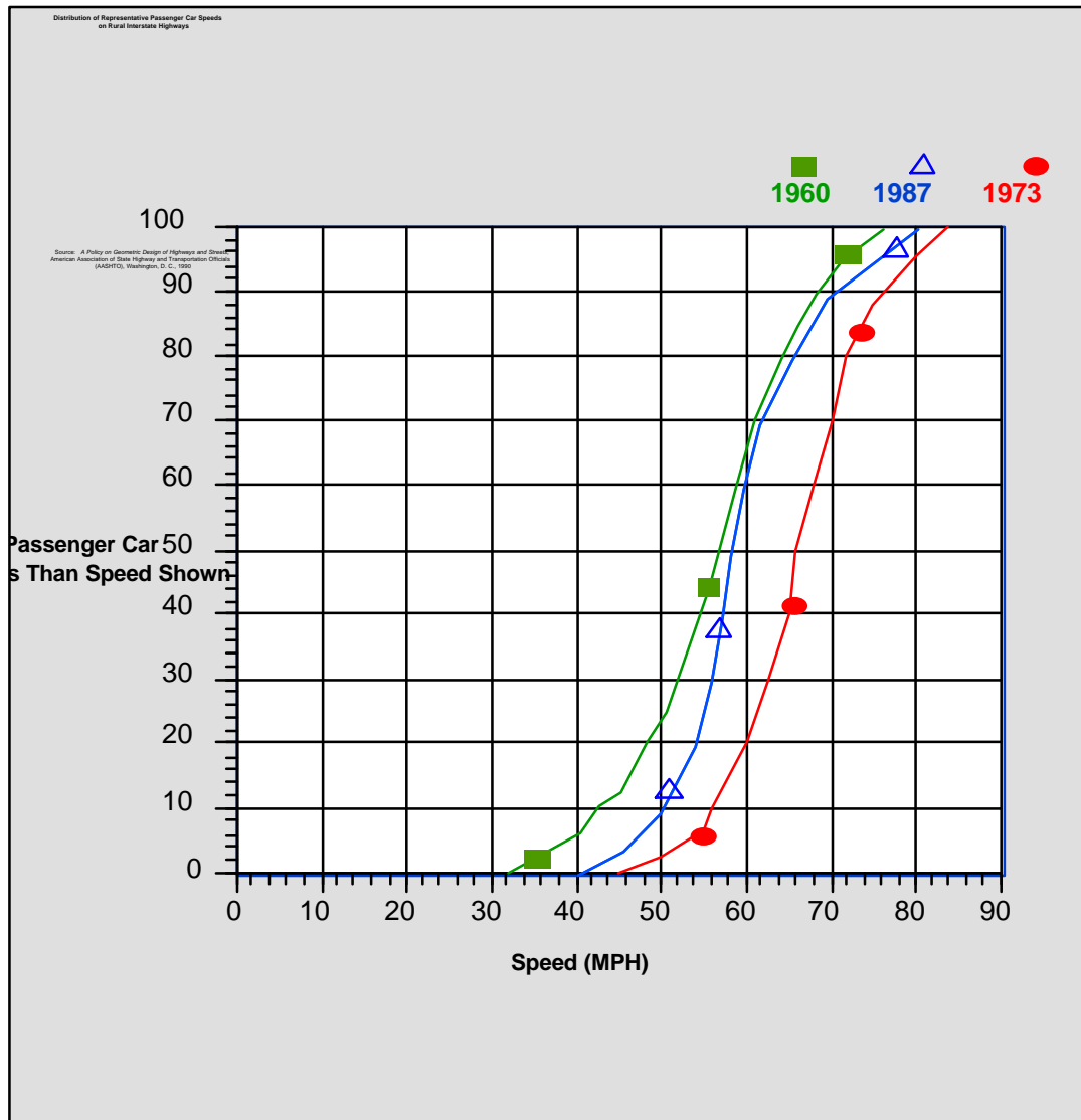
Figure 9. Distribution of vehicle speeds
