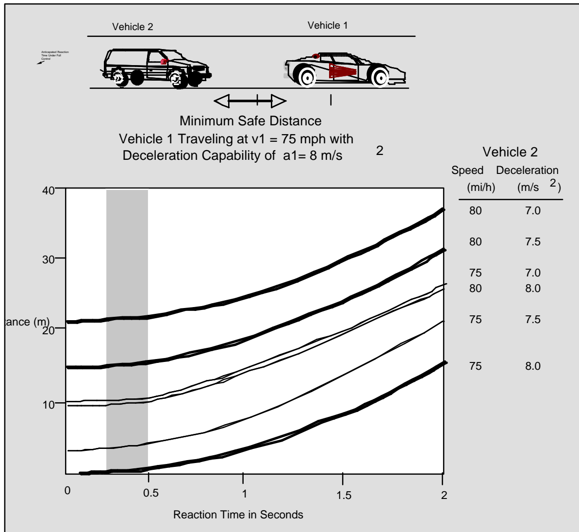
Figure 19. Minimum following distance
