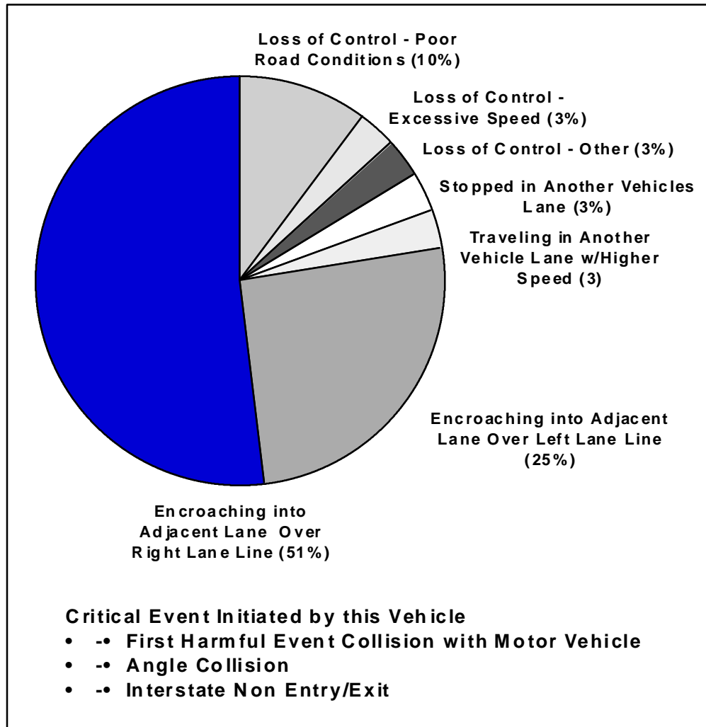
Figure 17. Critical event initiated by this vehicle which made crash imminent, angle collisions on interstate, non-junction, non-interchange
