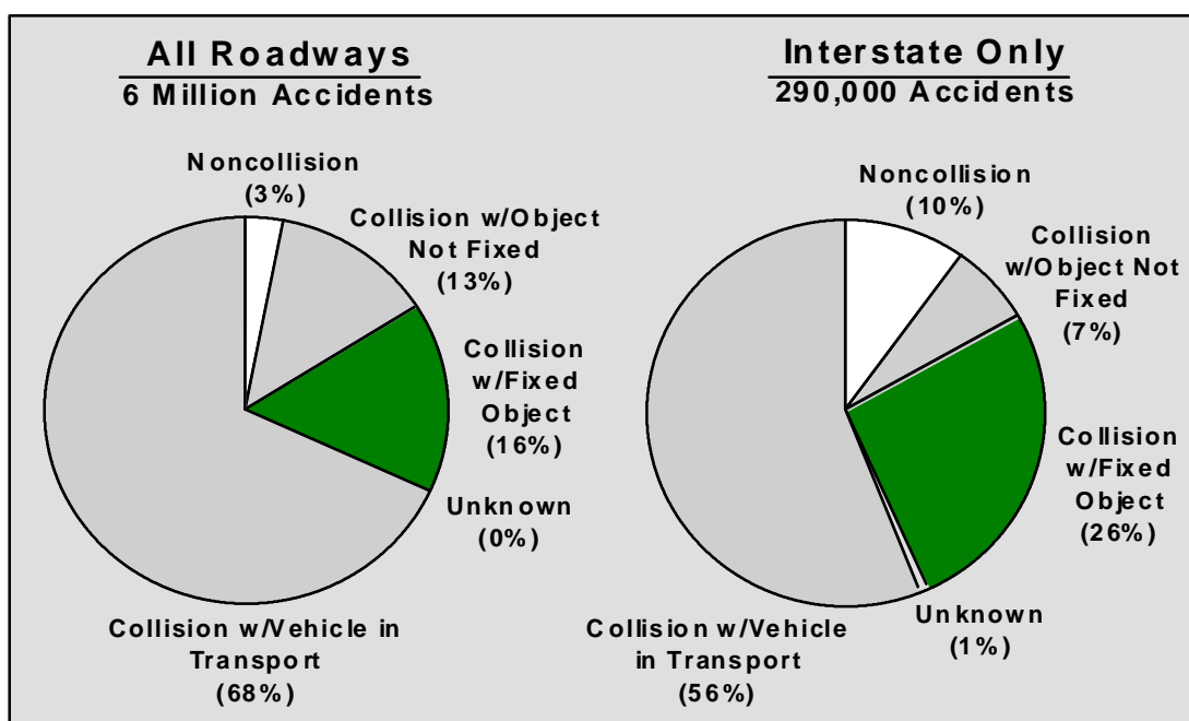
Figure 3. First harmful event, on interstates vs all roadways
