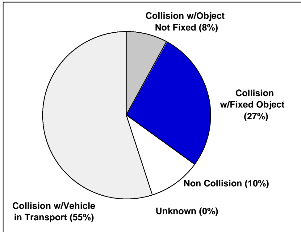
Figure 14. First harmful event for interstate non-junction, non-interchange crashes
