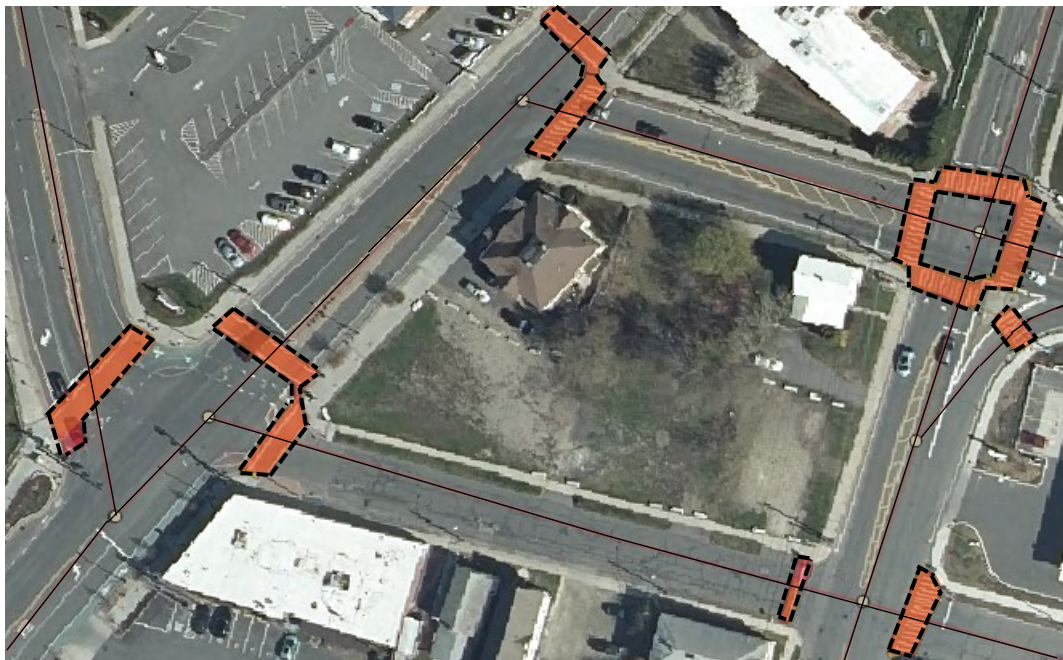
Figure 13. Overlays of 2019 and 2021 detection results
