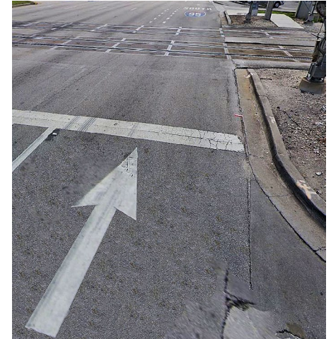
In this turn lane, approaching an I-95 on-ramp, a straight arrow has replaced a turn arrow. The arrow directs drivers across the at-grade railroad tracks, just ahead. At the top of the image is an I-95 South marking for additional guidance.
