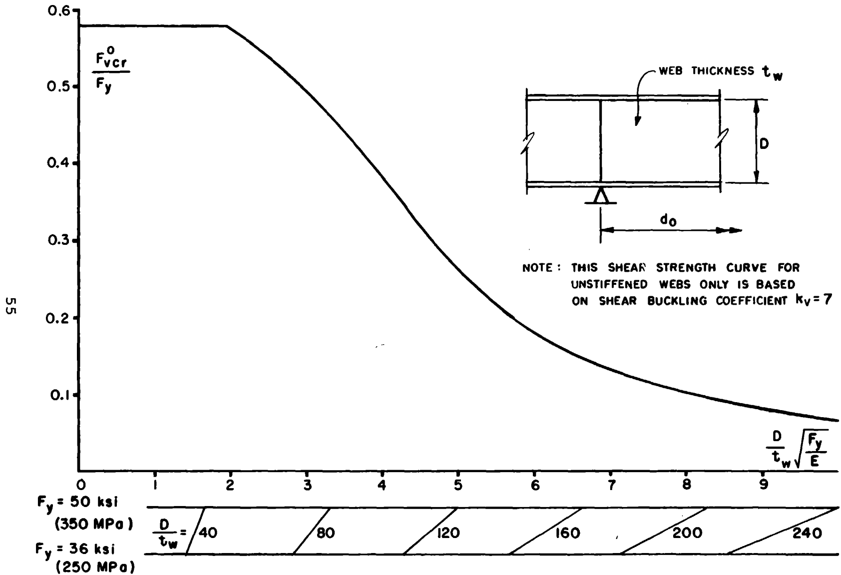
FIG. I.7.210 CRITICAL BUCKLING STRESS OF UNSTIFFENED WEB DUE TO SHEAR ACTING ALONE
