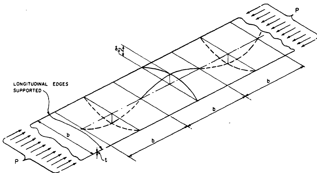
(b) THEORETICAL MODEL USED IN ANALYTICAL TREATMENT (F1)
