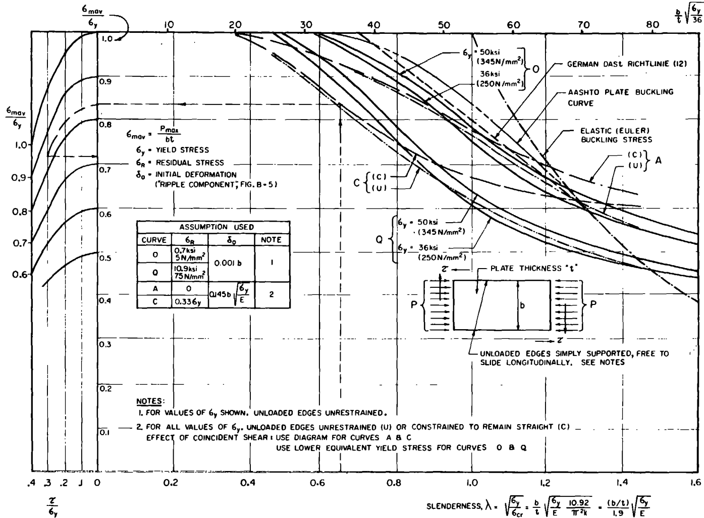
FIG. B-3. PLATE STRENGTH CURVES FOR UNSTIFFENED PANELS
