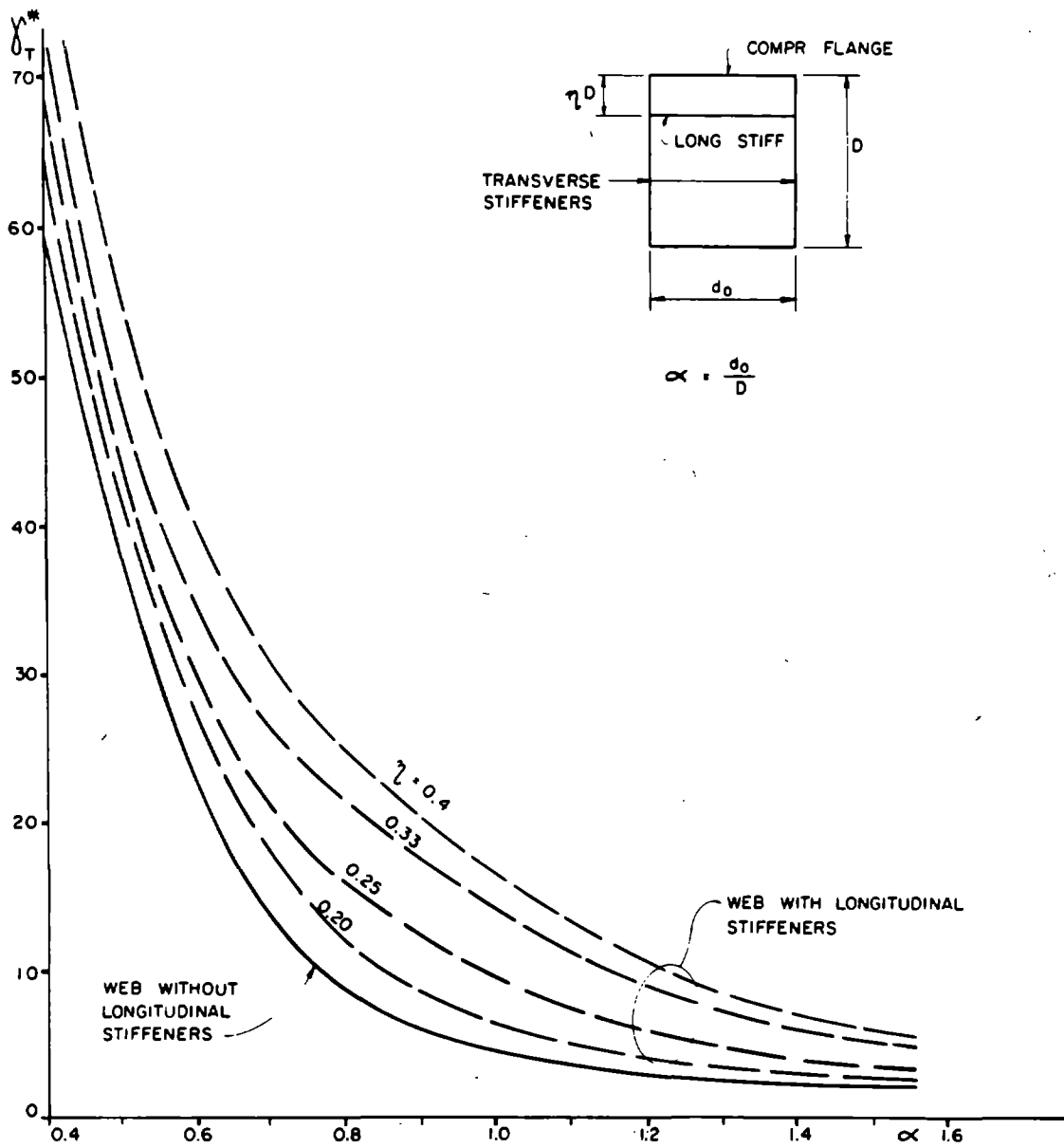
FIG. 1.7. 213 (A) RIGIDITY COEFFICIENTS \gamma_T^* FOR TRANSVERSE WEB STIFFENERS
