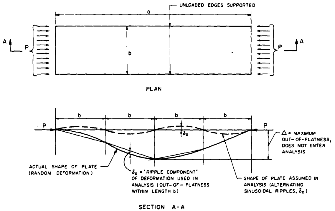
(a) DEFINITION OF "RIPPLE COMPONENT" OF PLATE IMPERFECTION
