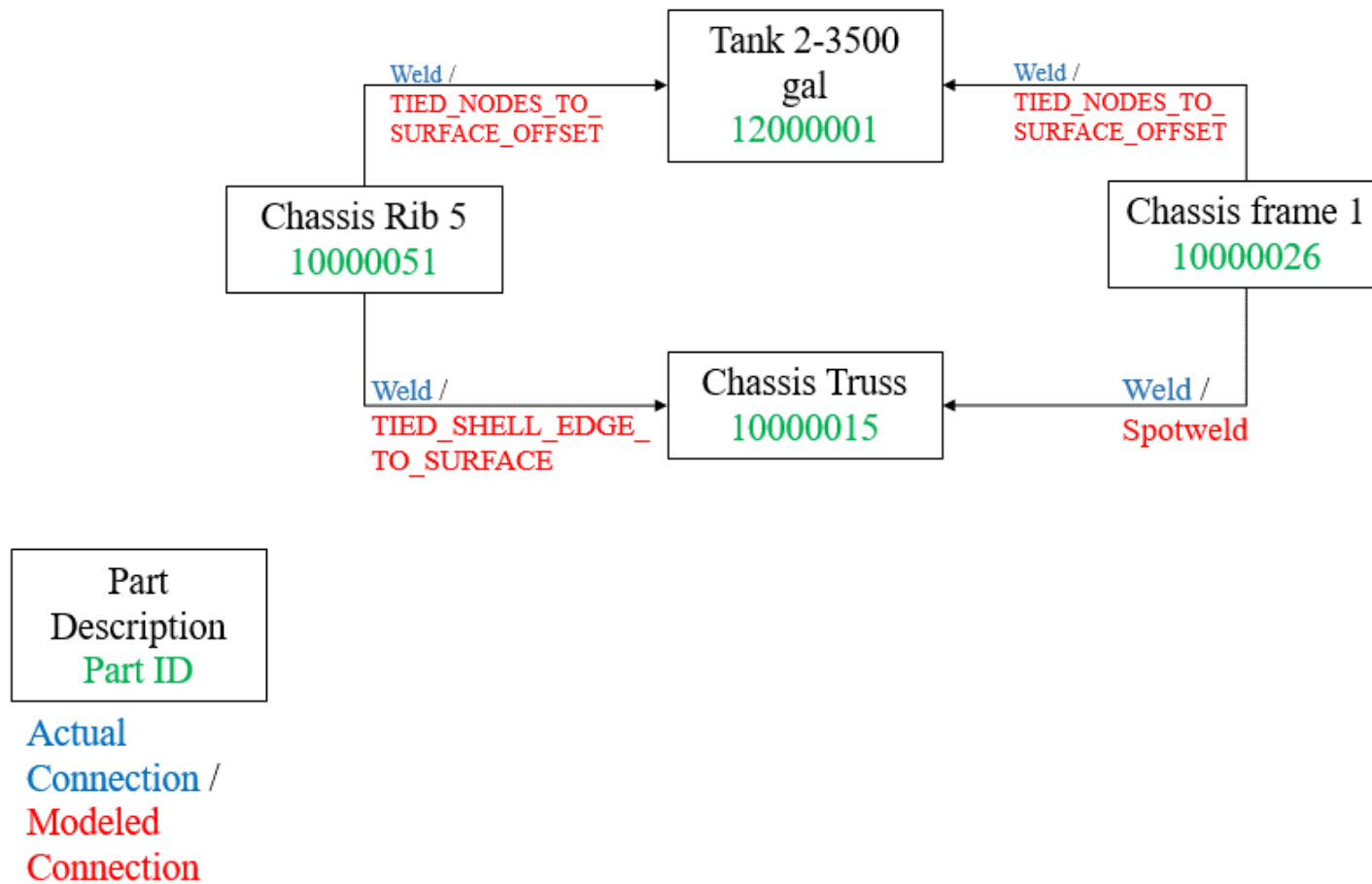
Figure B.5 Chassis to Tank-2 Connection Diagram
