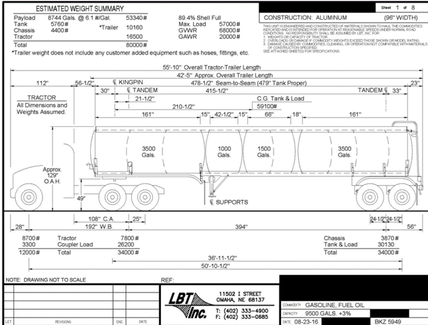
Figure 3.2 Standard Plan Drawings for Modeled Tank Trailer BKZ 5949
