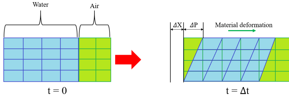
Figure 2.10 ALE Mesh Motion
