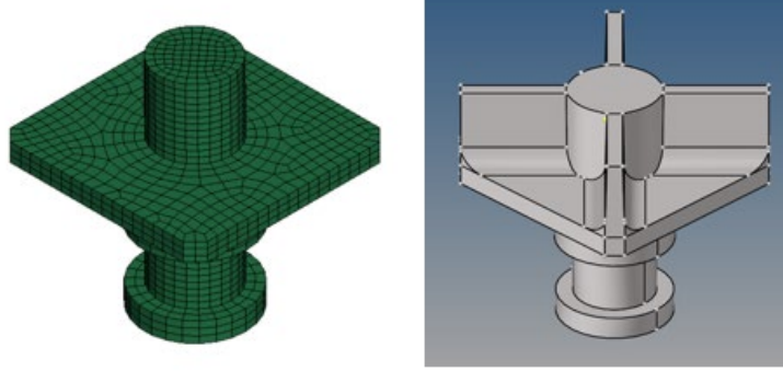
Figure 3.6 Pin Component
