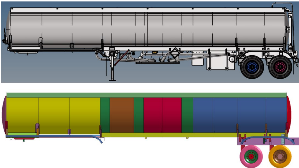
Figure 3.24 LBT Inc. Trailer Model Right View (Top) and LS-DYNA Model Right View (Bottom)
