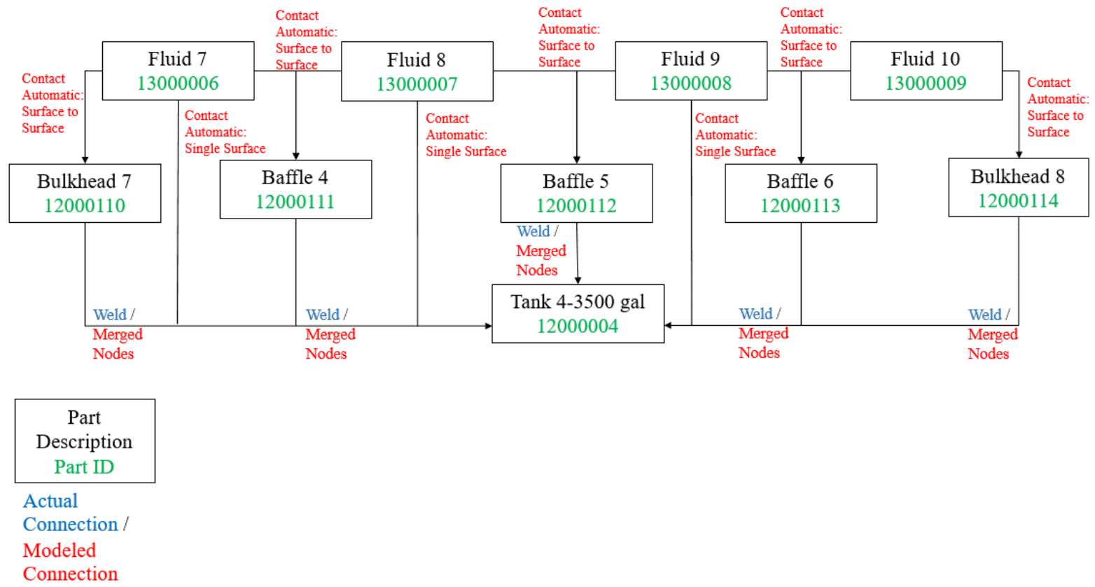
Figure D.4 Lagrangian Fluid to Tank Connection Diagram
