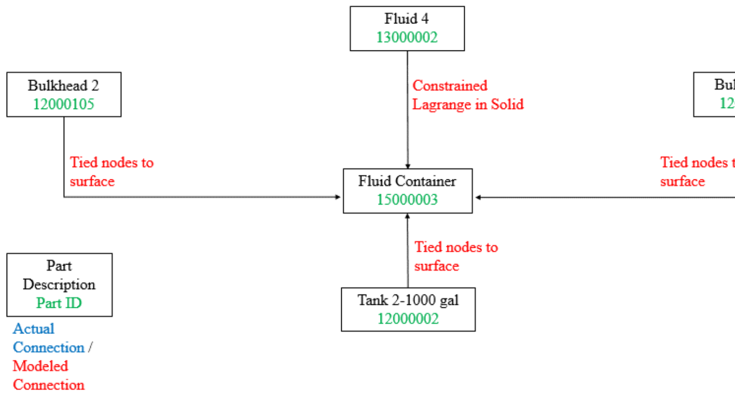
Figure E.2 ALE Fluid to Tank Connection Diagram
