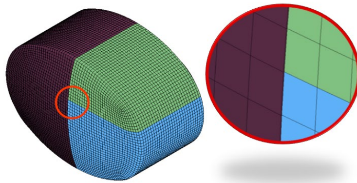
Figure 7.2 Tank Meshing
