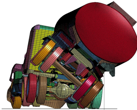
Figure 6.9 50 in. Barrier Maximum Roll at 900 ms
