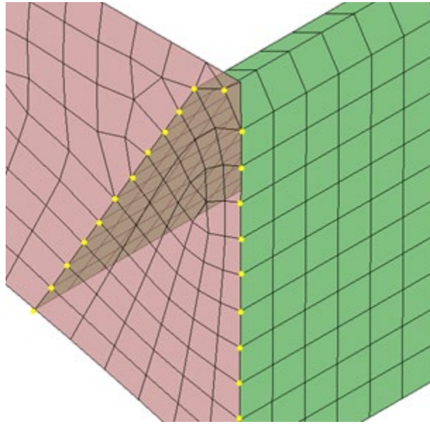
Figure 3.9 Merged Nodes
