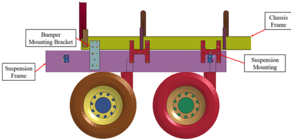
Figure 3.15 Suspension to Chassis Constraints
