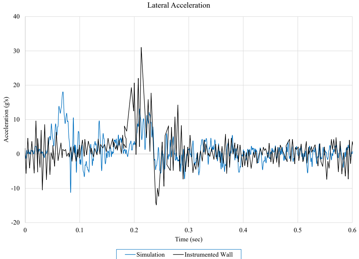
Figure 5.5 Lateral Acceleration
