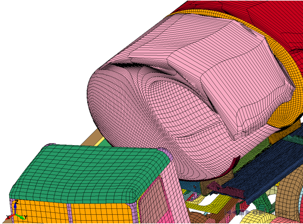
Figure 7.1 Fluid Mesh Deformation
