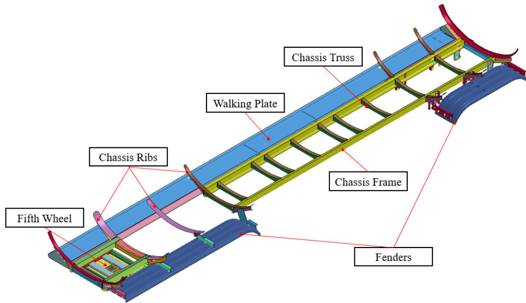
Figure 3.4 Chassis Model
