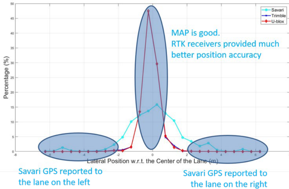
Figure 13 Vehicle Lateral Position with respect to the Lane Center
