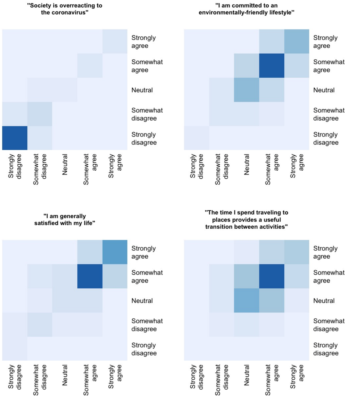
Figure 1: Heatmaps of Wave 1 and Wave 2 responses to four attitudinal statements; Wave 1 responses are recorded along the x-axis and Wave 2 responses are recorded along the y-axis
