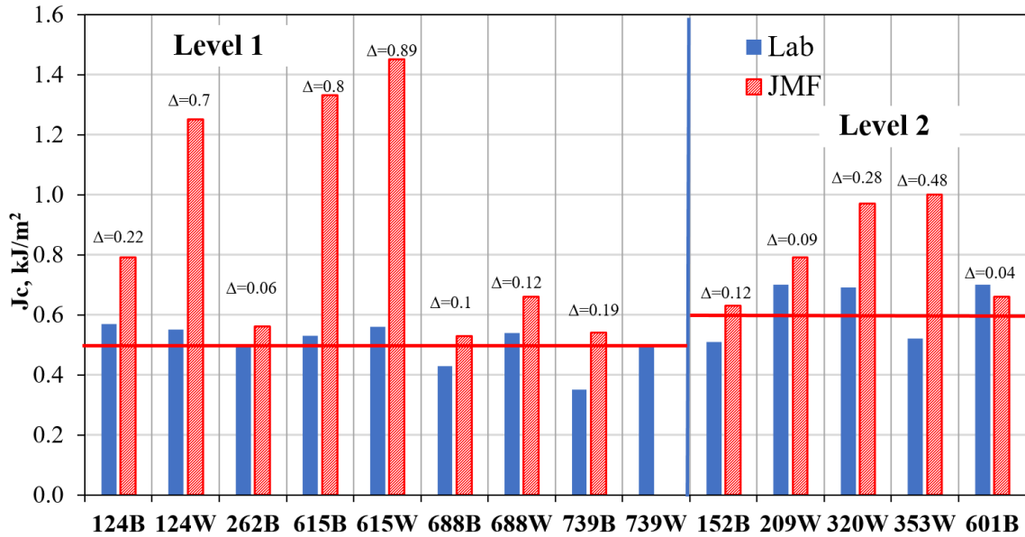
Figure 4. SCB test results
