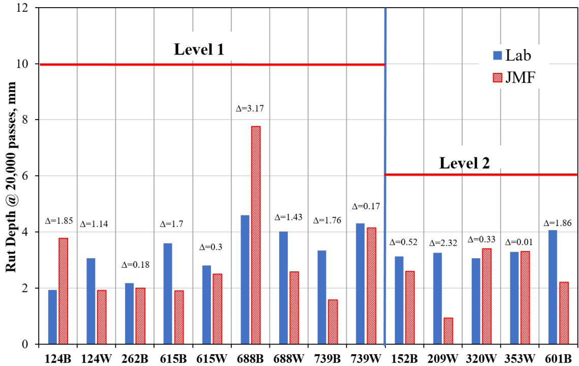
Figure 5. LWT test results
