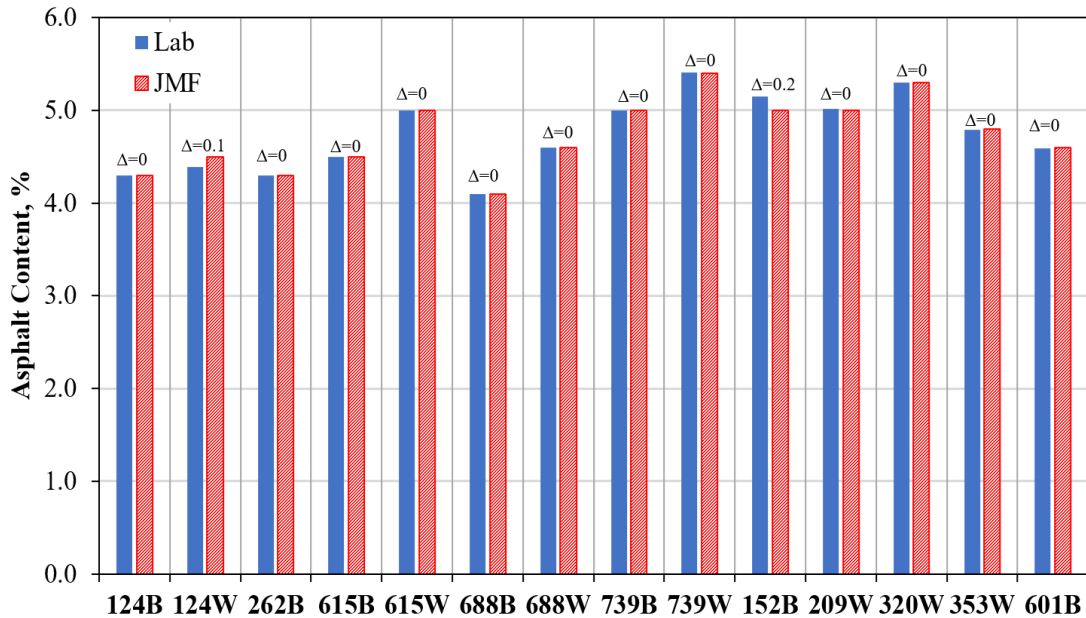
Figure 12. Asphalt content results
