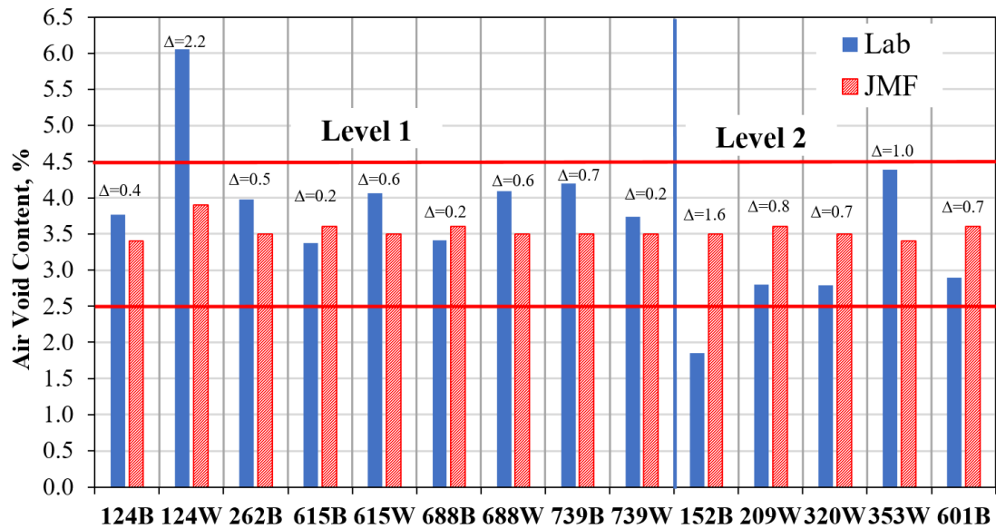
Figure 9. Air void content values
