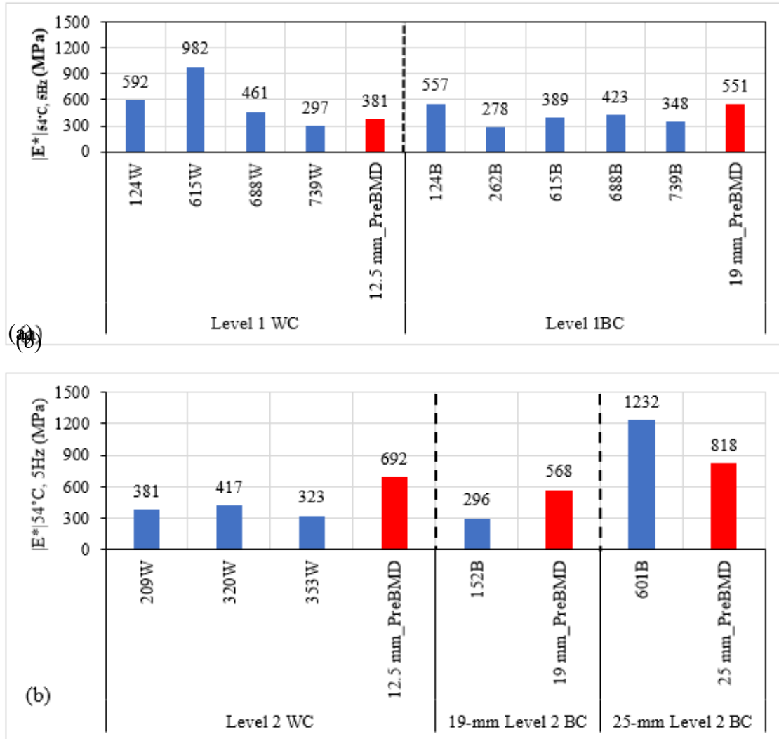
Figure 8. |E^*|_{54^\circ C, 5Hz} for (a) level 1 and (b) level 2 wearing and binder course mixtures
