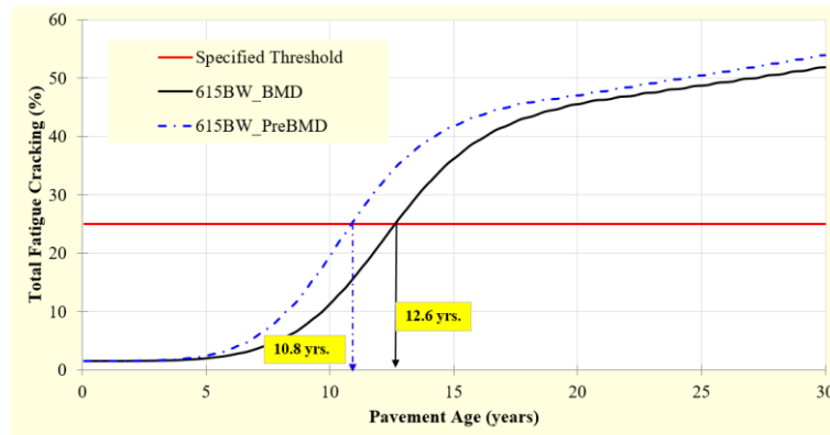
Figure 13. Pavement ME performance curves for 615BW
