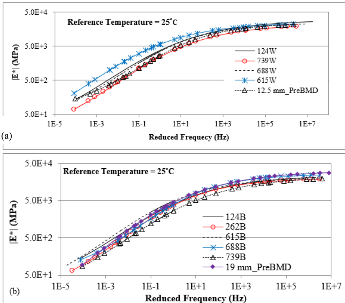
Figure 6. Dynamic modulus master curves for level 1 (a) wearing course and (b) binder course mixtures
