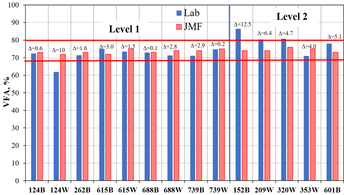
Figure 11. VFA results
