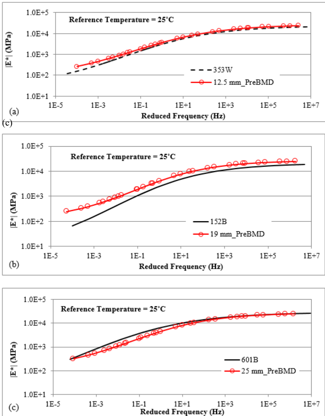
Figure 7. Dynamic modulus master curves for level 2 (a) wearing, (b) 19-mm binder course, and (c) 25-mm binder course mixtures
