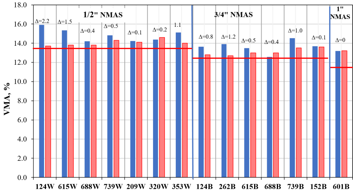
Figure 10. VMA results
