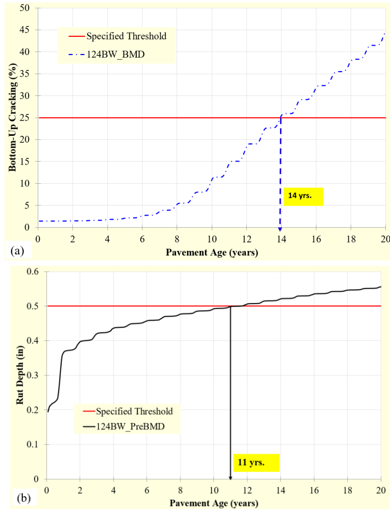
Figure 14. Pavement ME performance curves for 124BW
