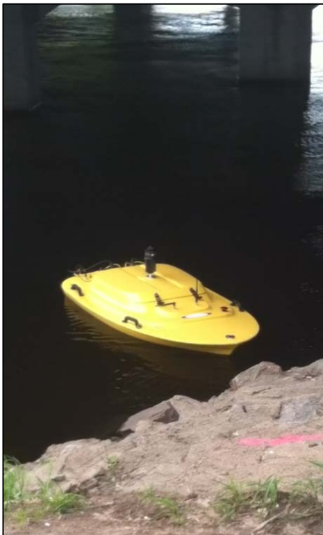
Z-Boat with the GNSS Antenna Replaced with a Reflective Prism
