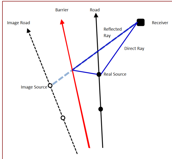
Figure 83 Illustration of Single Barrier Reflection Geometry
