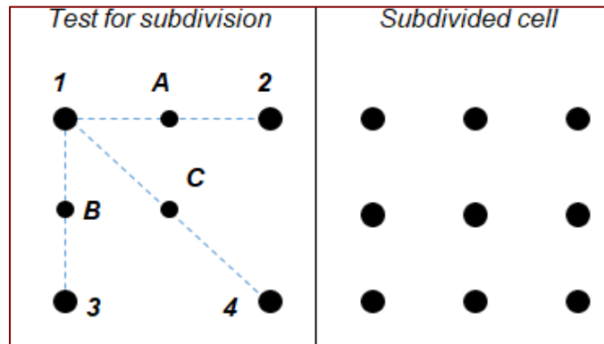
Figure 18 Subdivision of Grid Cells during Contour Computation
