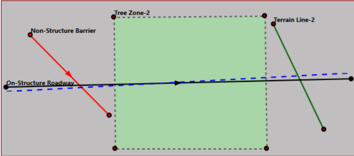
Figure 89 Permitted On-Structure/Non-Structure Crossing Examples – Plan Builder
