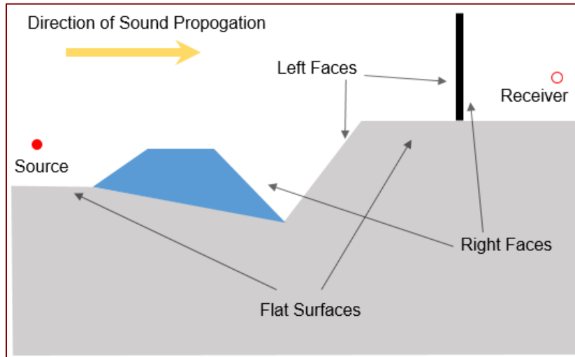
Figure 65 Vertical Geometry Definitions
