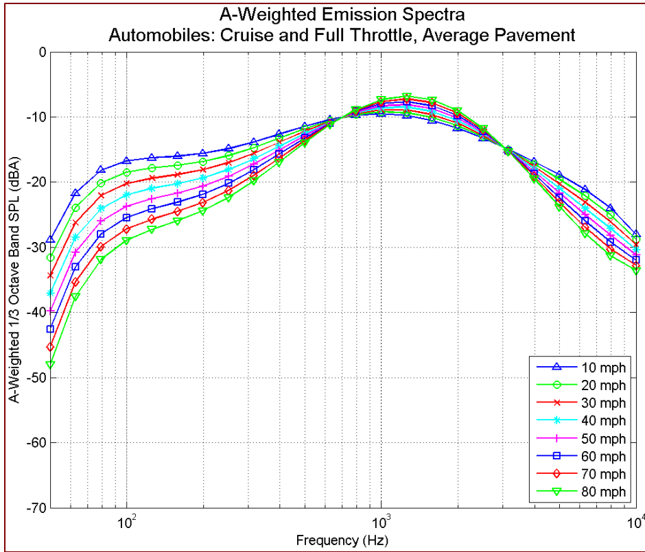
Figure 38 A-weighted emission spectra: automobiles, all throttle conditions, average pavement, by speed
