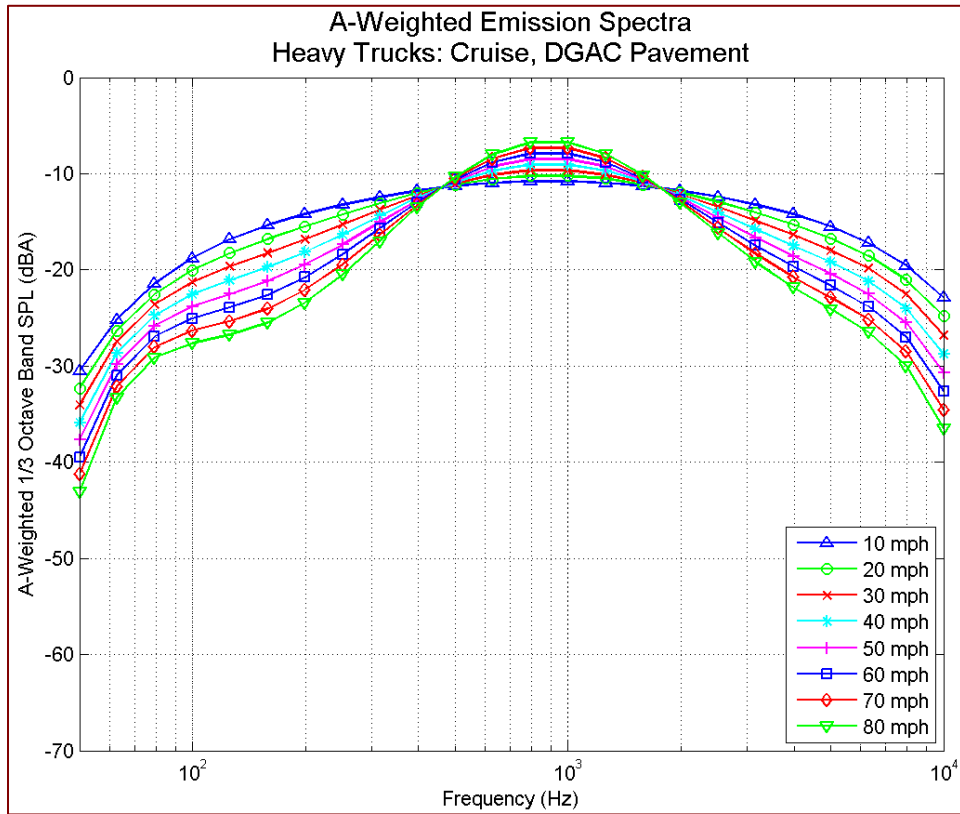
Figure 49 A-weighted emission spectra: heavy trucks, cruise throttle, DGAC pavement, by speed
