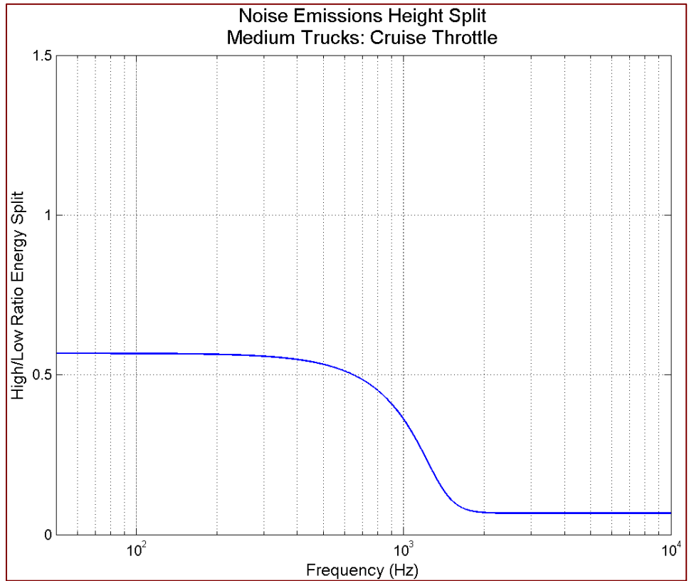
Figure 55 Sound emissions, high/low energy split by frequency: medium trucks, cruise throttle
