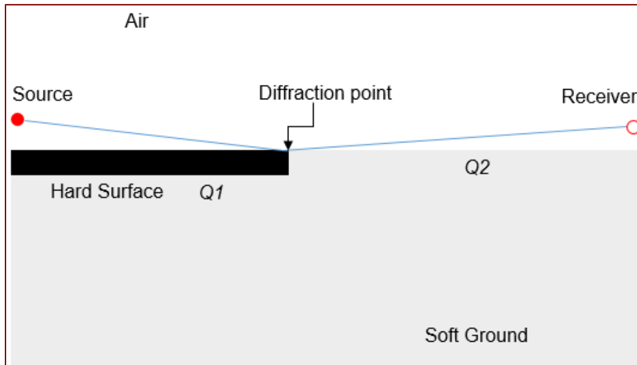
Figure 76 Example Geometry Showing an Impedance Discontinuity
