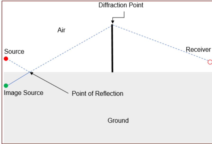
Figure 75 Example Geometry Showing Reflection
