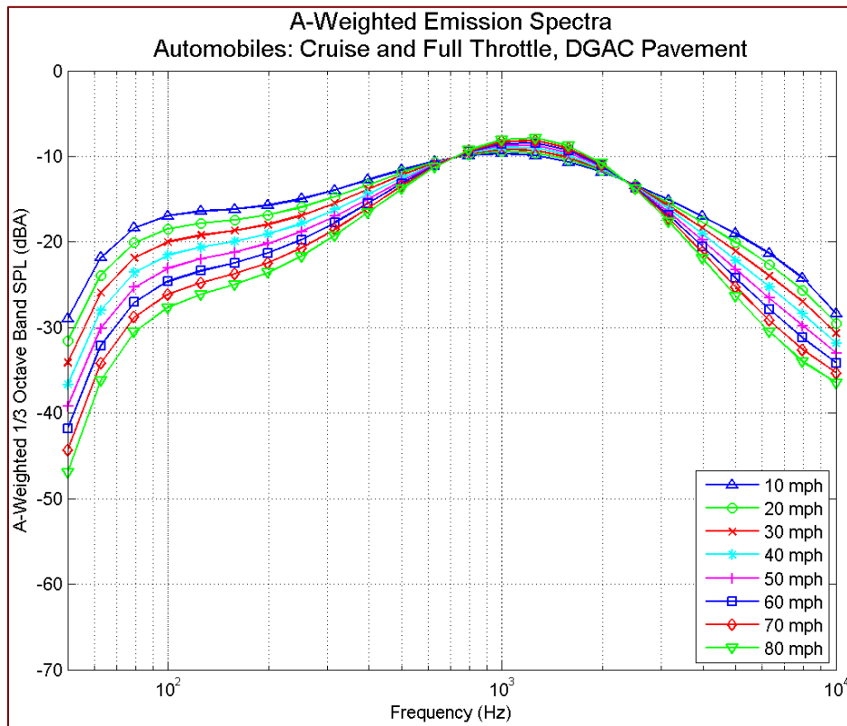
Figure 39 A-weighted emission spectra: automobiles, all throttle conditions, DGAC pavement, by speed
