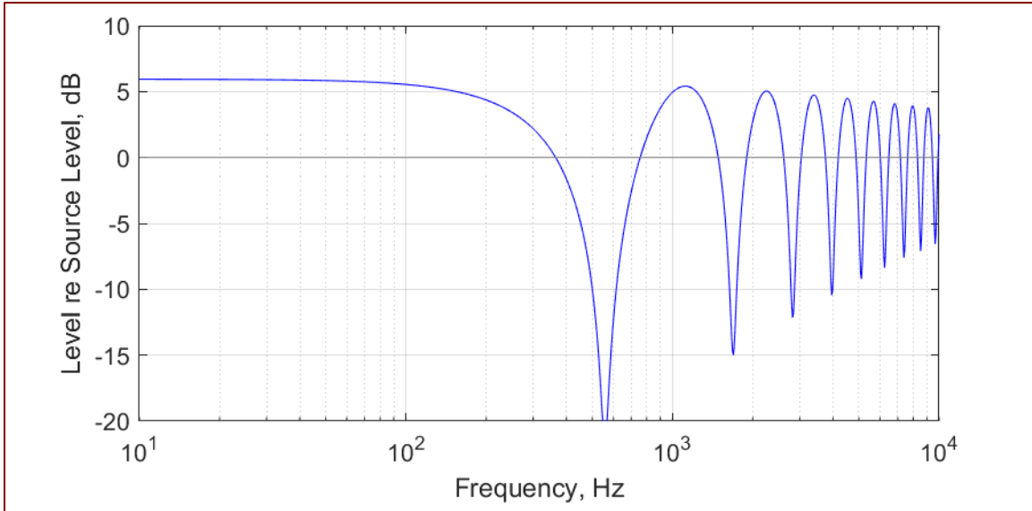
Figure 12 Example Interference Pattern for Single Reflection over Flat Ground. (Source Height = 1.5 m (5 ft), Receiver Height = 1.5 m (5 ft), Horizontal Distance = 15 m (50 ft), Ground Type = Hard Soil (5000 cgs Rayls))
