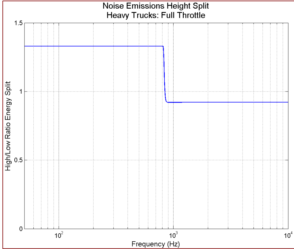
Figure 58 Sound emissions, high/low energy split by frequency: heavy trucks, full throttle
