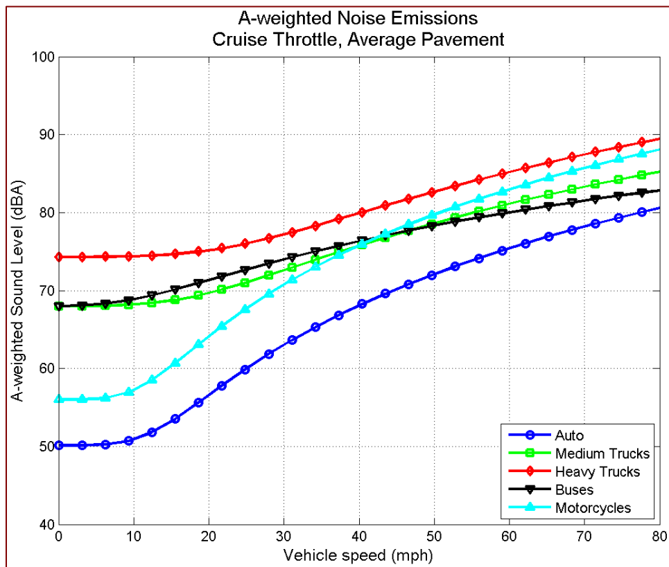
Figure 27 A-weighted sound level emissions as a function of speed: cruise throttle, average pavement, by vehicle type
