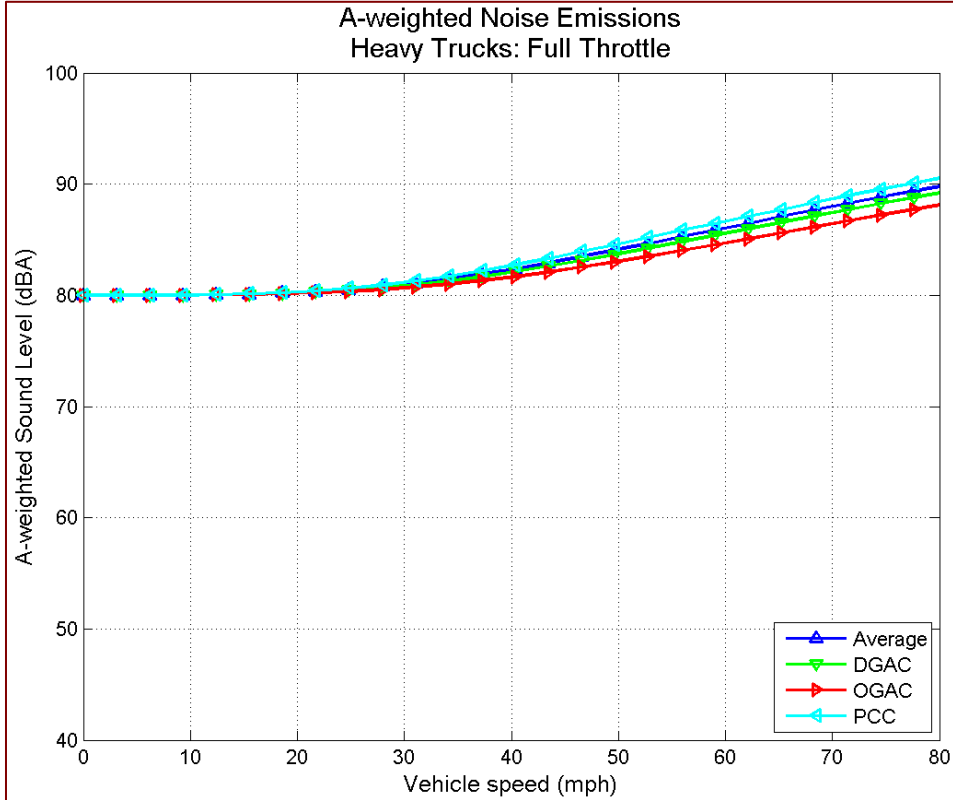
Figure 33 A-weighted sound level emissions as a function of speed: heavy trucks, full throttle, by pavement type
