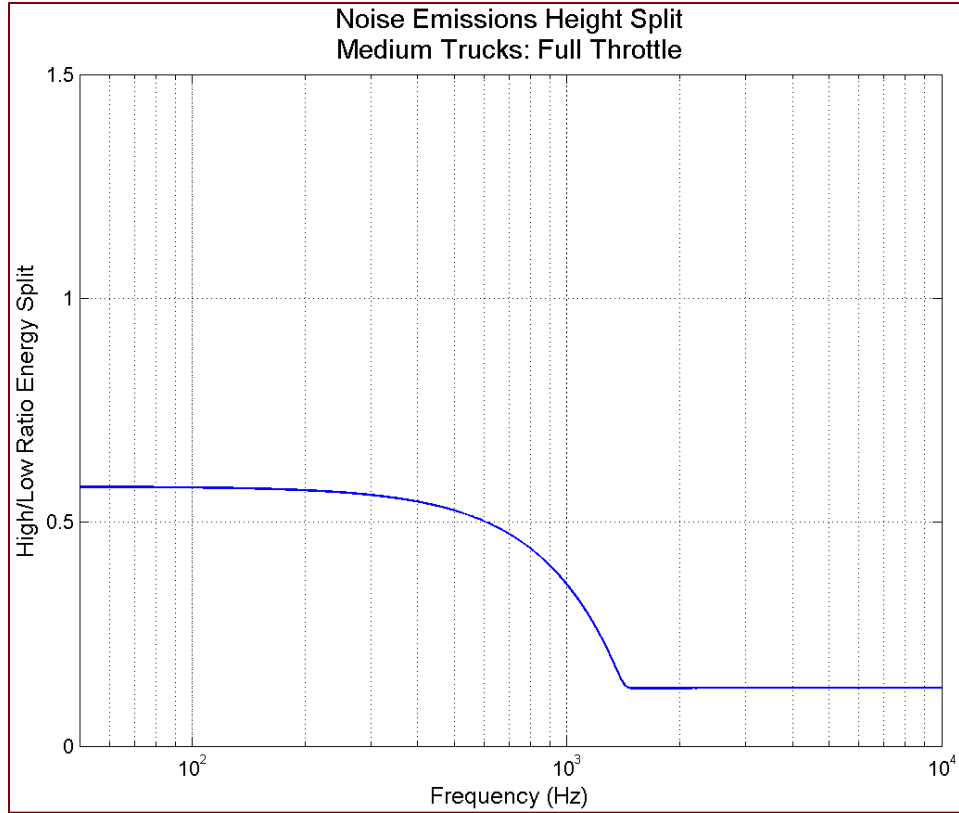
Figure 56 Sound emissions, high/low energy split by frequency: medium trucks, full throttle
