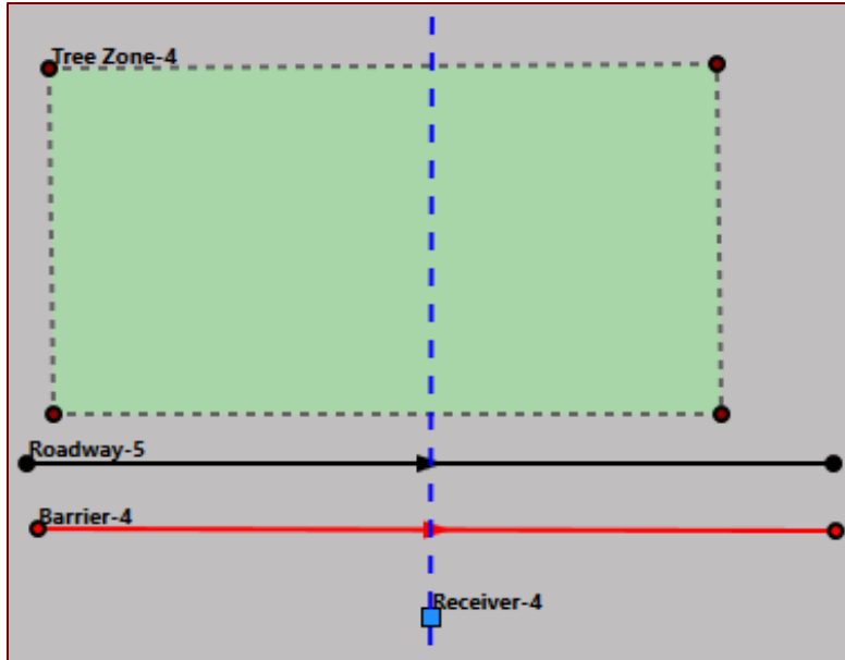
Figure 103 Non-Permitted Within Roadway Pavement Width Examples – Plan Builder
