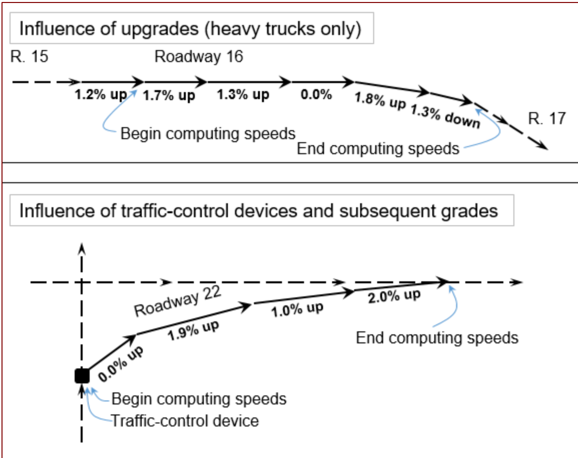
Figure 19 Geometrics for Speed Effects of Upgrades and Traffic-control Devices
