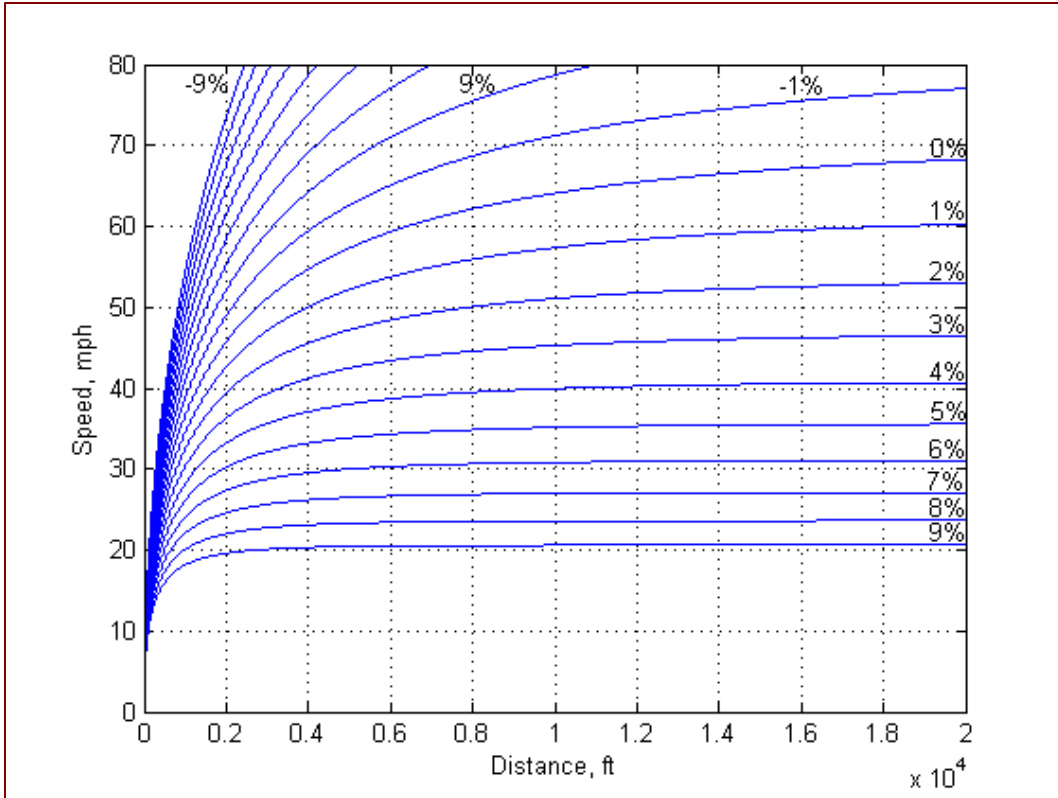
Figure 23 Acceleration away from traffic-control devices: Heavy trucks
