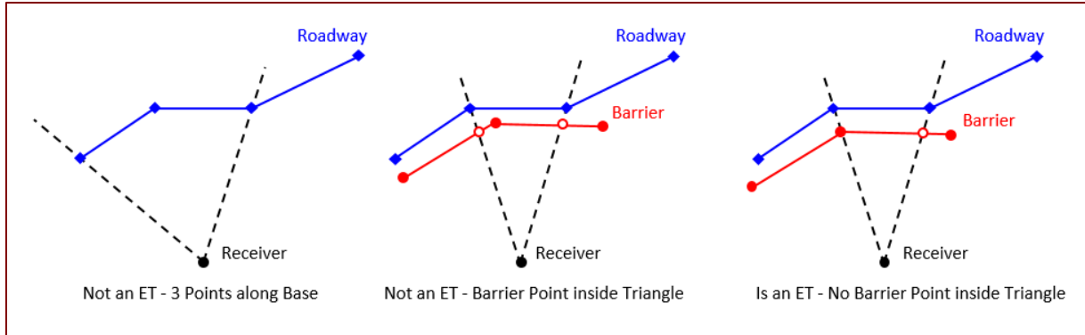
Figure 3 Examples and Counter Examples of Elemental Triangles
