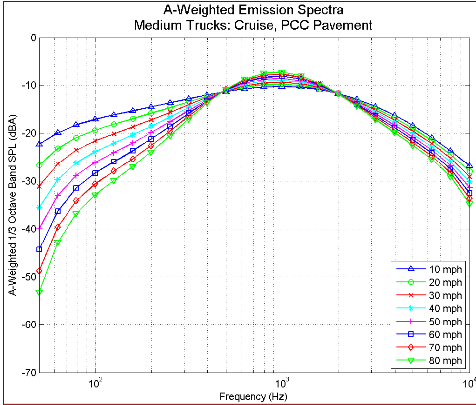
Figure 46 A-weighted emission spectra: medium trucks, cruise throttle, PCC pavement, by speed
