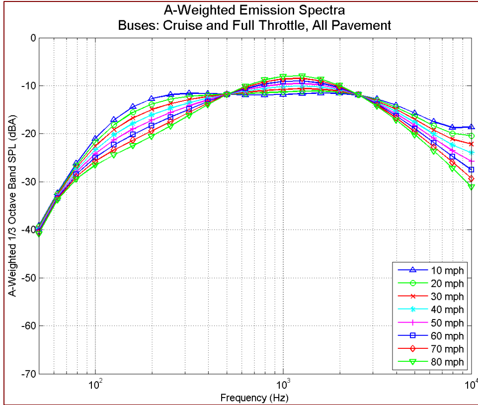
Figure 52 A-weighted emission spectra: buses, all pavements and throttle conditions, by speed
