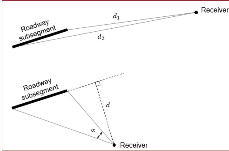
Figure 9 Definition of Relevant Distances and Angles
