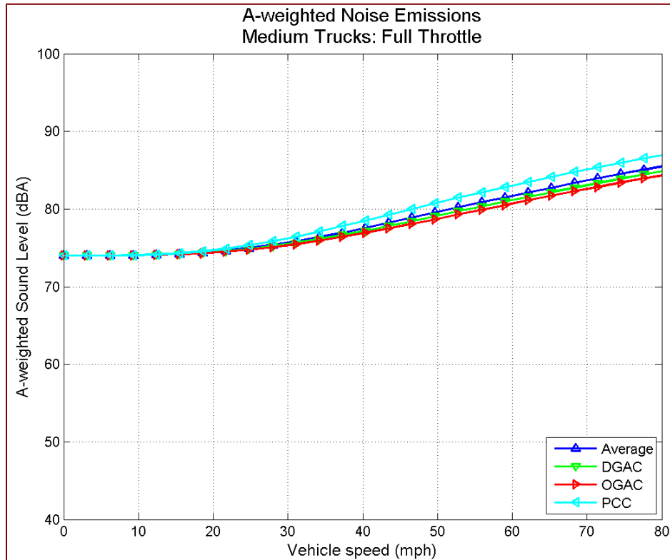
Figure 31 A-weighted sound level emissions as a function of speed: medium trucks, full throttle, by pavement type
