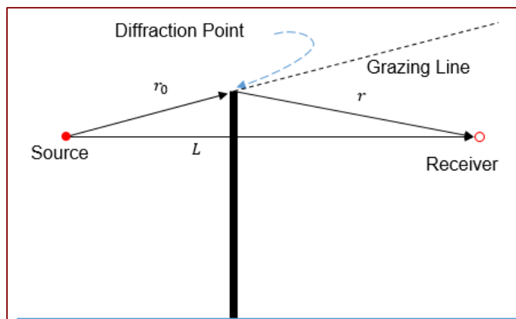
Figure 69 Single Diffraction Geometry
