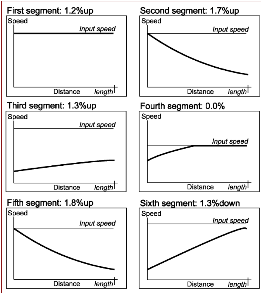
Figure 25 Speeds for Roadway 16 – Upgrades
