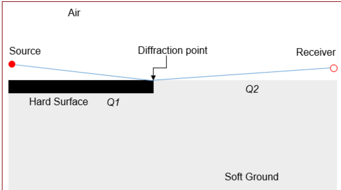
Figure 11 Example Geometry Showing Diffraction due to an Impedance Discontinuity
