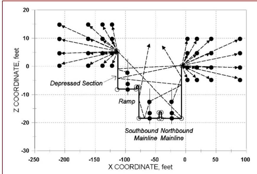
Figure 81 Detailed Input and Representative Rays
