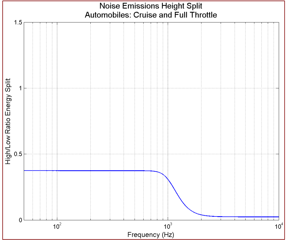
Figure 54 Sound emissions, high/low energy split by frequency: automobiles, cruise, and full throttle
