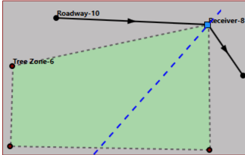
Figure 101 Non-Permitted Shared Point Examples – Plan Builder
