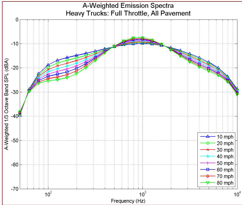
Figure 47 A-weighted emission spectra: heavy trucks, full throttle, all pavements, by speed
