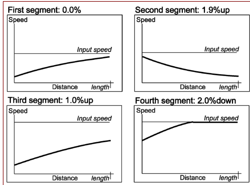
Figure 26 Speeds for Roadway 22 – Traffic-control devices and subsequent grades
