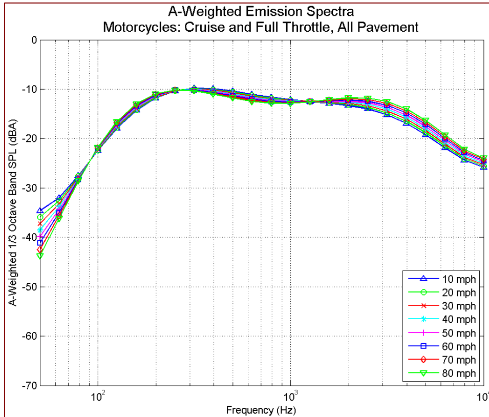
Figure 53 A-weighted emission spectra: motorcycles, all pavements and throttle conditions, by speed
