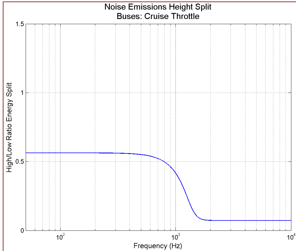
Figure 59 Sound emissions, high/low energy split by frequency: buses, cruise throttle
