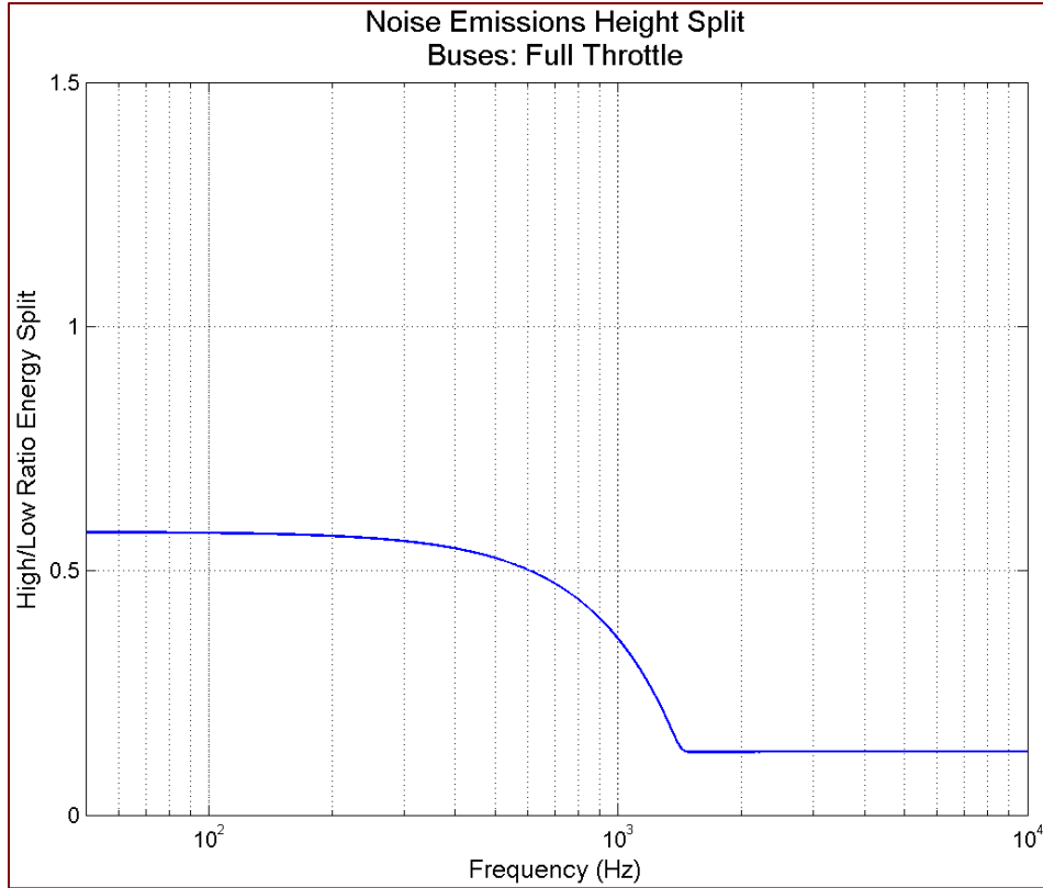
Figure 60 Sound emissions, high/low energy split by frequency: buses, full throttle
