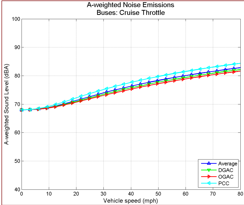
Figure 34 A-weighted sound level emissions as a function of speed: buses, cruise throttle, by pavement type
