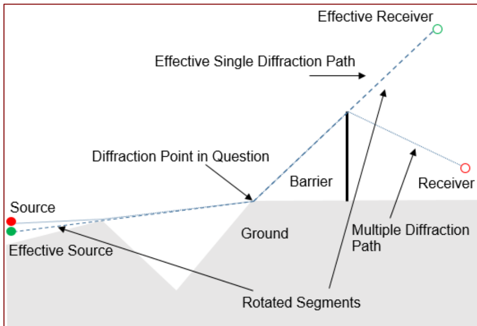
Figure 70 Example of Multiple Diffractions
