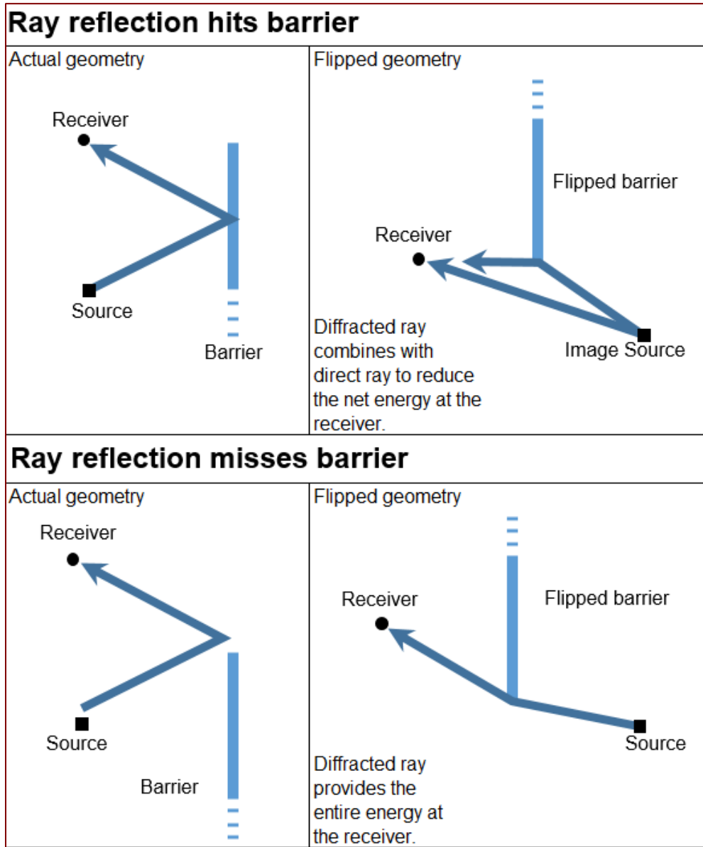
Figure 82 Partial Reflection near tops of Parallel Barriers
