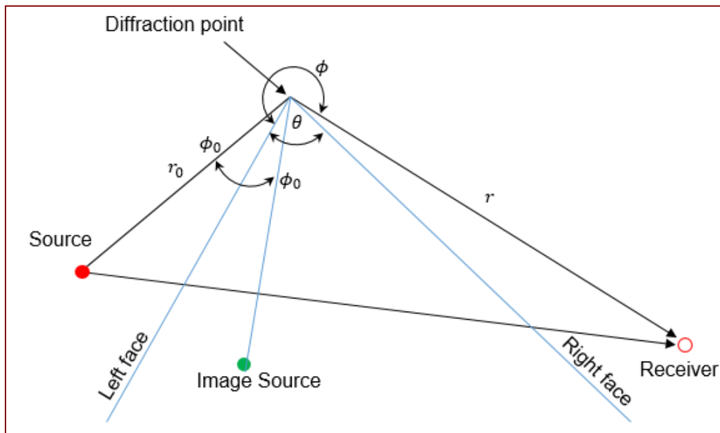
Figure 74 Diffraction Geometry
