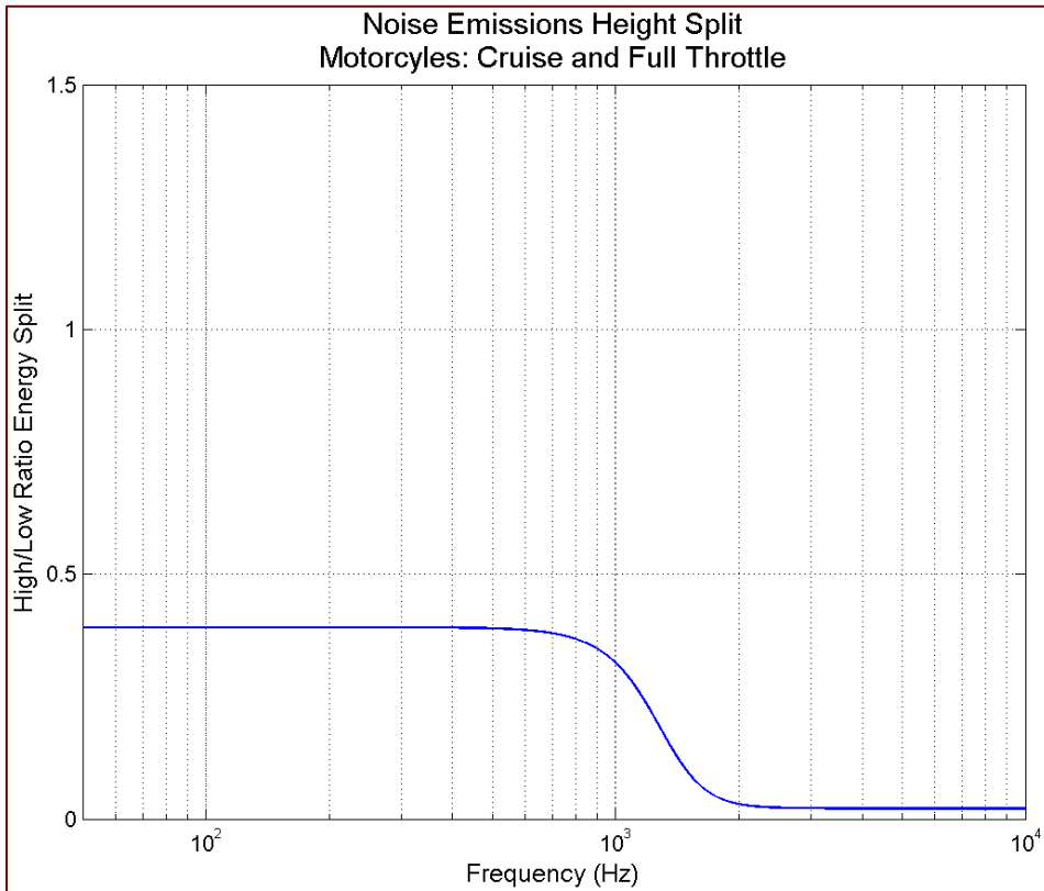
Figure 61 Sound emissions, high/low energy split by frequency: motorcycles, cruise and full throttle
