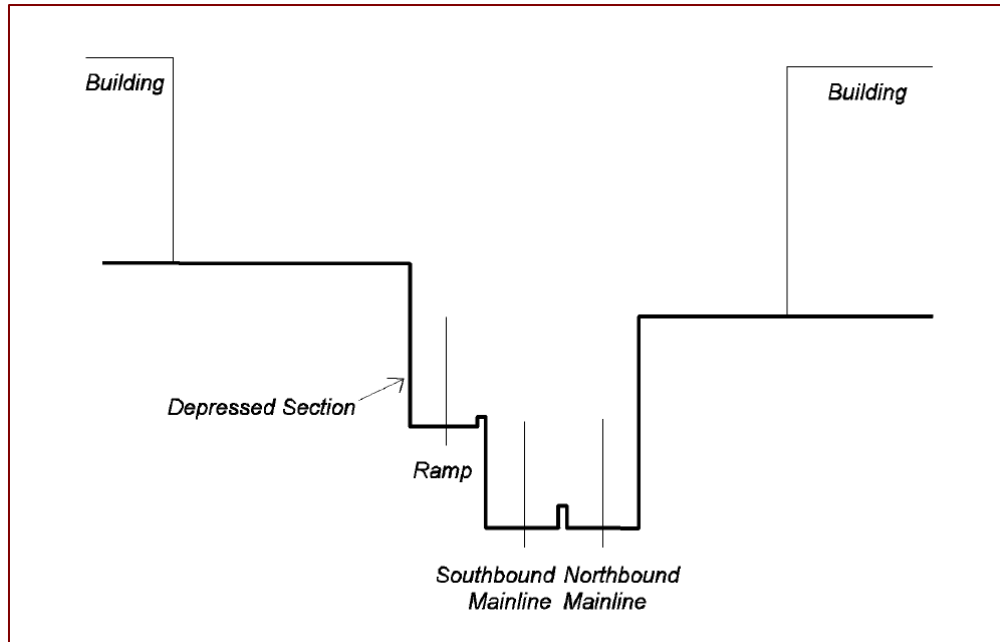
Figure 80 Typical Depressed Section in a Highly Urbanized Area
