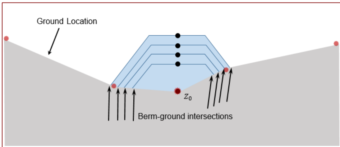
Figure 67 Example Berm, Shown at Four Perturbation Heights
