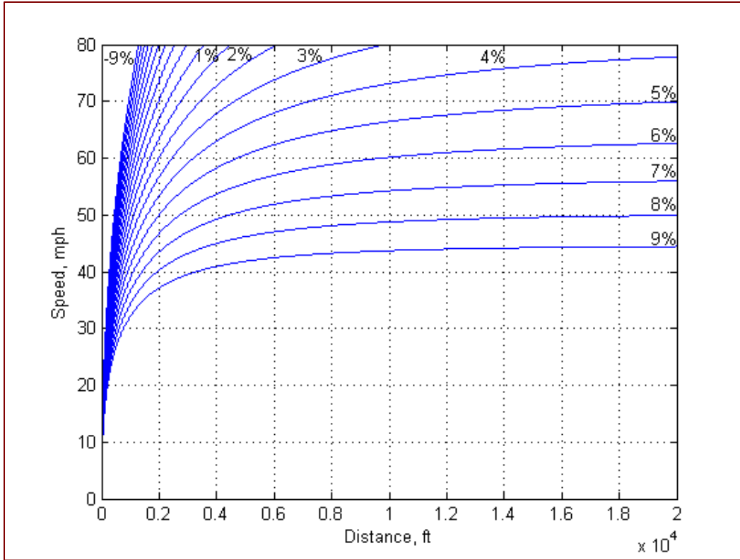
Figure 21 Acceleration away from traffic-control devices: Automobiles and motorcycles
