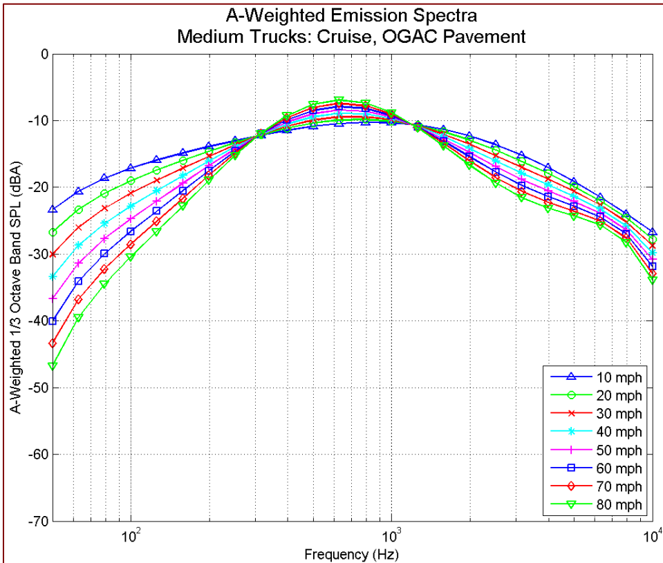
Figure 45 A-weighted emission spectra: medium trucks, cruise throttle, OGAC pavement, by speed
