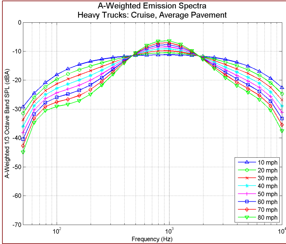
Figure 48 A-weighted emission spectra: heavy trucks, cruise throttle, average pavement, by speed
