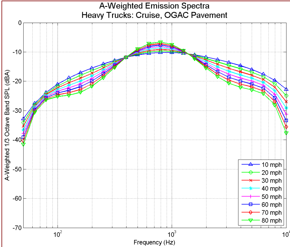
Figure 50 A-weighted emission spectra: heavy trucks, cruise throttle, OGAC pavement, by speed
