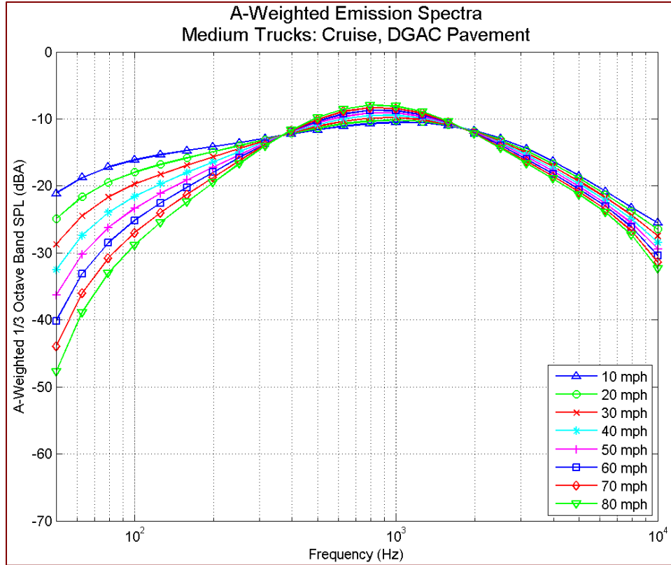
Figure 44 A-weighted emission spectra: medium trucks, cruise throttle, DGAC pavement, by speed
