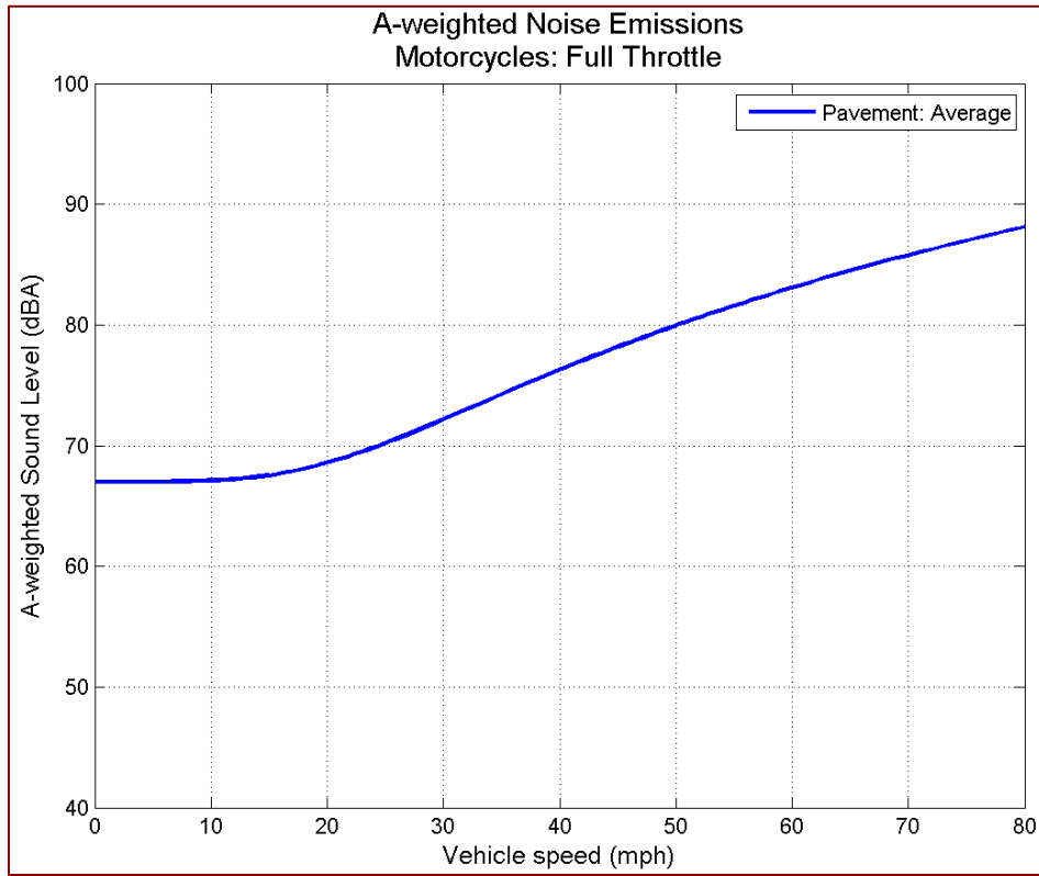
Figure 37 A-weighted sound level emissions as a function of speed: motorcycles, full throttle, average pavement
