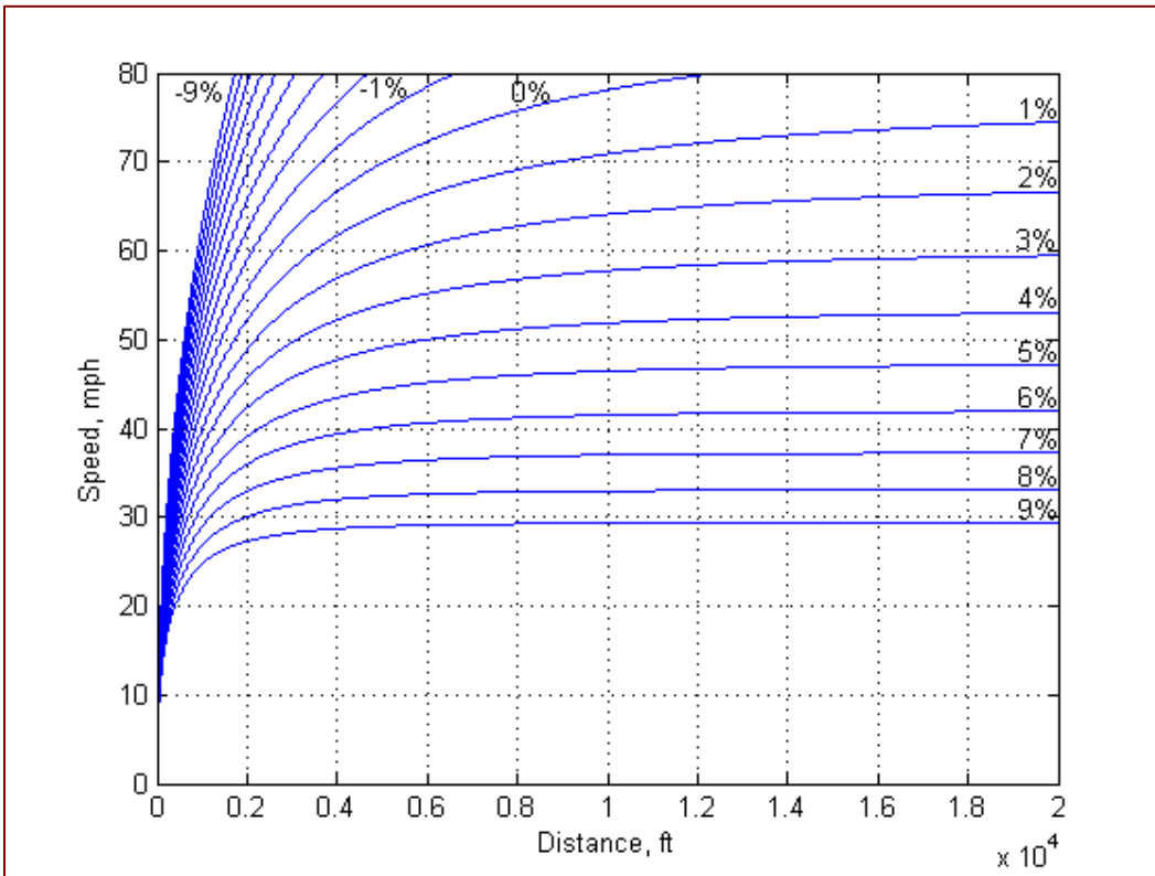
Figure 22 Acceleration away from traffic-control devices: medium trucks and buses
