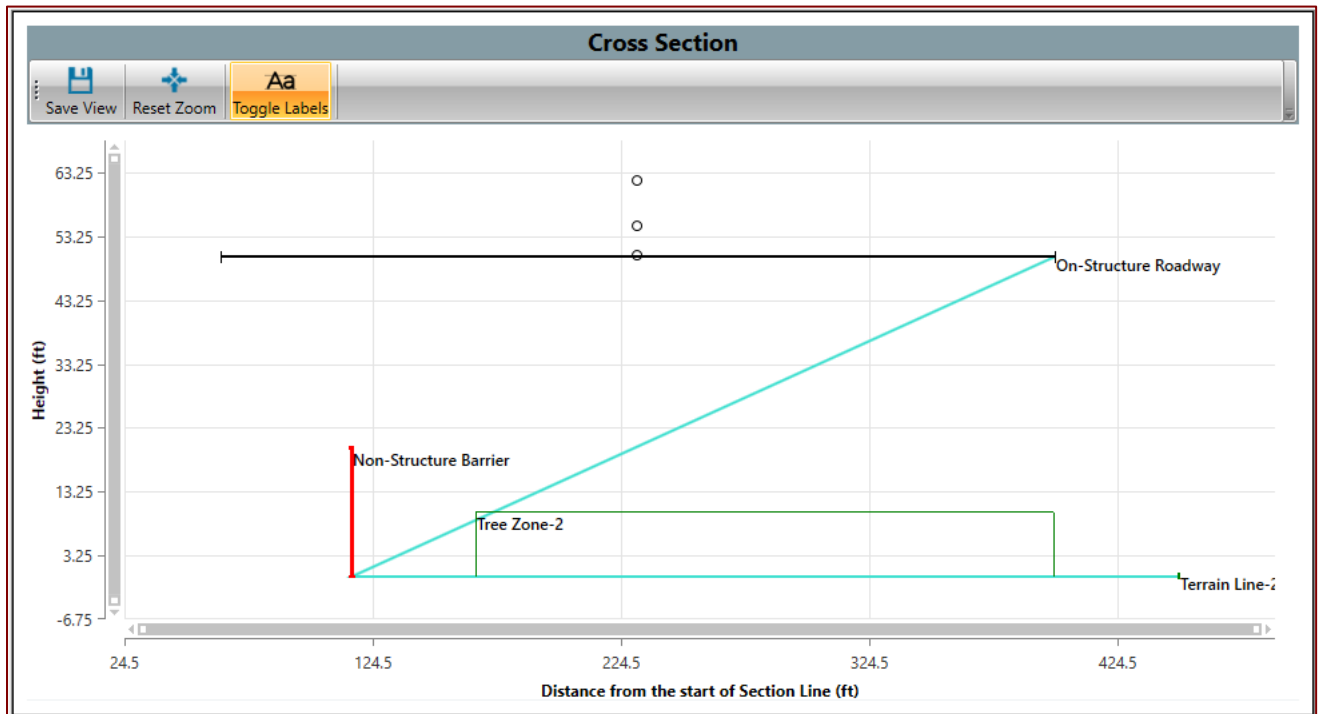
Figure 90 Permitted On-Structure/Non-Structure Crossing Examples – Section View
