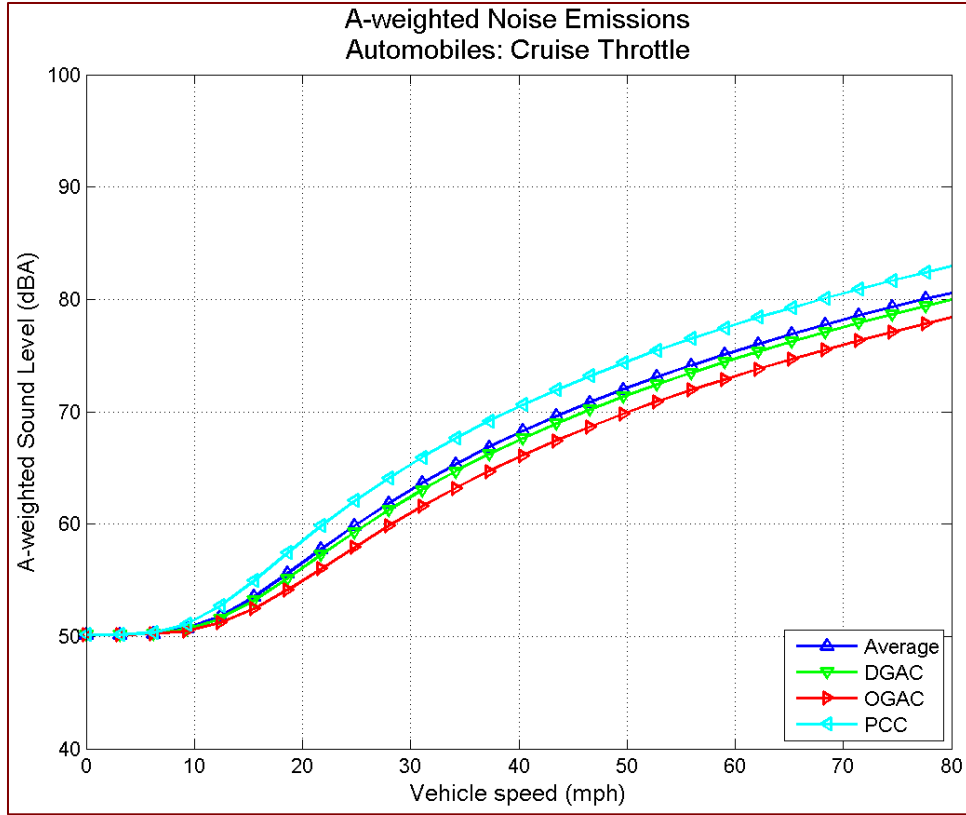
Figure 28 A-weighted sound level emissions as a function of speed: automobiles, cruise throttle, by pavement type
