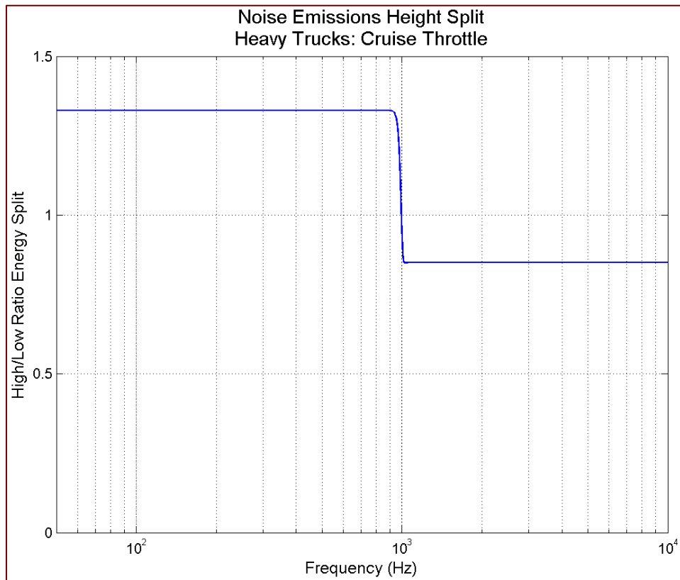
Figure 57 Sound emissions, high/low energy split by frequency: heavy trucks, cruise throttle
