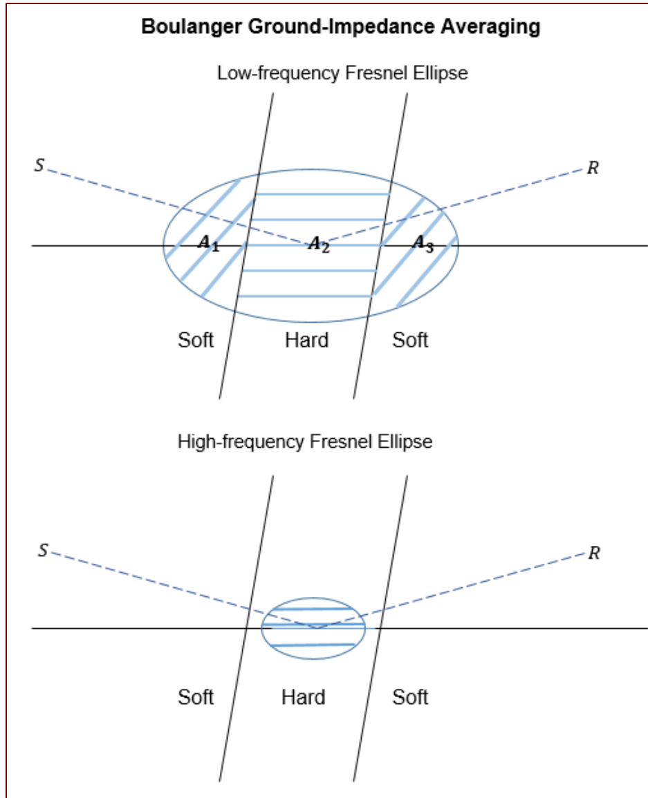
Figure 78 Ground Impedance Evaluation at Two Frequencies
