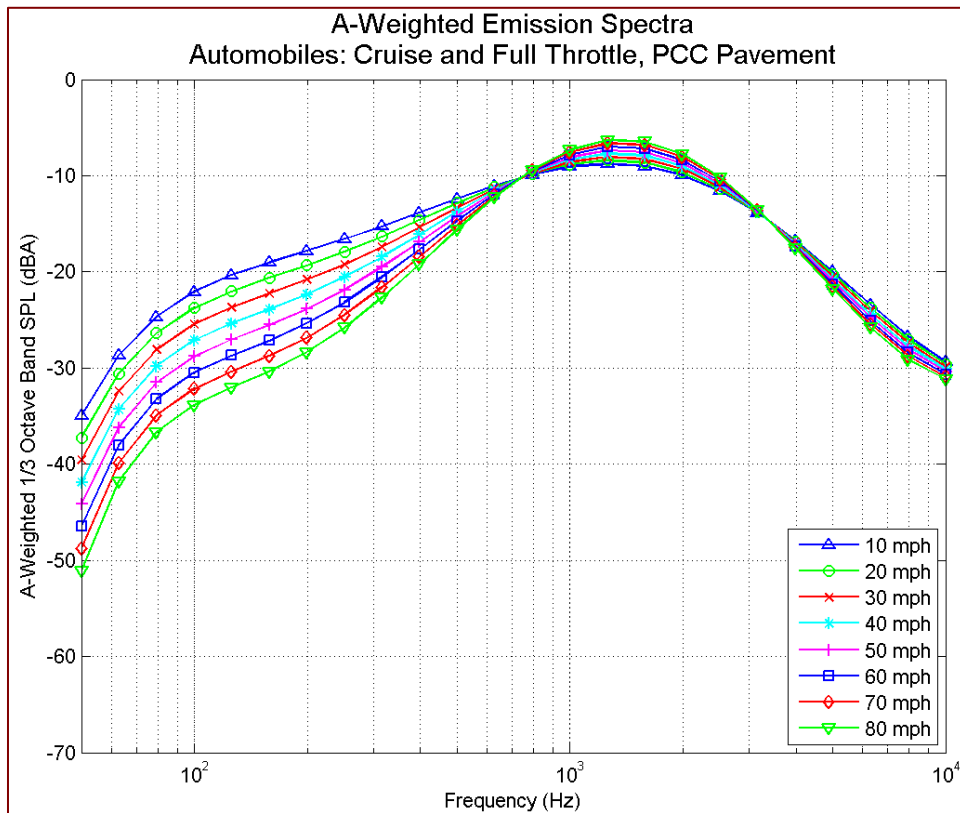
Figure 41 A-weighted emission spectra: automobiles, all throttle conditions, PCC pavement, by speed
