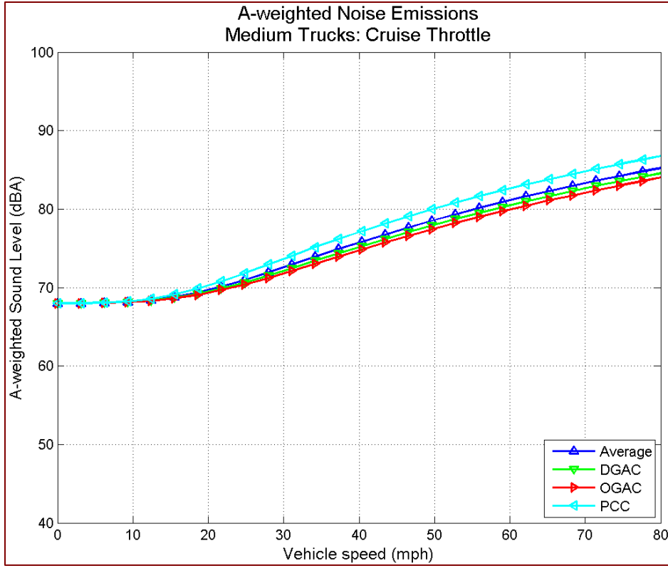
Figure 30 A-weighted sound level emissions as a function of speed: medium trucks, cruise throttle, by pavement type
