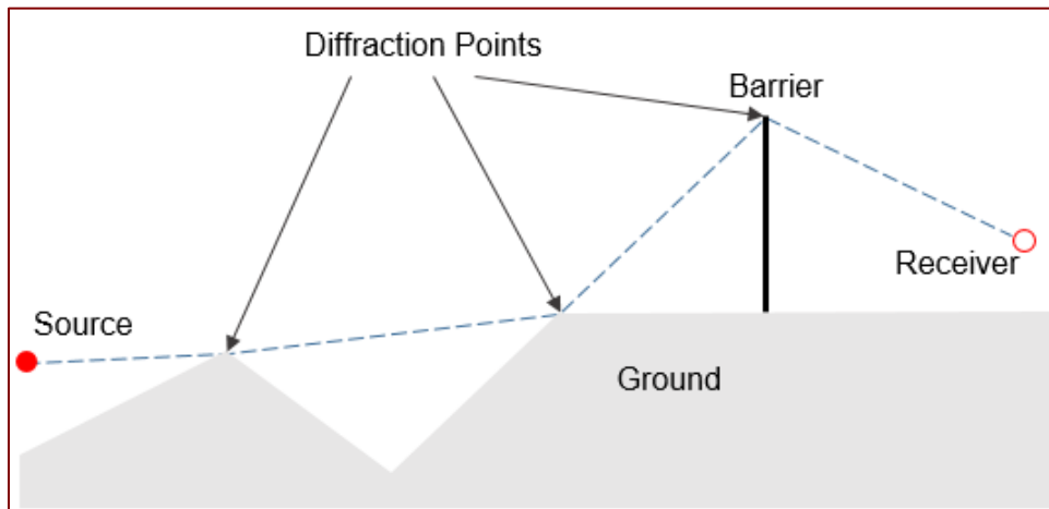
Figure 70 Example of Multiple Diffractions
