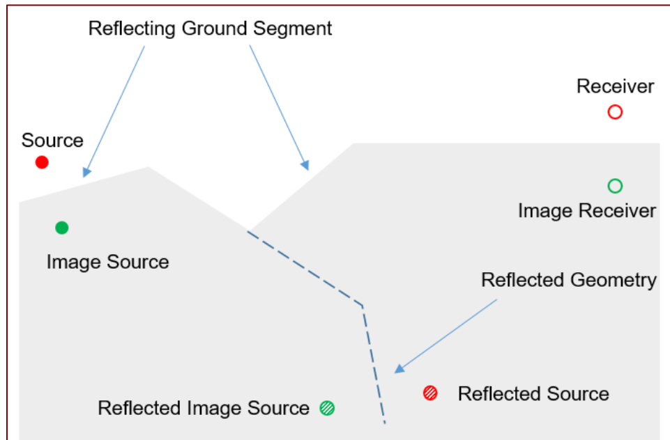
Figure 72 Example of a Geometry with Reflections
