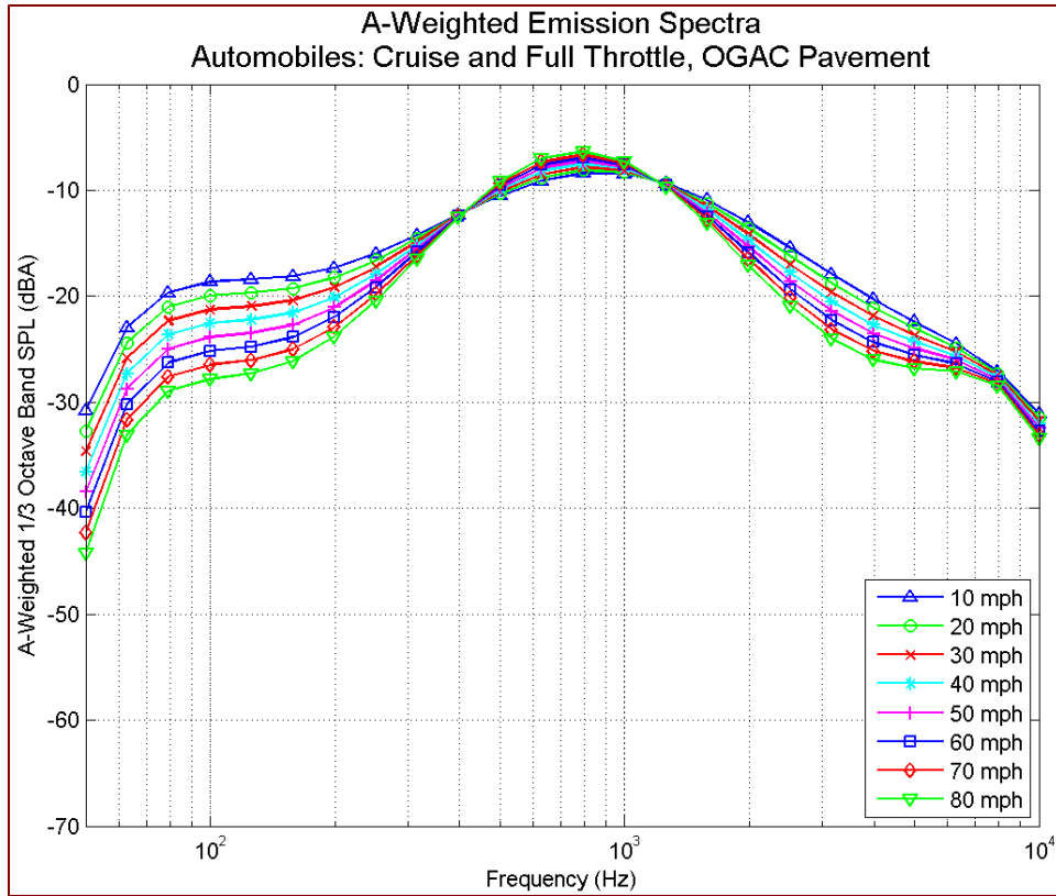
Figure 40 A-weighted emission spectra: automobiles, all throttle conditions, OGAC pavement, by speed
