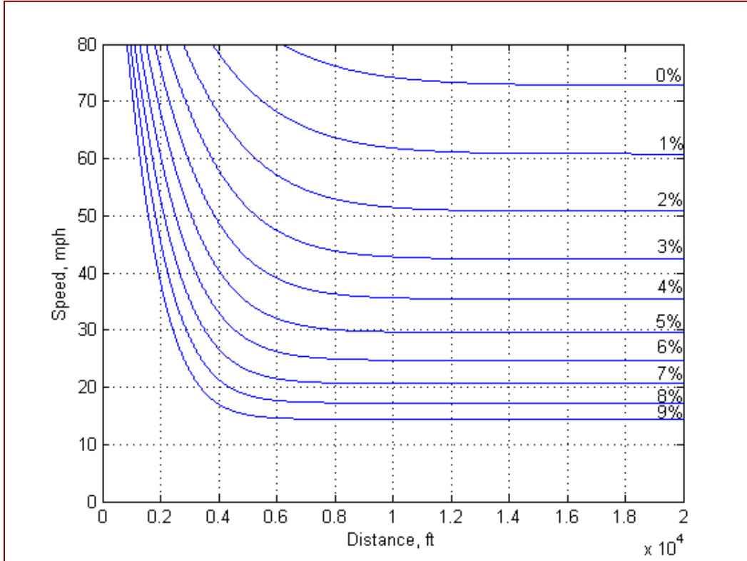
Figure 24 Deceleration caused by upgrades 1.5 percent or more: Heavy trucks
