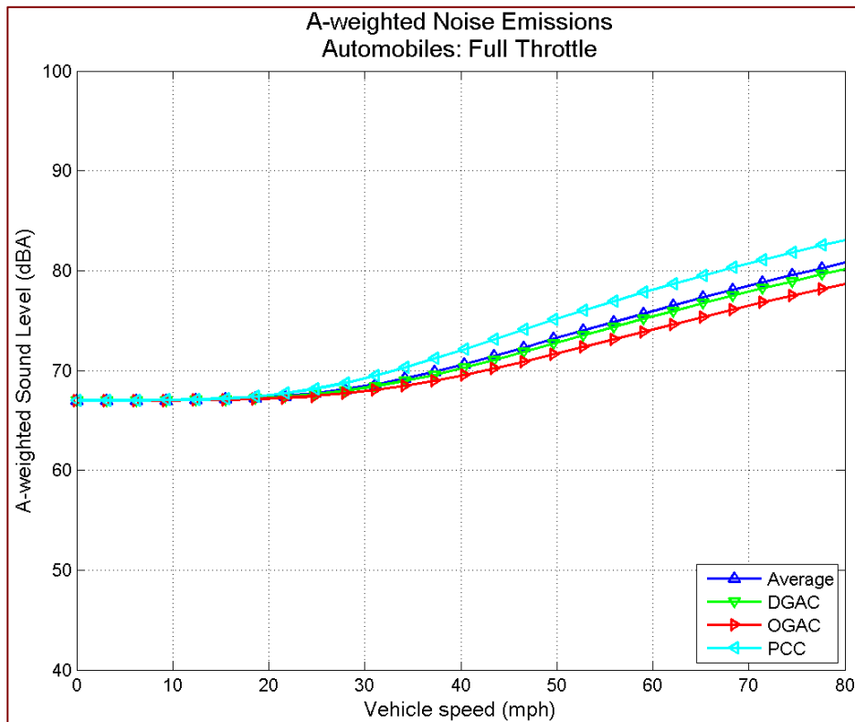
Figure 29 A-weighted sound level emissions as a function of speed: automobiles, full throttle, by pavement type
