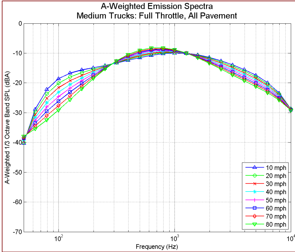
Figure 42 A-weighted emission spectra: medium trucks, full throttle, all pavements, by speed
