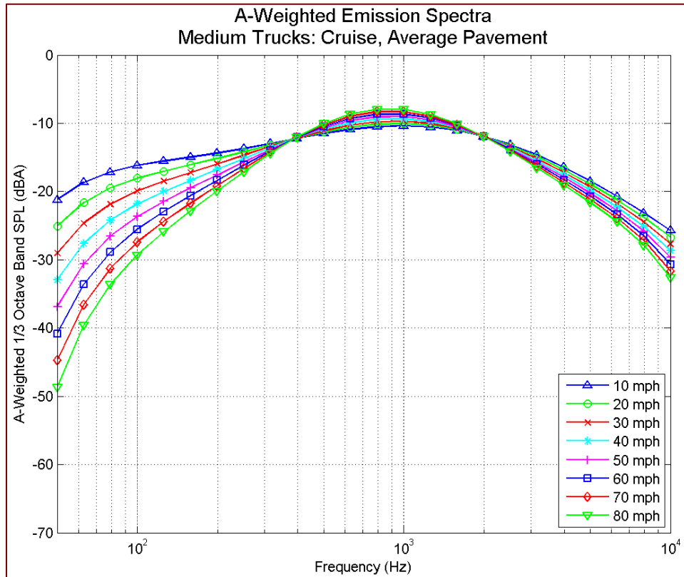
Figure 43 A-weighted emission spectra: medium trucks, cruise throttle, average pavement, by speed
