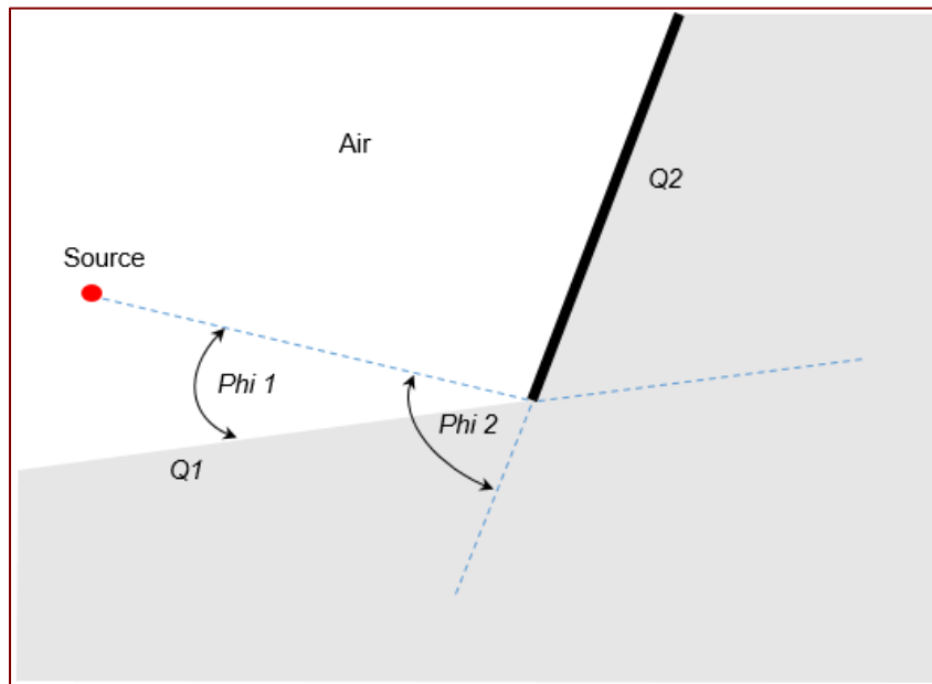
Figure 77 Example Geometry for Corner Diffraction
