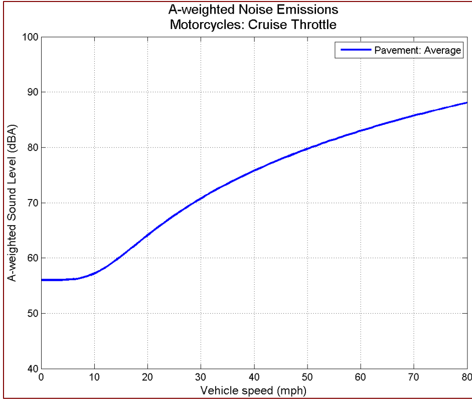
Figure 36 A-weighted sound level emissions as a function of speed: motorcycles, cruise throttle, average pavement
