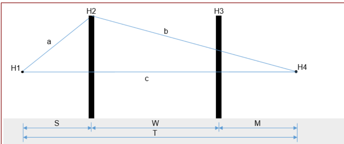
Figure 79 Foss Double-Barrier Geometry
