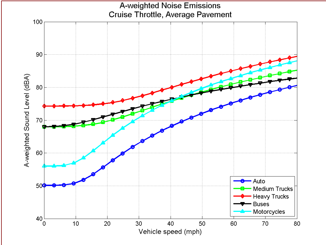
Figure 6 A-Weighted Reference Energy Mean Emission Levels under Cruise Conditions
