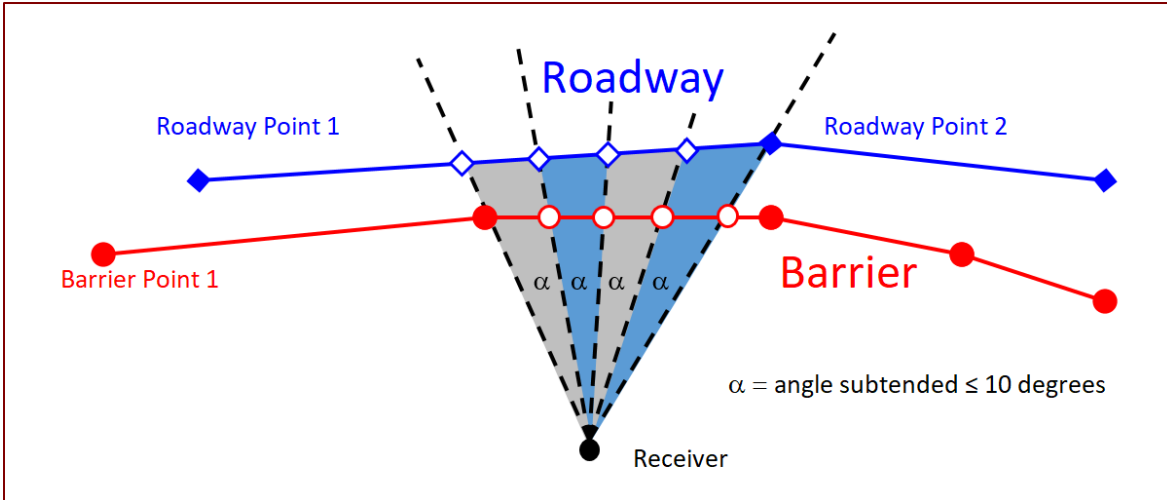
Figure 63 Maximum Elemental Triangle Set to 10 Degrees
