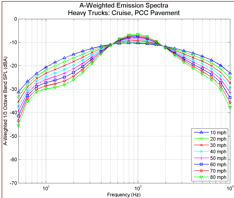
Figure 51 A-weighted emission spectra: heavy trucks, cruise throttle, PCC pavement, by speed
