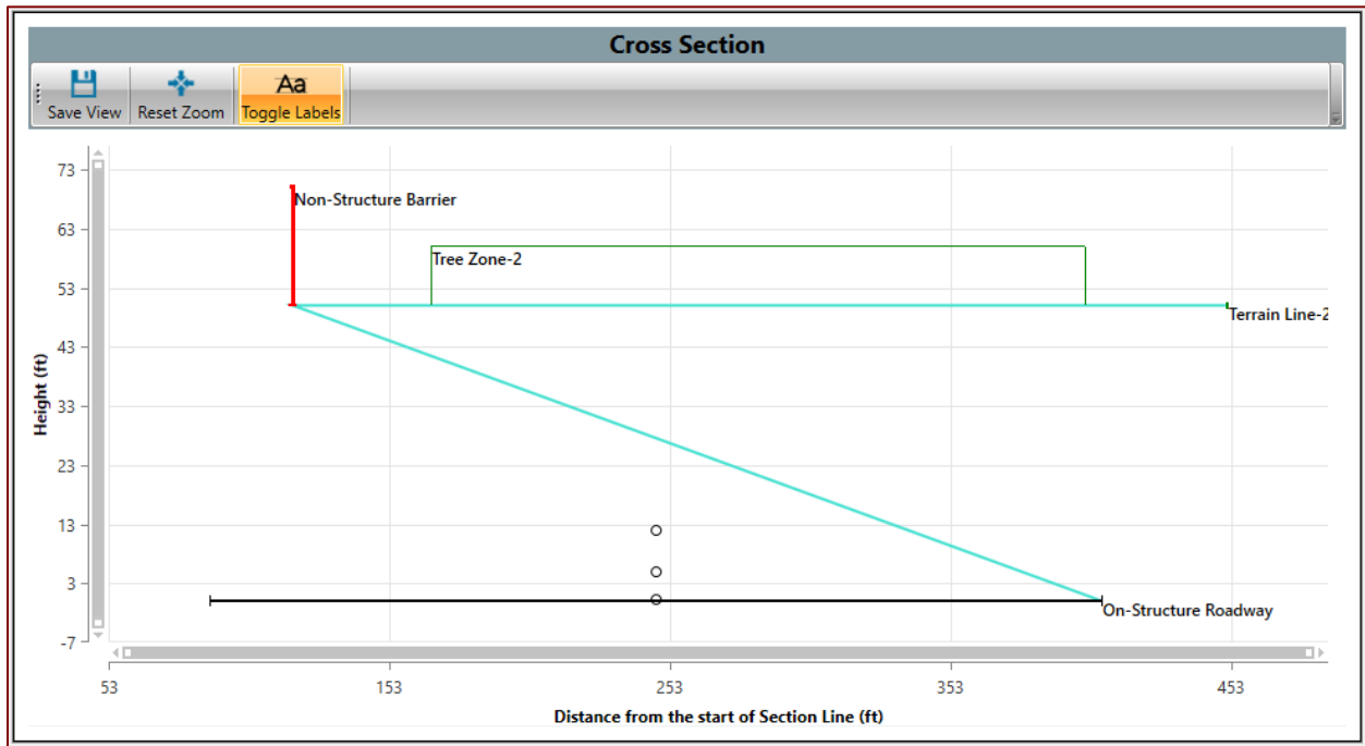
Figure 92 Non-Permitted On-Structure/Non-Structure Crossing Examples – Section View
