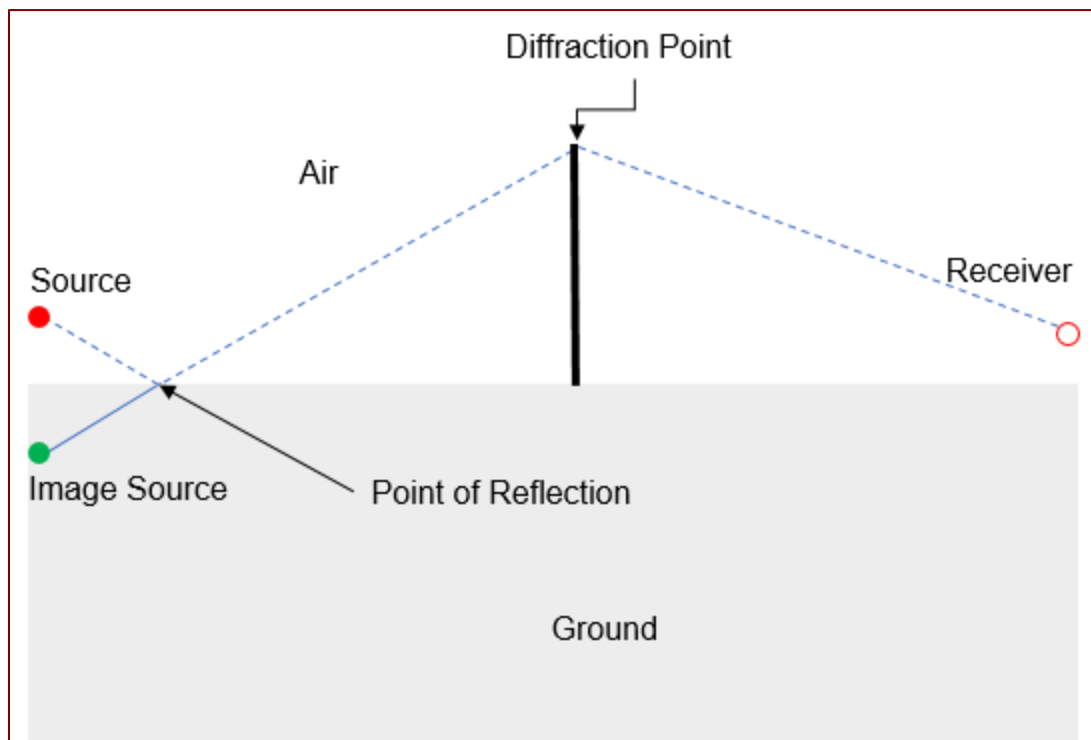
Figure 10 Example Geometry Showing a Reflection and Diffraction due to Change in Vertical Geometry
