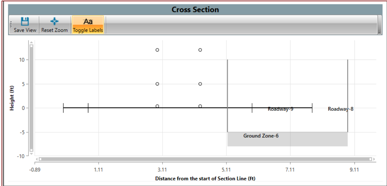
Figure 106 Permitted Within Roadway Pavement Width Examples – Section View
