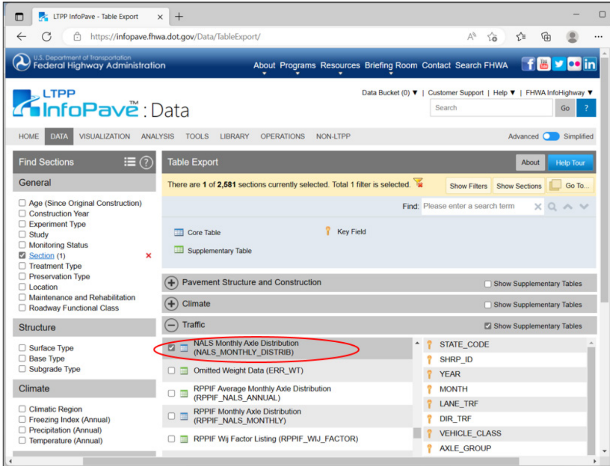
Figure 17. Screenshot. InfoPave Table Export menu with a checkbox showing “selected” next to the traffic table label, “NALS Monthly Axle Distribution (NALS_MONTHLY_DISTRIB).” (3)
