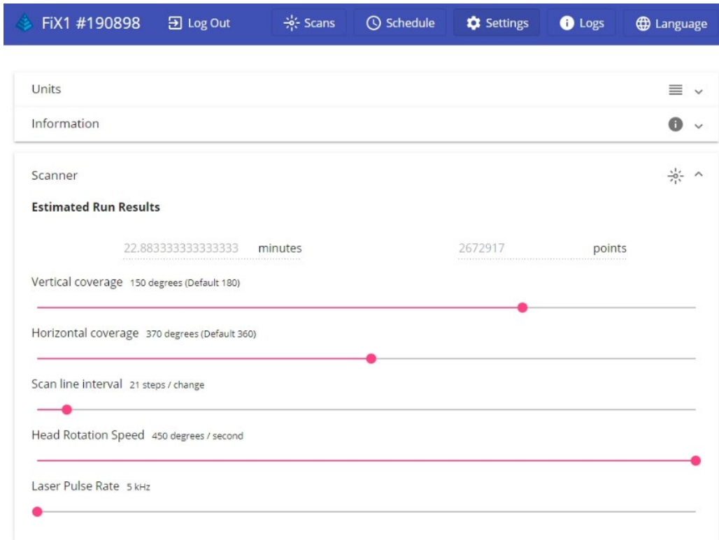
Figure 7.5. Carlson FiX1 scan settings screen.
