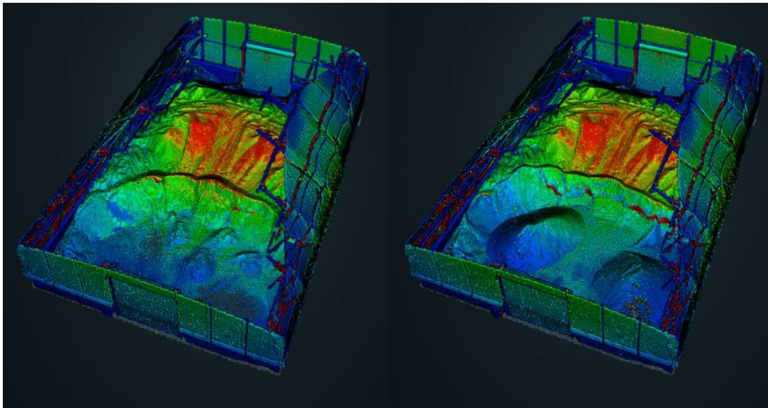
Figure 7.3. Point cloud renderings of the Delaware DOT pile in two configurations (Conditions D1, left, and D2, right).
