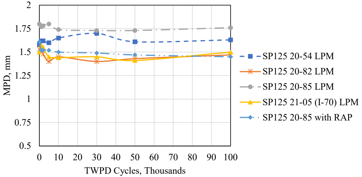
Figure 5-15 MPD of fabricated slabs at different TWPD cycles for, (a) plant produced mixes, and (b) lab produced mixtures
