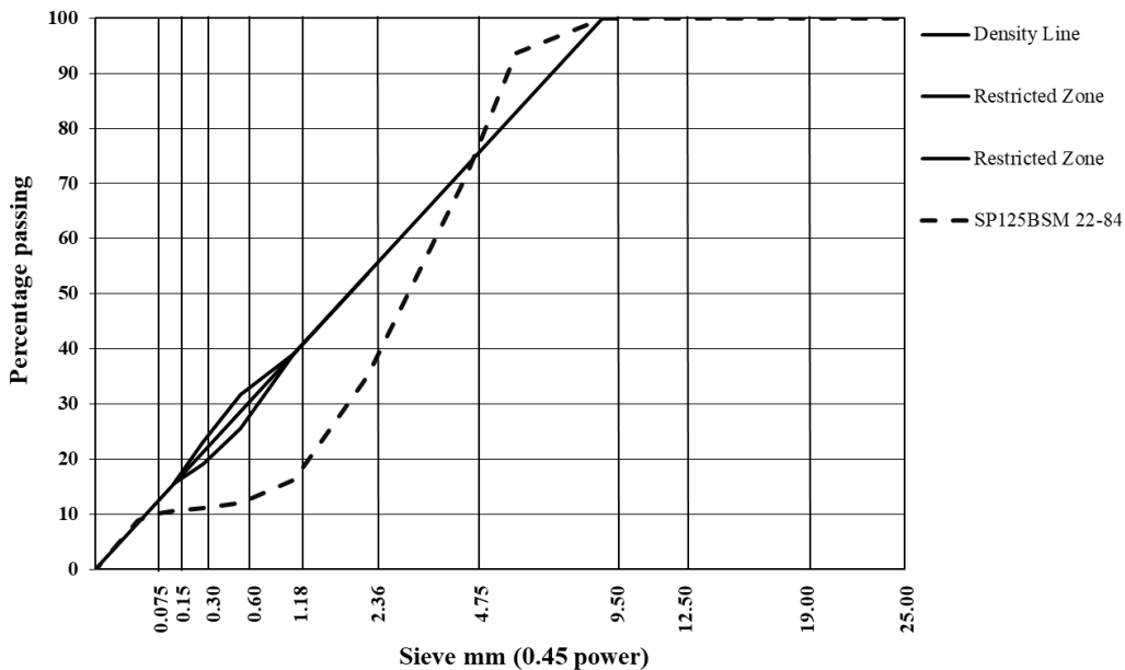
Figure 5-18 Aggregate gradation for I-70 Cooper County mix (SP125BSM 22-84)
