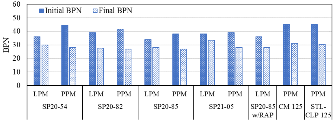
Figure 5-14 BPN results of investigated mixtures
