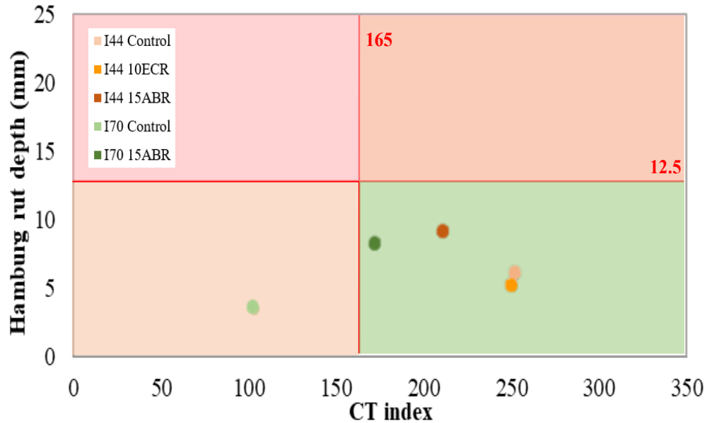
Figure 4-2 Hamburg-CT interaction plot
