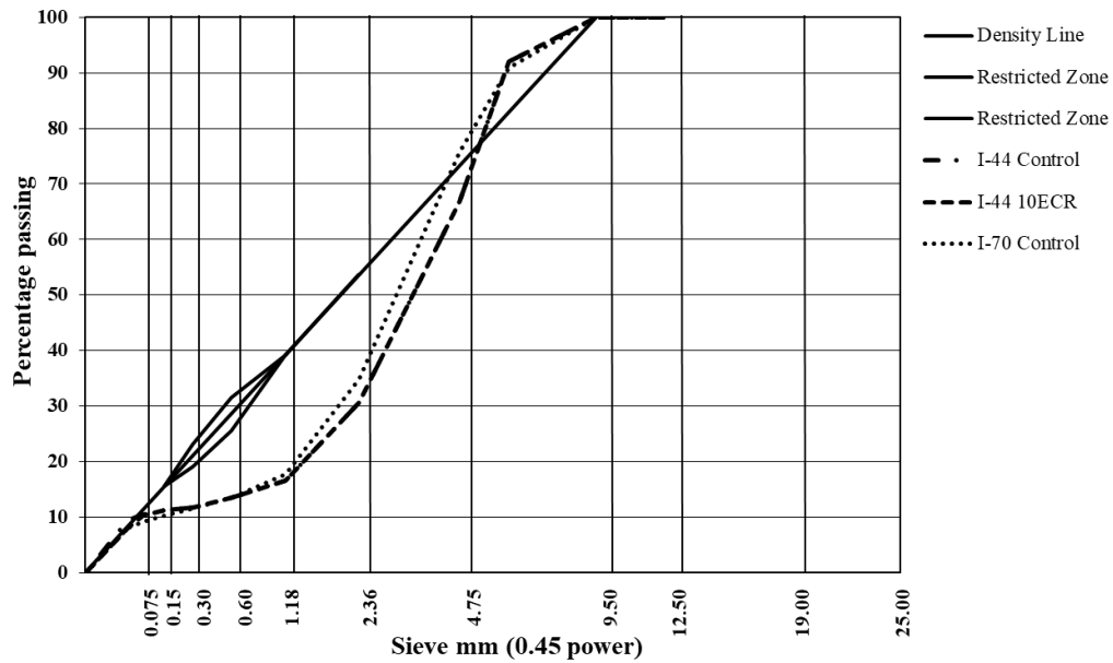
Figure 2-1 Aggregate gradation used for all mixes
