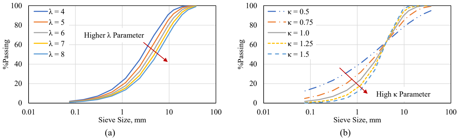
Figure B-9-1 Mix gradation impact on value of Weibull distribution parameters. (a) Impact of mix gradation, \lambda parameter and (b) impact of mix gradation, \kappa parameter
