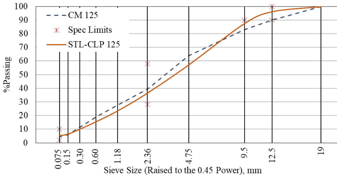
(b) DG mixtures
