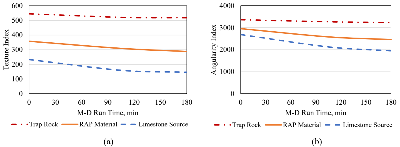
Figure 5-12 (a & b) Texture and angularity indices of RAP aggregate material source which included trap rock and limestone.
