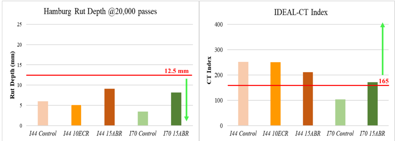
Figure 4-1 Performance of mixes in (a) IDEAL-CT test and (b) Hamburg rutting test (red line represents the threshold)
