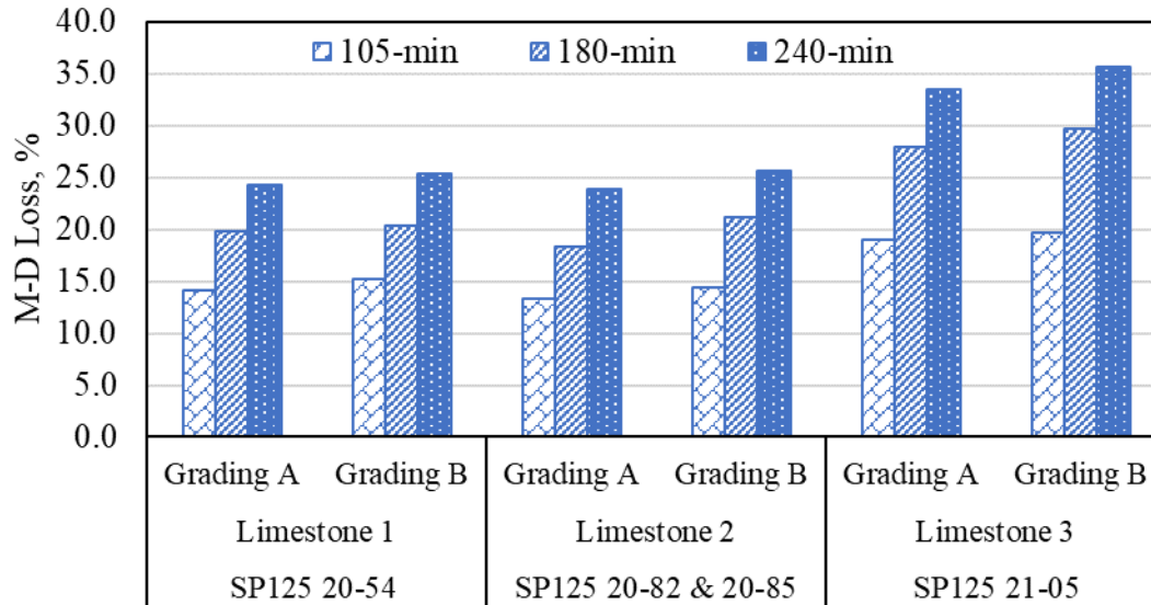
Figure 5-10 MD abrasion loss percentage for different gradings at different run times
