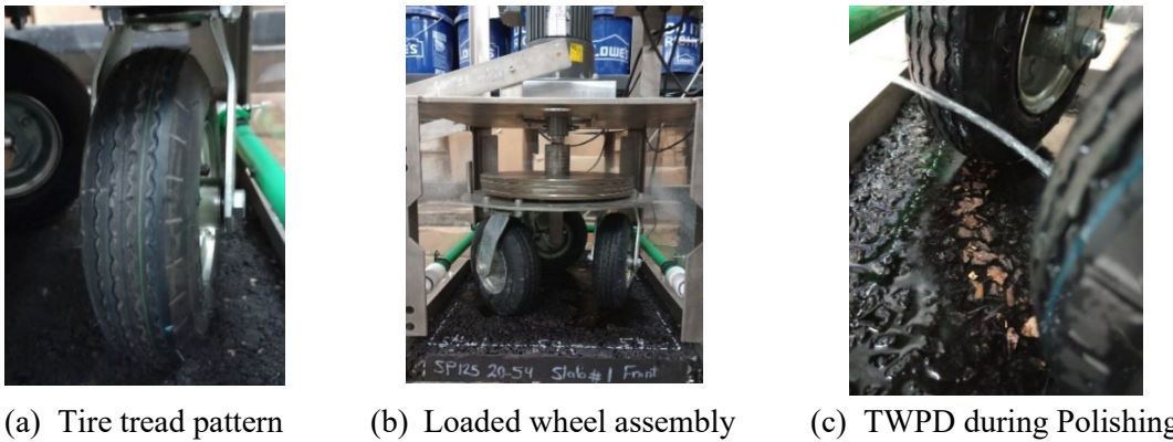
Figure 5-5 NCAT three-wheel polishing device
