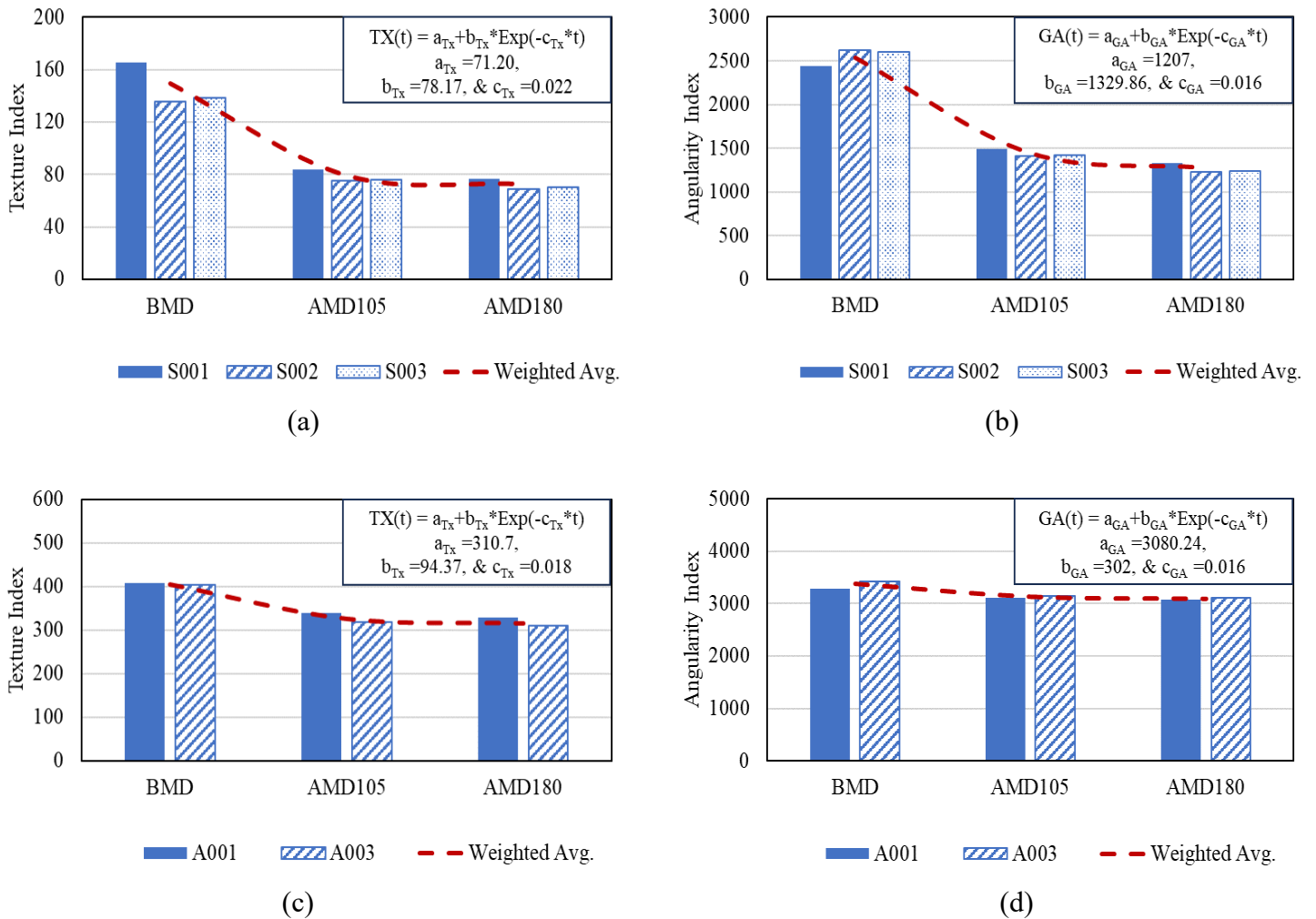
Figure 5-11. The Texture and Angularity Indices of aggregate sources of SP125 21-05 (I-70) (BMD = Before M-D polishing, AMD = After M-D polishing). (a) Texture Index of Trap Rock 1, (b) Angularity Index of Trap Rock 1, (c) Texture Index of Limestone 3, (d) Angularity Index of Limestone 3,
