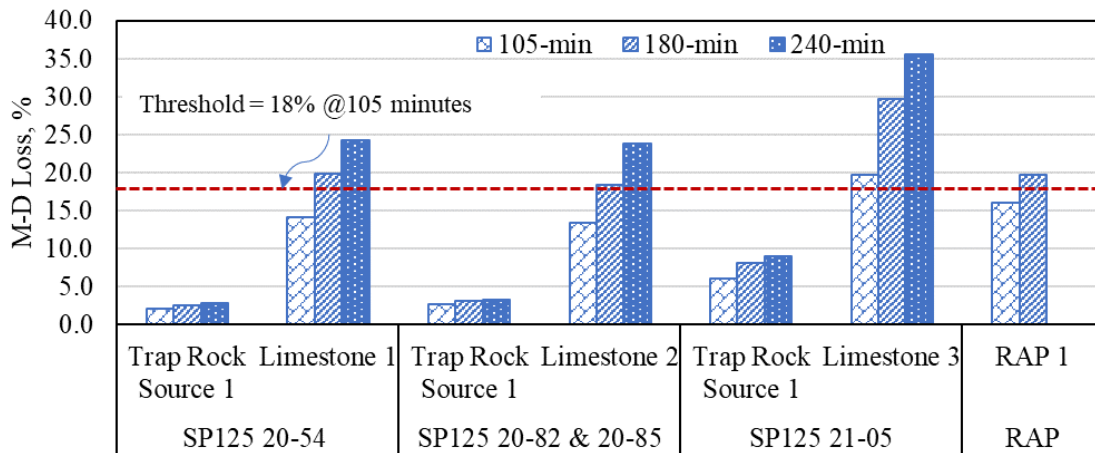
Figure 5-9 MD abrasion loss percentage for investigated aggregates
