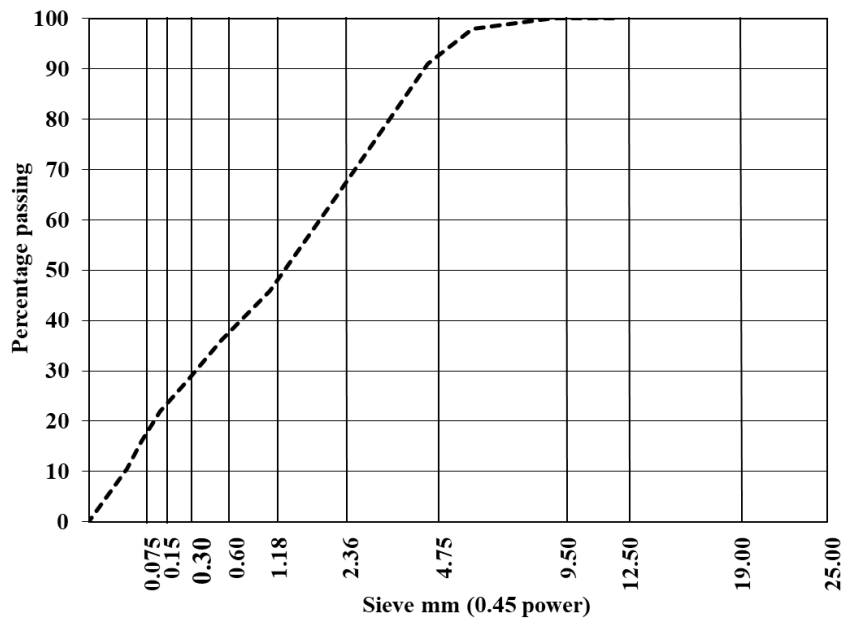
Figure 2-2 Aggregate gradation used for RAP stockpile
