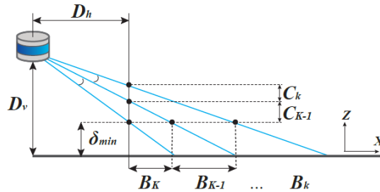
Figure 9. Graph. Horizontal/vertical spacing between points in the ZX plane at \delta_{min} . The mounting height D_v and setback distance D_h from the road affect the spacing [33].
