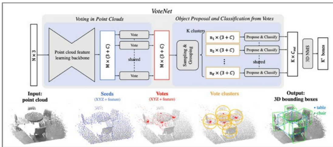
Figure 22. Diagram. VoteNet architecture [95].
