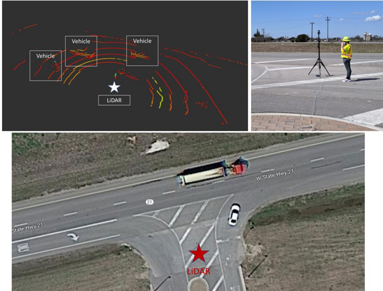
Figure 31. Graph and photos. The data collection site on the RELIS Campus (02-TAMU).
