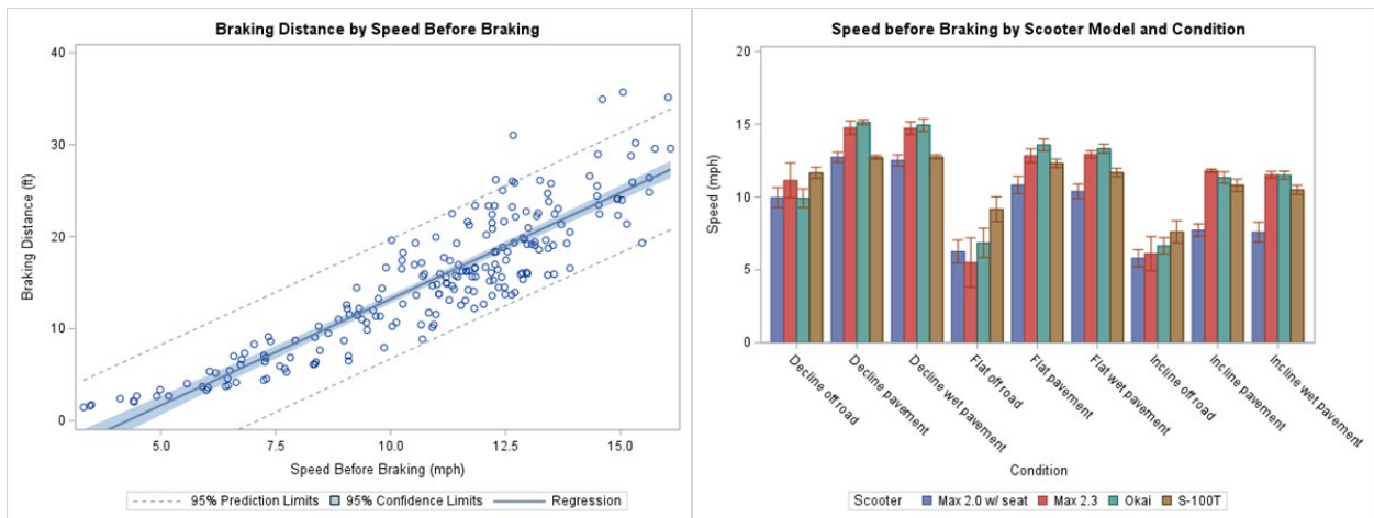
Figure 23. Braking distance by speed before braking (left) and by scooter model and condition (right).
