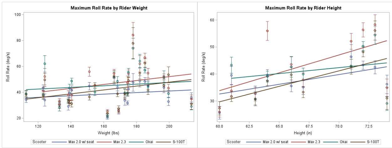
Figure 27. Maximum roll rate by rider weight (left) and by rider height (right).
