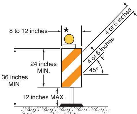
VERTICAL PANEL
