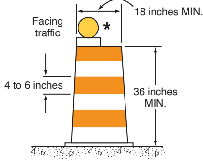
DRUM
