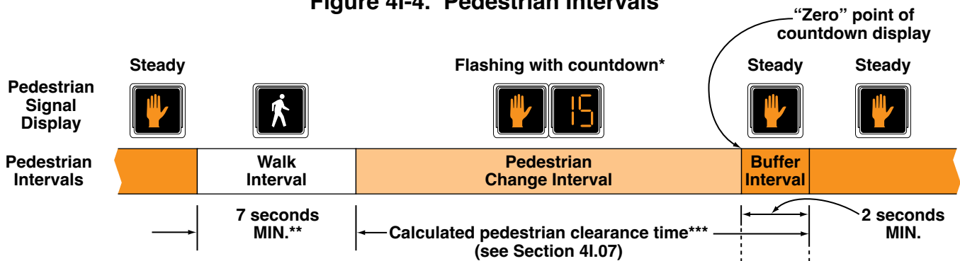
Figure 4I-4. Pedestrian Intervals
