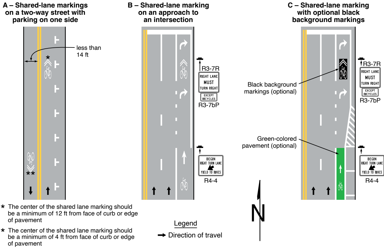
Figure 9E-9. Examples of Shared-Lane Marking Applications
