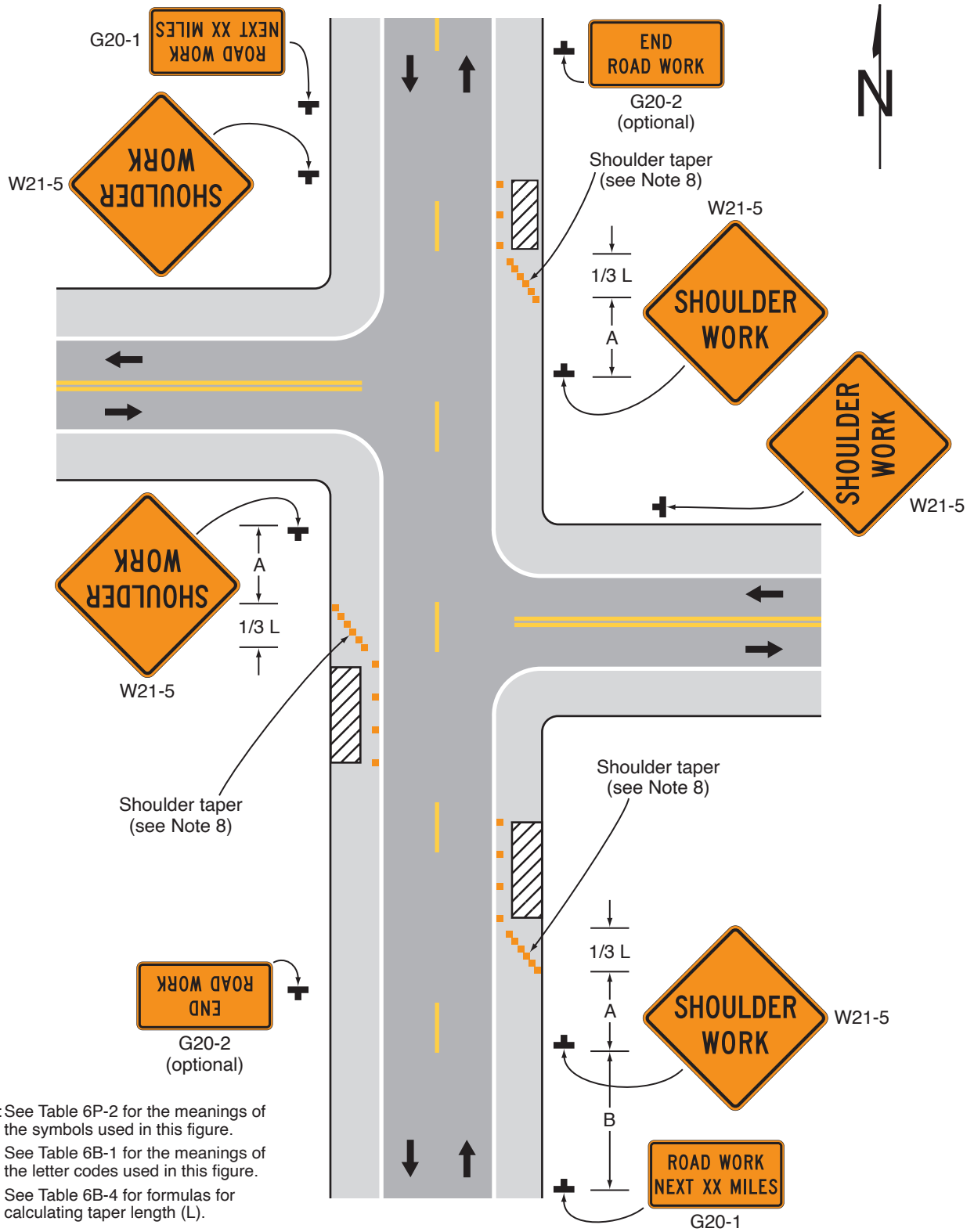
Typical Application 3
