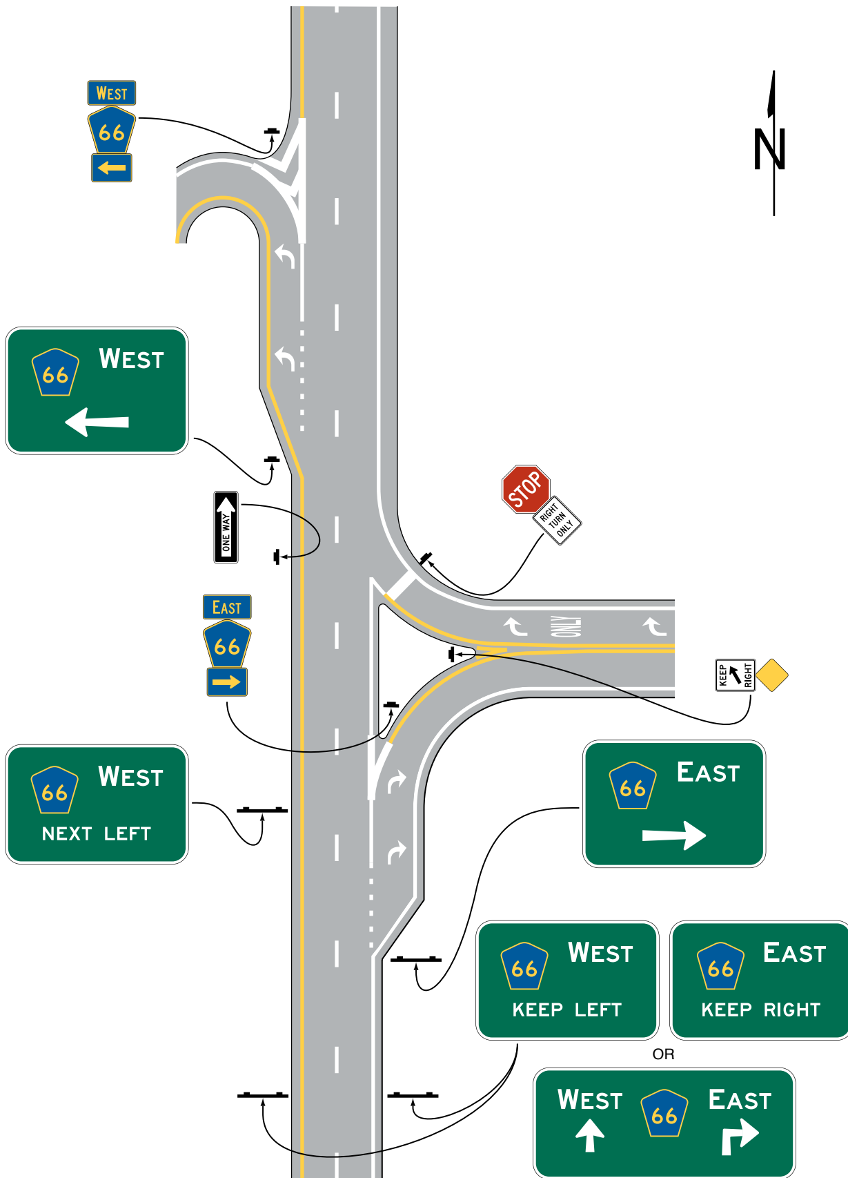
A – Intercepted crossroad with left turns prohibited
