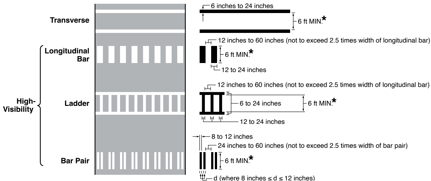
Figure 3C-1. Crosswalk Markings
