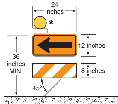
DIRECTION INDICATOR BARRICADE **
