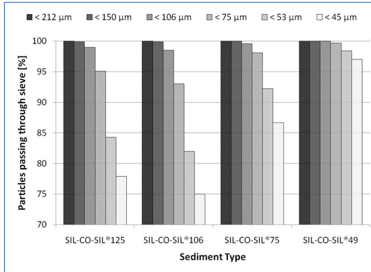
Figure 3. Particle Size Distributions.
