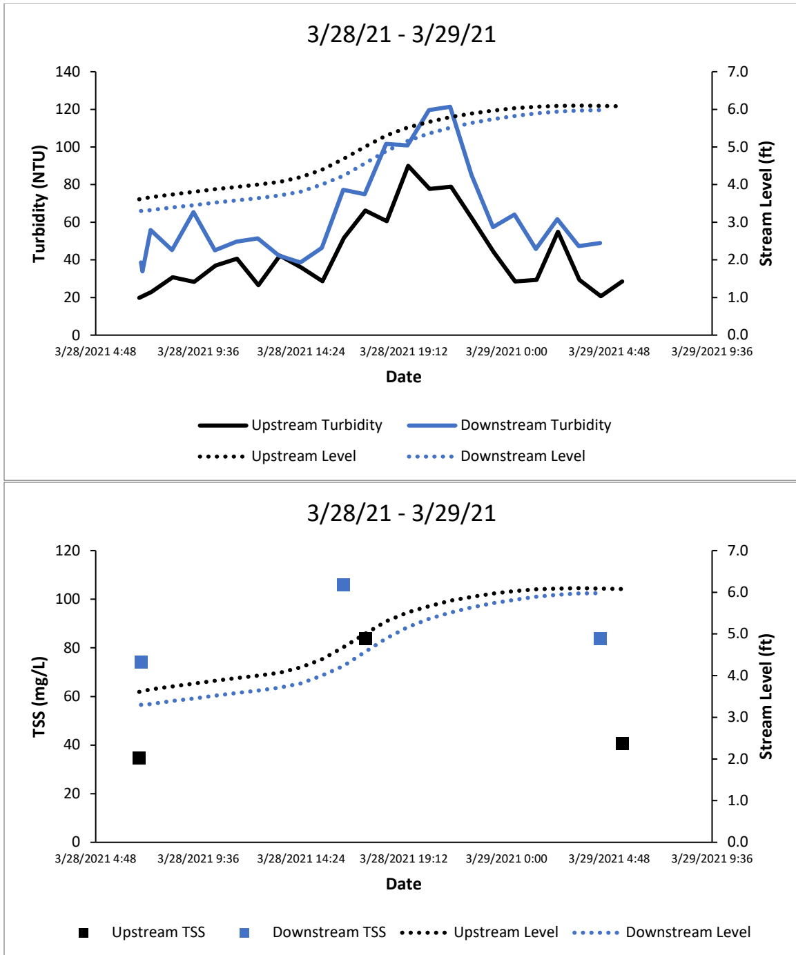
Figure A46. Turbidity (top) and TSS (bottom) in Swift Creek.
