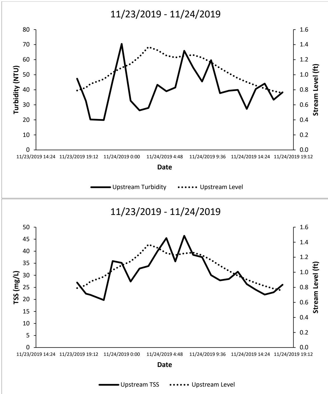
Figure A27. Turbidity (top) and TSS (bottom) in Swift Creek.
