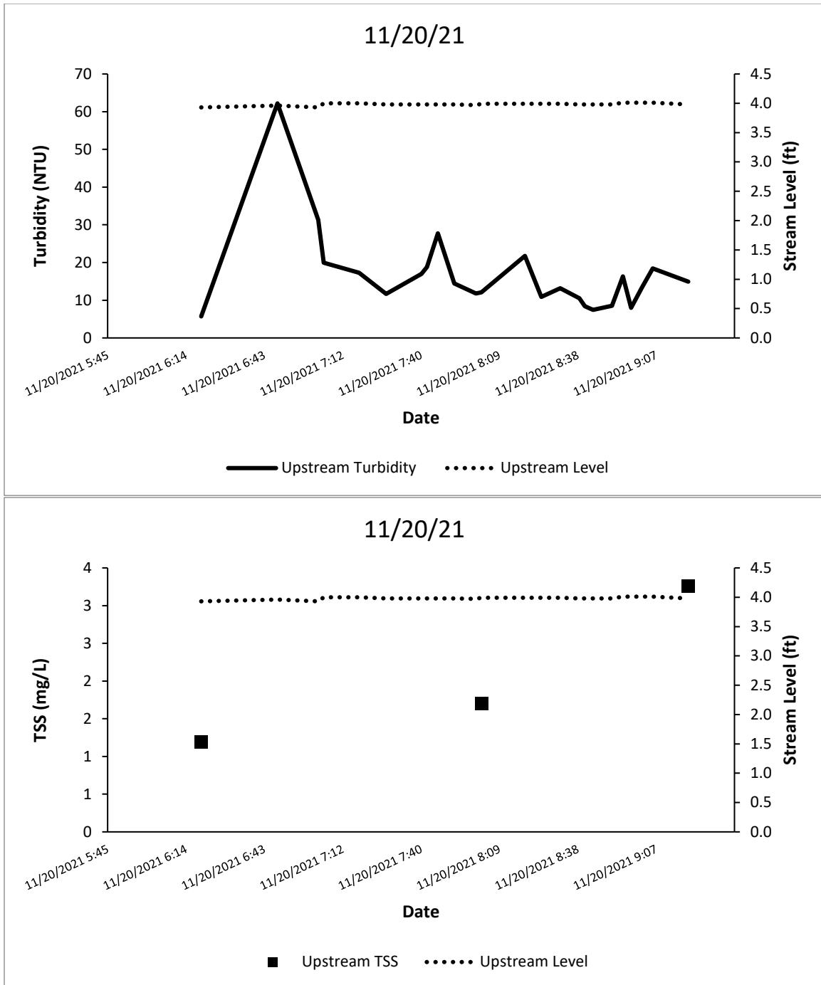
Figure A52. Turbidity (top) and TSS (bottom) in Swift Creek.
