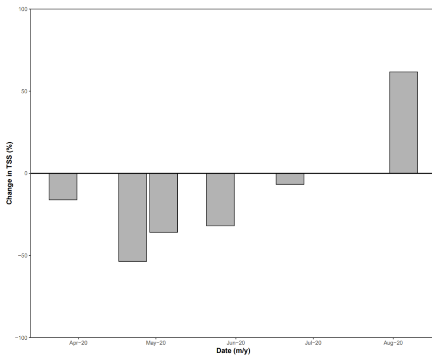
Figure A16. Average TSS change for basin 1 per storm event.
