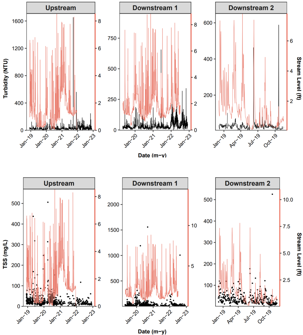
Figure 23. Swift Creek daily turbidity and TSS. The red line is Swift Creek level as noted by the red right-hand y-axis. Black line and black dots represent the turbidity and TSS respectively.
