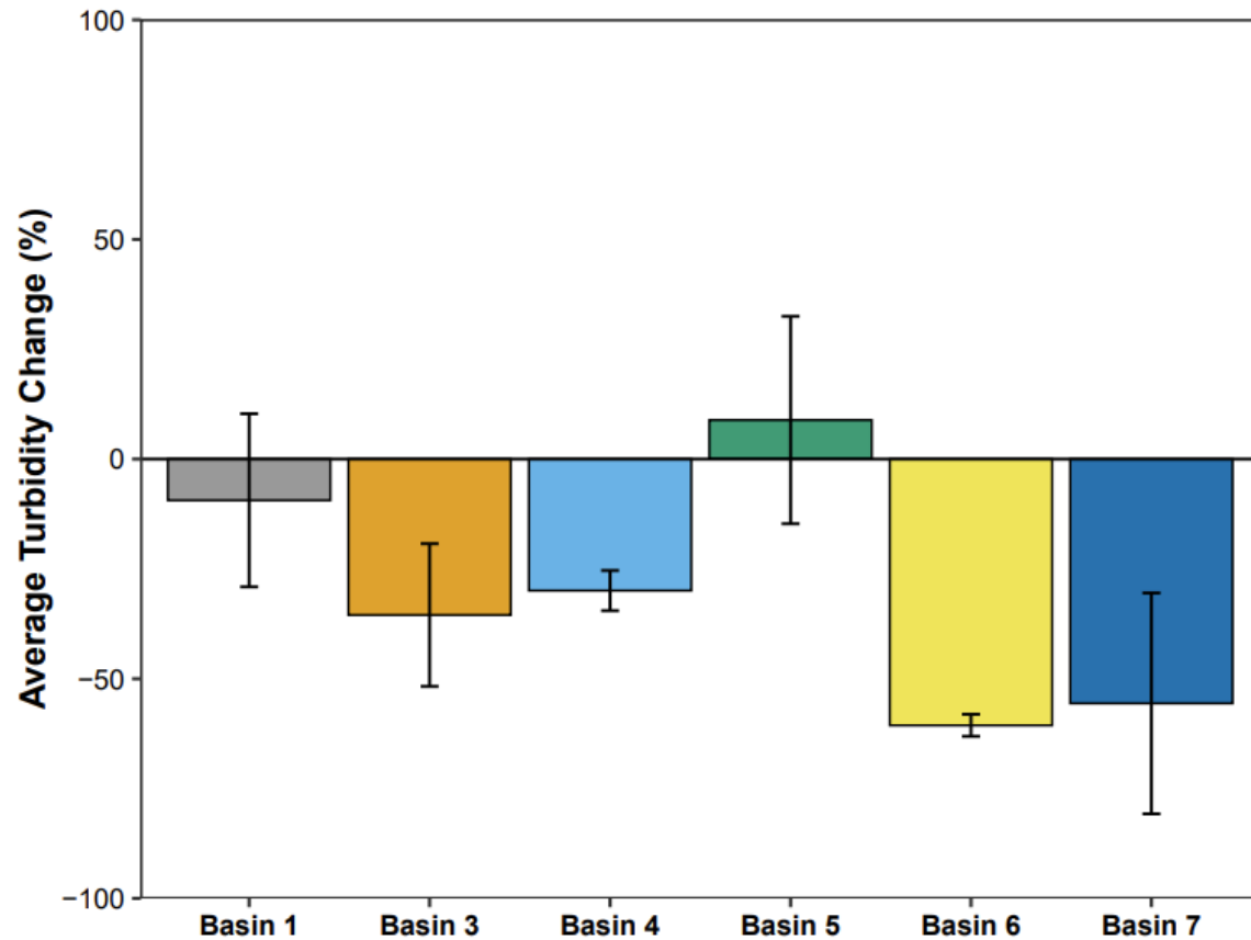
Figure 15. Average change in turbidity for the sediment basins. Negative change means the first baffle sample had higher turbidity than the skimmer sample. Error bars \pm 1 SE. n=number of storms from Table 1.
