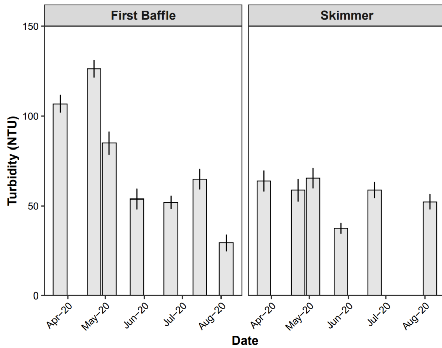
Figure A1. Average turbidity for basin 1 per storm event.
