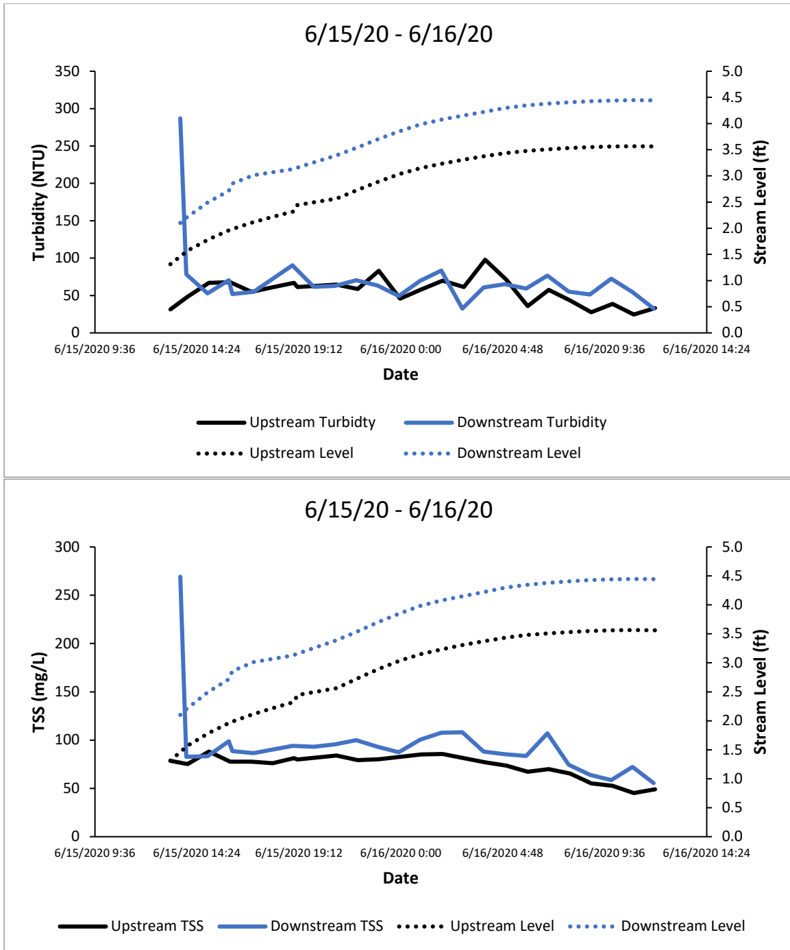
Figure A33. Turbidity (top) and TSS (bottom) in Swift Creek.
