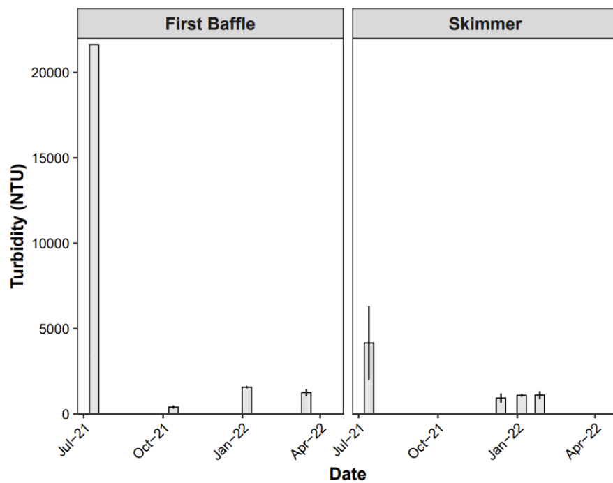
Figure A13. Average turbidity for basin 7 per storm event.
