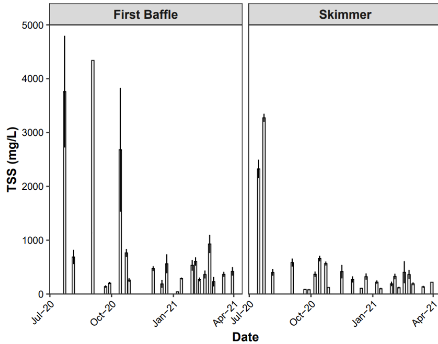
Figure A6. Average TSS for basin 3 per storm event.
