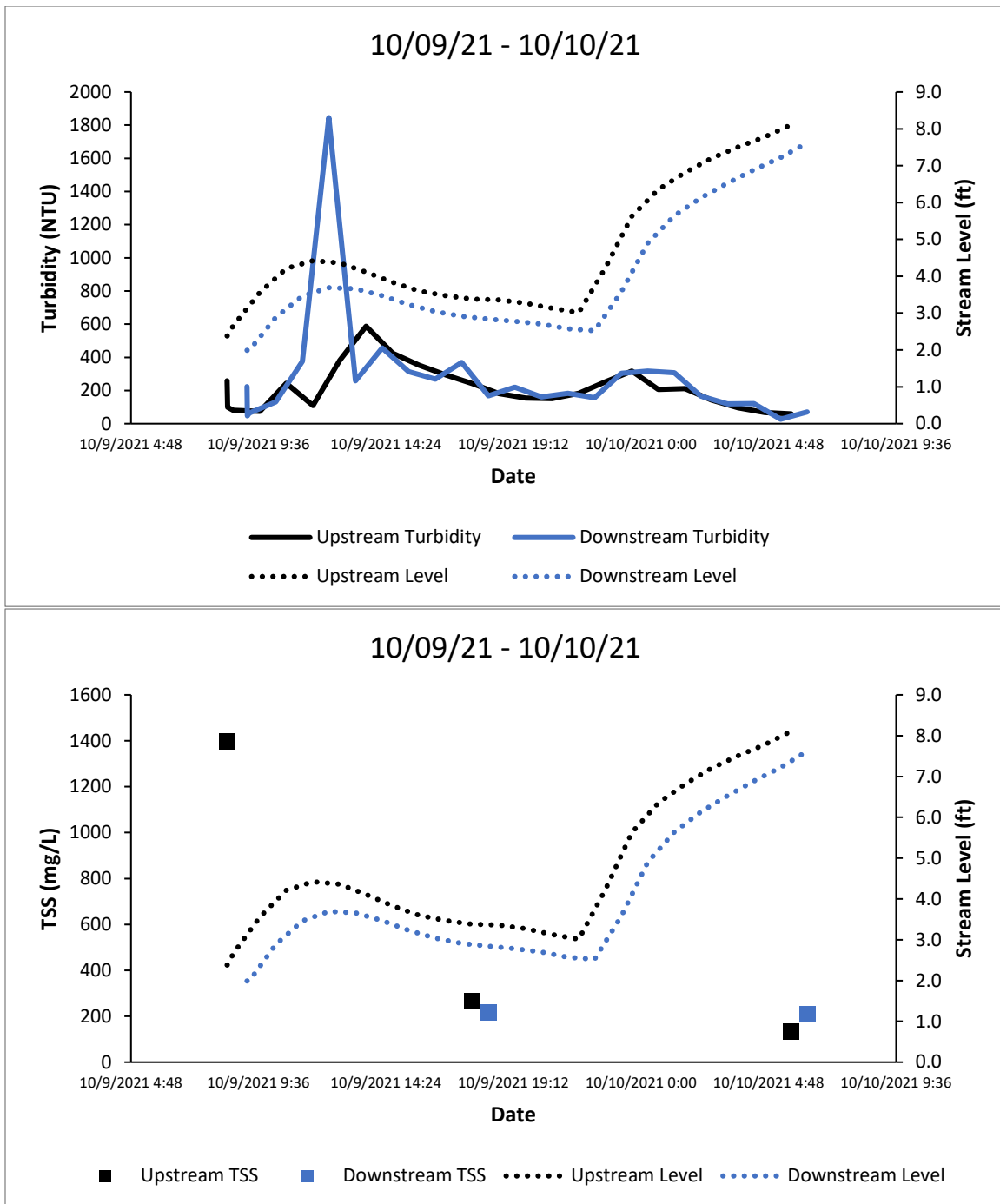
Figure A51. Turbidity (top) and TSS (bottom) in Swift Creek.
