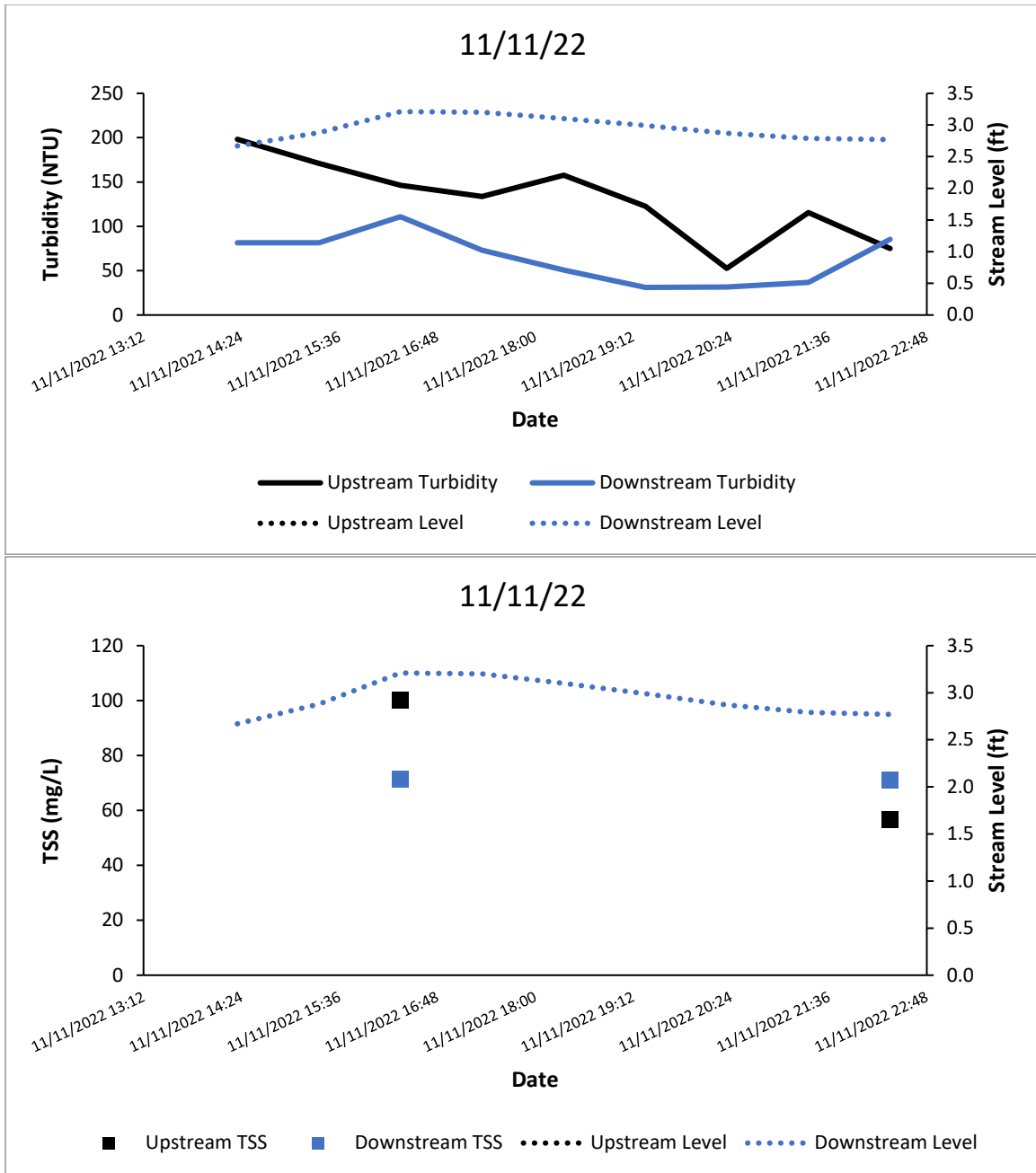
Figure A69. Turbidity (top) and TSS (bottom) in Swift Creek.
