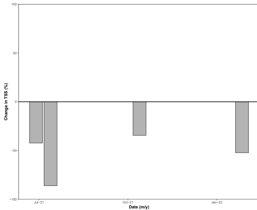
Figure A22. Average TSS change for basin 5 per storm event.
