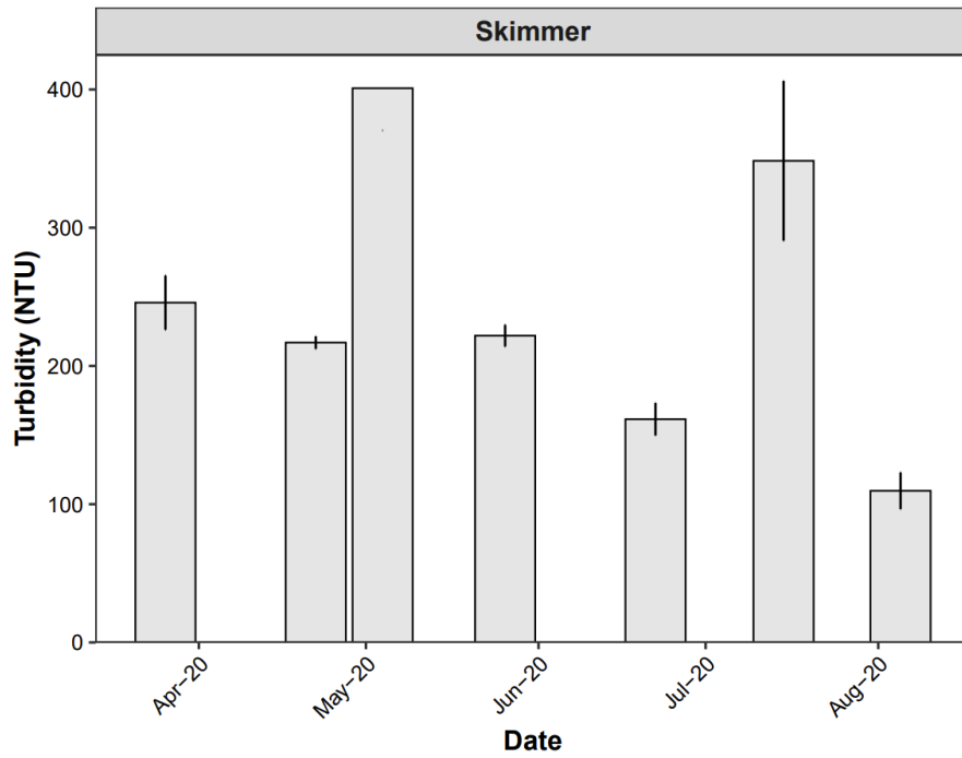
Figure A3. Average turbidity for basin 2 per storm event.
