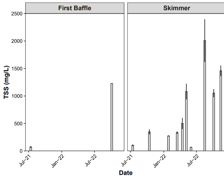
Figure A12. Average TSS for basin 6 per storm event.
