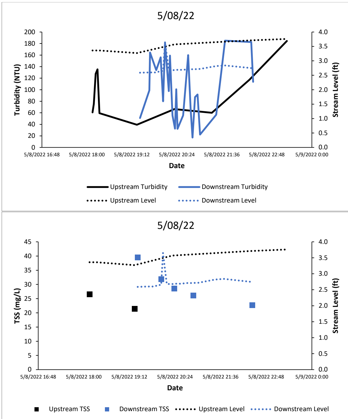
Figure A60. Turbidity (top) and TSS (bottom) in Swift Creek.
