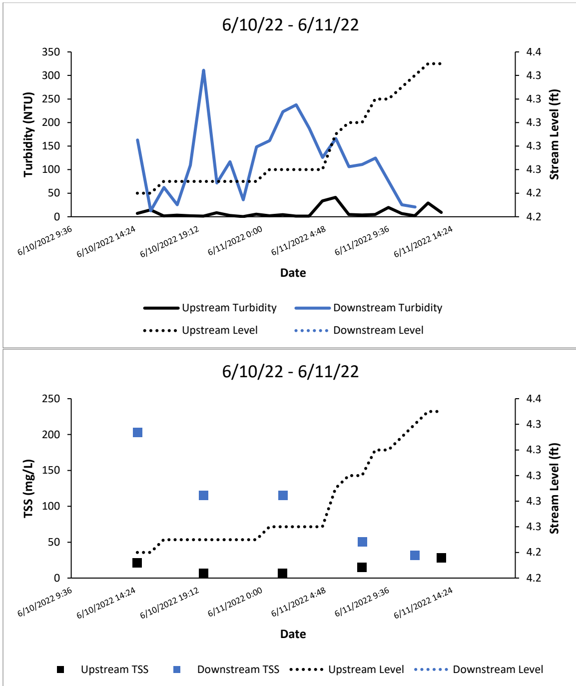
Figure A63. Turbidity (top) and TSS (bottom) in Swift Creek.
