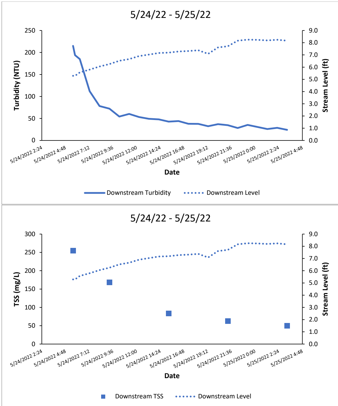
Figure A62. Turbidity (top) and TSS (bottom) in Swift Creek.
