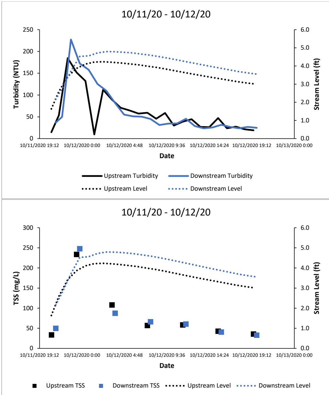
Figure A39. Turbidity (top) and TSS (bottom) in Swift Creek.
