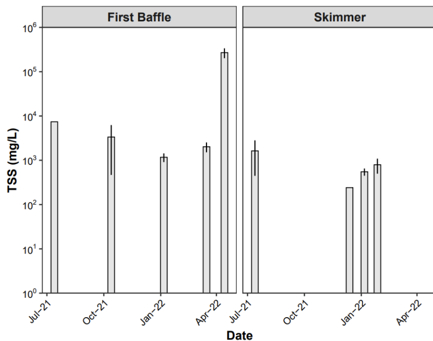
Figure A14. Average TSS for basin 7 per storm event.
