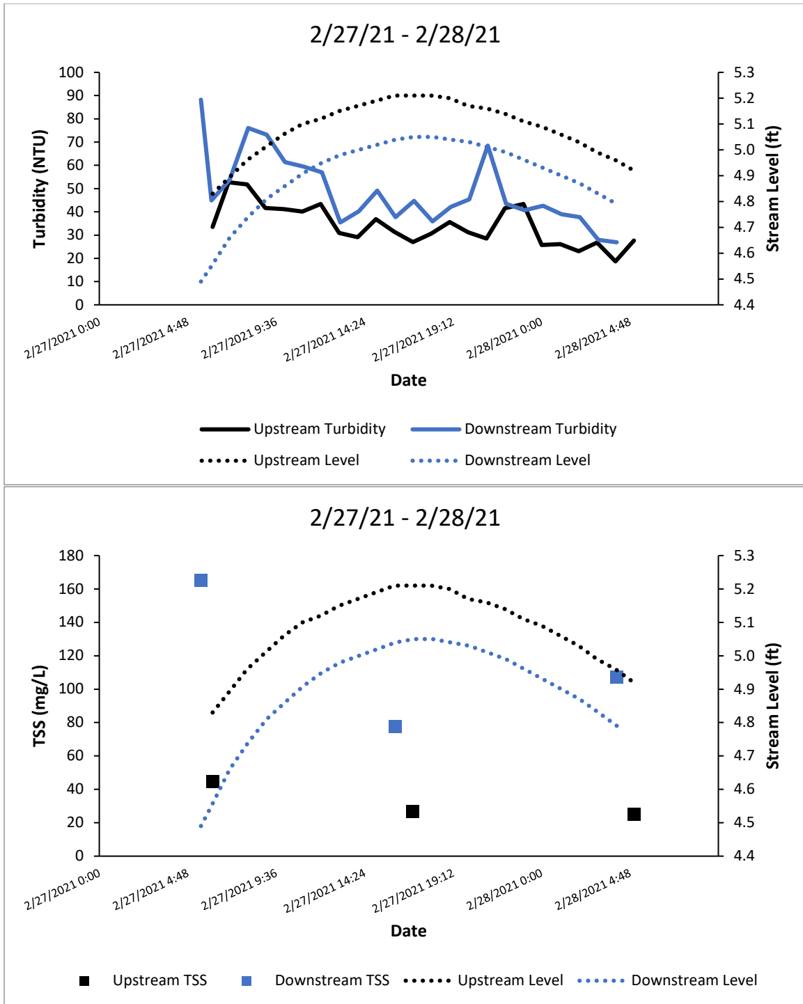
Figure A45. Turbidity (top) and TSS (bottom) in Swift Creek.
