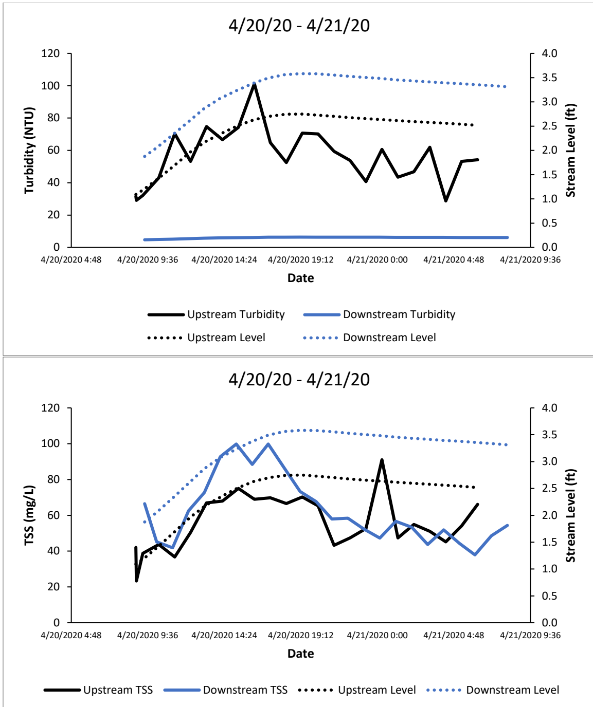
Figure A31. Turbidity (top) and TSS (bottom) in Swift Creek.
