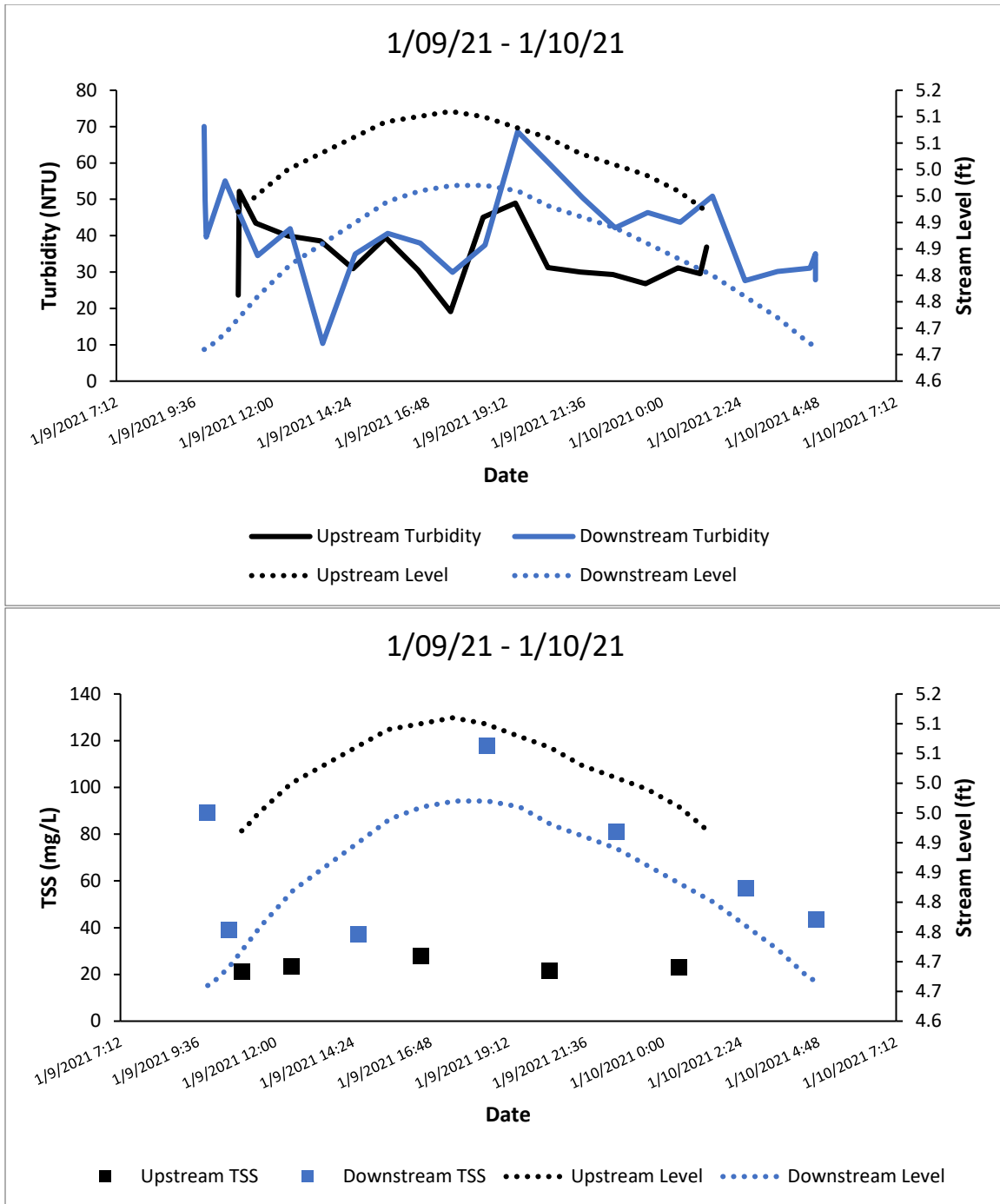
Figure A43. Turbidity (top) and TSS (bottom) in Swift Creek.
