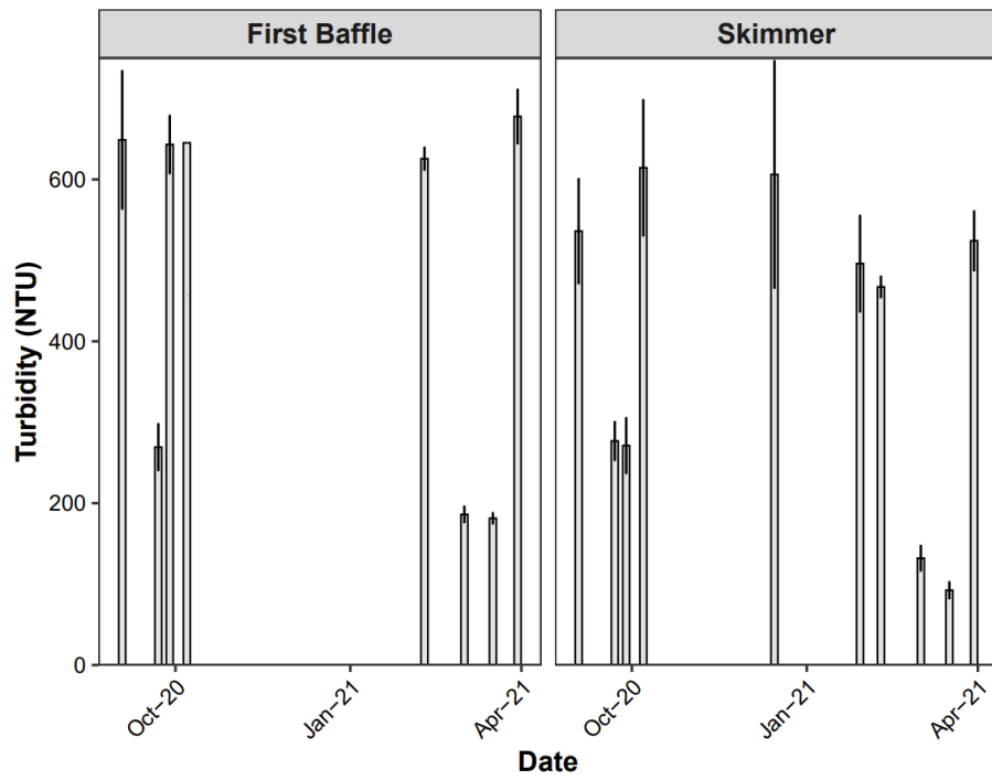
Figure A7. Average turbidity for basin 4 per storm event.
