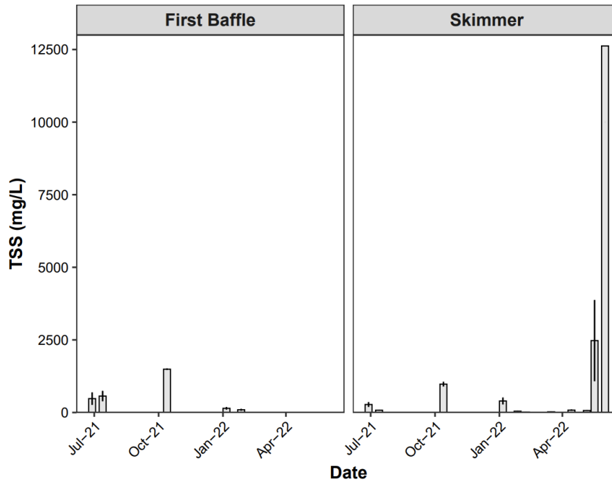
Figure A10. Average TSS for basin 5 per storm event.
