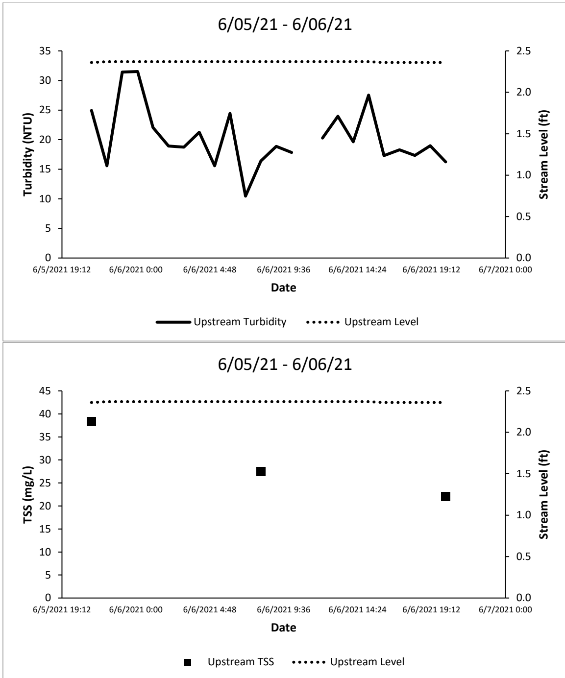
Figure A47. Turbidity (top) and TSS (bottom) in Swift Creek.
