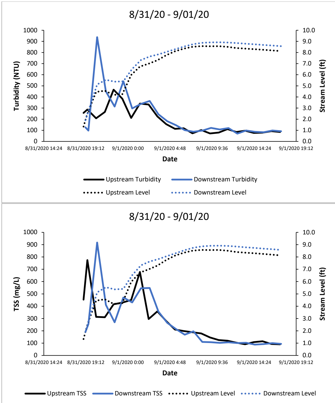
Figure A37. Turbidity (top) and TSS (bottom) in Swift Creek.
