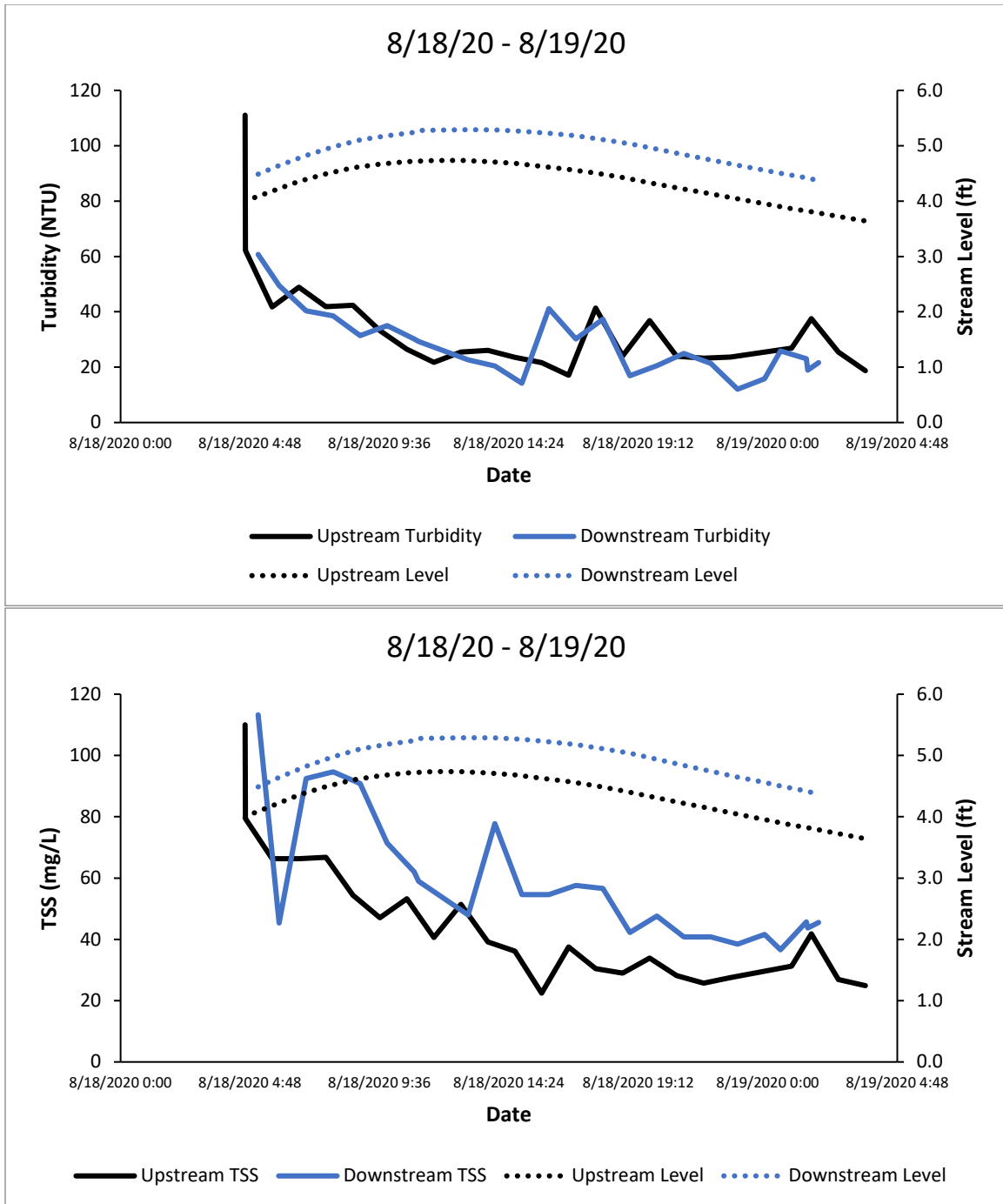
Figure A36. Turbidity (top) and TSS (bottom) in Swift Creek.
