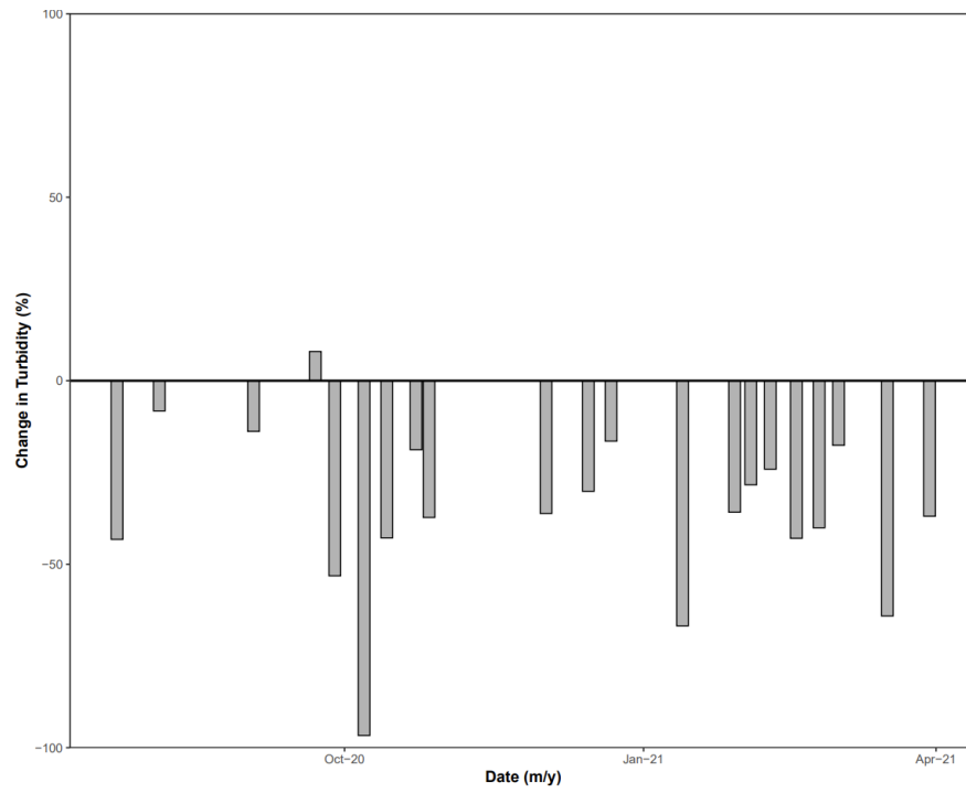
Figure A17. Average turbidity change for basin 3 per storm event.
