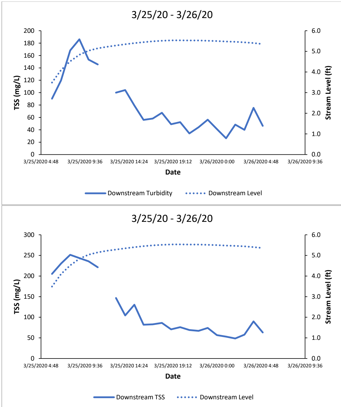
Figure A30. Turbidity (top) and TSS (bottom) in Swift Creek.
