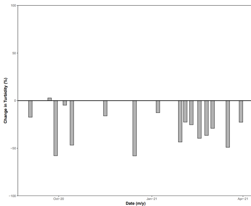
Figure A19. Average turbidity change for basin 4 per storm event.
