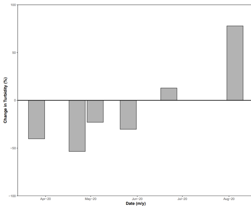
Figure A15. Average turbidity change for basin 1 per storm event.
