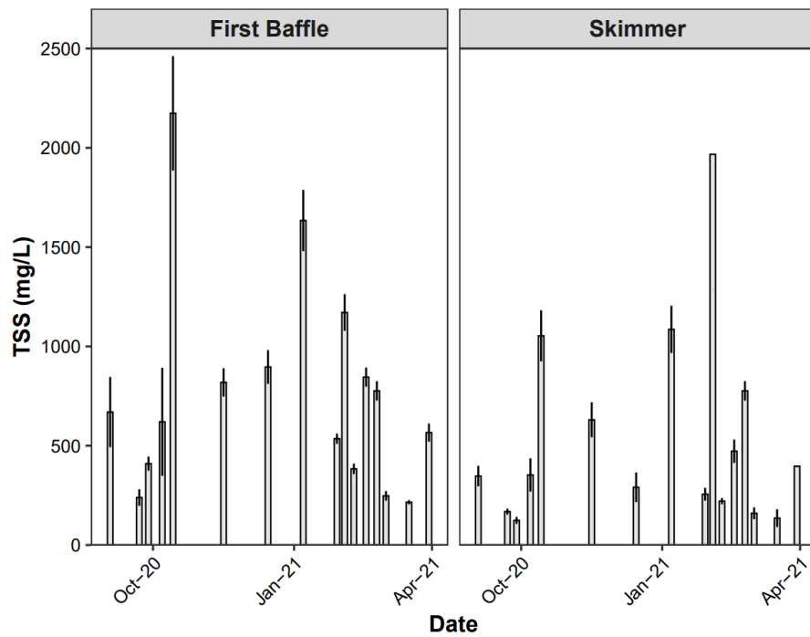
Figure A8. Average TSS for basin 4 per storm event.
