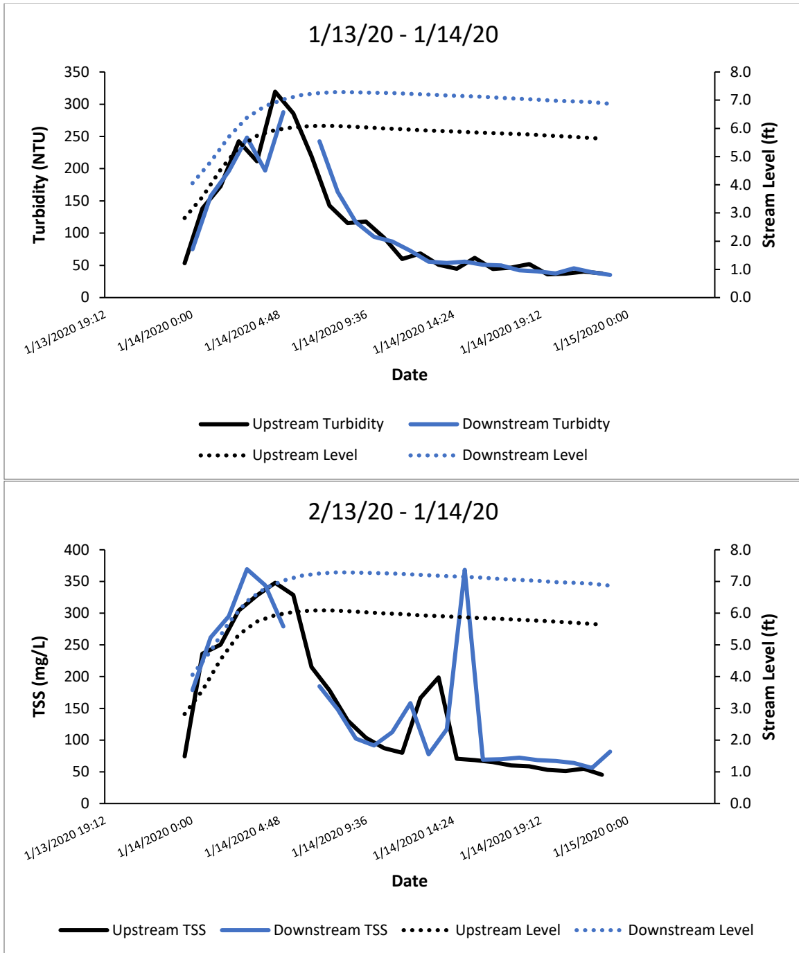
Figure A29. Turbidity (top) and TSS (bottom) in Swift Creek.
