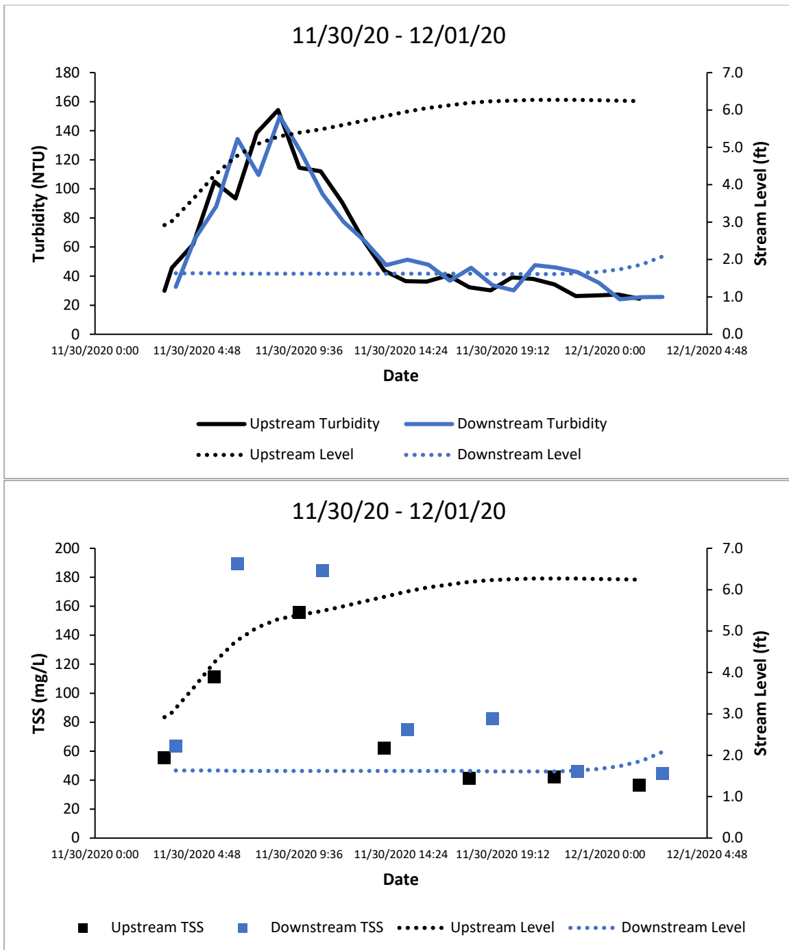
Figure A41. Turbidity (top) and TSS (bottom) in Swift Creek.
