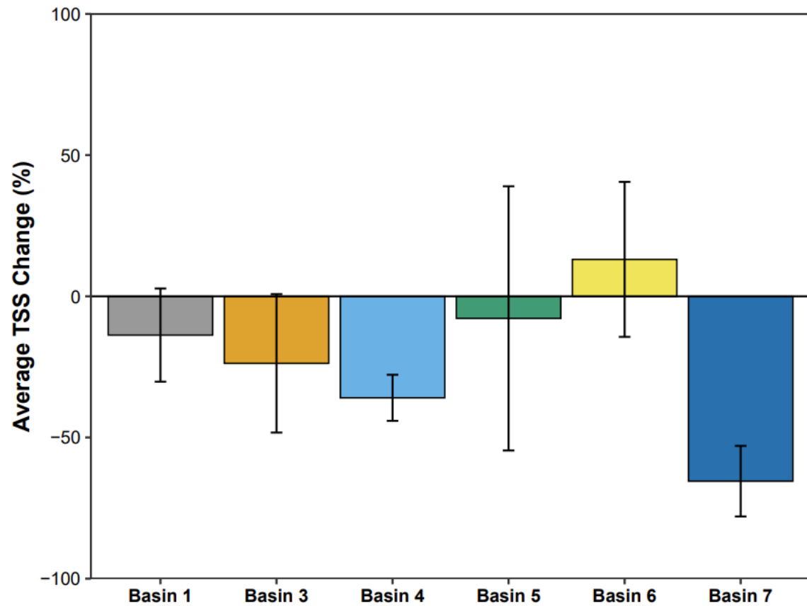
Figure 16. Average change in total suspended solids (TSS) for the sediment basins. Negative change means the first baffle sample was higher than the skimmer sample. Error bars \pm 1 SE. n=number of storms from Table 1.
