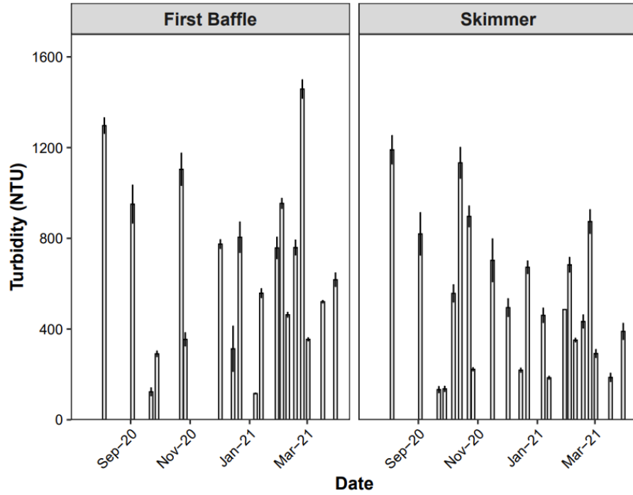
Figure A5. Average turbidity for basin 3 per storm event.
