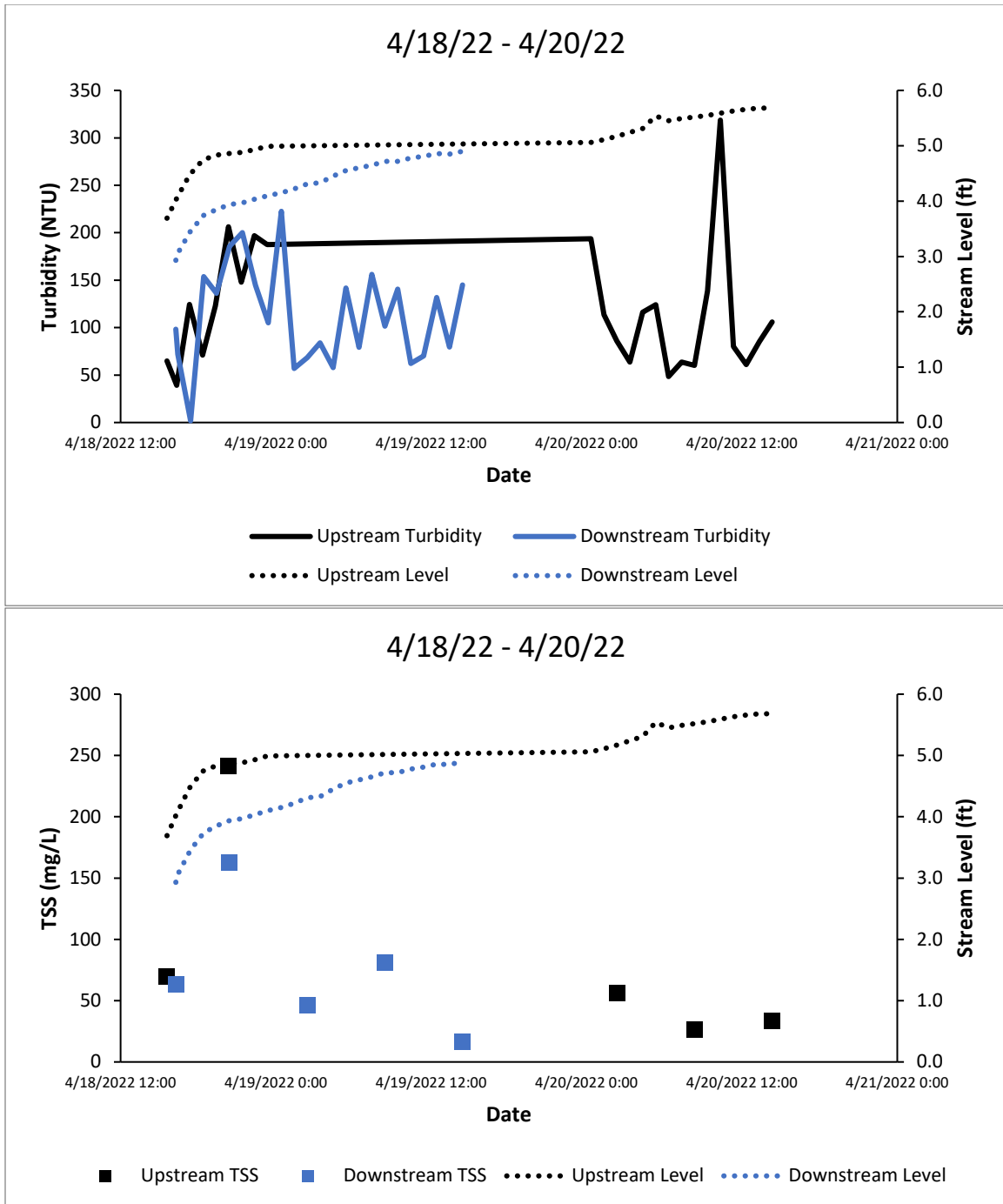
Figure A59. Turbidity (top) and TSS (bottom) in Swift Creek.
