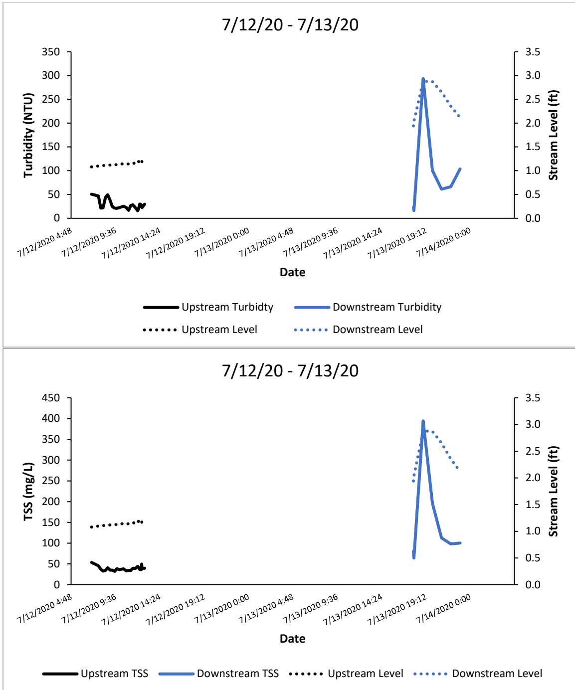
Figure A34. Turbidity (top) and TSS (bottom) in Swift Creek.
