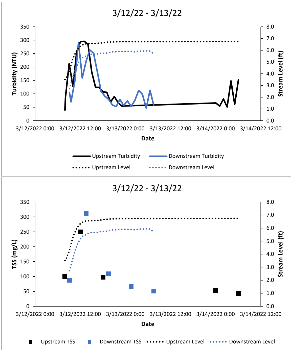
Figure A57. Turbidity (top) and TSS (bottom) in Swift Creek.
