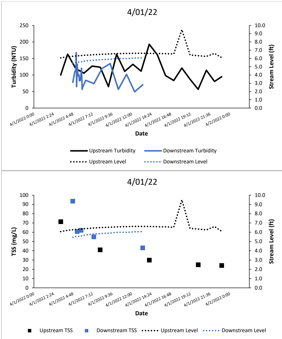
Figure A58. Turbidity (top) and TSS (bottom) in Swift Creek.
