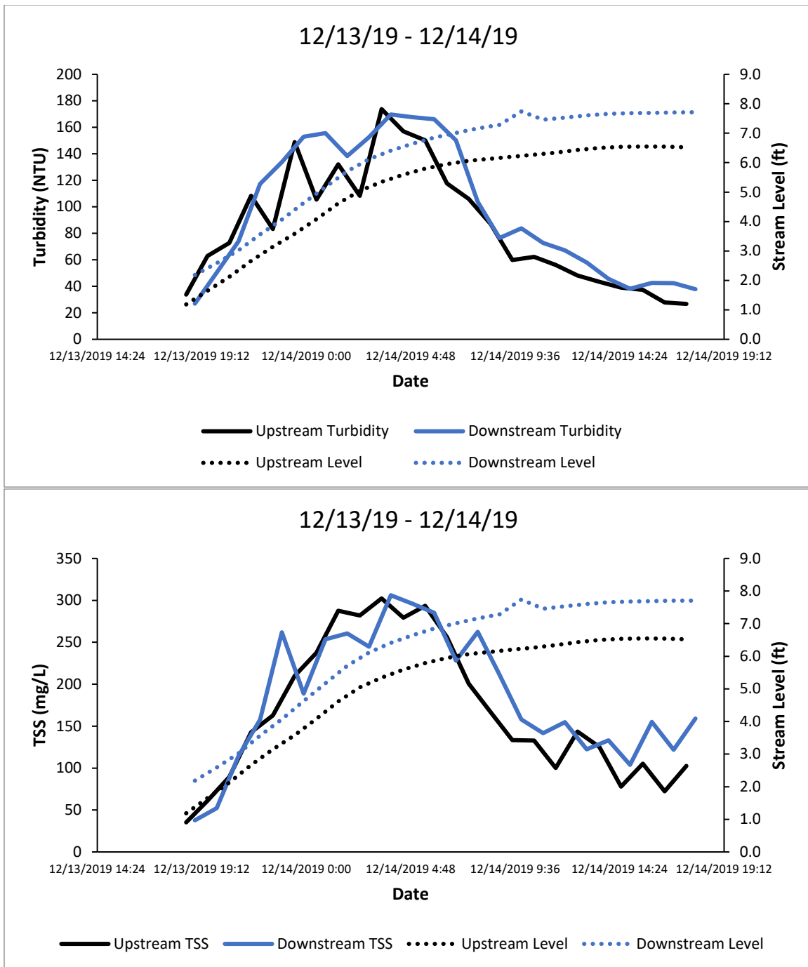
Figure A28. Turbidity (top) and TSS (bottom) in Swift Creek.
