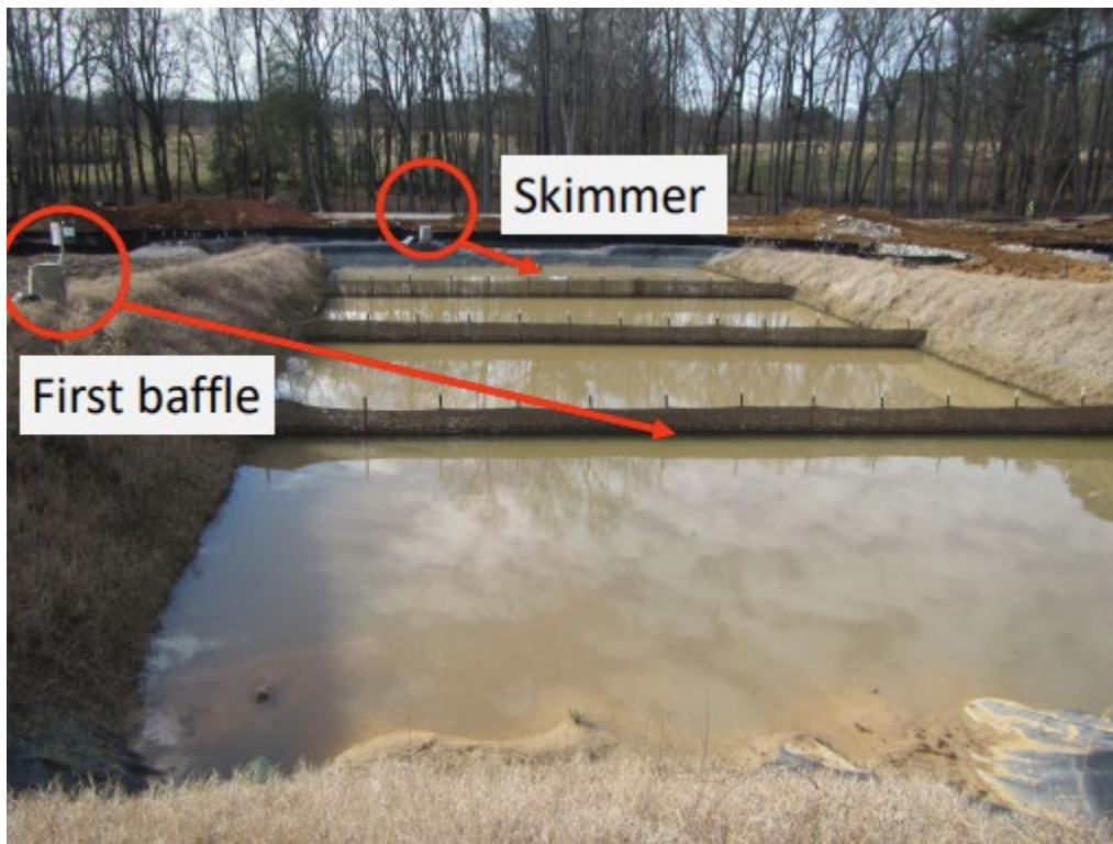
Figure 1. Sediment basin sampler setup.
