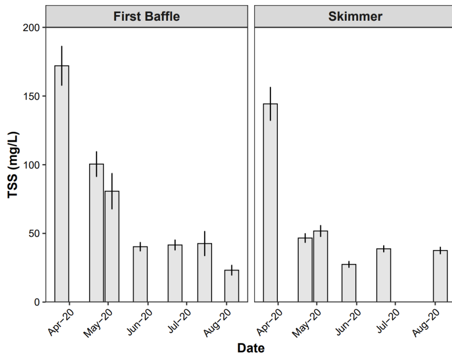
Figure A2. Average TSS for basin 1 per storm event.
