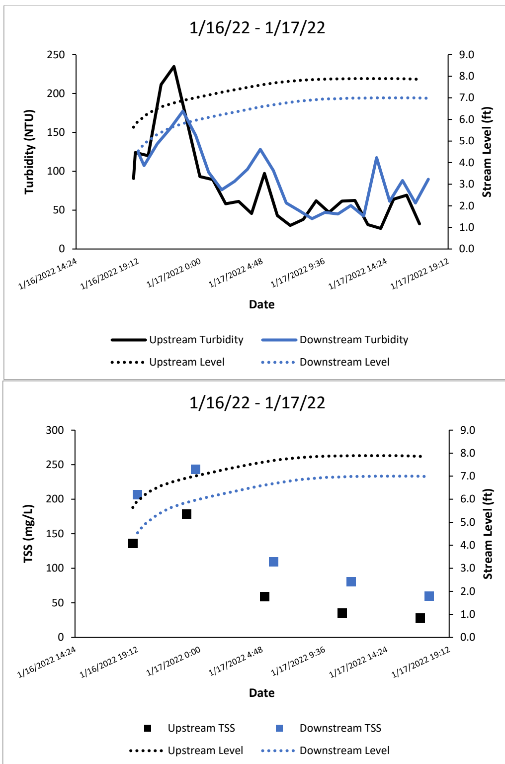
Figure A55. Turbidity (top) and TSS (bottom) in Swift Creek.
