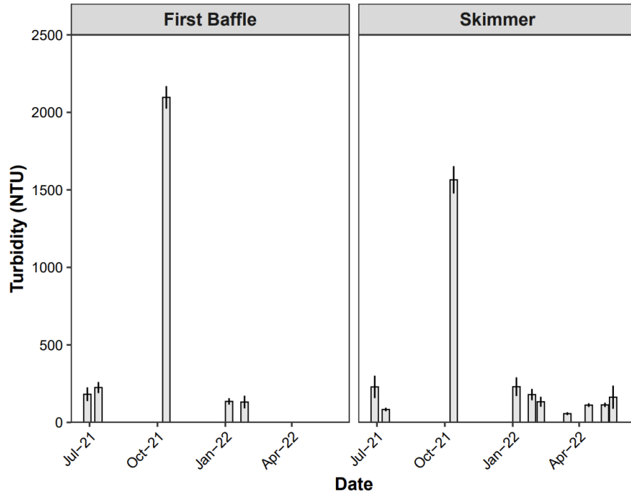
Figure A9. Average turbidity for basin 5 per storm event.
