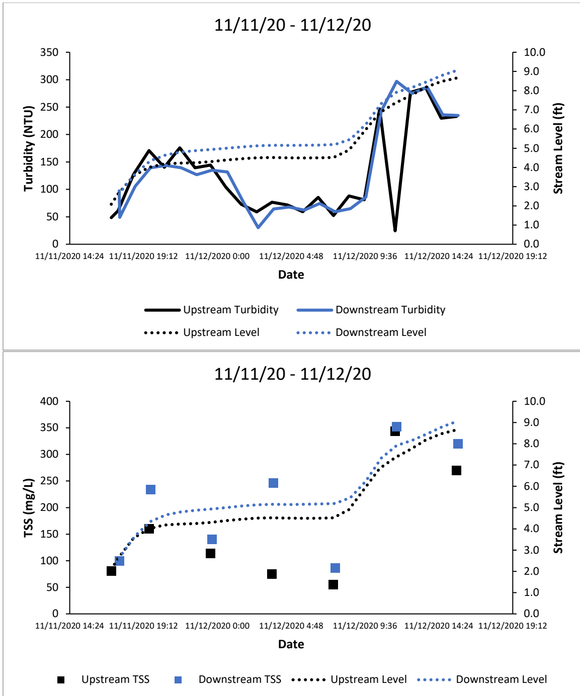
Figure A40. Turbidity (top) and TSS (bottom) in Swift Creek.
