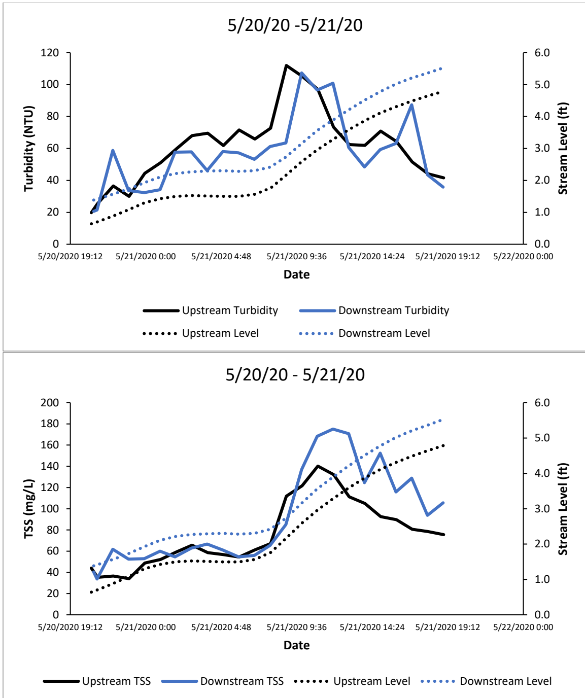
Figure A32. Turbidity (top) and TSS (bottom) in Swift Creek.
