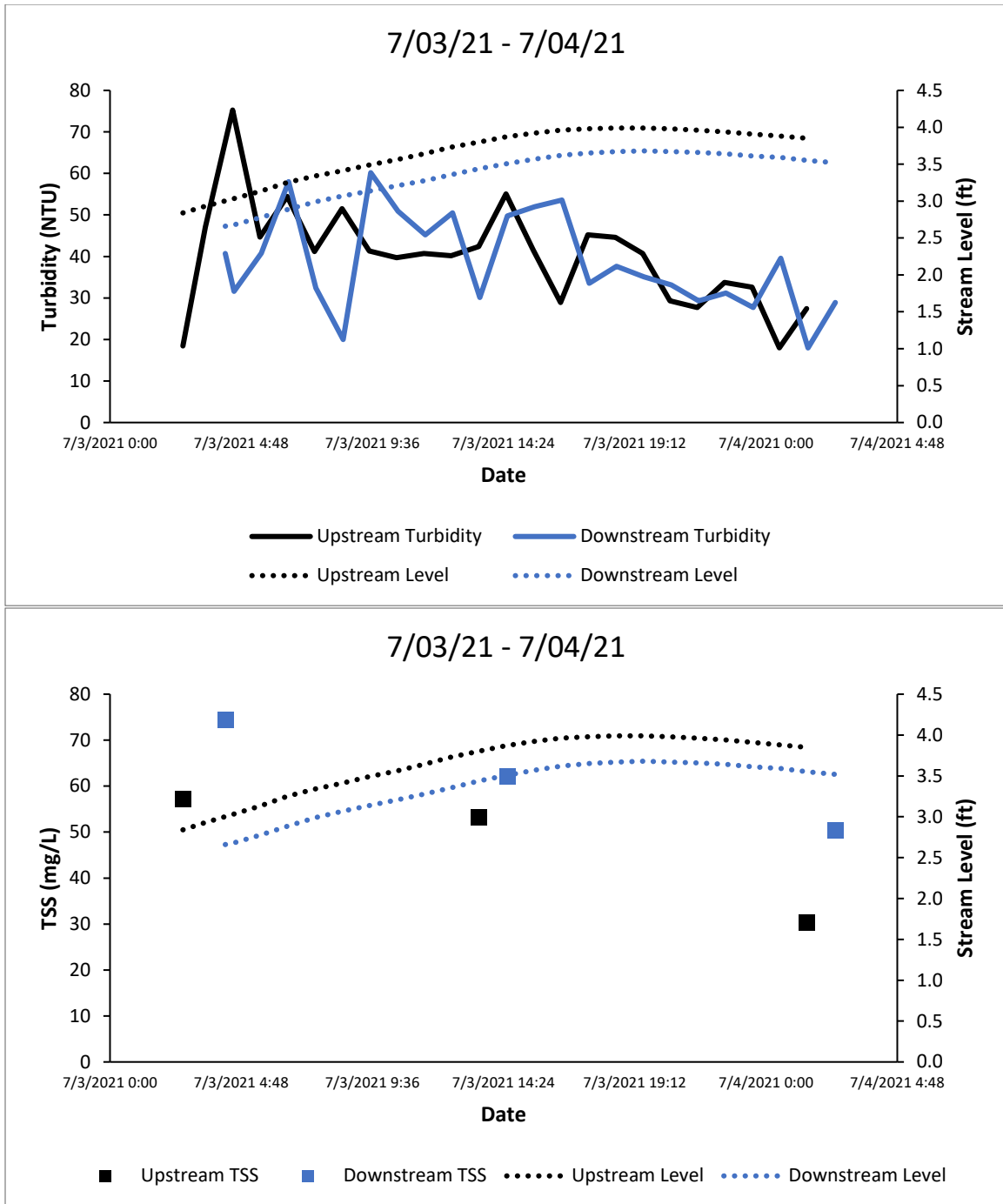
Figure A49. Turbidity (top) and TSS (bottom) in Swift Creek.
