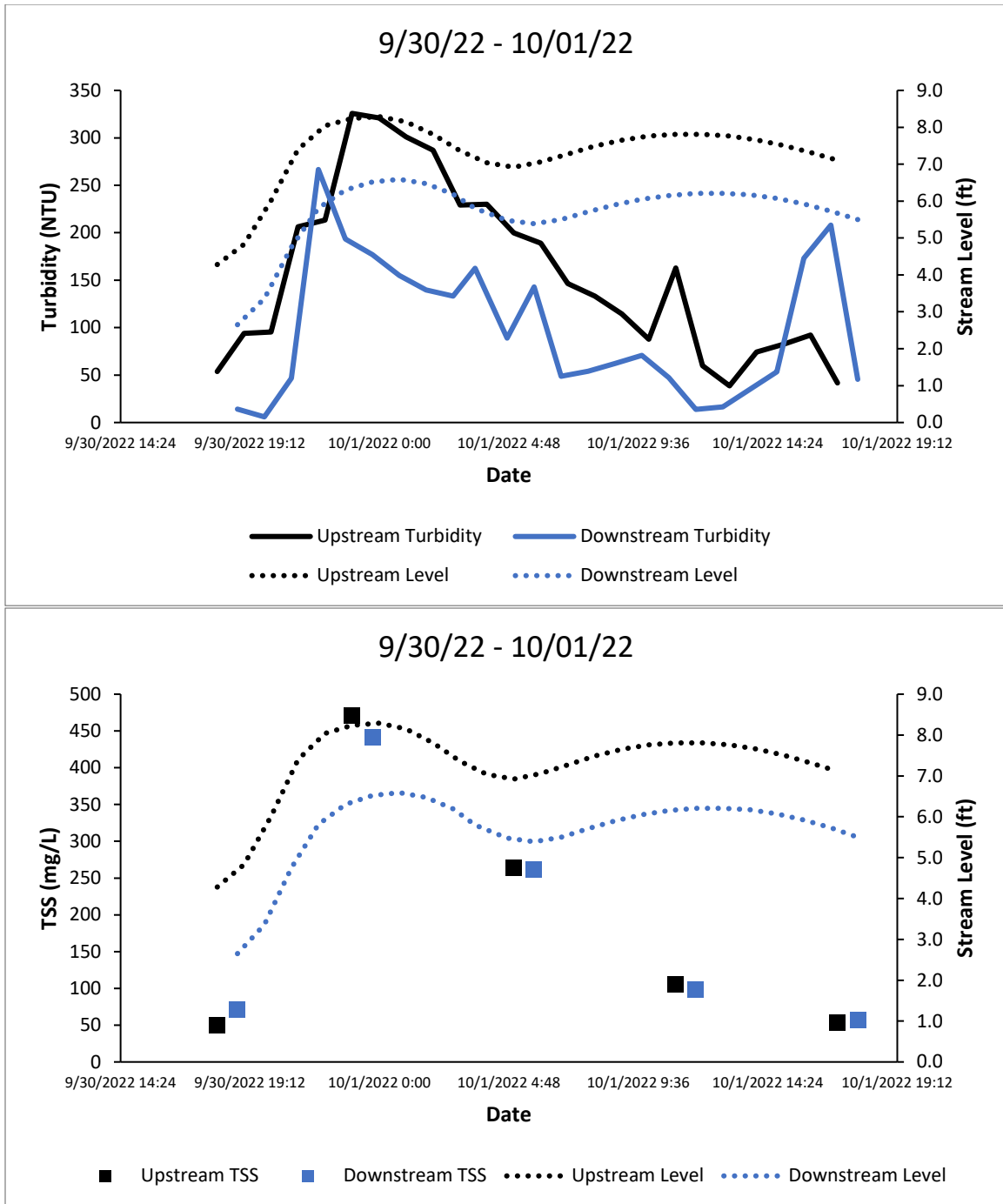
Figure A67. Turbidity (top) and TSS (bottom) in Swift Creek.
