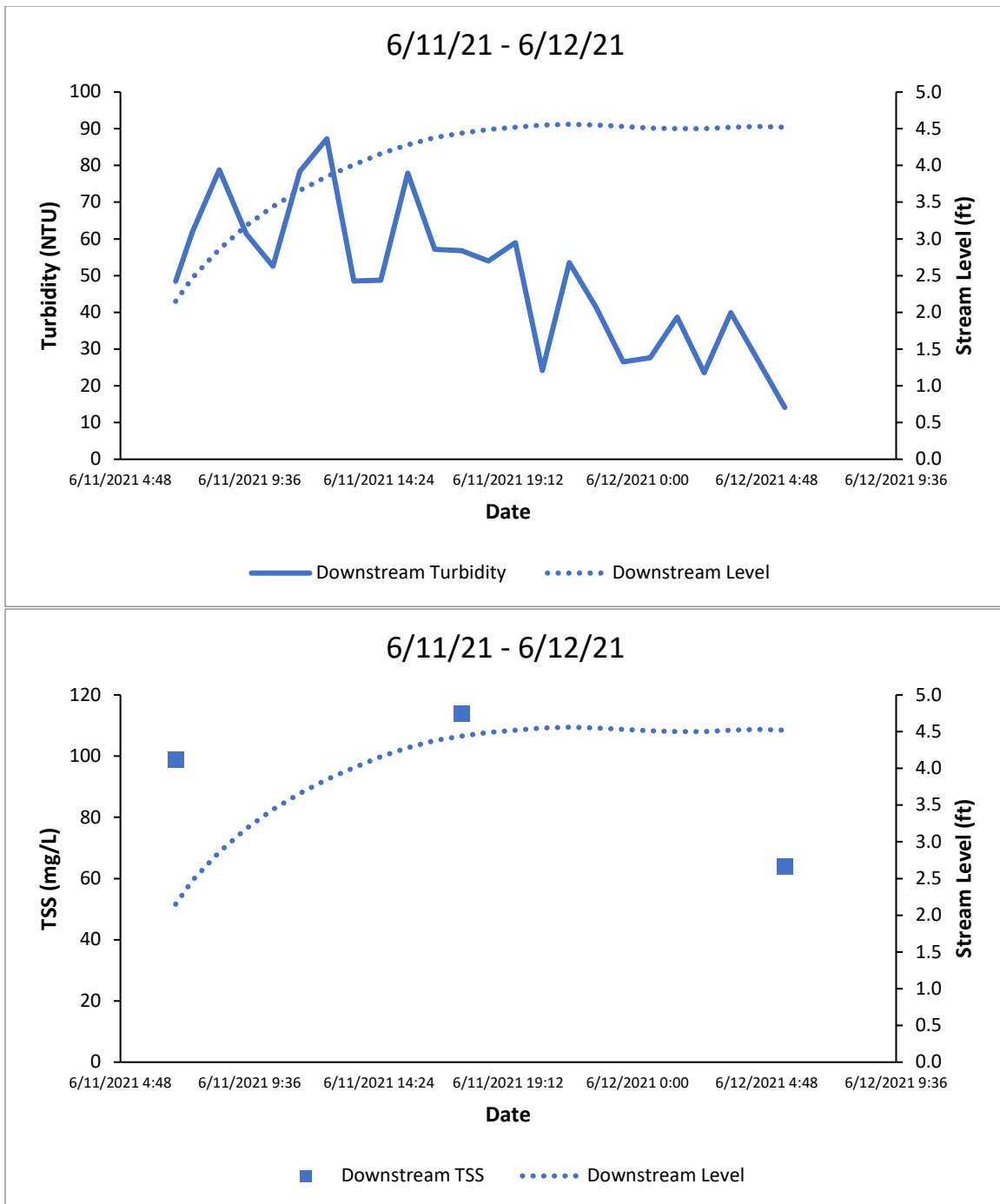
Figure A48. Turbidity (top) and TSS (bottom) in Swift Creek.
