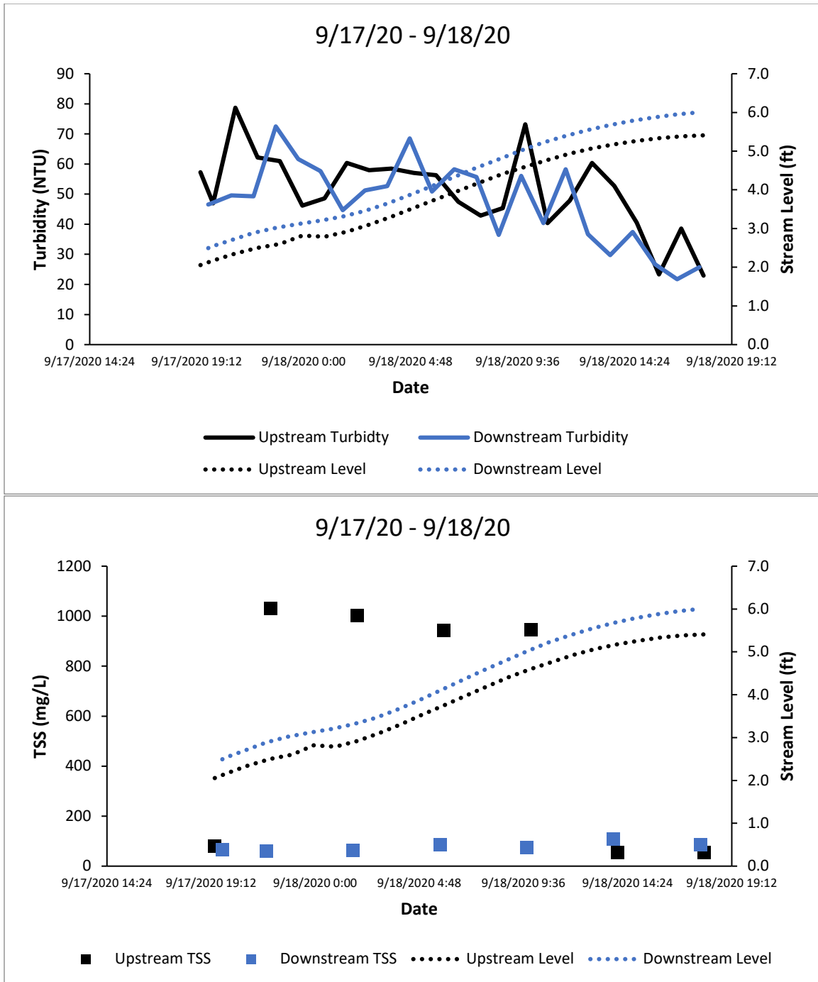
Figure A38. Turbidity (top) and TSS (bottom) in Swift Creek.
