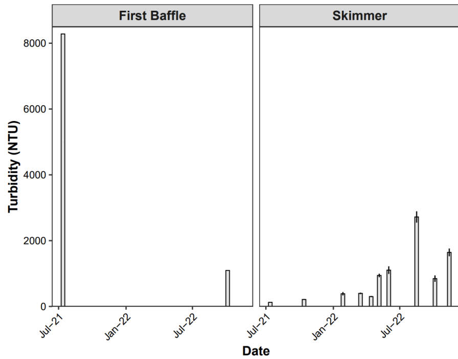
Figure A11. Average turbidity for basin 6 per storm event.
