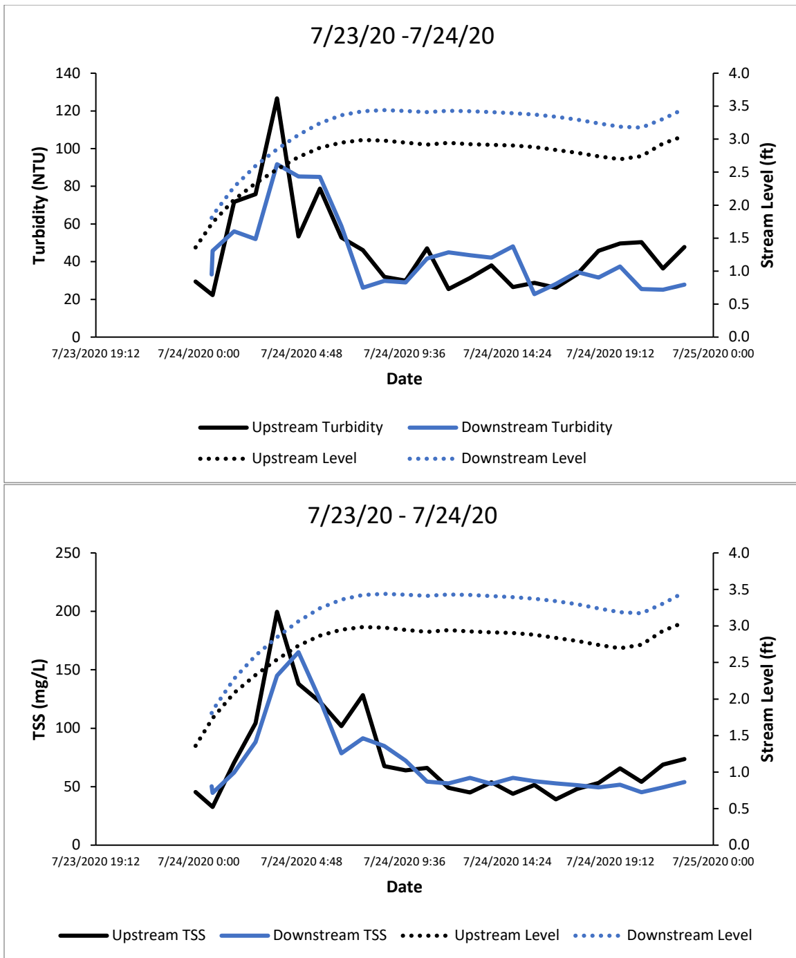
Figure A35. Turbidity (top) and TSS (bottom) in Swift Creek.
