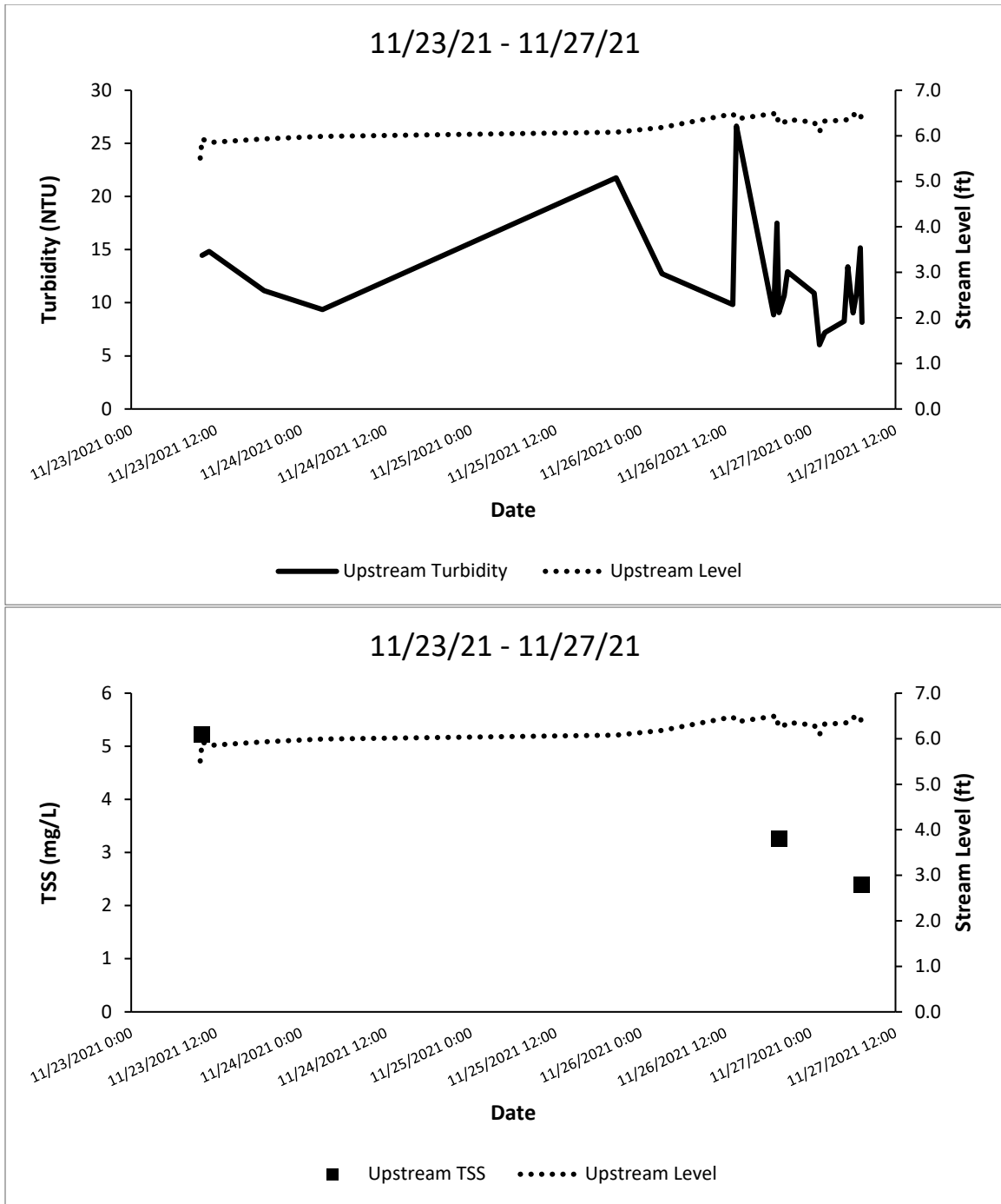
Figure A53. Turbidity (top) and TSS (bottom) in Swift Creek.
