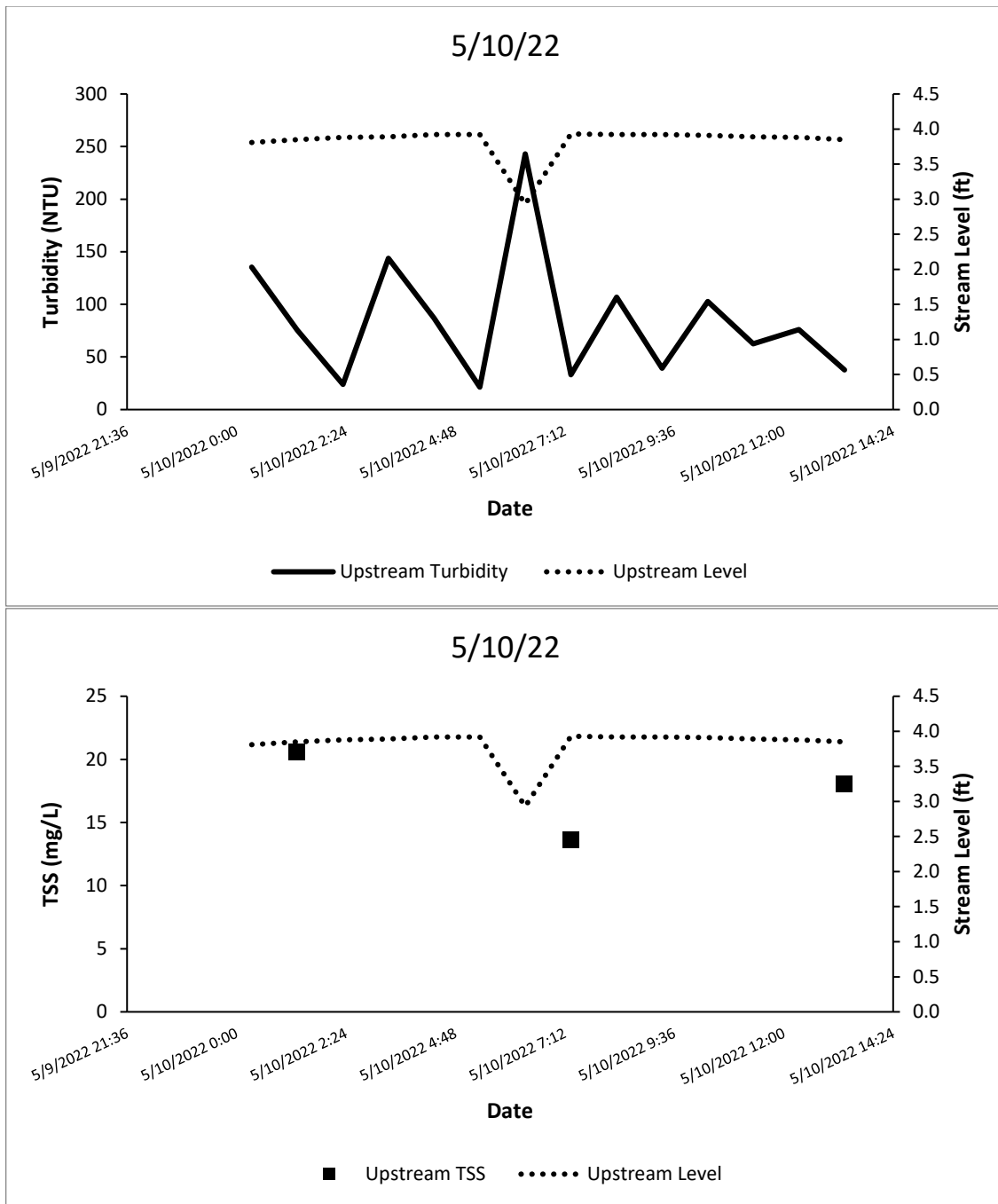
Figure A61. Turbidity (top) and TSS (bottom) in Swift Creek.
