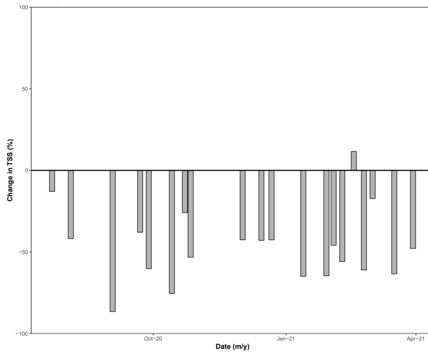
Figure A18. Average TSS change for basin 3 per storm event.
