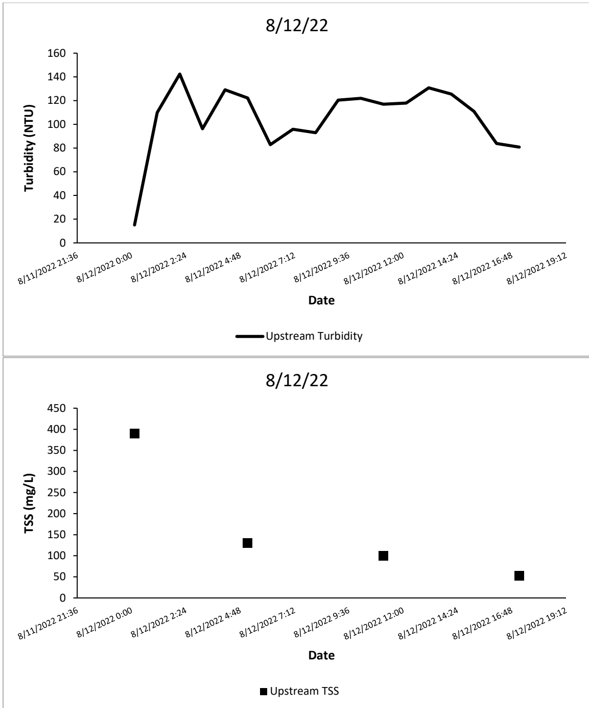
Figure A64. Turbidity (top) and TSS (bottom) in Swift Creek.
