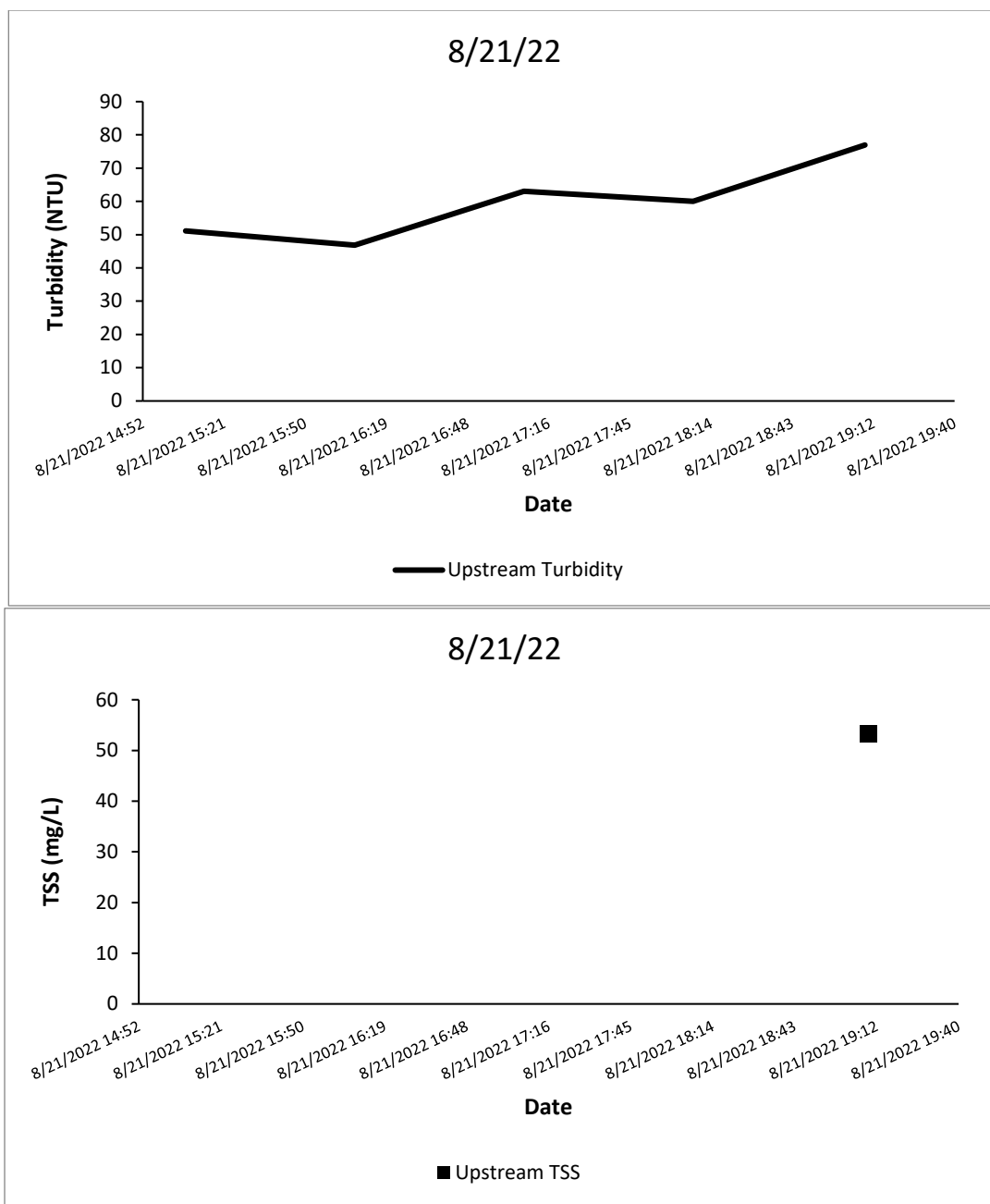
Figure A65. Turbidity (top) and TSS (bottom) in Swift Creek.
