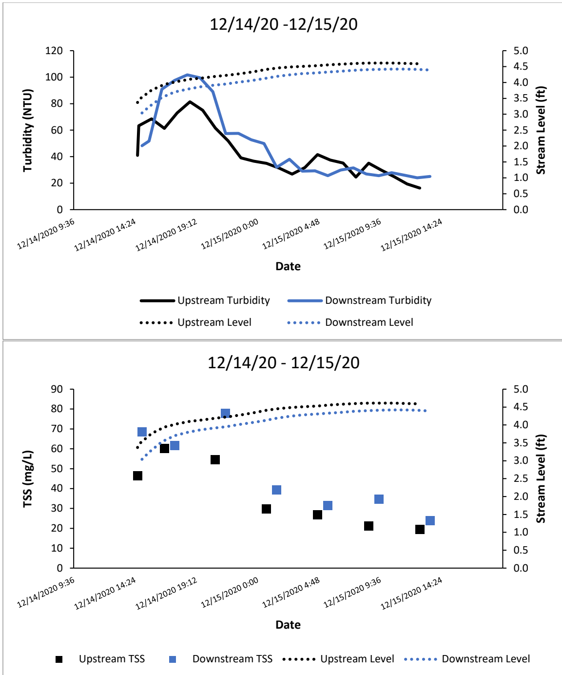
Figure A42. Turbidity (top) and TSS (bottom) in Swift Creek.
