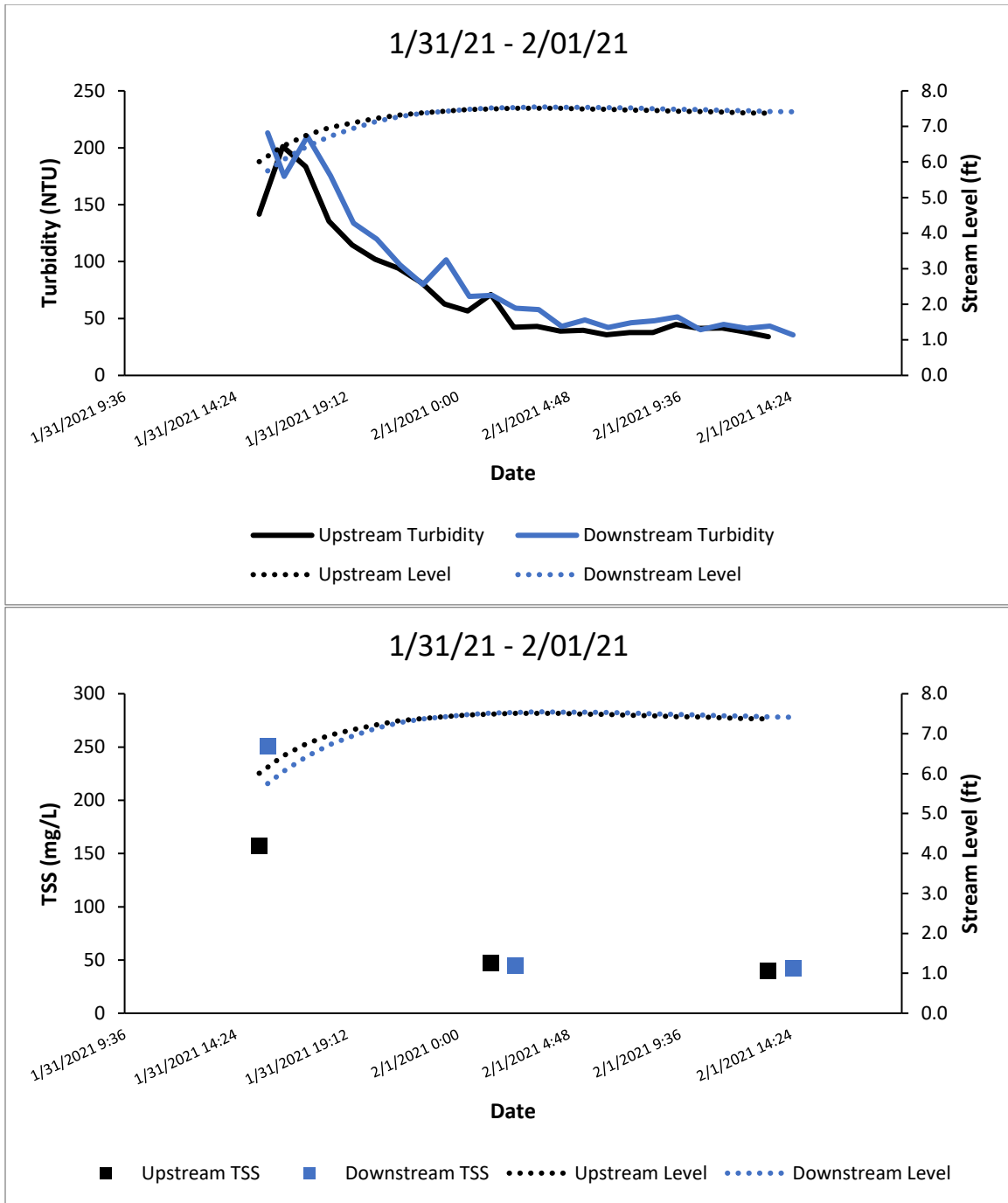
Figure A44. Turbidity (top) and TSS (bottom) in Swift Creek.
