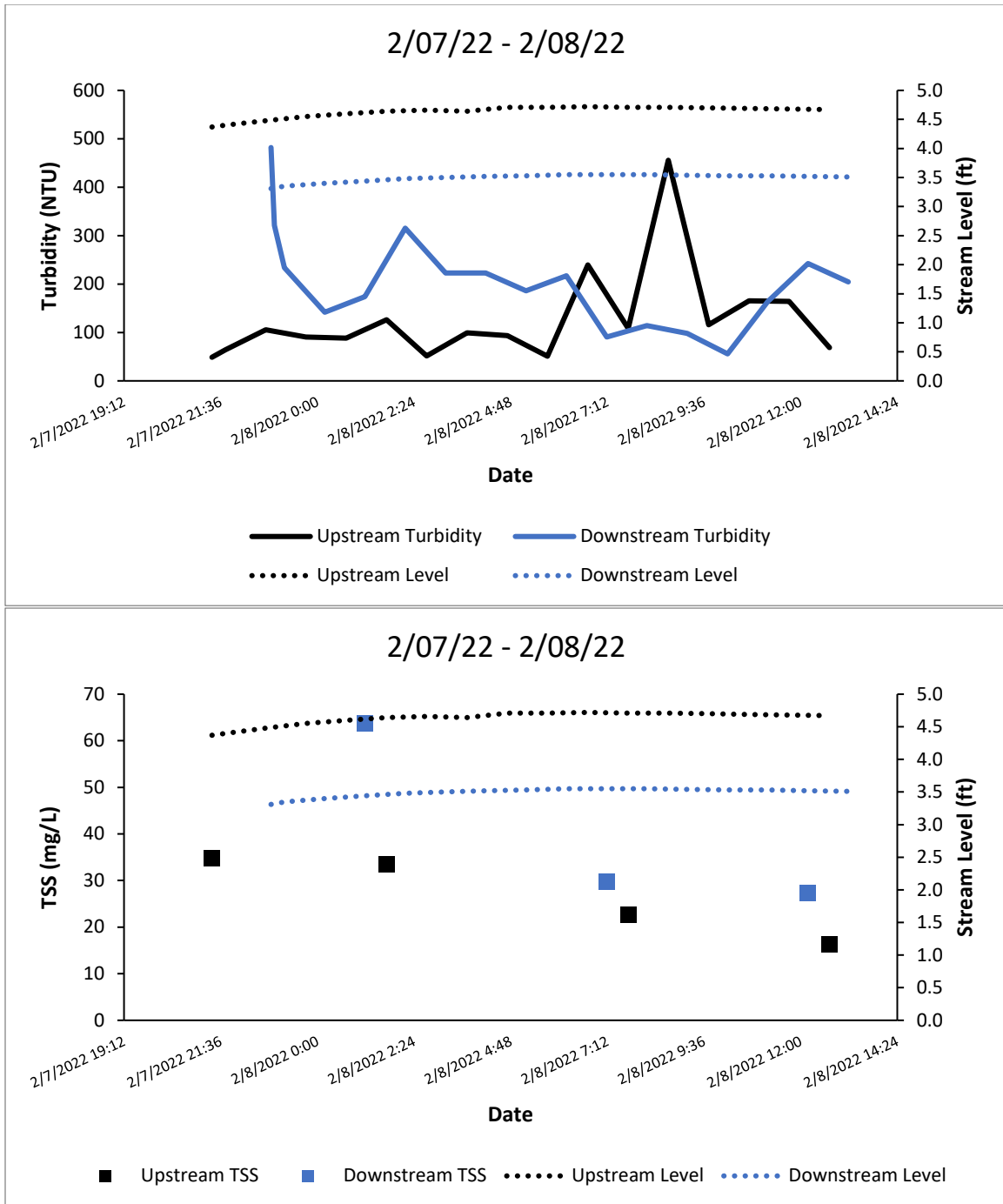
Figure A56. Turbidity (top) and TSS (bottom) in Swift Creek.
