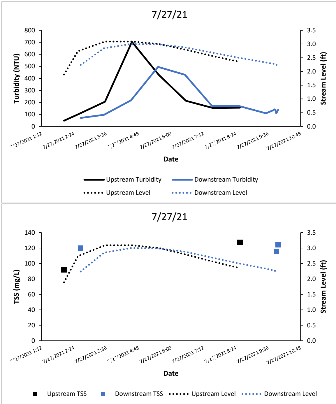
Figure A50. Turbidity (top) and TSS (bottom) in Swift Creek.
