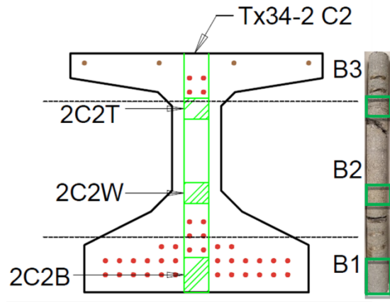
(c) X-ray CT Scan Locations of C2
