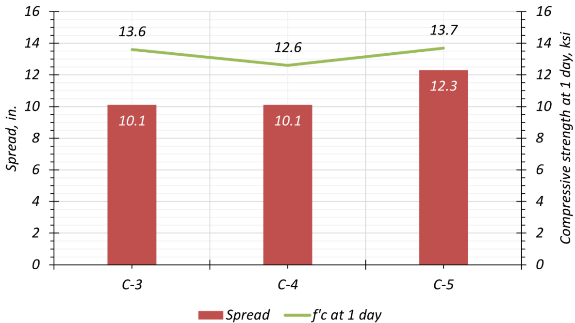
Figure 4.19. Comparison of Flow Spread and 1-Day Compressive Strength for Different Type III Cements and Identical Mixture Proportions.
