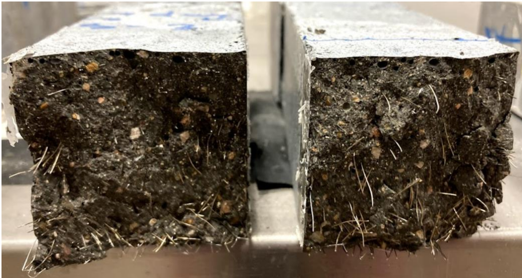
(b) Tx34-2 Tension Specimen—As-Cast Orientation with Improved Fiber Distribution
