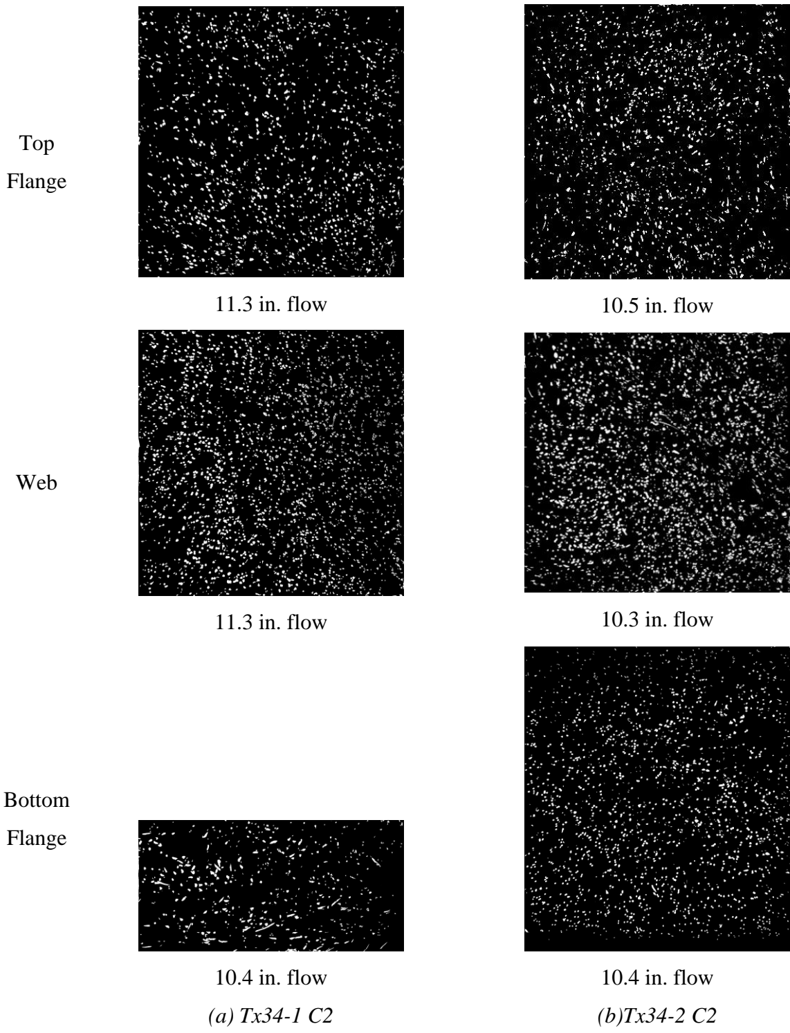
Figure 8.32. Fiber Concentration Comparison between Tx34-1 and Tx34-2.
