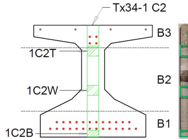
(c) X-ray CT Scan Locations of C2
