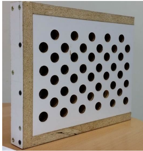
Figure 5. The symmetrical circular pattern for IR camera calibration.
