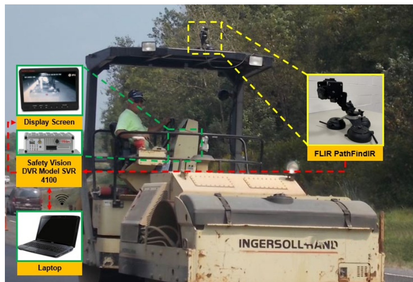
Figure 1. Vision-based roller system.
