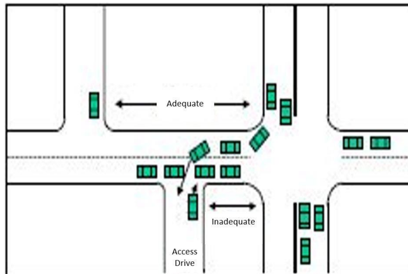
Figure 25: Corner Clearance (83)
