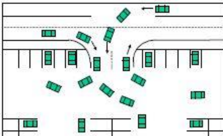
Figure 29: Insufficient Throat Length (90)
