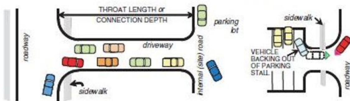
Figure 27: Driveway Throat (73)
