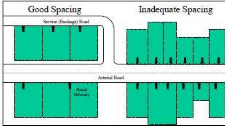
Figure 23: Good and Inadequate Driveway Spacing (74)
