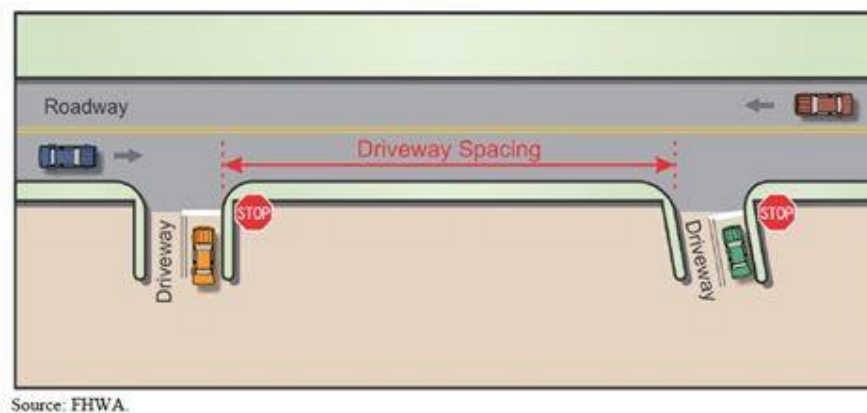
Figure 22: Unsignalized Driveway Spacing (32)
