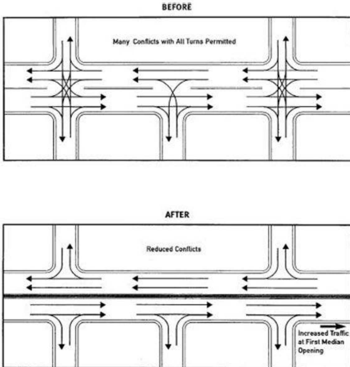
Figure 32: Median Left-Turn Conflict Comparison (32, 33)
