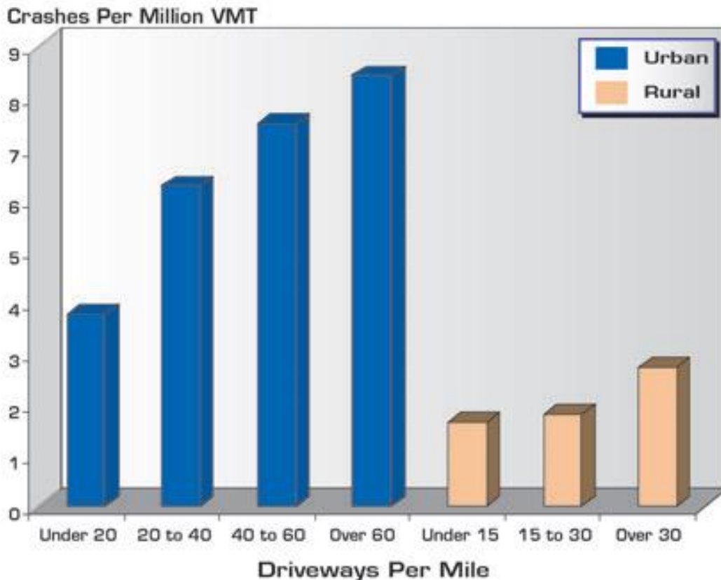
Figure 24: Correlation of Driveway Density with Increased Crash Rate (5)
