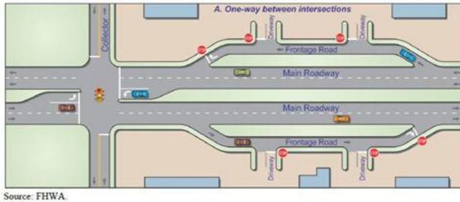
Figure 17: Frontage Road (32)
