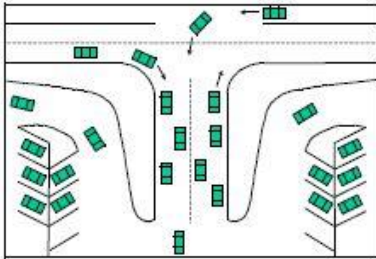
Figure 28: Adequate Throat Length (90)
