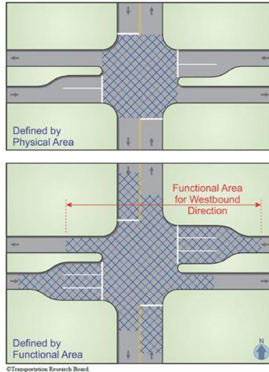
Figure 26: Intersection Functional Area (32)
