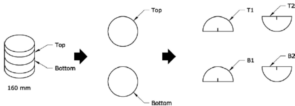
Figure 5.11 IFIT Specimen Preparation (figure taken from Illinois, 2016)
