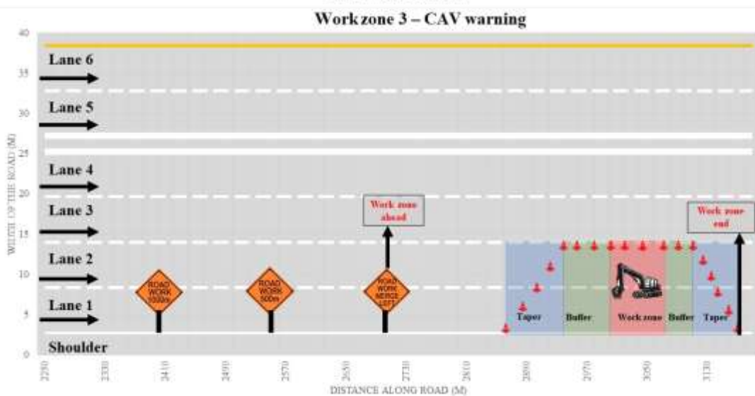
Figure 12: Work zone #3 illustration and critical points under various scenarios
