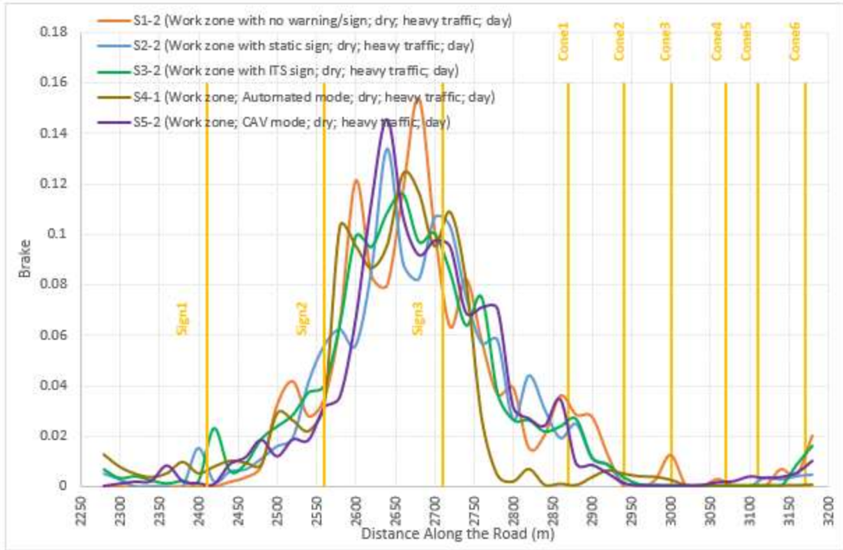
Figure 19: Brake use comparison among various types of warning scenarios in work zone #3 (heavy traffic)
