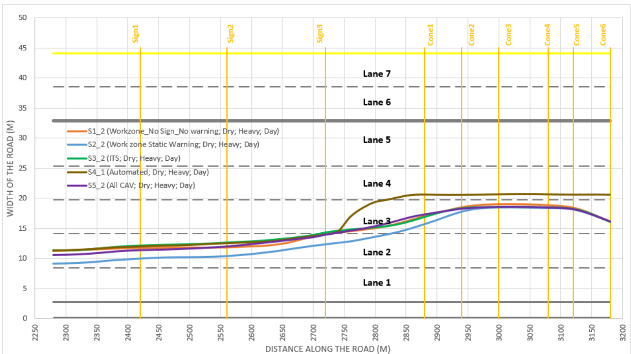
Figure 20: Lateral distance movement comparison among various types of warning scenarios in work zone #3 (heavy traffic)
