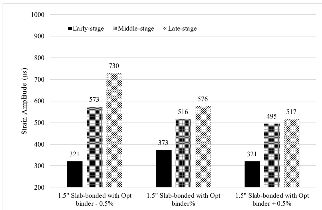
Figure 42. Longitudinal strain amplitude for high and low binder mixes.
