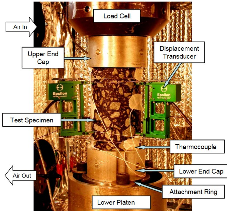
Figure 4. Test specimen with transducers and thermocouples (Soltani & Anderson, 2005).
