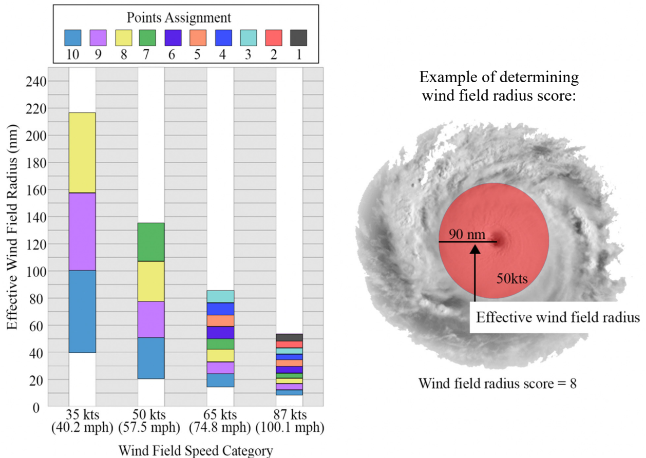
Figure 2. HSI wind field point assignments. Chart obtained from [15].
