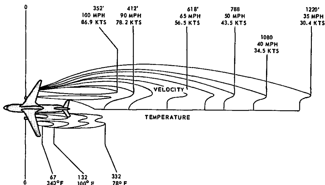
FIGURE 23. Jet Blast - Typical Heavy Jet
