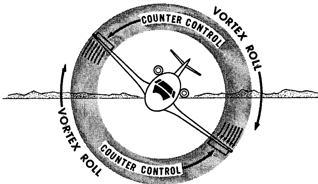
FIGURE 3. Induced Roll.
