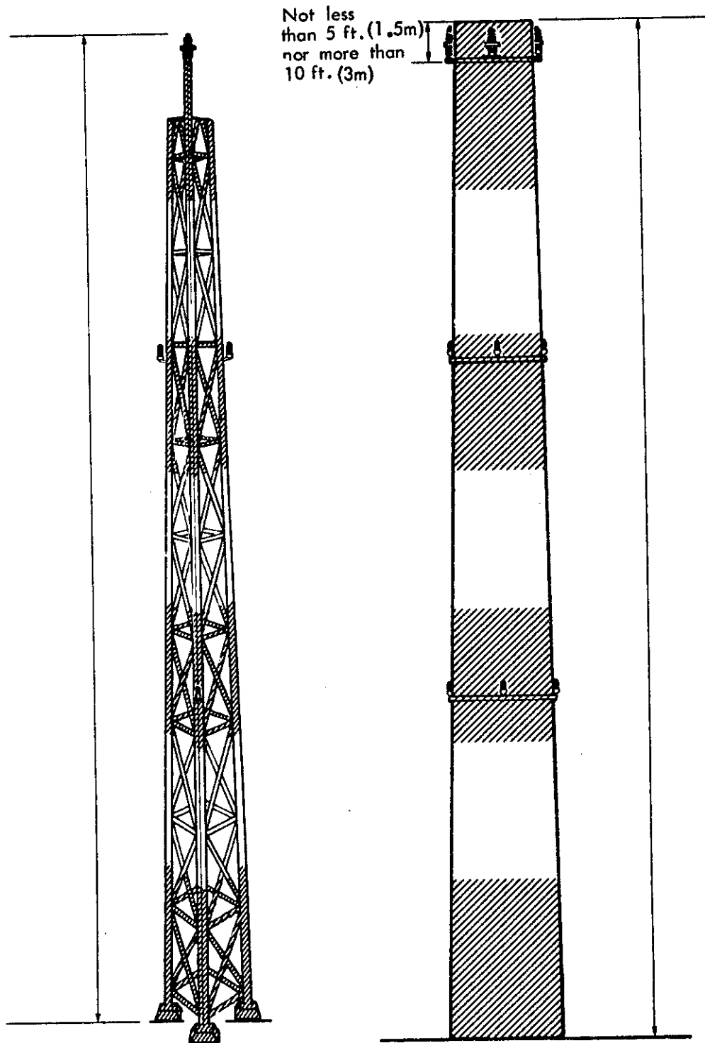
More than 300 ft. (90m) but not more than 450 ft. (135m) PAINTING AND LIGHTING OF CHIMNEYS, POLES, TOWERS AND SIMILAR OBSTRUCTIONS Fig. 2.
