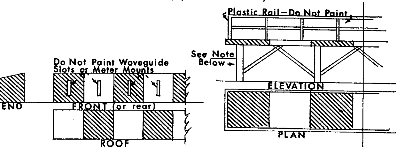
DIRECTIONAL LOCALIZER WAVEGUIDE SHELTER
