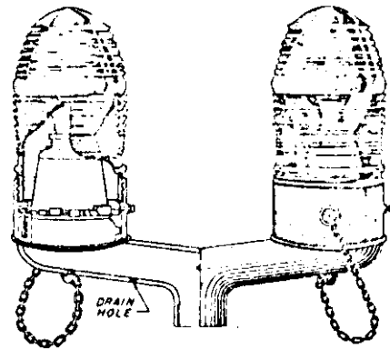
DOUBLE OBSTRUCTION
