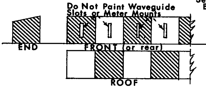
DIRECTIONAL LOCALIZER WAVEGUIDE SHELTER
