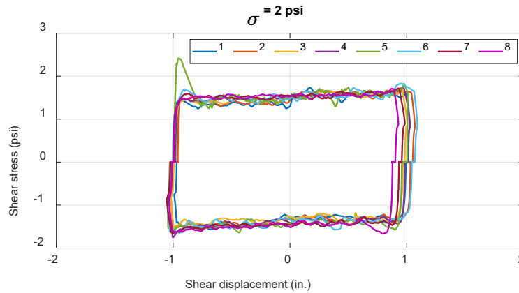
Figure 4.20: Cyclic shear stress-displacement relationship for HMA layer with felt paper.
