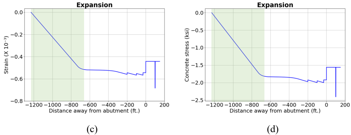
Figure 5.37: Axial behavior of transition slab connected with CRCP (temperature increase): (a) Axial force; (b) Longitudinal displacement; (c) Strain; (d) Concrete stress.
