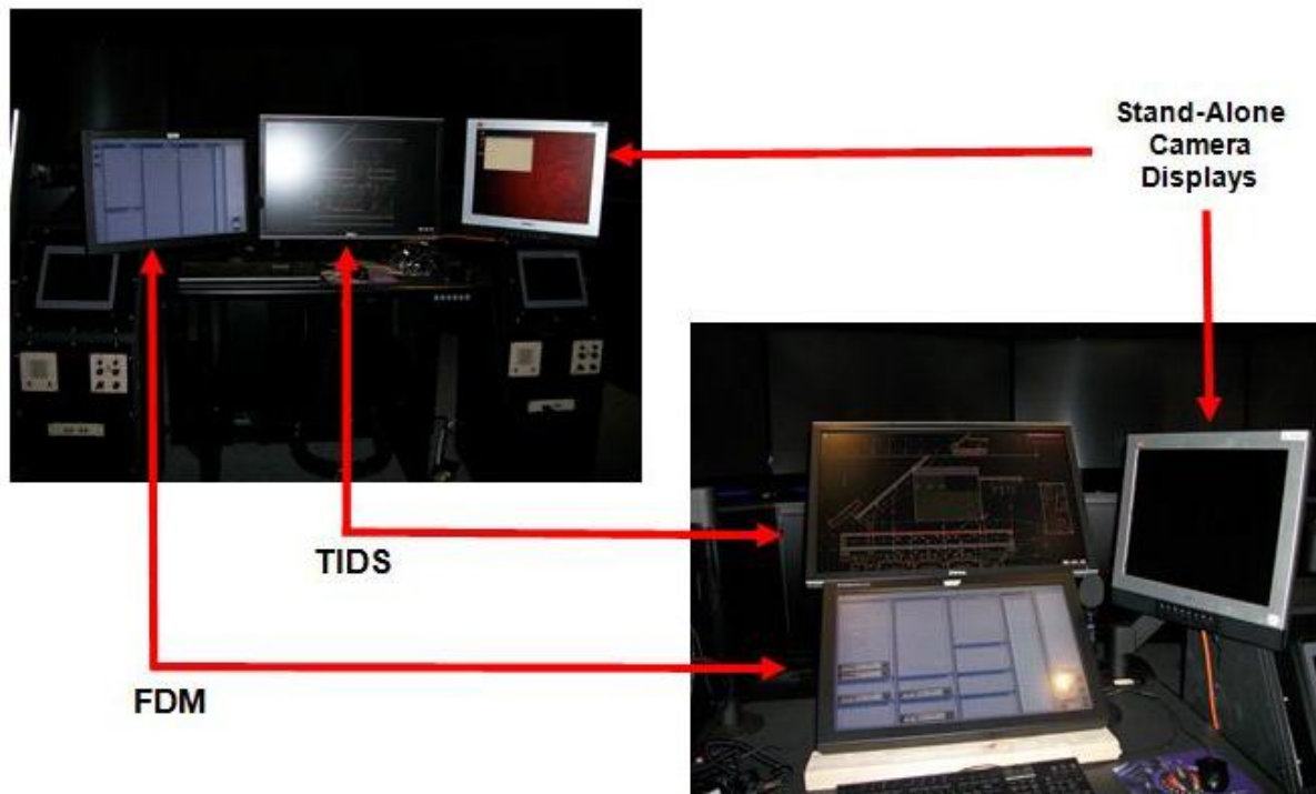
Figure 4. An example of the two display configurations. TIDS = Tower Information Display System and FDM = Flight Data Manager.
