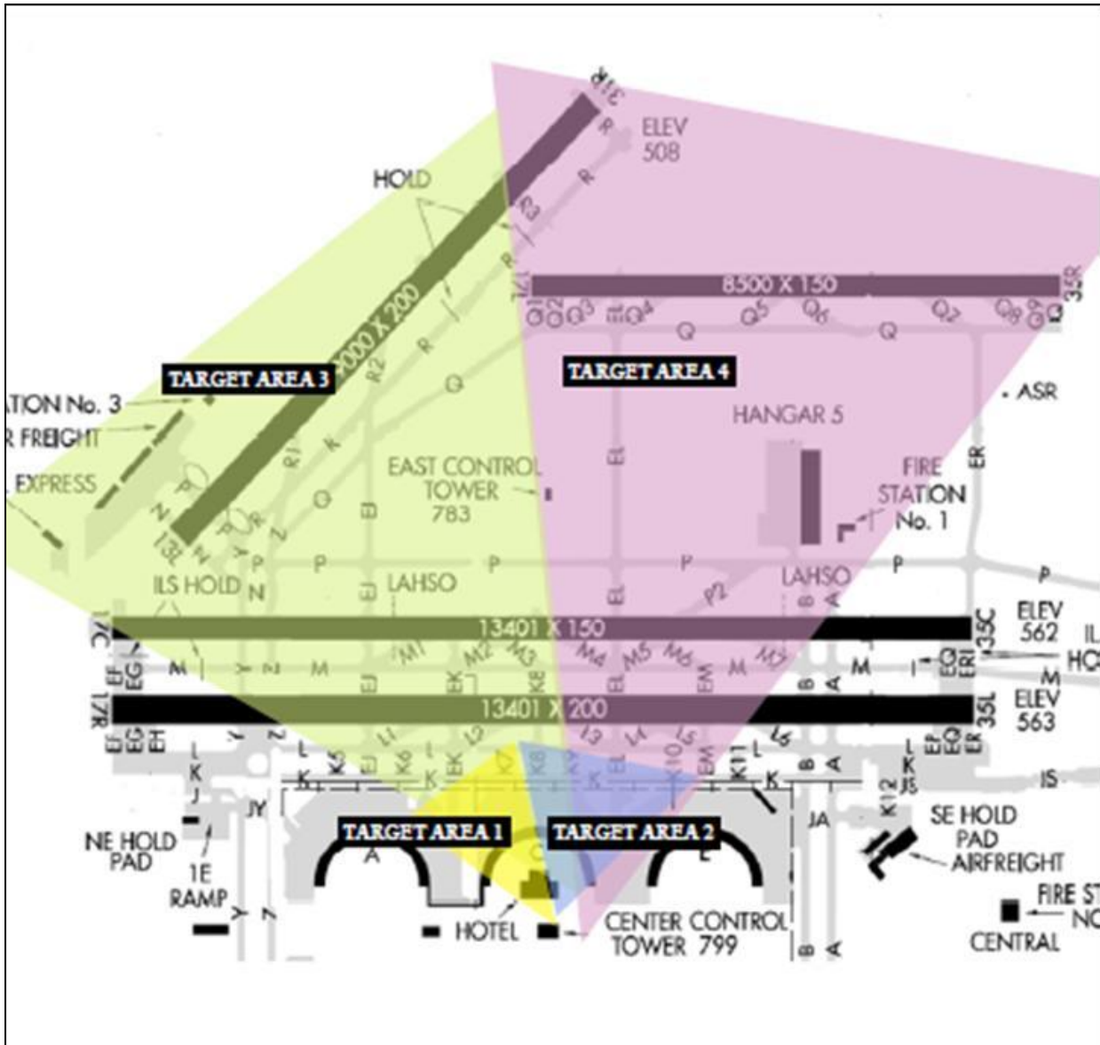
Figure. Potential coverage and viewing areas from Center Control Tower camera placement.
