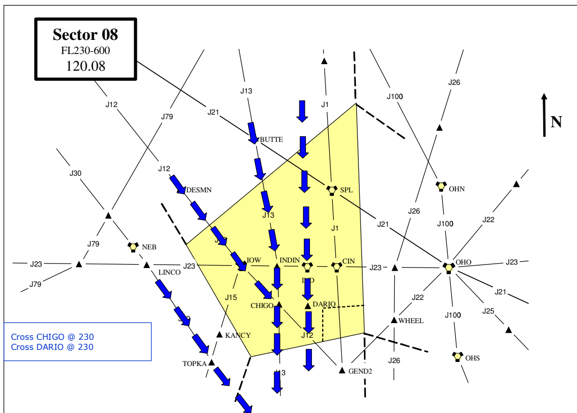
Figure 1. Airspace configuration.
