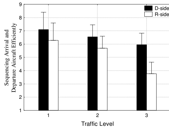
Figure 62. Over-the-shoulder rating of performance on sequencing arrival and departure aircraft efficiently as a function of Traffic Level and Controller Position.
