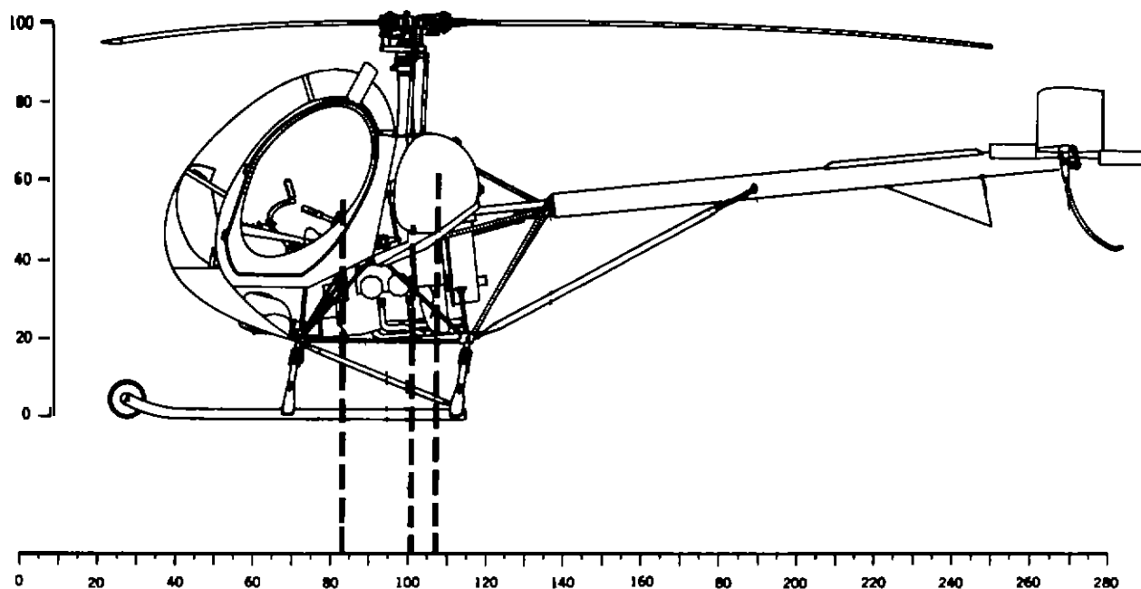
FIGURE 47—Datum line forward of helicopter
