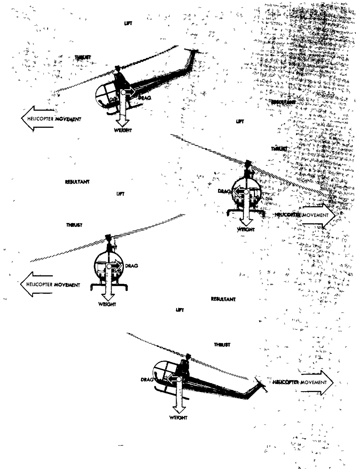
FIGURE 11 — Forces acting on the helicopter during forward, sideward, and rearward flight
