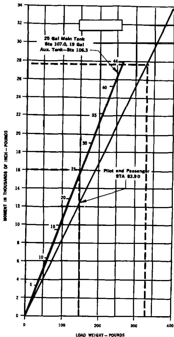
FIGURE 48—Loading chart
