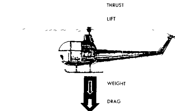
VERTICAL DESCENT
