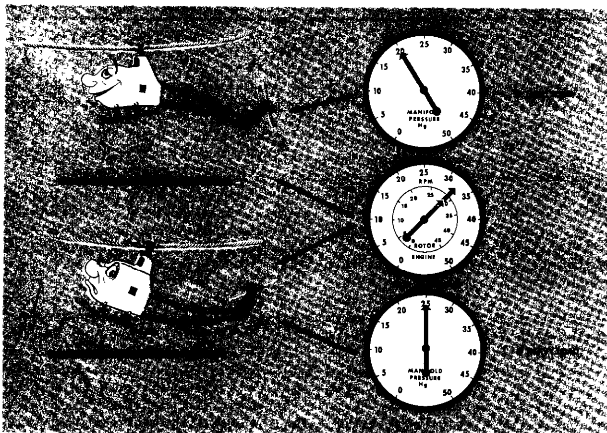
FIGURE 62—Heavy loads (high gross weights) decrease helicopter performance.
