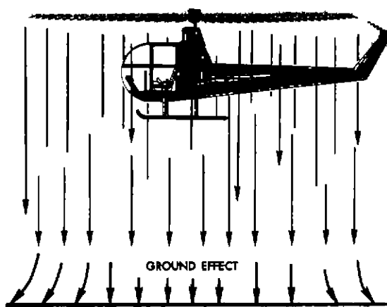
FIGURE 21 Ground effect results when the rotor downwash field is altered from its free air state by the presence of the surface
