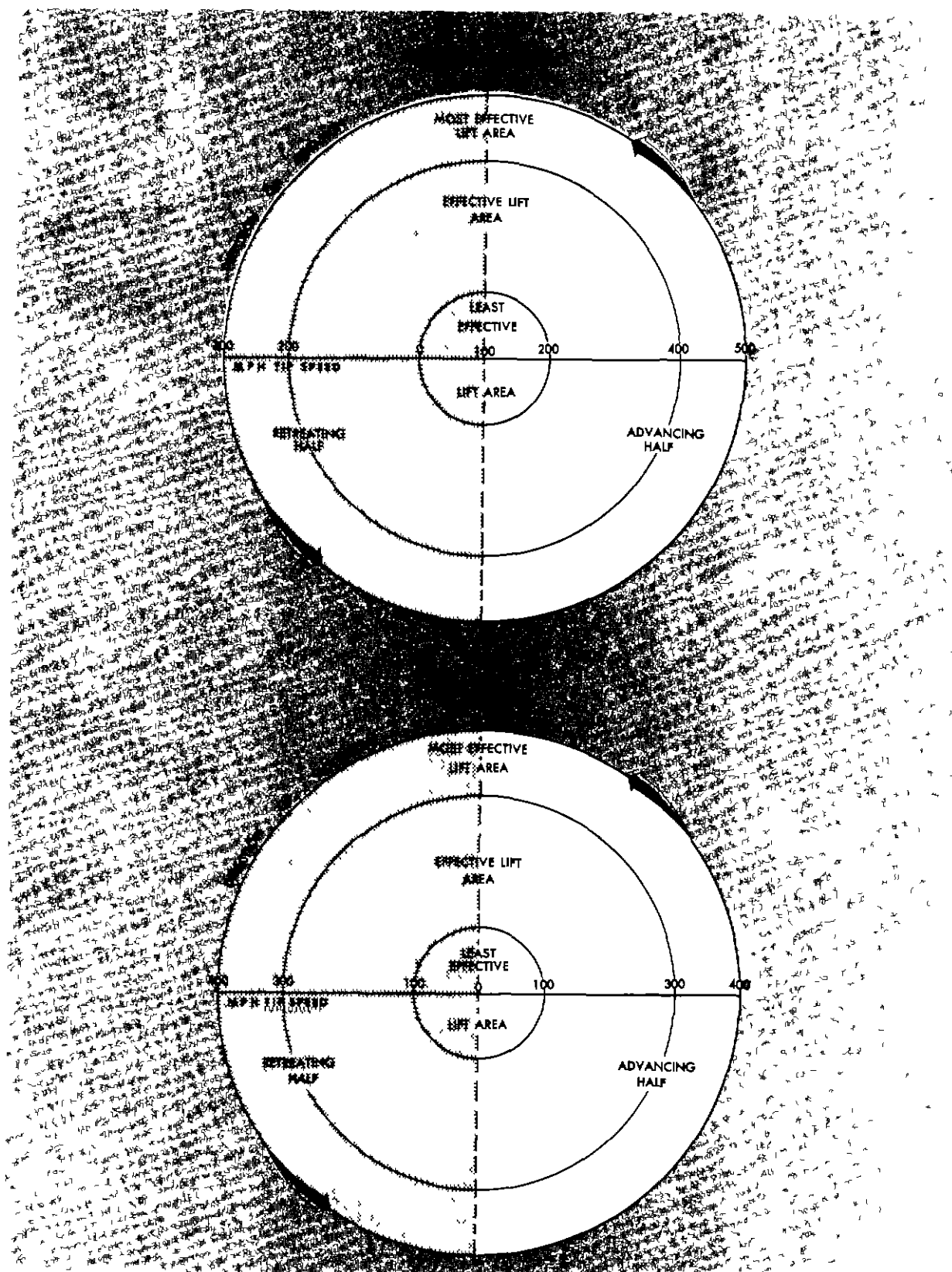
FIGURE 15—Comparison of rotor blade speeds for the advancing blade and retreating blade during hovering and forward flight
