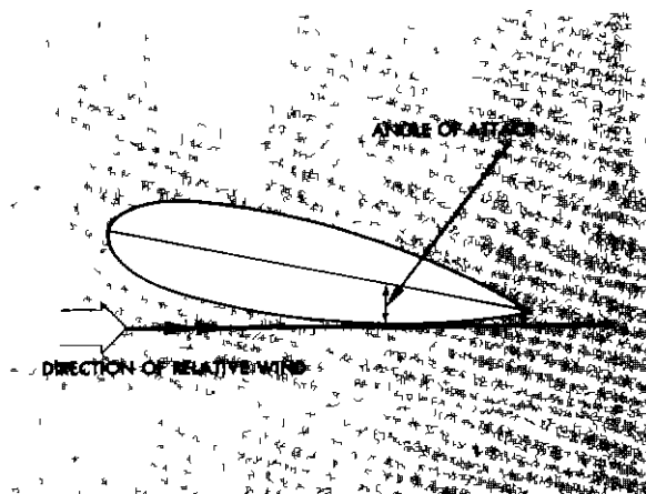
FIGURE 5—Angle of attack is the angle between the relative wind line and the chord line
