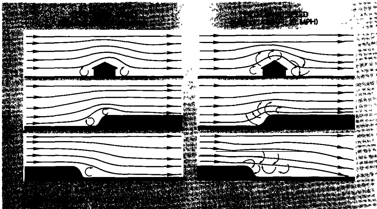
FIGURE 81 —Eddy currents are formed when the wind flows over uneven ground or obstructions
