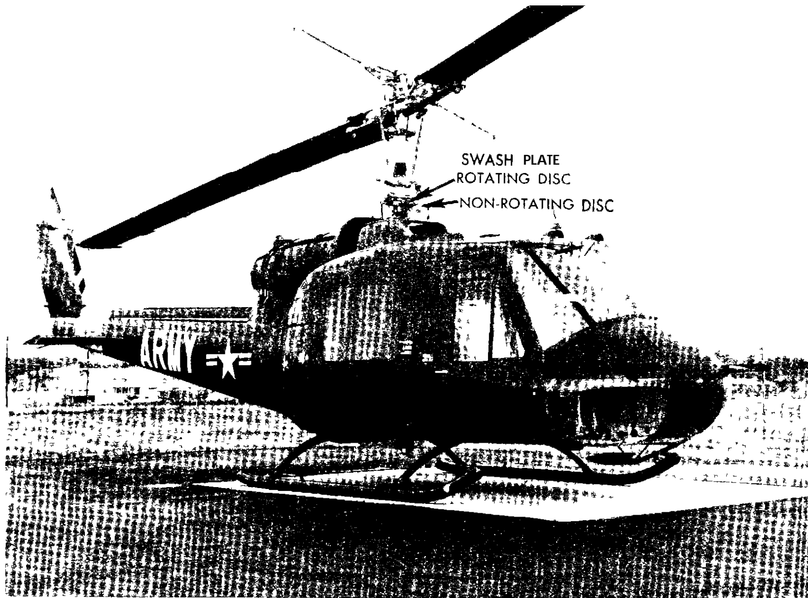
FIGURE 36—Swash plate system for one helicopter
