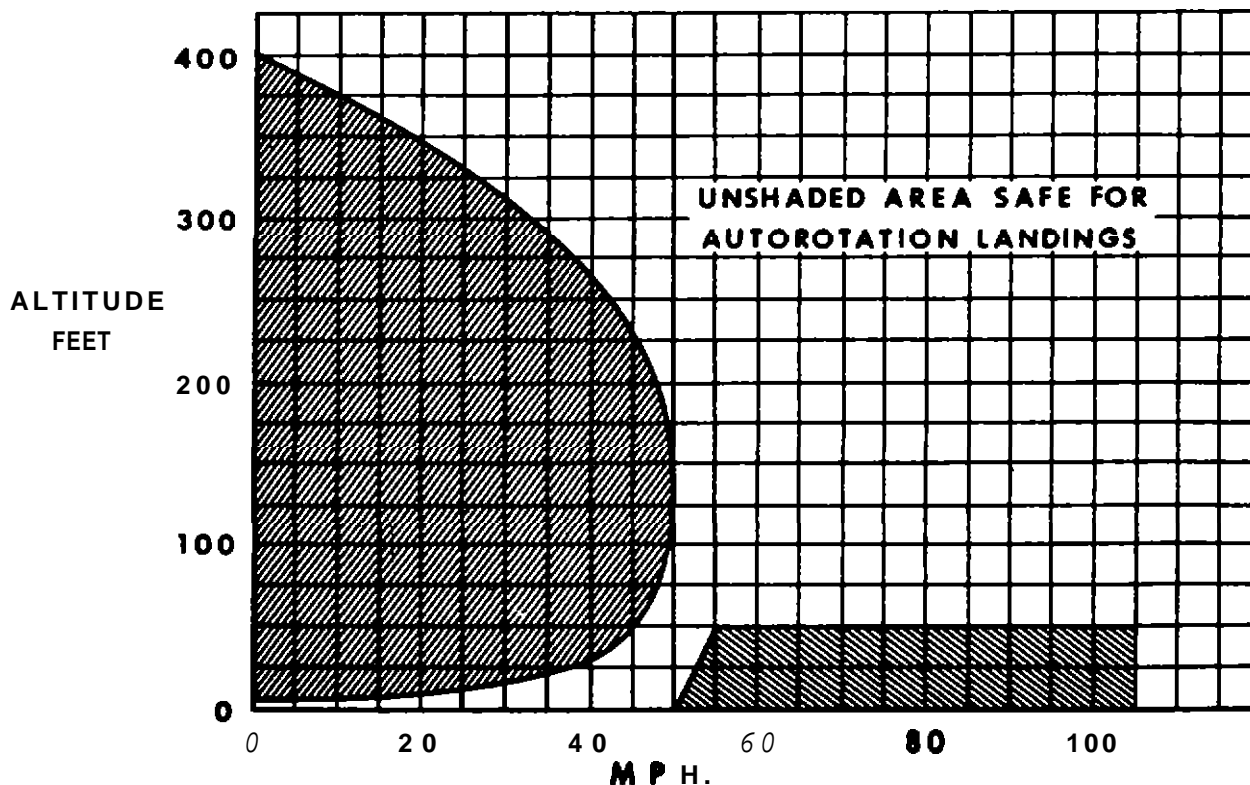
FIGURE 44—Airspeed vs altitude limitations chart
