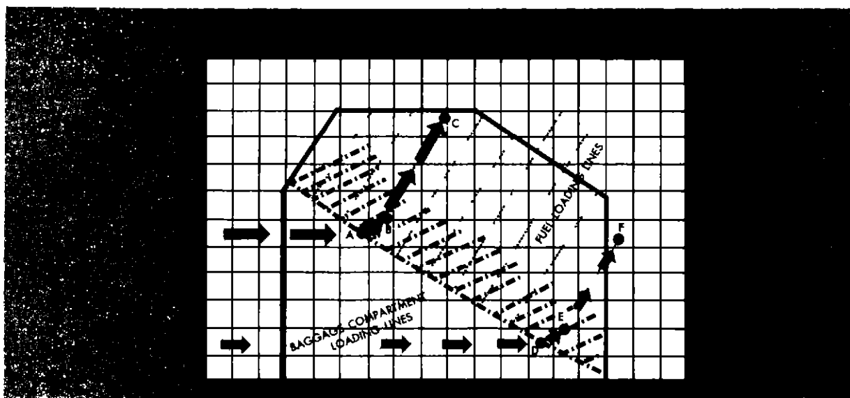
FIGURE 46—Loading chart illustrating the solution to sample problems 1 and 2
