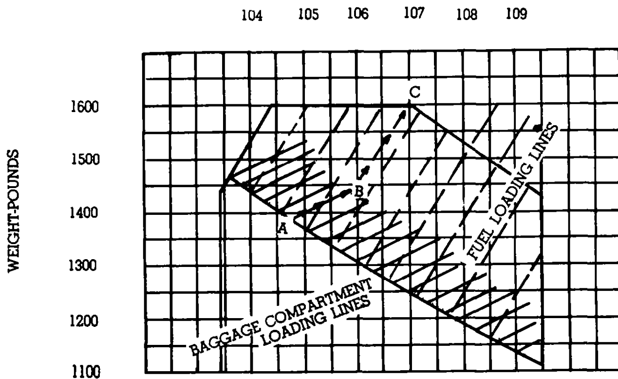
FIGURE 41 —Loading chart
