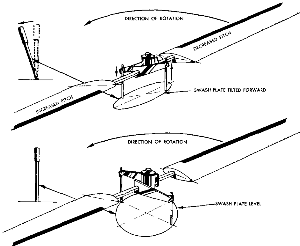
FIGURE 35—Cyclic stick movements are transmitted by a mechanical linkage through the swash plate to the rotor pitch horns and result in a change in the pitch angle of each rotor blade.
