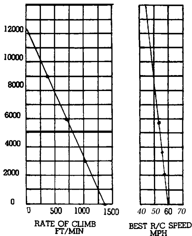
FIGURE 60—Rate of climb and best rate of climb speed chart.
