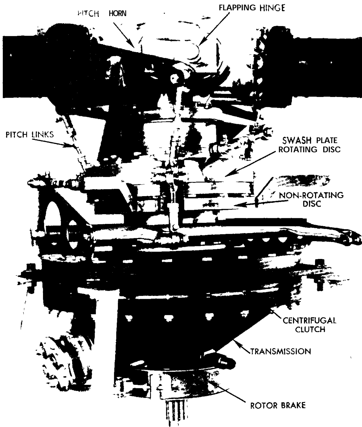
FIGURE 34 -Various components of the rotor System in One Helicopter
