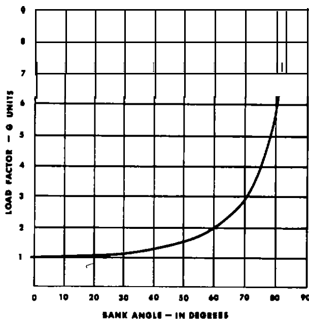
FIGURE 26—Load factor chart.
