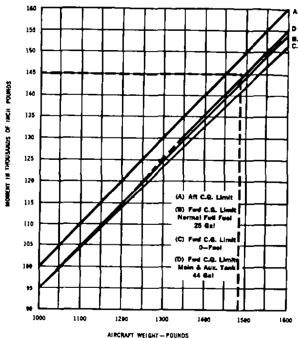
FIGURE 49—Center-of gravity chart
