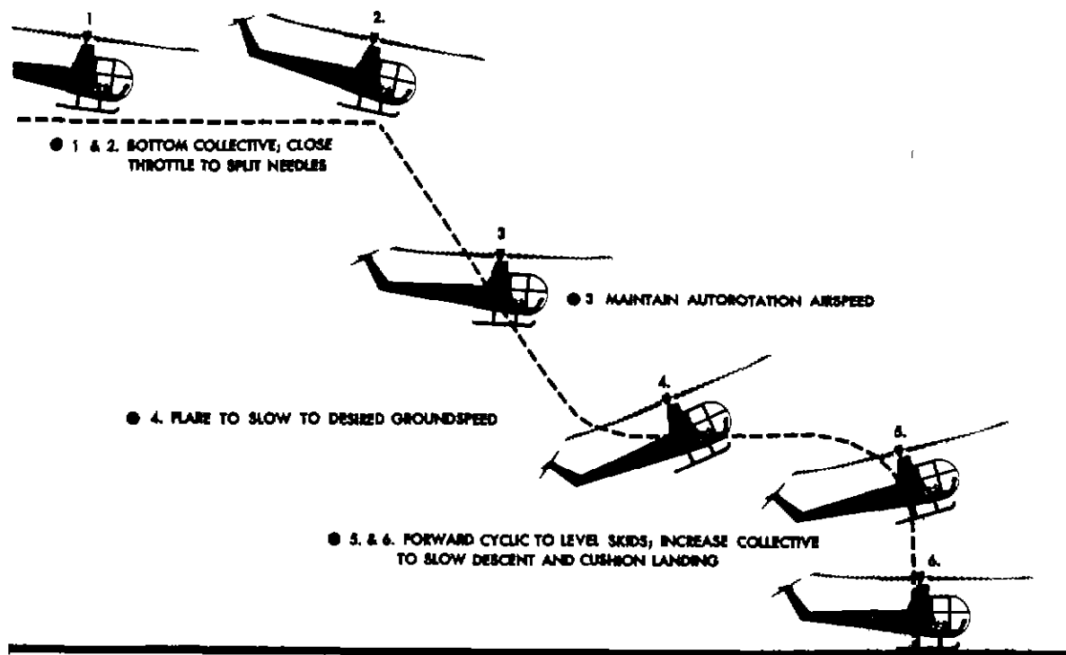
FIGURE 77 —Flare autorotation and touchdown
