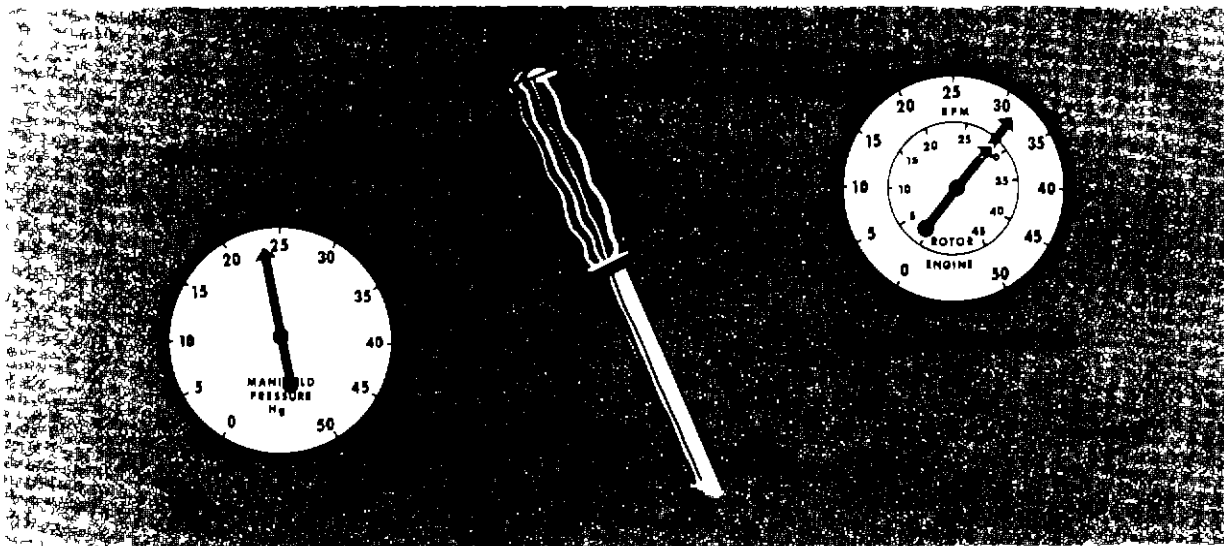
FIGURE 29—Collective pitch stick is primary control for manifold pressure; throttle is primary control for RPM. A change in either control results in a change in both manifold pressure and RPM.
