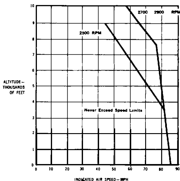
FIGURE 39 —Chart showing never-exceed ( V_{ne} ) speed limits
