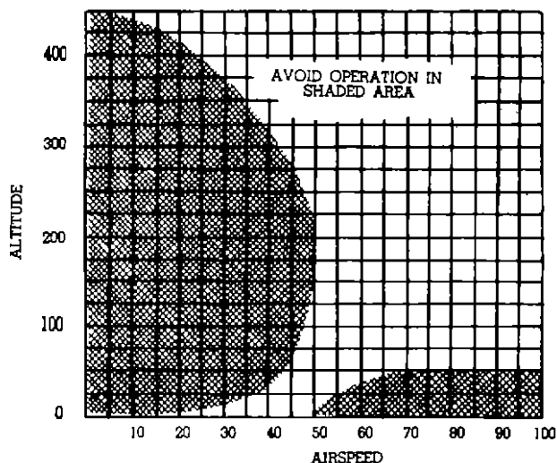
FIGURE 43—Airspeed vs altitude limitations chart.
