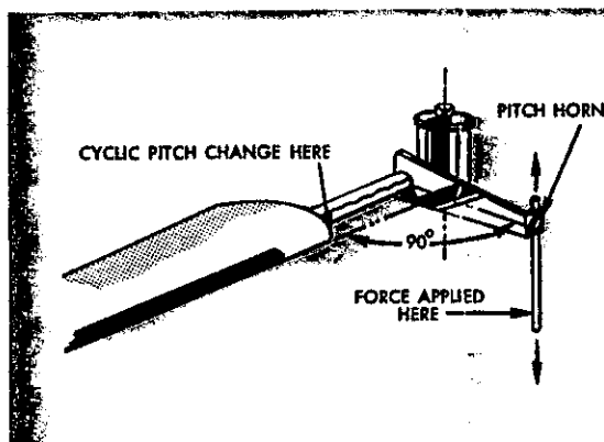
FIGURE 34.—Rotor blade pitch horns are located 90^\circ ahead of or behind (depending on the manufacturer) the rotor blade so that helicopter reaction will be in the direction of cyclic stick displacement.
