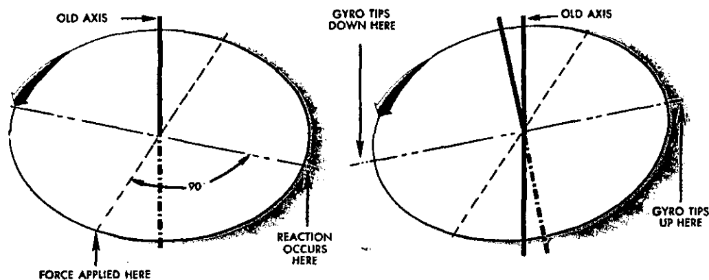
FIGURE 13.—Gyroscopic Precession Principle: When a force is applied to a spinning gyro, the maximum reaction occurs 90^\circ later in the direction of rotation.
