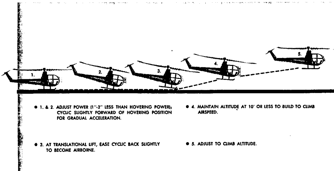
FIGURE 75.—High altitude (running) takeoff.
