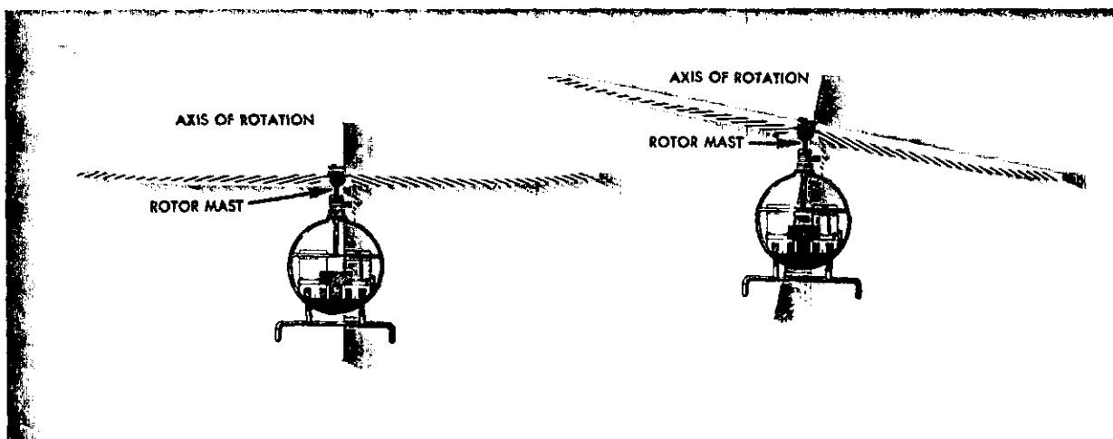
FIGURE 18.—The axis of rotation is the imaginary line about which the rotor rotates and is perpendicular to the tip-path plane.
