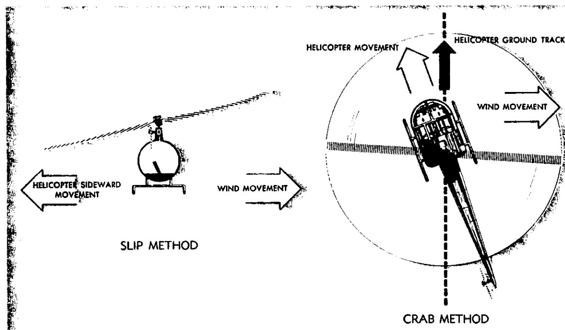
FIGURE 71.—Comparison of the slip method and crab method of wind drift correction.
