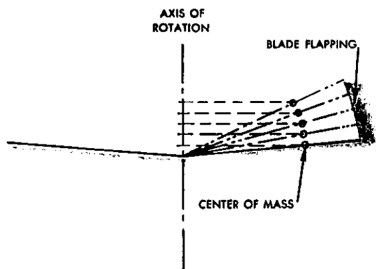
FIGURE 19.—Coriolis effect is the change in blade velocity to compensate for the change in distance of the center of mass from the axis of rotation as the blades flap.
