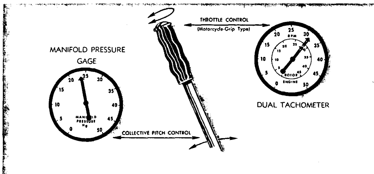
FIGURE 29.—Collective pitch stick is primary control for manifold pressure; throttle is primary control for RPM. A change in either control results in a change in both manifold pressure and RPM.
