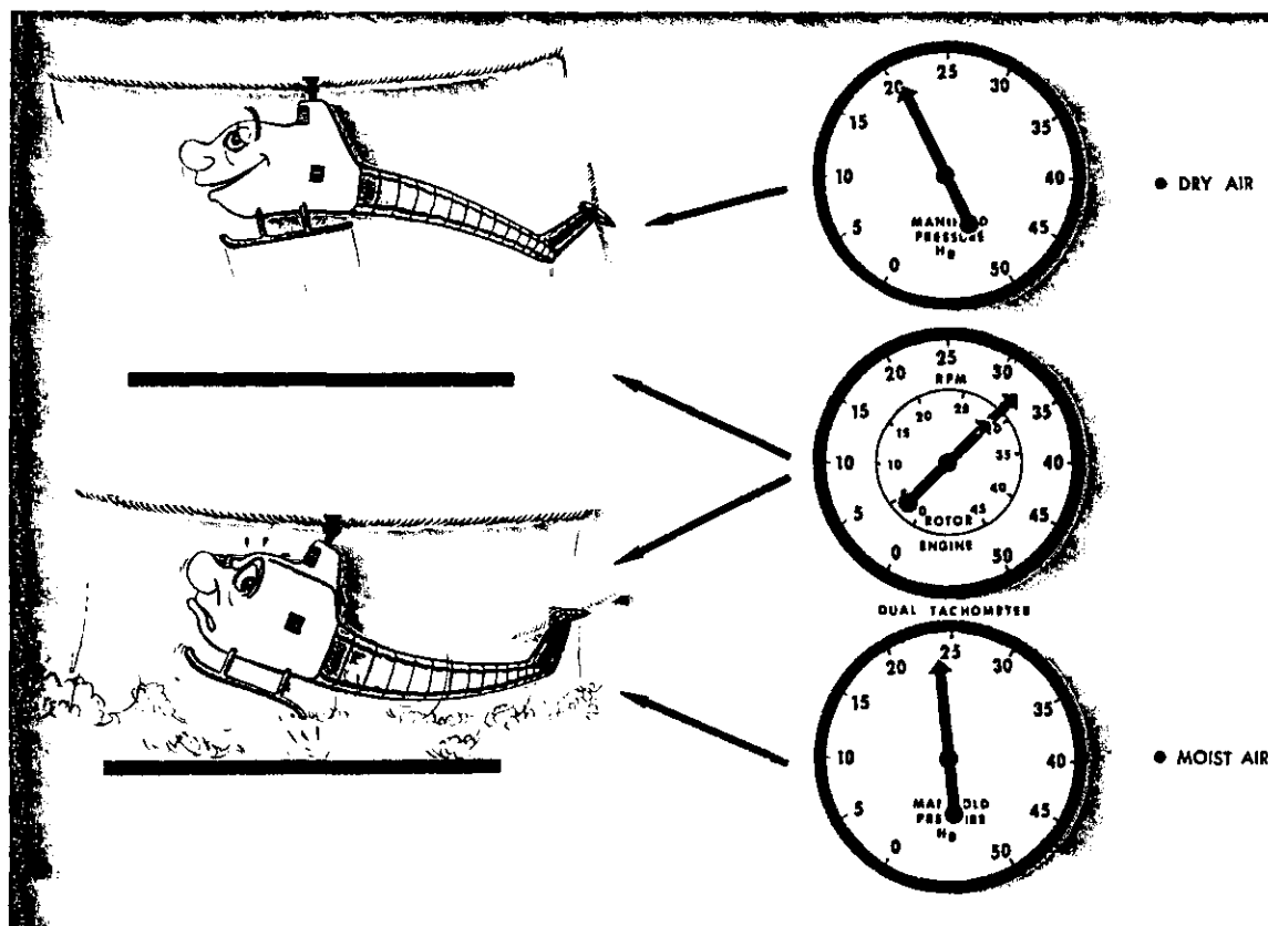
FIGURE 54.—High humidity (especially on hot days) reduces helicopter performance.
