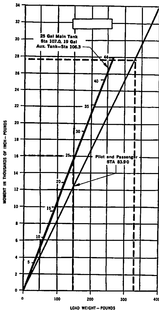
FIGURE 48.—Loading chart.
