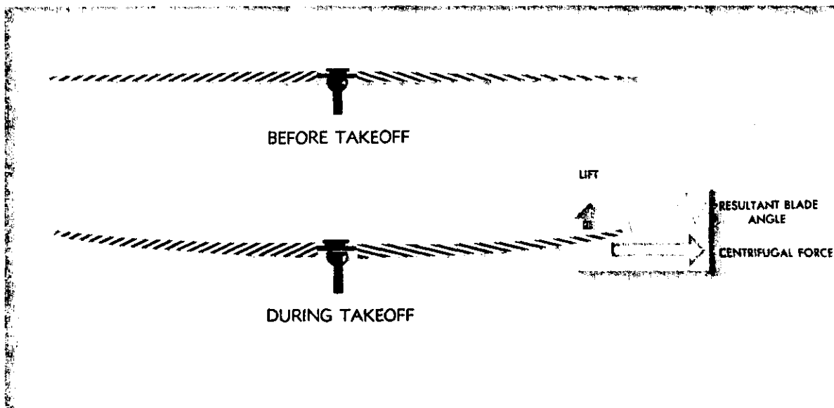
FIGURE 17.—Blade coning is a result of lift and centrifugal force.
