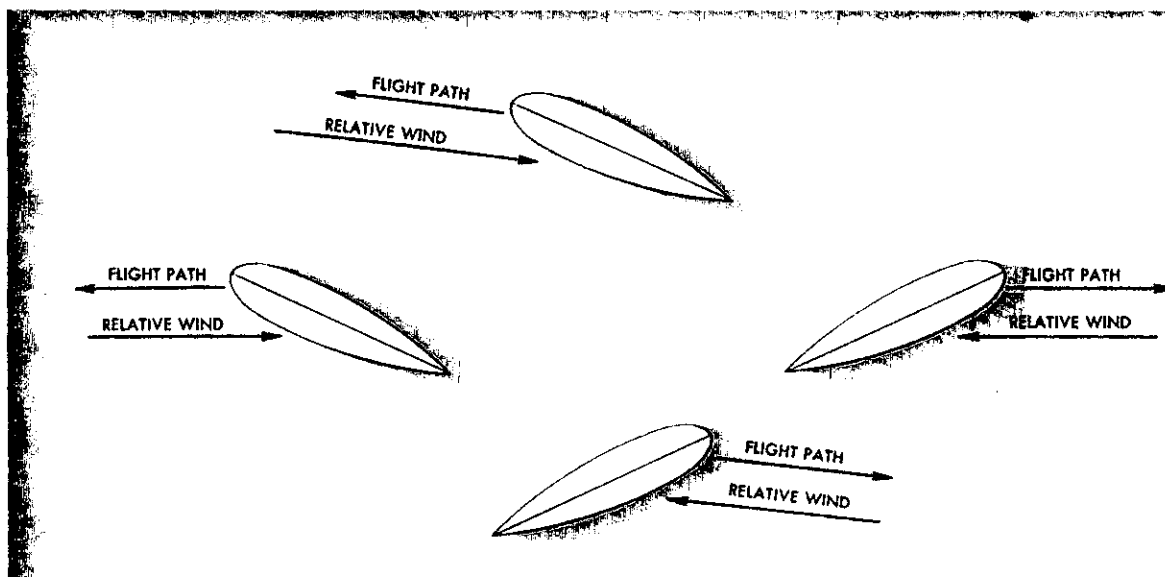
FIGURE 3.—Relationship between the flight path of an airfoil and relative wind. Relative wind is parallel and in the opposite direction to the flight path.
