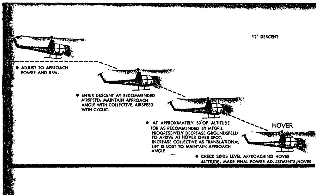
FIGURE 72.—Normal approach to a hover.
