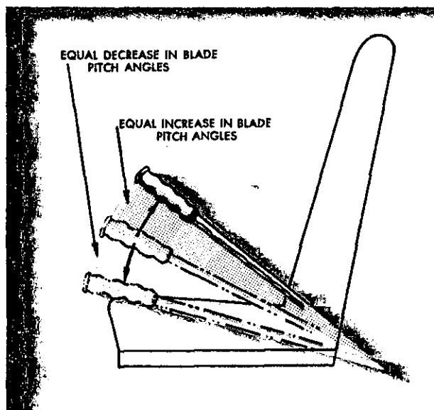
FIGURE 28.—Collective pitch stick movement produces equal changes in blade pitch angles.
