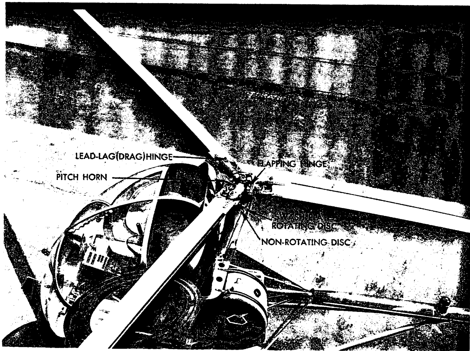
FIGURE 37.—Various components of the rotor system in one helicopter.
