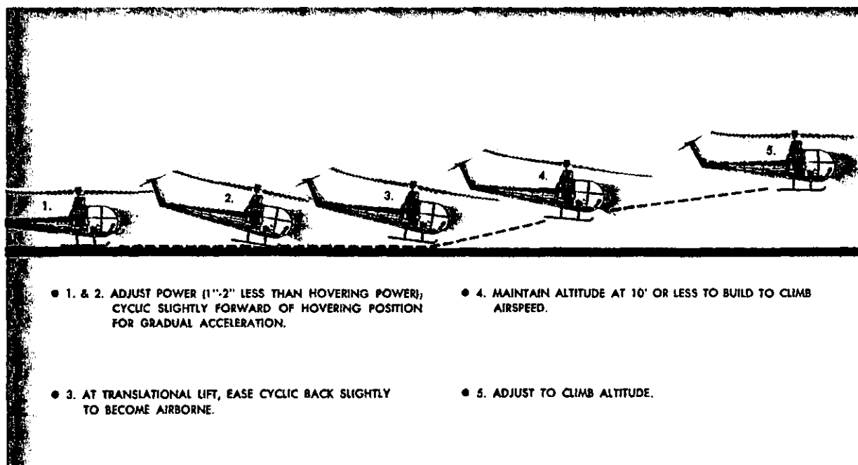
FIGURE 75.—High altitude (running) takeoff.
