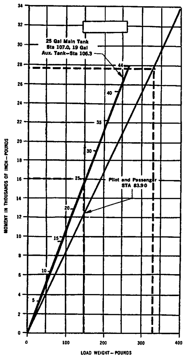
FIGURE 48.—Loading chart.
