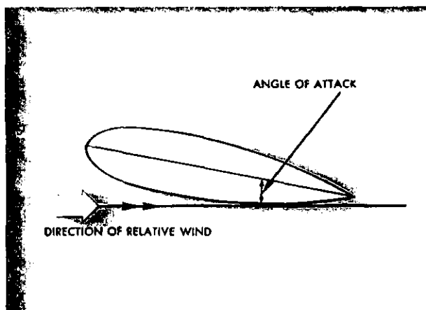
FIGURE 5.—Angle of attack is the angle between the relative wind line and the chord line.
