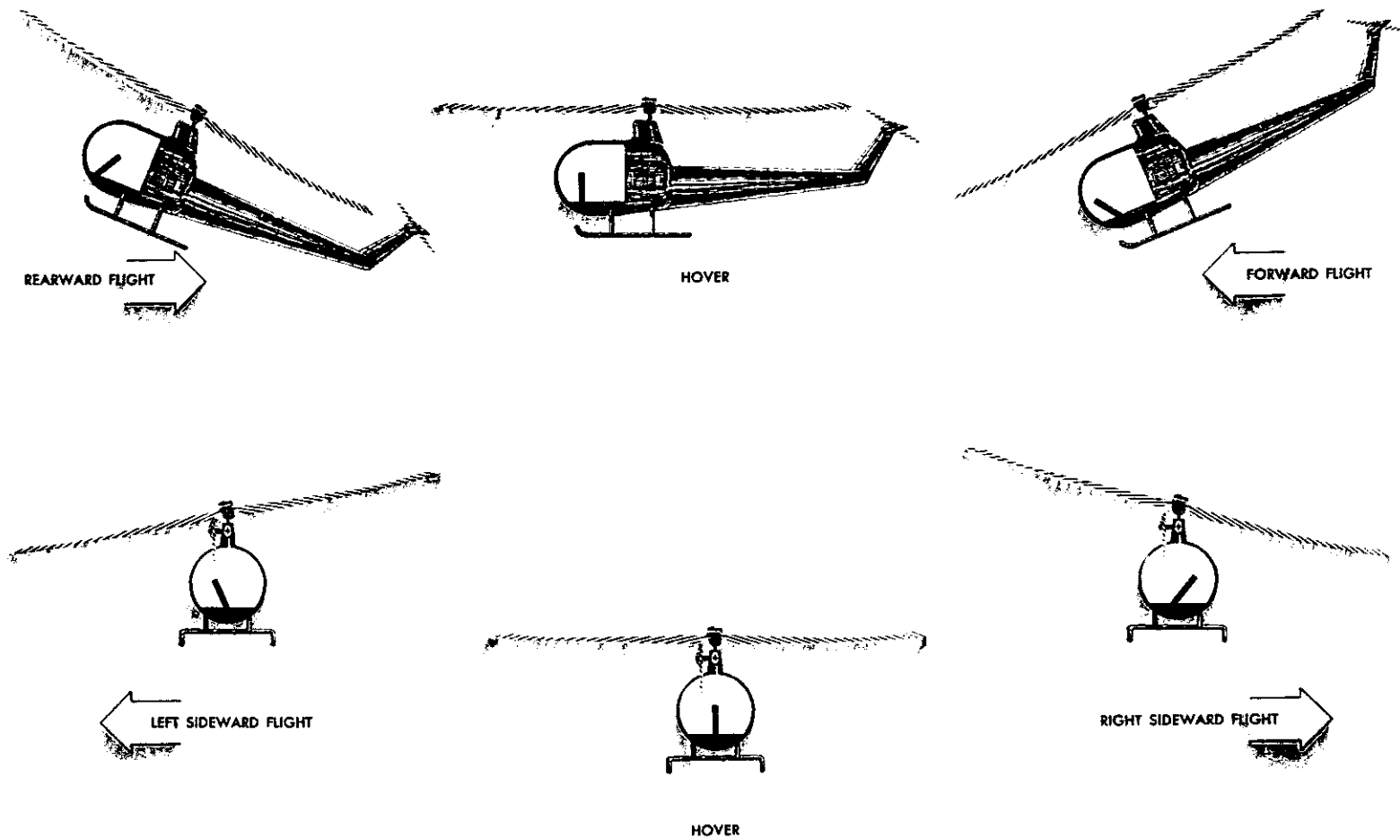
Figure 32.—Relationship of cyclic stick position to rotor disc position and helicopter movement.
