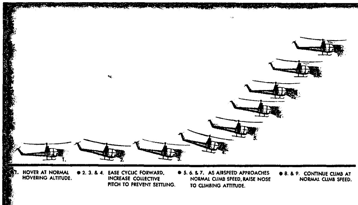
FIGURE 70.—Normal takeoff from a hover.
