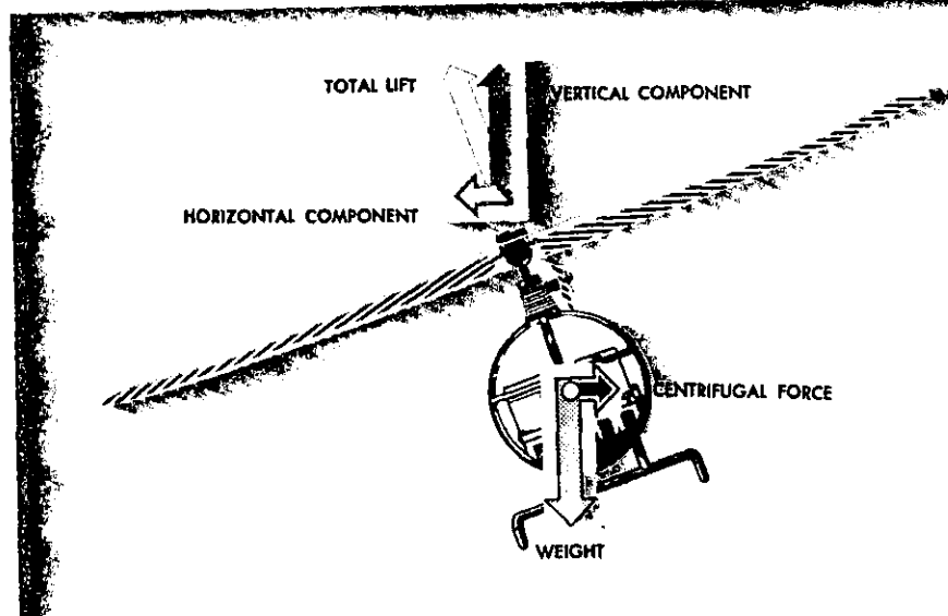
FIGURE 24.—Forces acting on a helicopter in a turn. Lift causes the helicopter to turn when it is banked.
