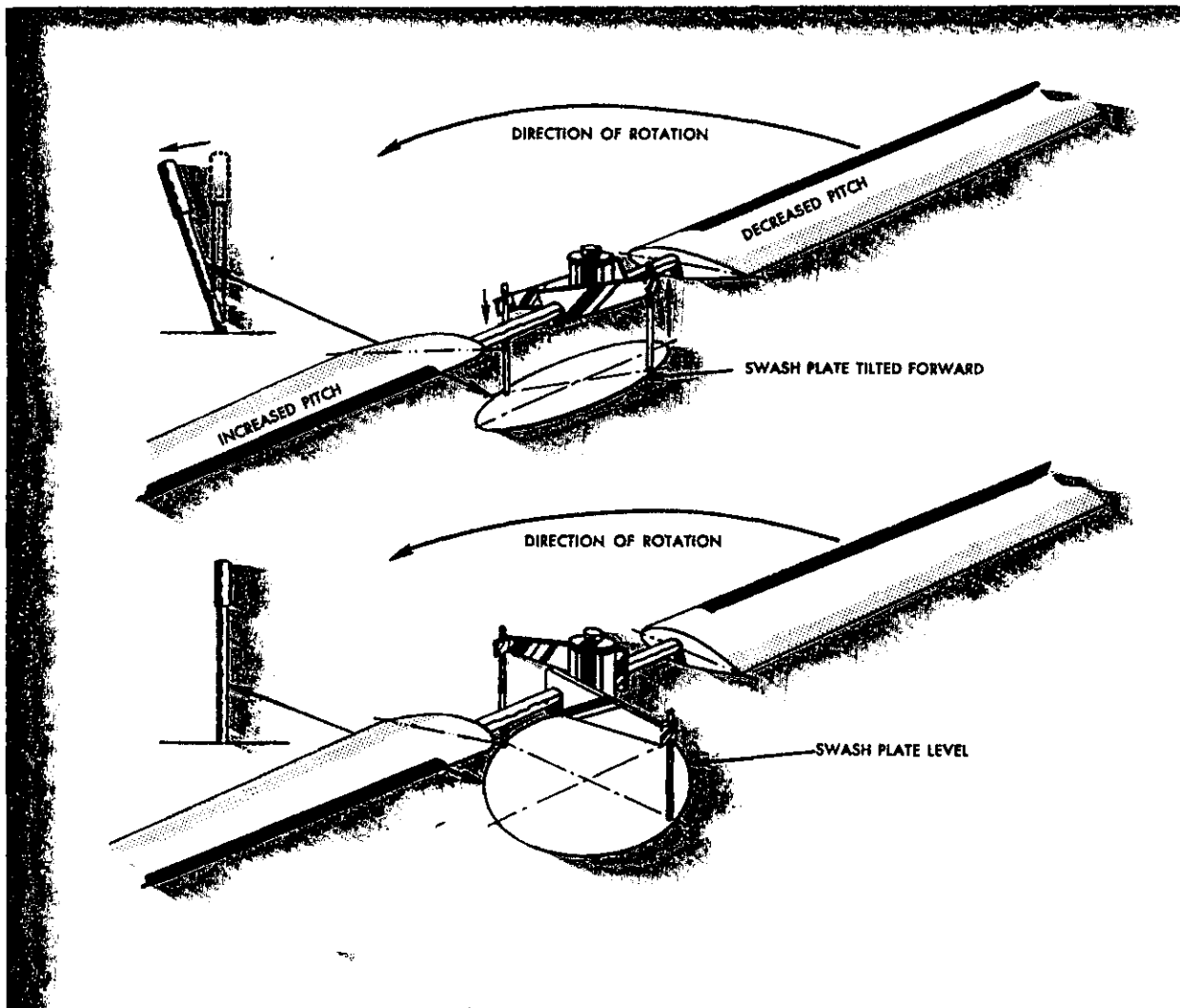
FIGURE 35.—Cyclic stick movements are transmitted by a mechanical linkage through the swash plate to the rotor pitch horns and result in a change in the pitch angle of each rotor blade.
