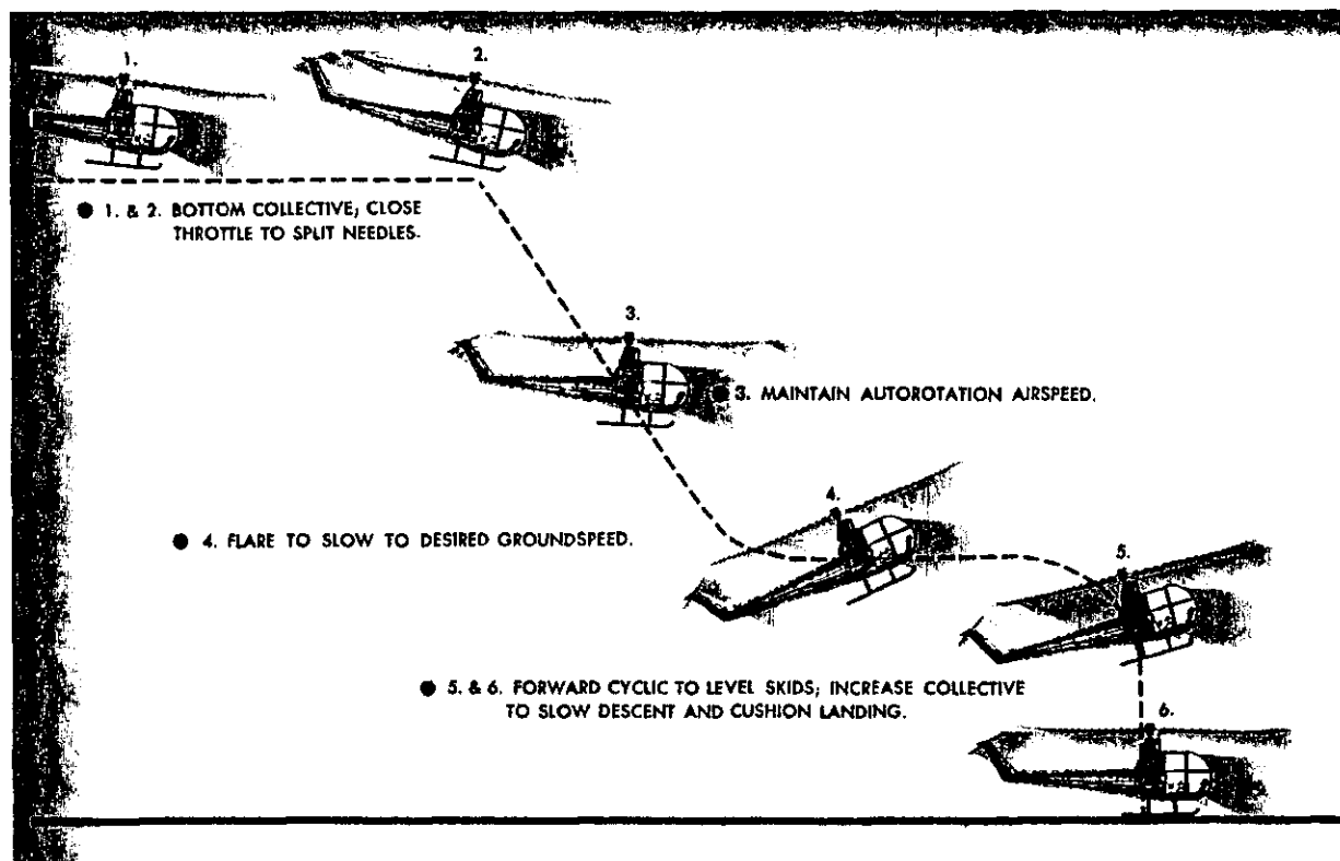
FIGURE 77.—Flare autorotation and touchdown.
