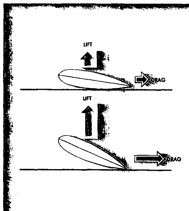
FIGURE 8.—Relationship between angle of attack and lift and drag forces. As the angle of attack increases, lift and drag increase.
