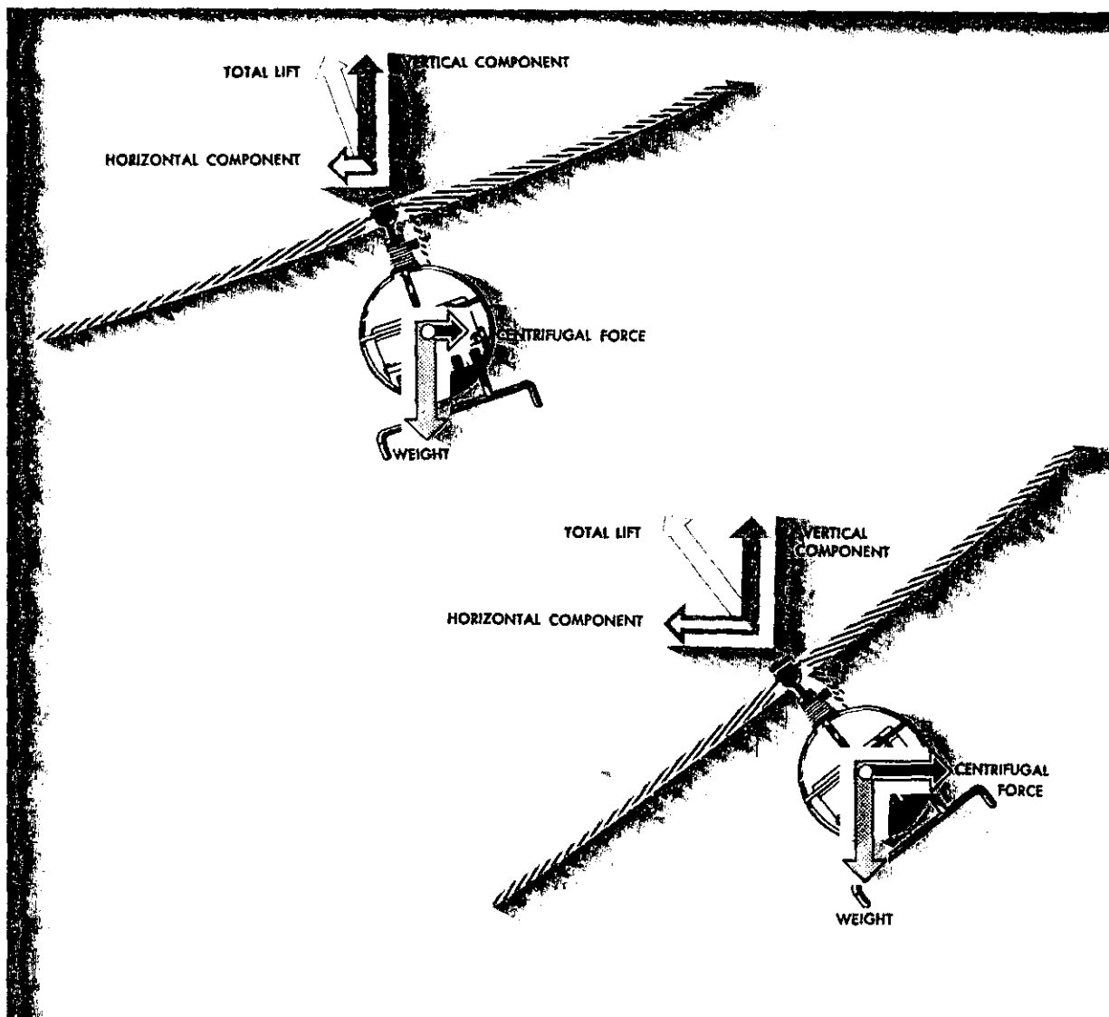
FIGURE 25.—Relationship between angle of bank and total lift force. As the angle of bank increases, the total lift force is tilted more horizontally, resulting in a faster rate of turn.
