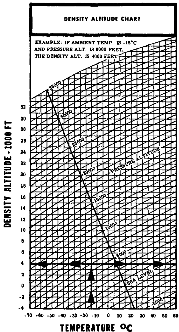
FIGURE 51.—Density altitude chart.
