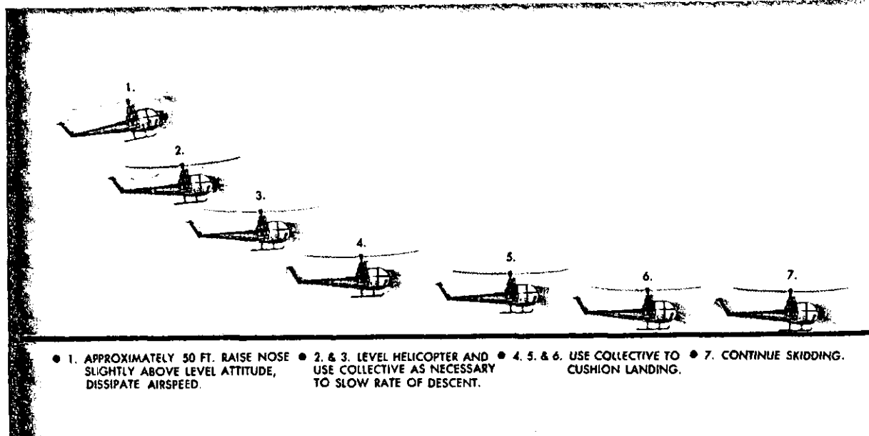
FIGURE 74.—Running landing.
