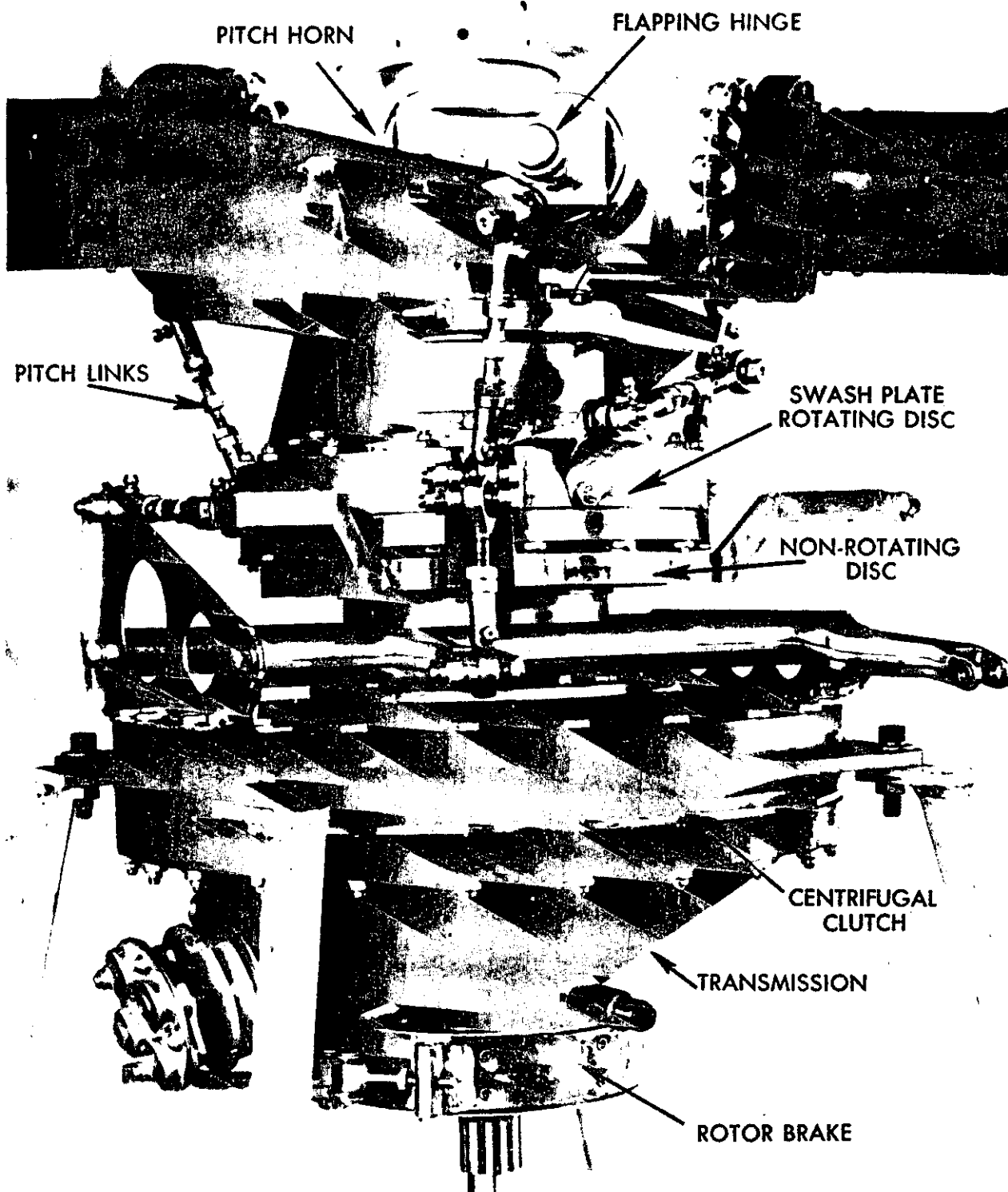
FIGURE 33.—Various components of the rotor system in one helicopter.
