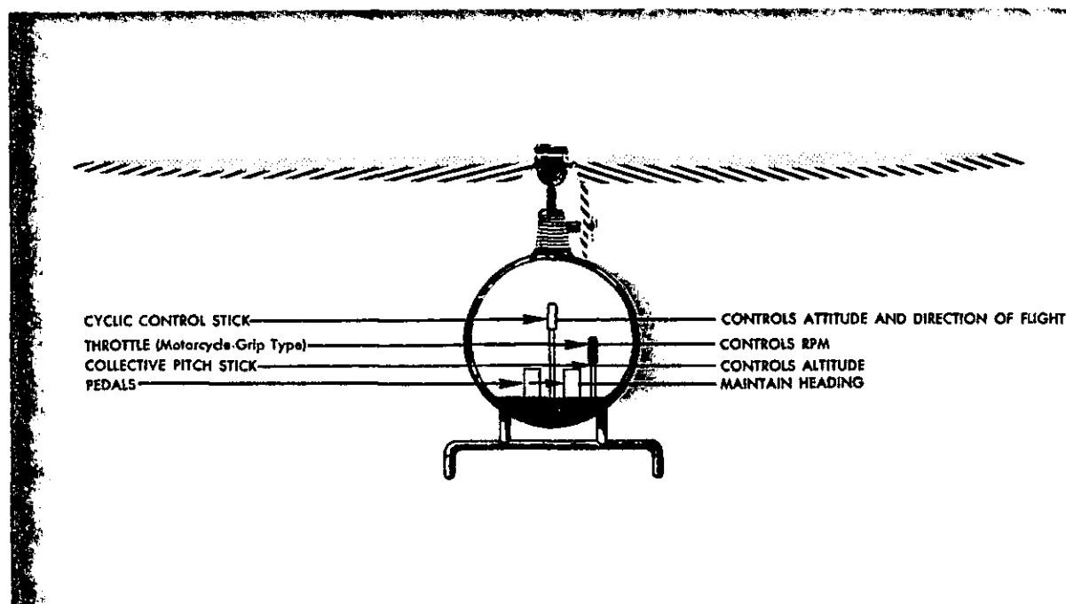
FIGURE 27.—Controls of the helicopter and the principal function of each control.
