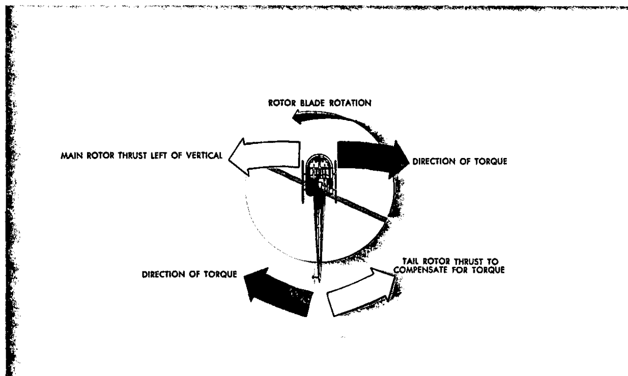
FIGURE 20.—Drift, caused by tail rotor thrust, is compensated for by rigging the mast or cyclic pitch system to have a built-in tilt of the tip-path plane to the left.
