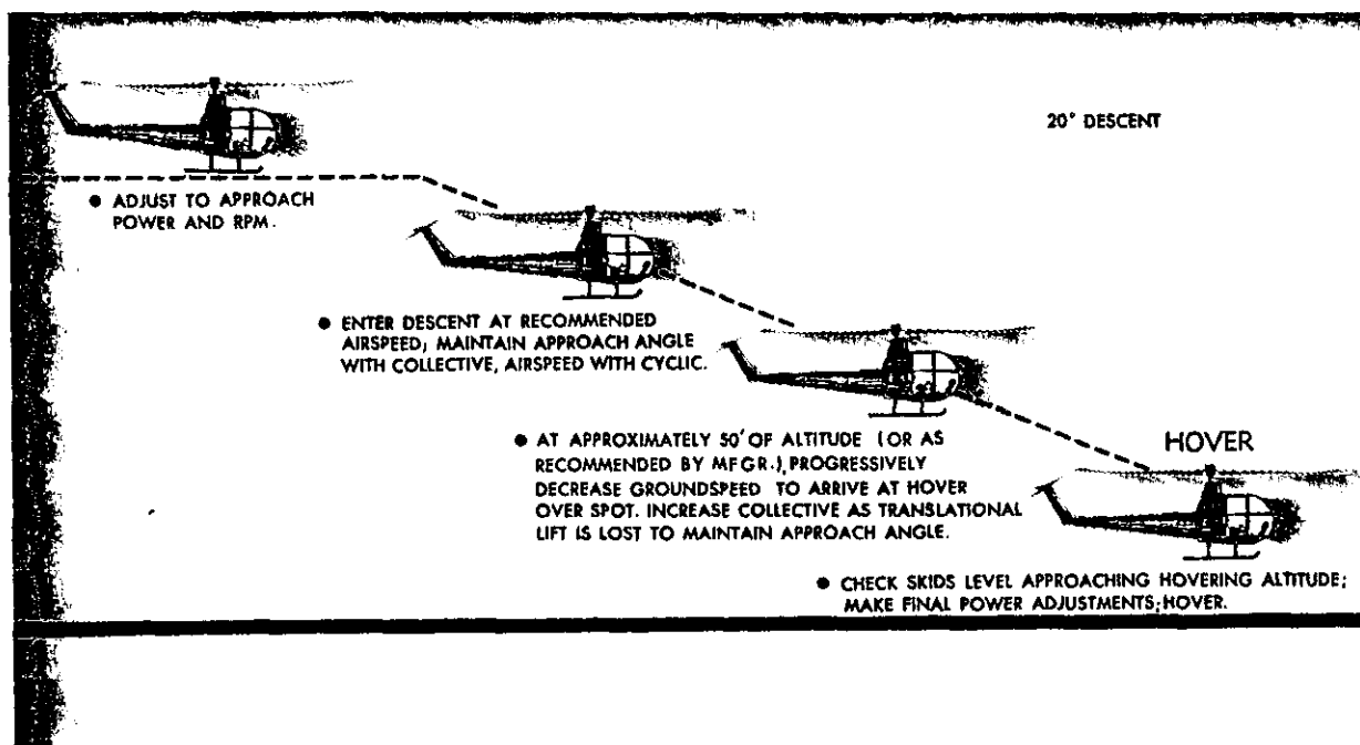
FIGURE 73.—Steep approach to a hover.
