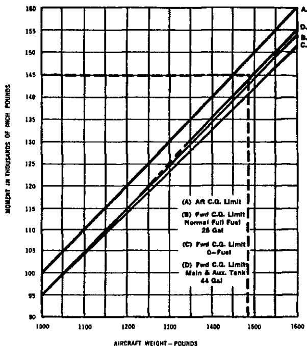
FIGURE 49.—Center-of-gravity chart.
