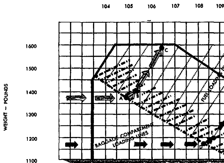
FIGURE 46.—Loading chart illustrating the solution to sample problems 1 and 2.
