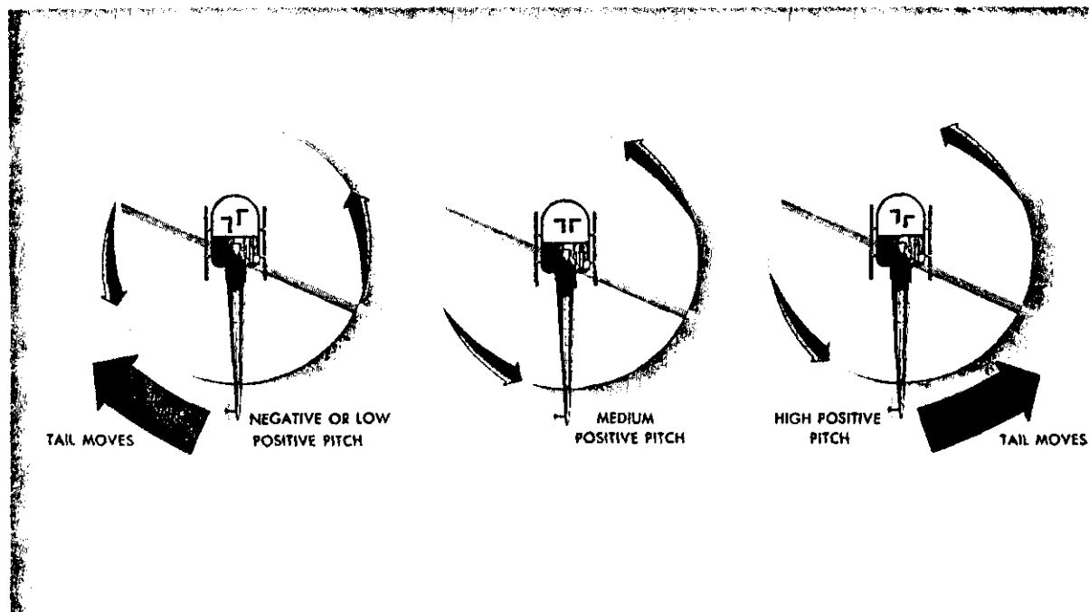
FIGURE 31.—Tail rotor pitch angle and thrust in relation to pedal positions during cruising flight.
