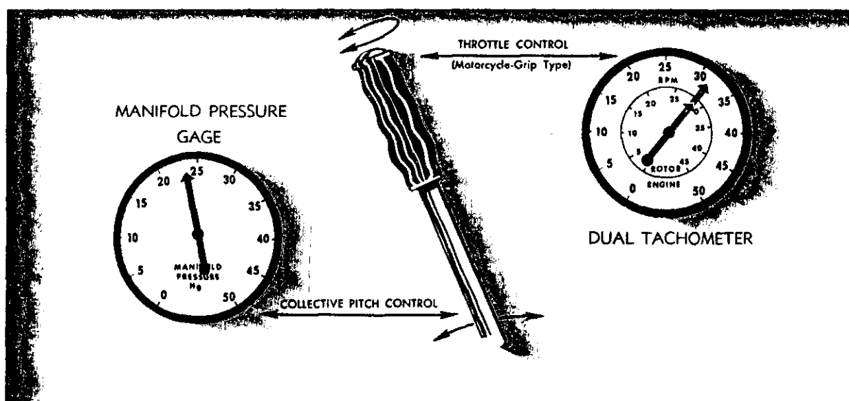
FIGURE 29.—Collective pitch stick is primary control for manifold pressure; throttle is primary control for rotor RPM. A change in either control results in a change in both manifold pressure and rotor RPM.
