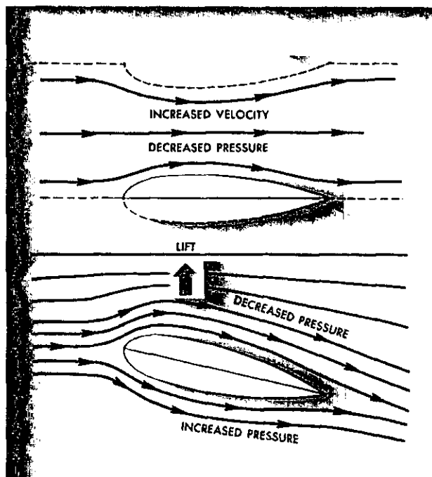
FIGURE 7.—(Top) Bernoulli's Principle: Increased air velocity produces decreased pressure; (Bottom) Lift is produced by an airfoil through a combination of decreased pressure above the airfoil (as per Bernoulli's Principle), and increased pressure beneath.
