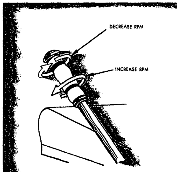
FIGURE 30.—Throttle control: Rotating the throttle outboard (viewed from the top) increases rotor RPM; rotating it in-board decreases rotor RPM.
