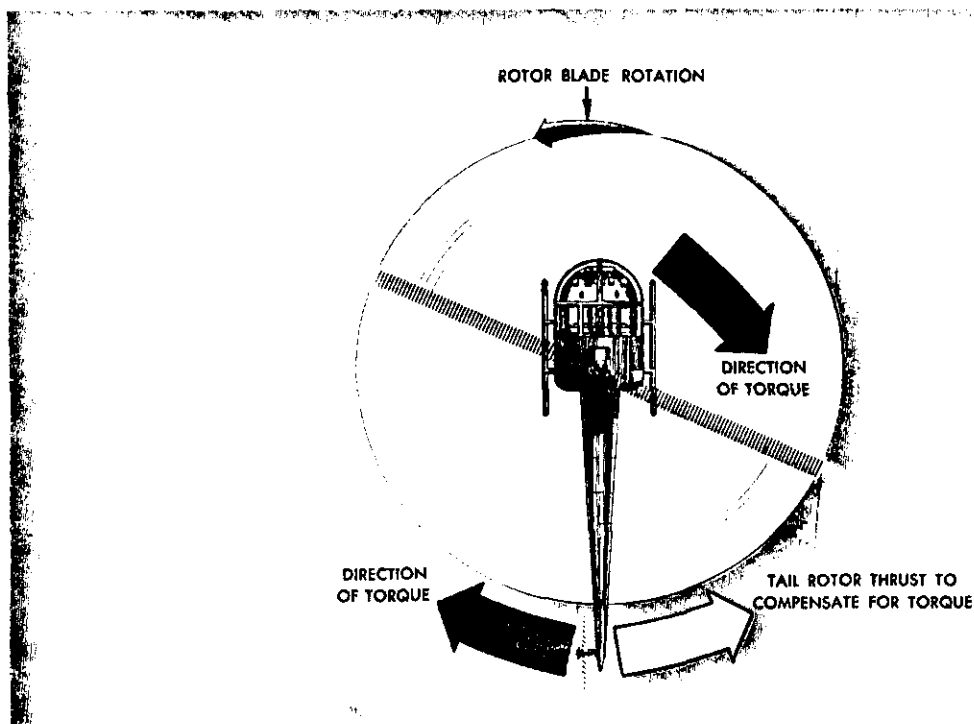
FIGURE 12.—Tail rotor thrust compensates for the torque effect of the main rotor.
