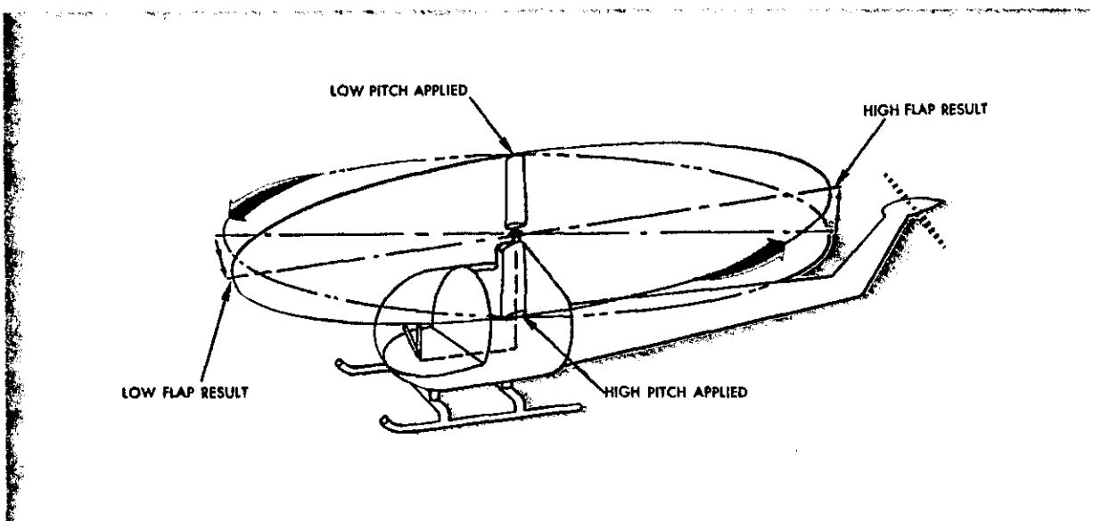
FIGURE 14.—Rotor disc acts like a gyro. When a rotor blade pitch change is made, maximum reaction occurs approximately 90^\circ later in the direction of rotation.
