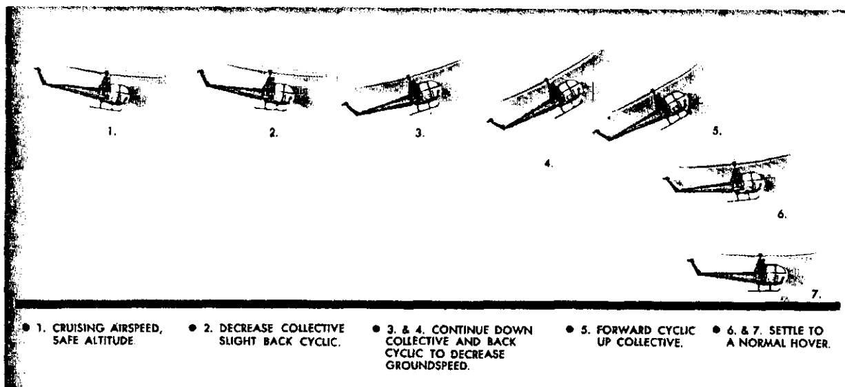
FIGURE 78.—Rapid deceleration or quick stop.
