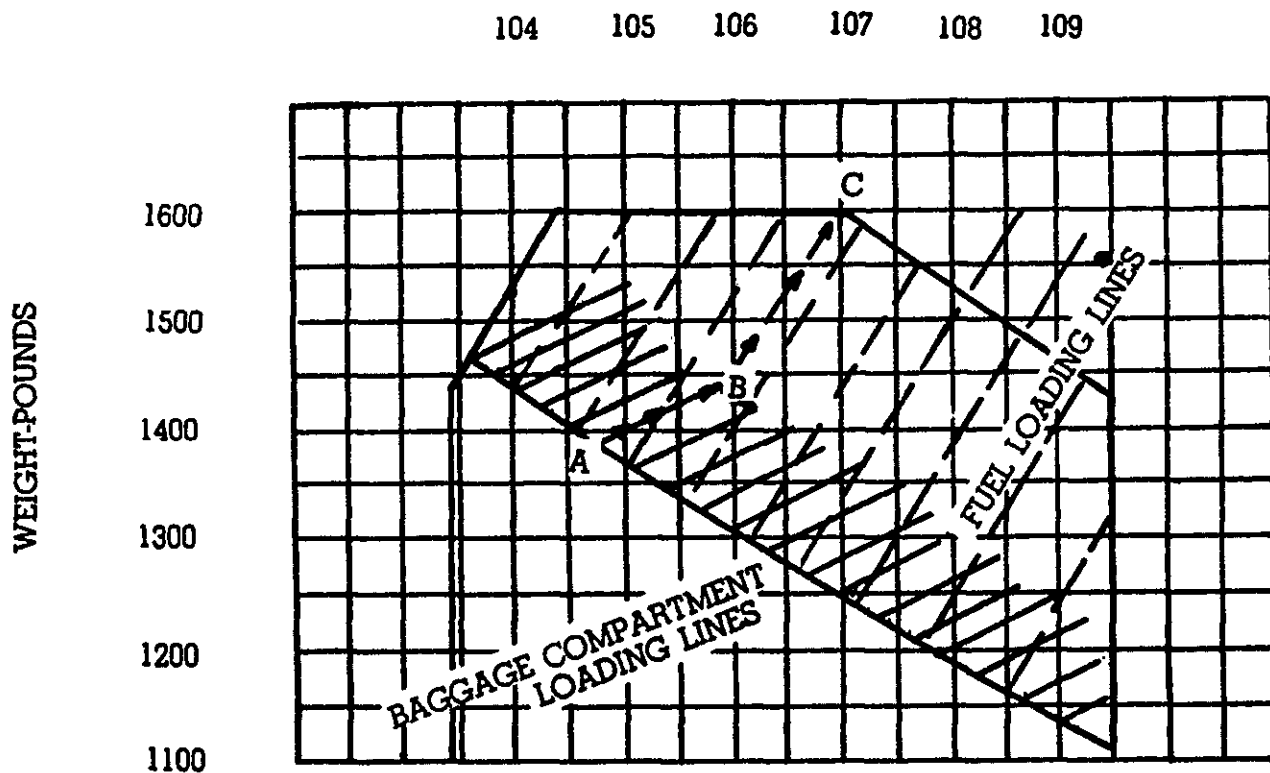
FIGURE 41.—Loading chart.
