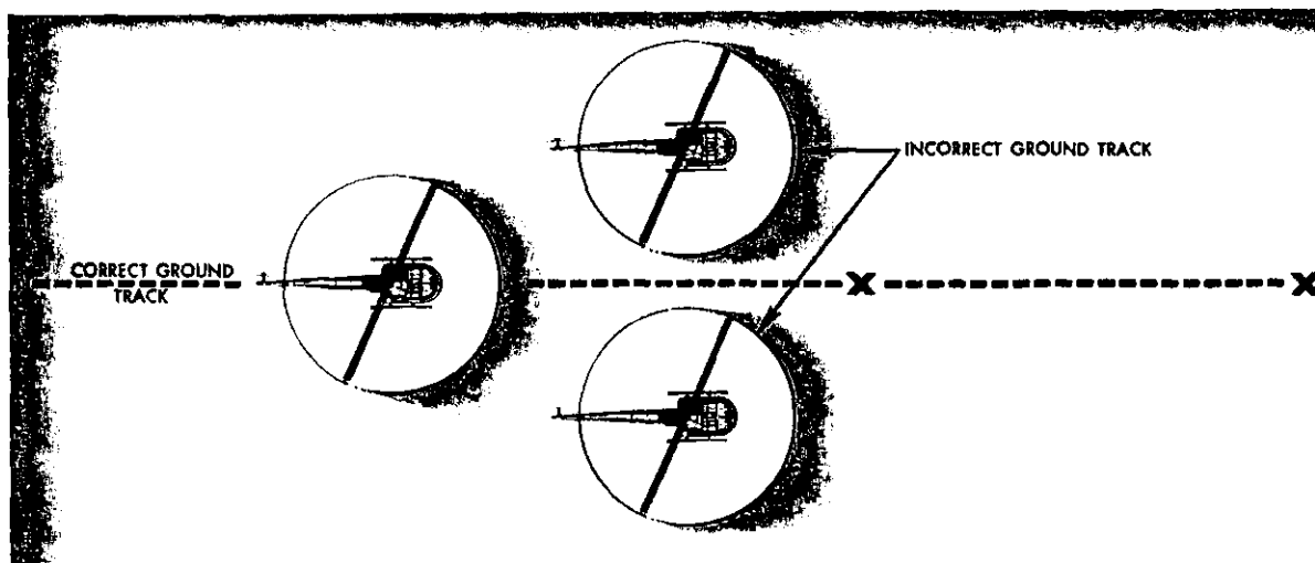
FIGURE 68.—Use of reference points in maintaining proper ground track in forward or rearward hovering flight.
