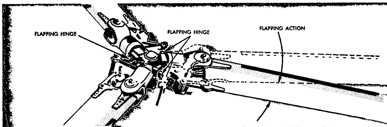
FIGURE 16.—Flapping action about the flapping hinges. Drag hinges can also be seen.
