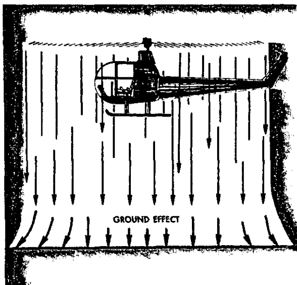
FIGURE 21.—Ground effect results from the cushion of denser air built up between the ground and helicopter by the air displaced downward by the rotor.
