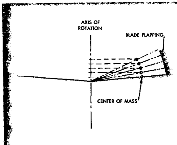
FIGURE 19.—Coriolis effect is the change in blade velocity to compensate for the change in distance of the center of mass from the axis of rotation as the blades flap.
